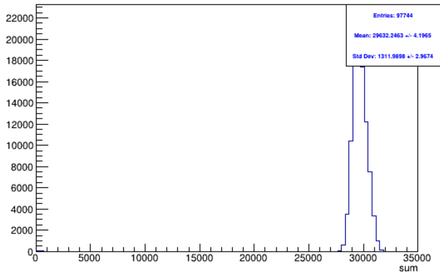
Run 5251 triggerwise, sums: All
