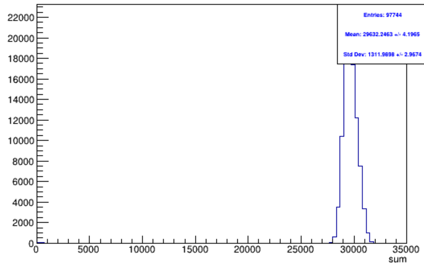
Run 5251 triggerwise, sums: Beam OFF
