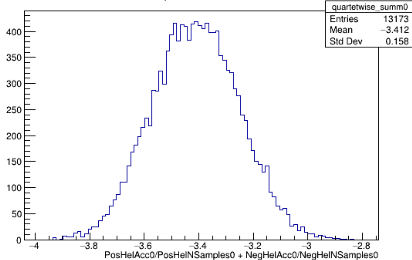
Run 5252 quartetwise, Sums0: All
