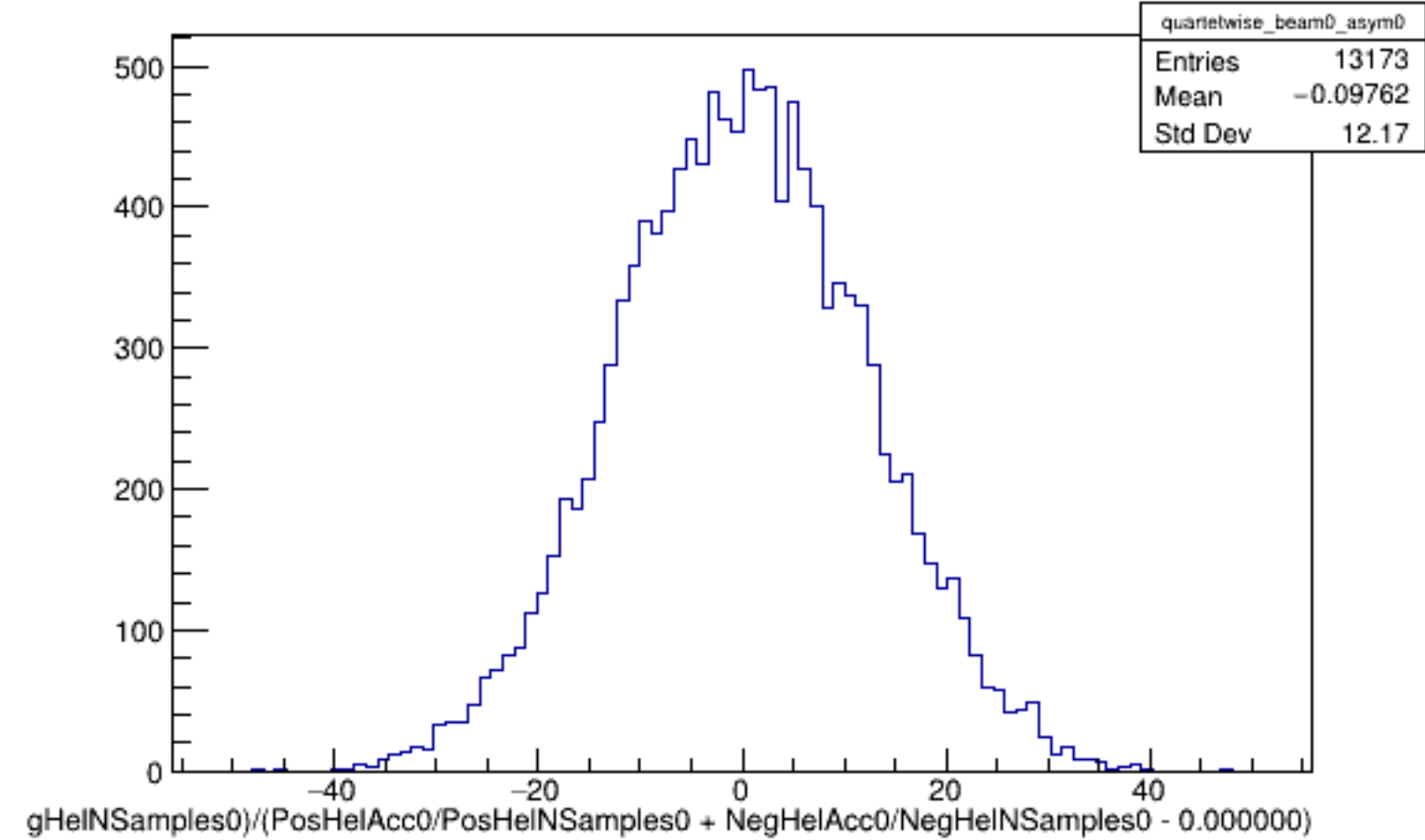
Run 5252 quartetwise, Asyms0 (Raw): Beam OFF
