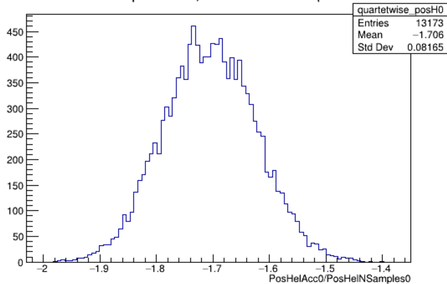
Run 5252 quartetwise, PosHelAcc0/NSamples0: All
