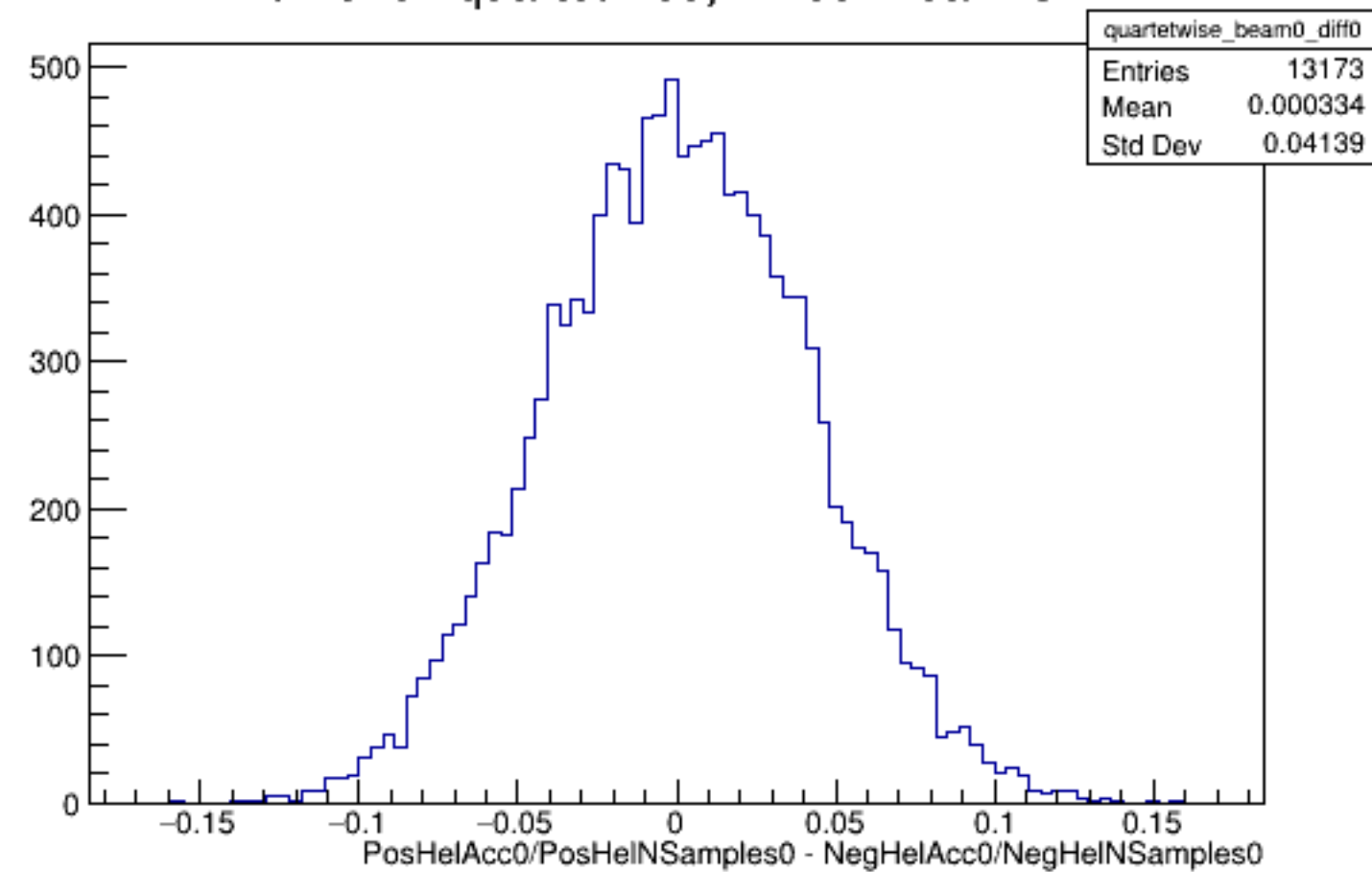
Run 5252 quartetwise, Diffs0: Beam OFF
