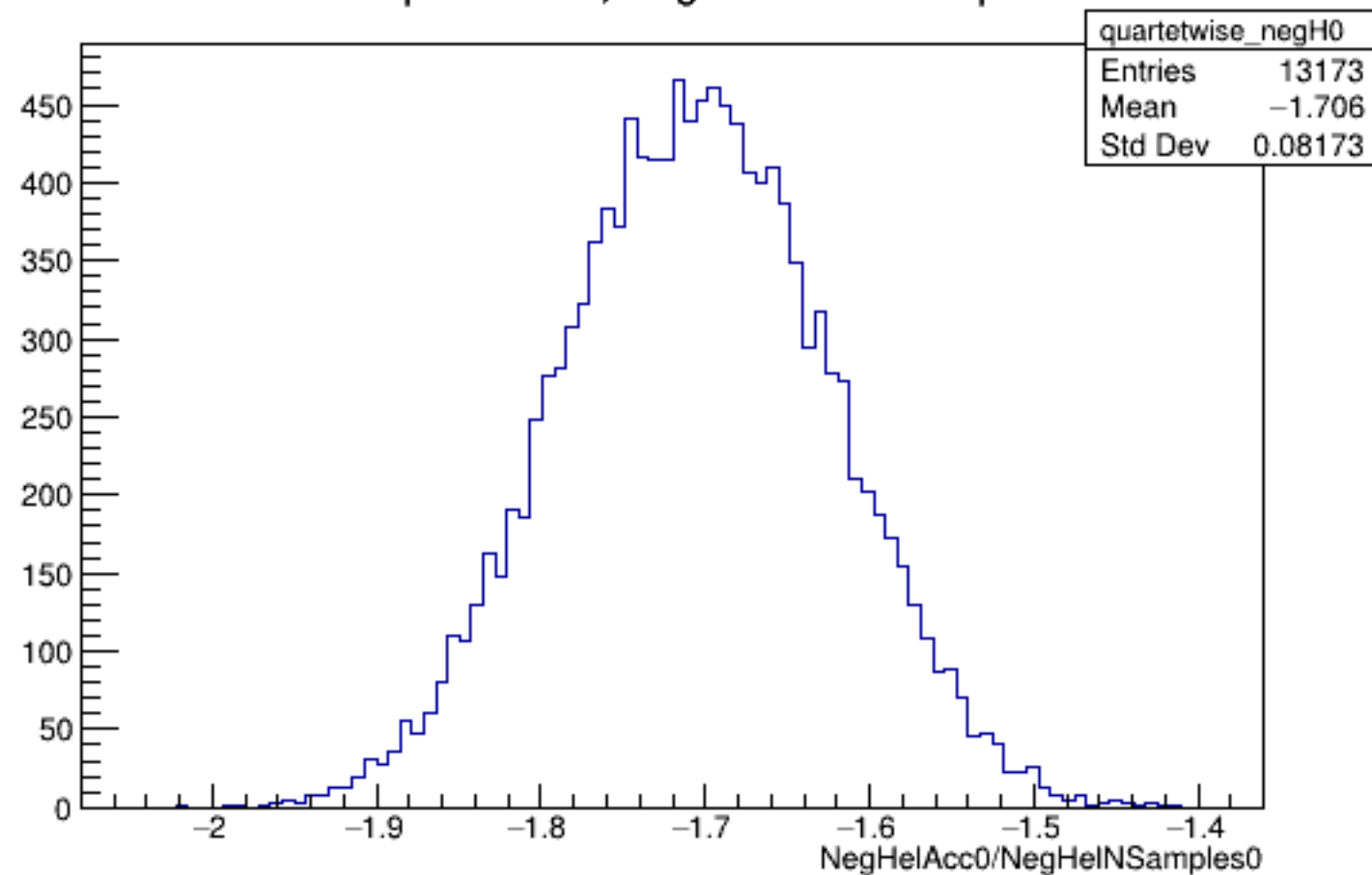
Run 5252 quartetwise, NegHelAcc0/NSamples0: All
