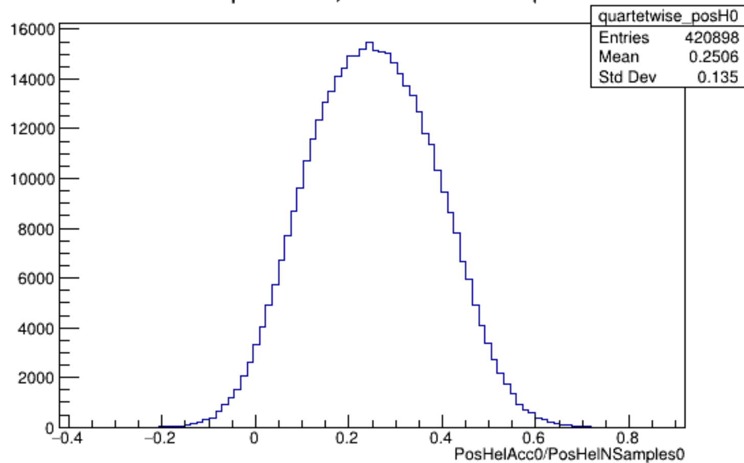
Run 5265 quartetwise, PosHelAcc0/NSamples0: All
