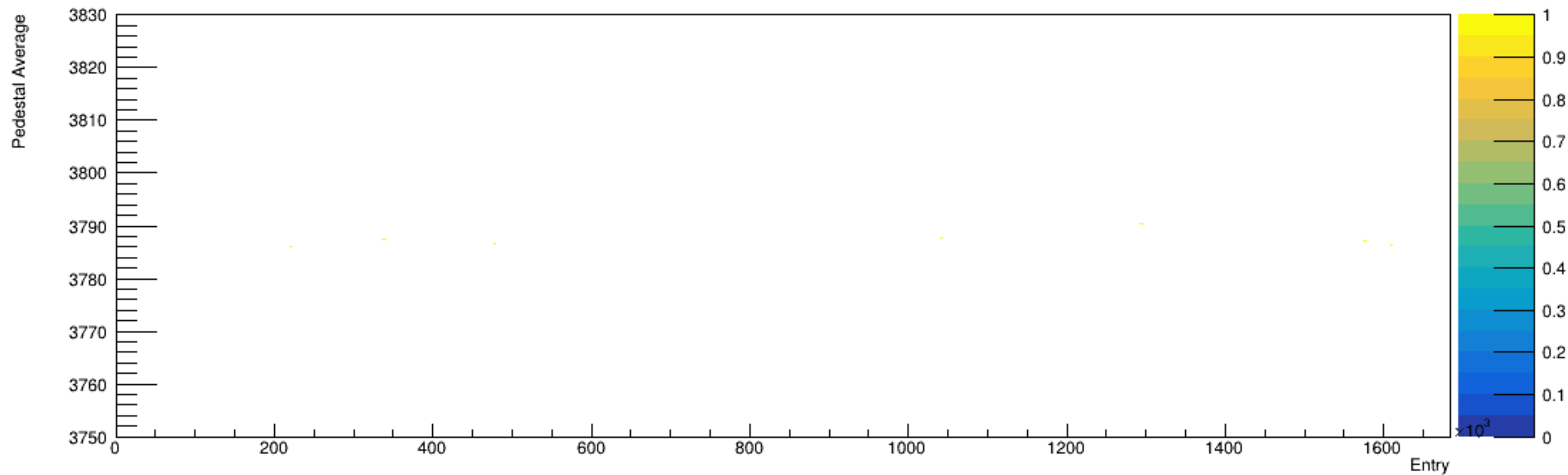
Run 5265, snapshots: Pedestal vs. Time
