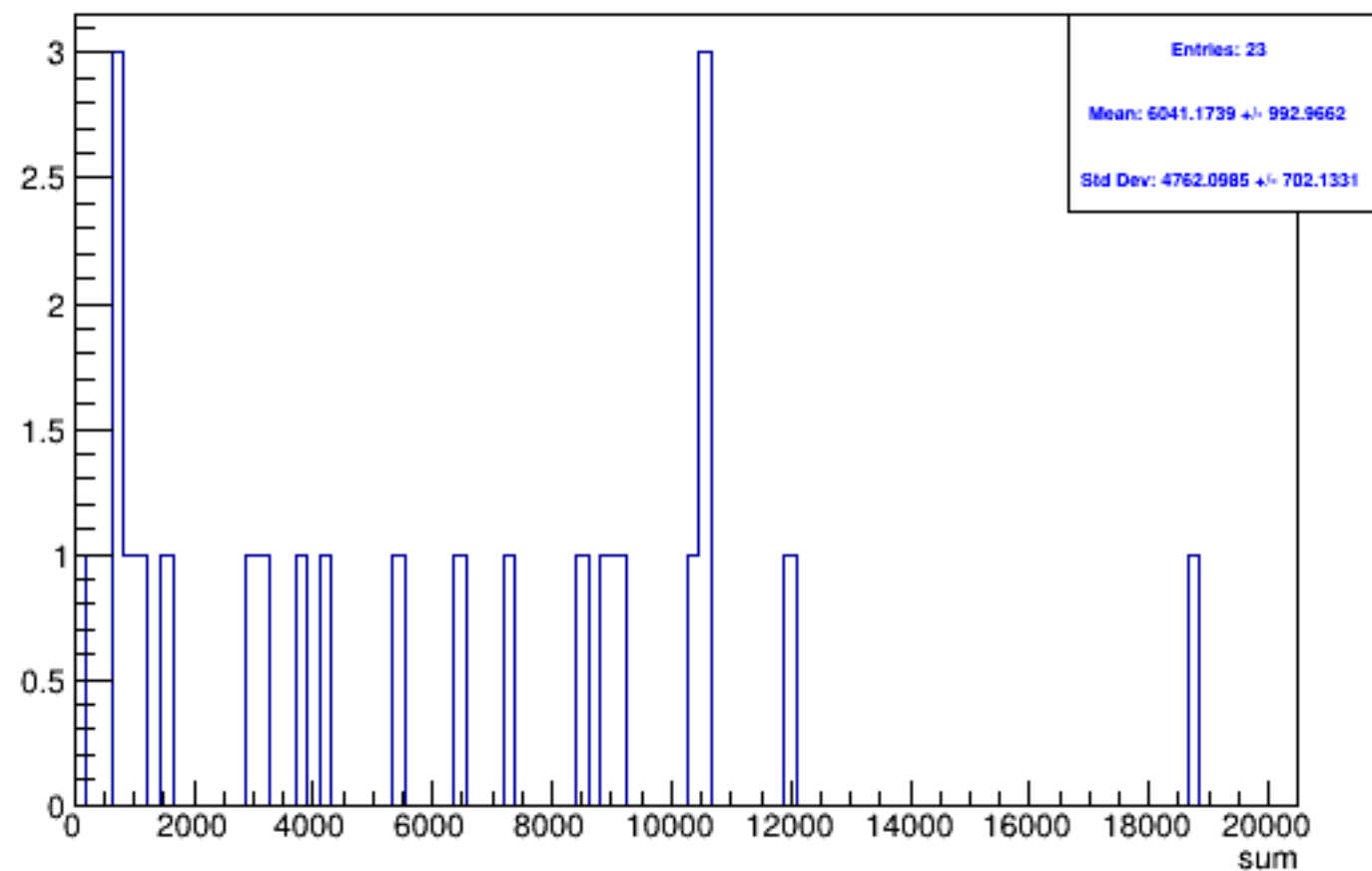
Run 5265 triggerwise, sums: All
