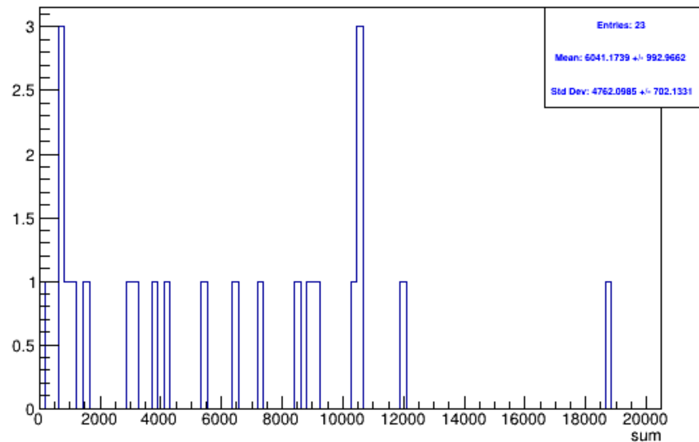
Run 5265 triggerwise, sums: Beam OFF
