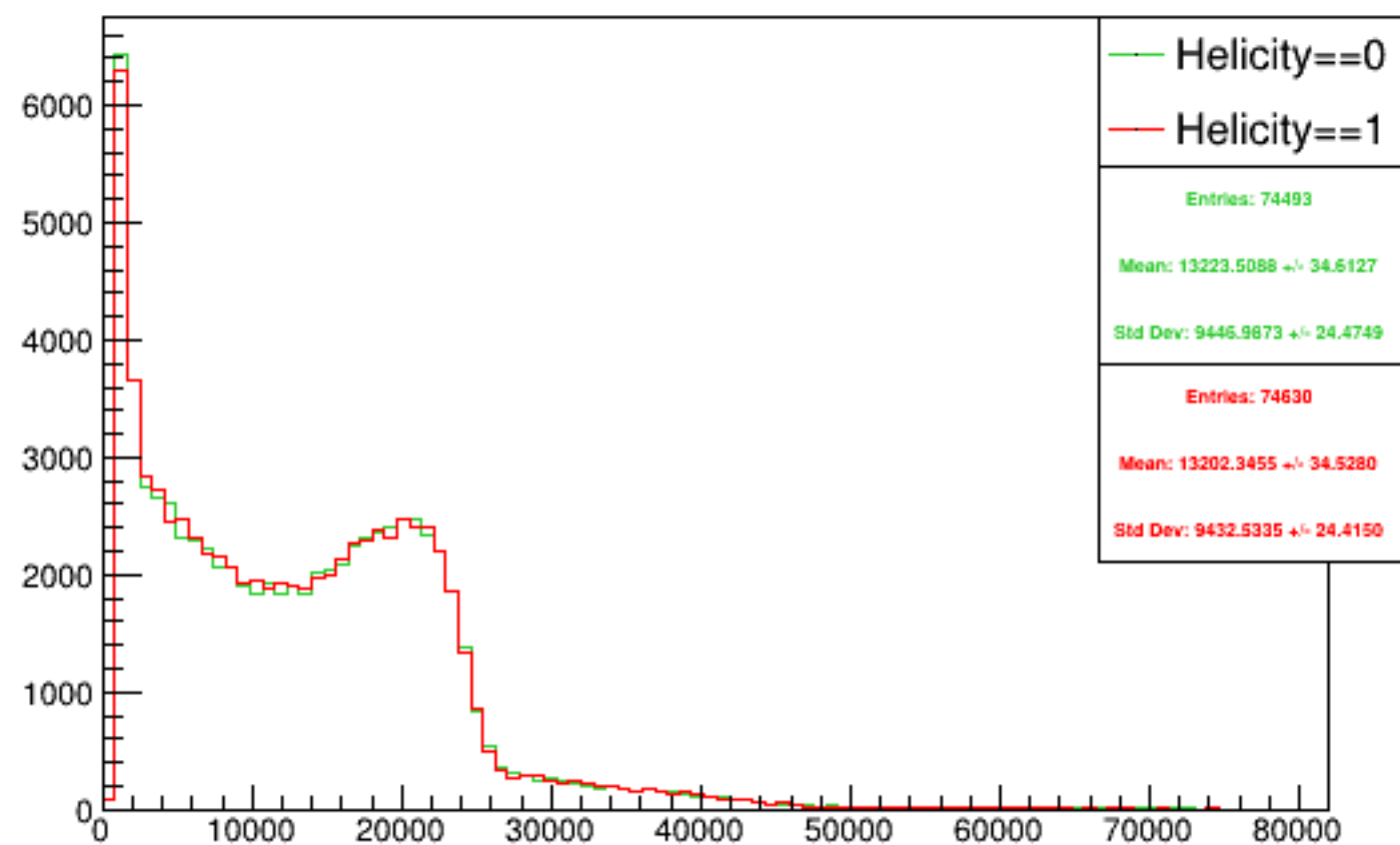
Run 5271 triggerwise, sums: Beam ON, Laser ON
