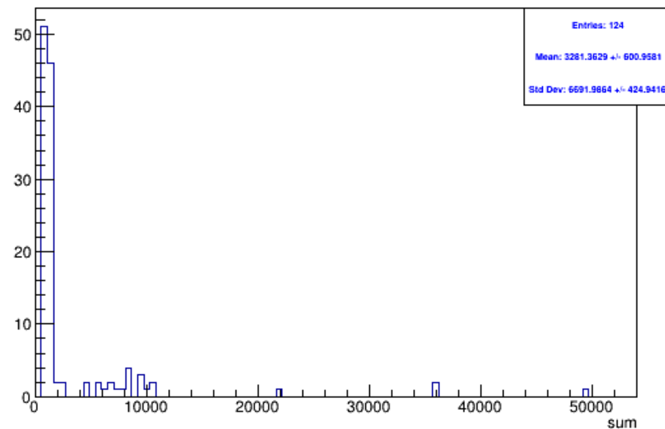
Run 5271 triggerwise, sums: Beam OFF
