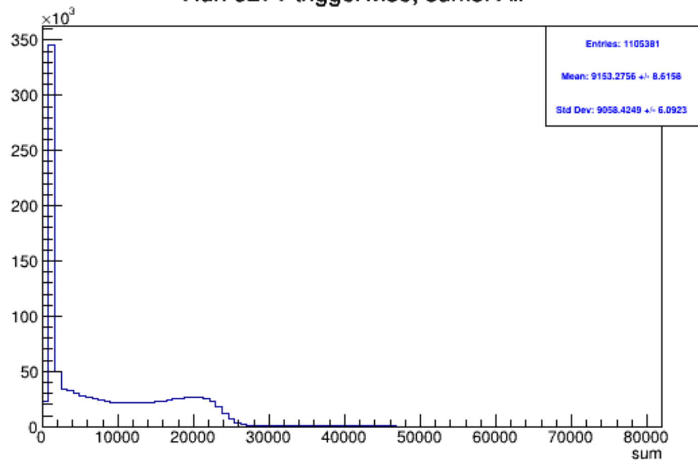
Run 5271 triggerwise, sums: All
