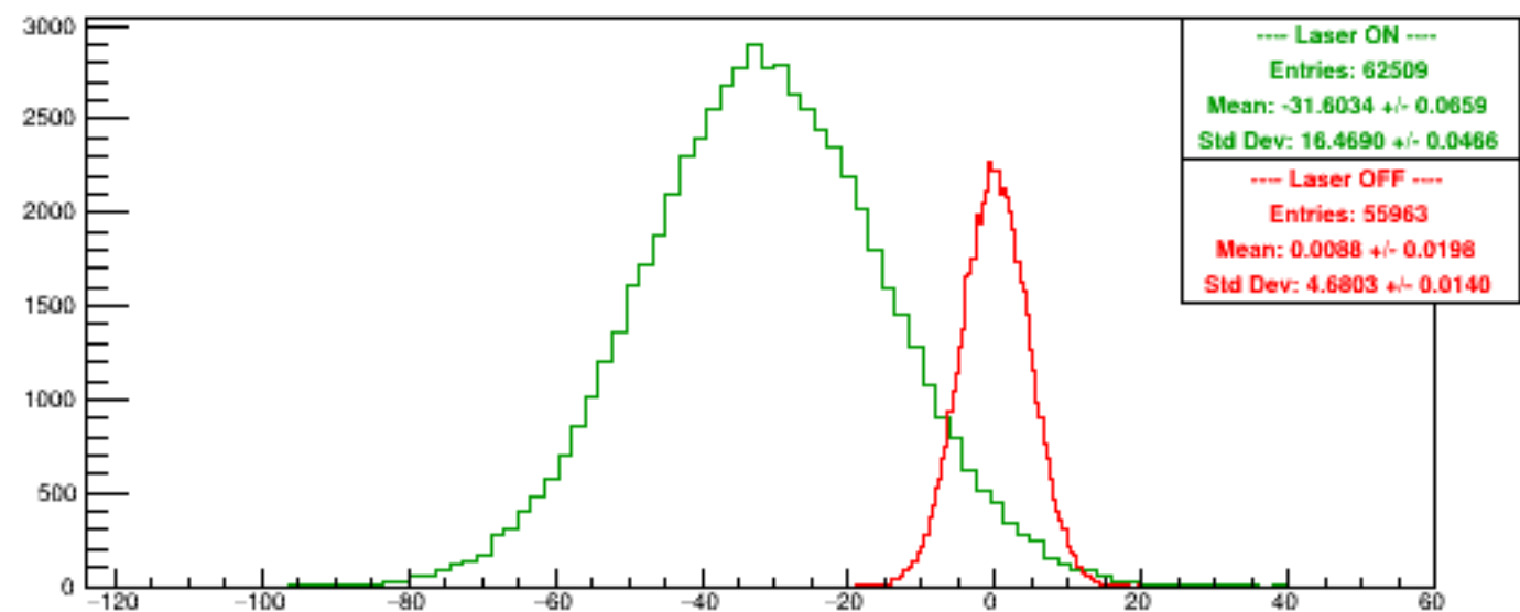
Run 5274 quartetwise, Asyms4
