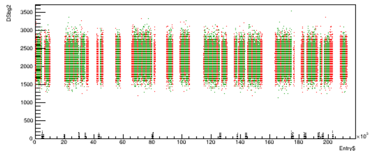
Run 5274 quartetwise, DSbg2 vs time
