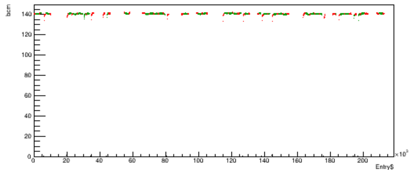
Run 5274 quartetwise, posH4 vs time
