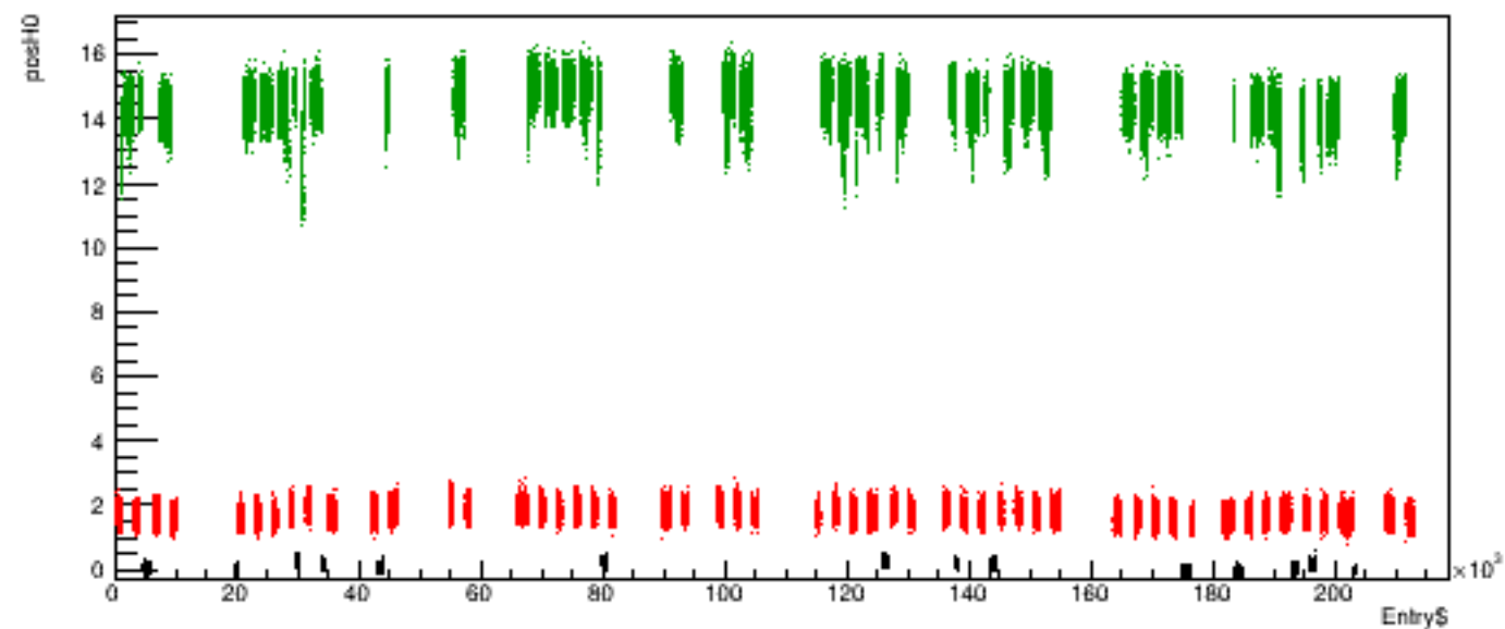
Run 5274 quartetwise, posH0 vs time
