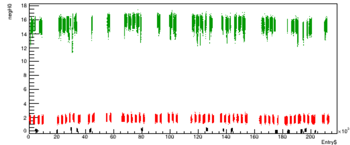
Run 5274 quartetwise, negH0 vs time
