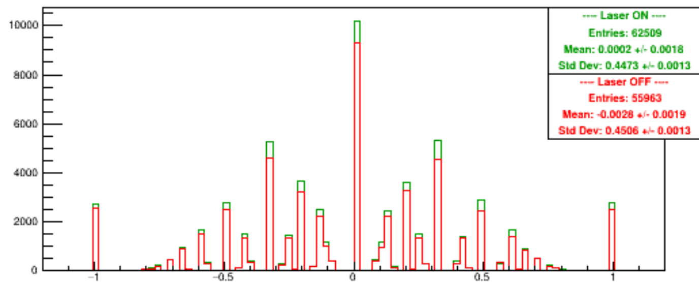
Run 5274 quartetwise, Asyms USbg1
