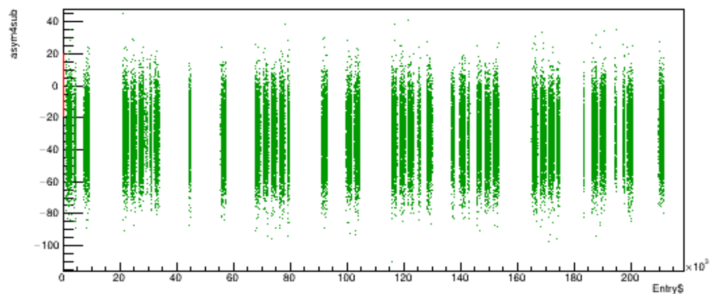
Run 5274 quartetwise, asym4sub vs time
