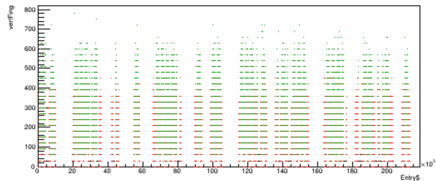
Run 5274 quartetwise, vertFing vs time
