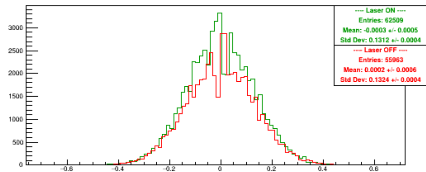
Run 5274 quartetwise, Asyms DSbg1
