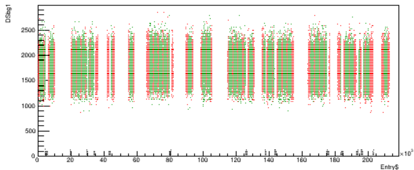
Run 5274 quartetwise, DSbg1 vs time
