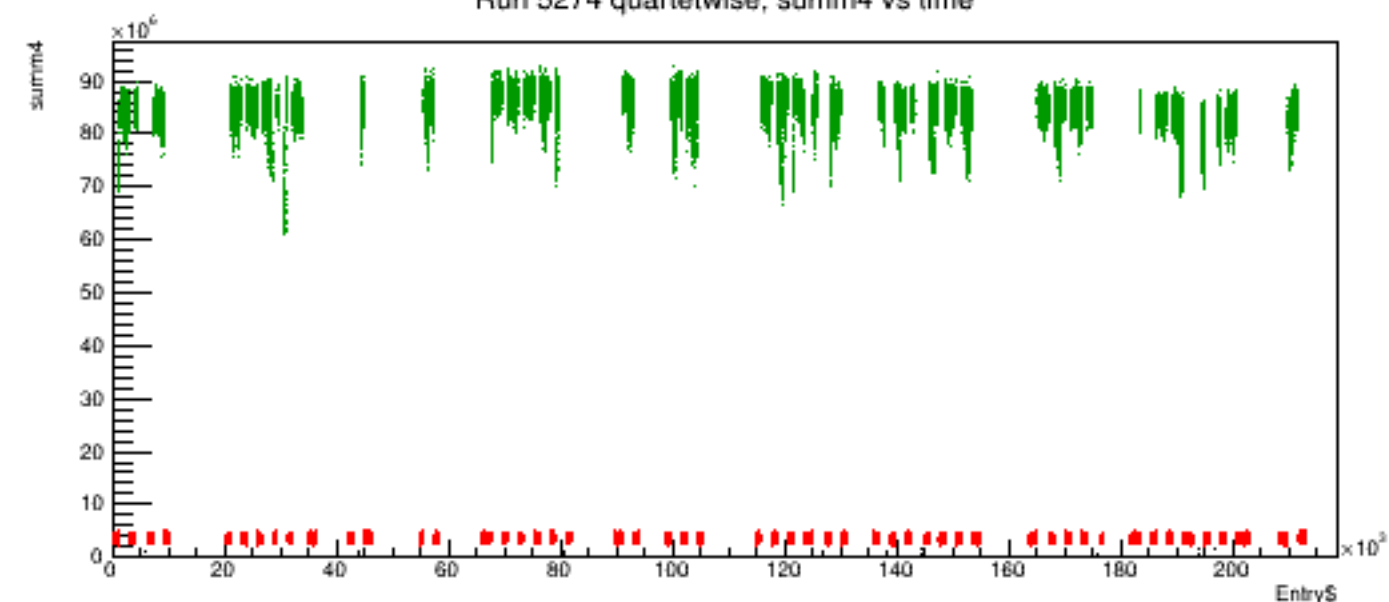
Run 5274 quartetwise, summ4 vs time
