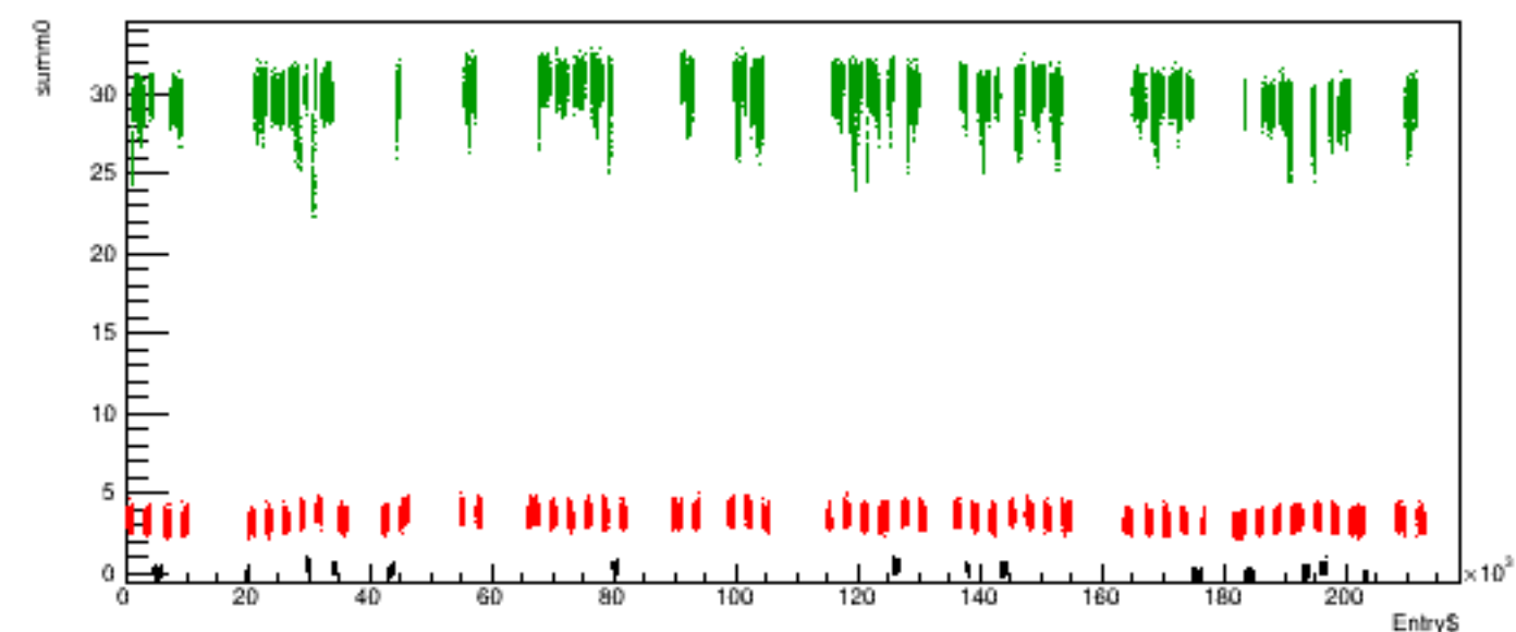
Run 5274 quartetwise, summ0 vs time
