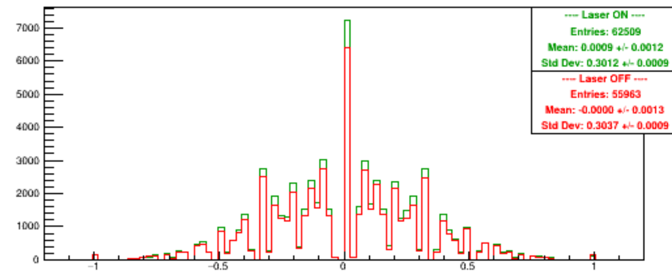
Run 5274 quartetwise, Asyms USbg2
