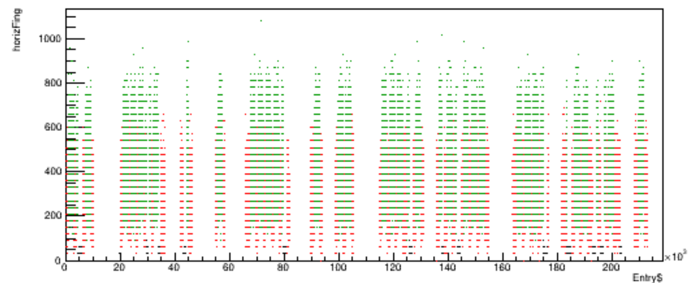
Run 5274 quartetwise, horizFing vs time
