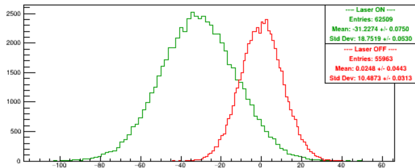
Run 5274 quartetwise, Asyms0
