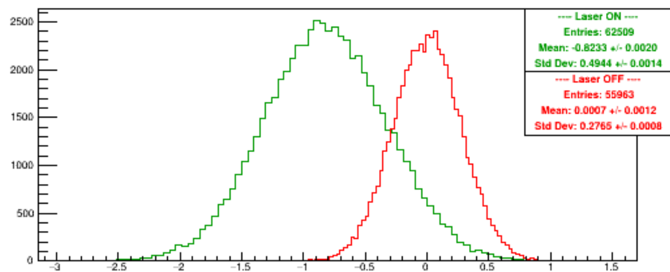
Run 5274 quartetwise, Diffs0
