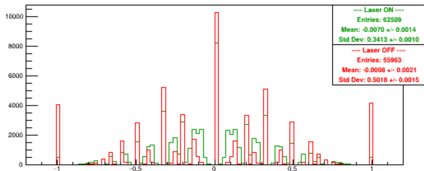
Run 5274 quartetwise, Asyms Horiz Finger
