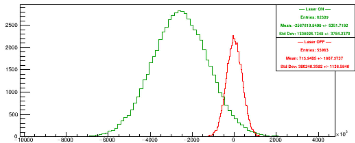
Run 5274 quartetwise, Diffs4
