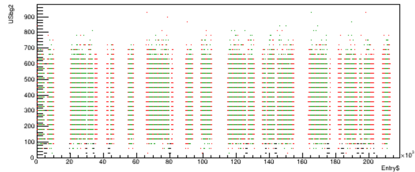
Run 5274 quartetwise, USbg2 vs time
