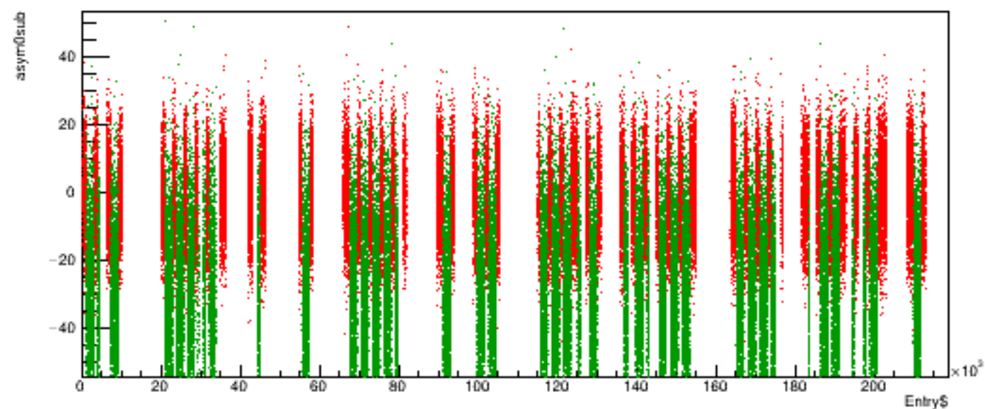
Run 5274 quartetwise, asym0sub vs time
