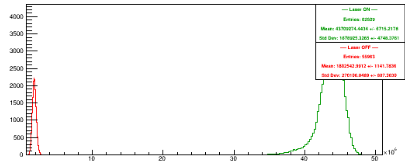
Run 5274 quartetwise, NegHelAcc4
