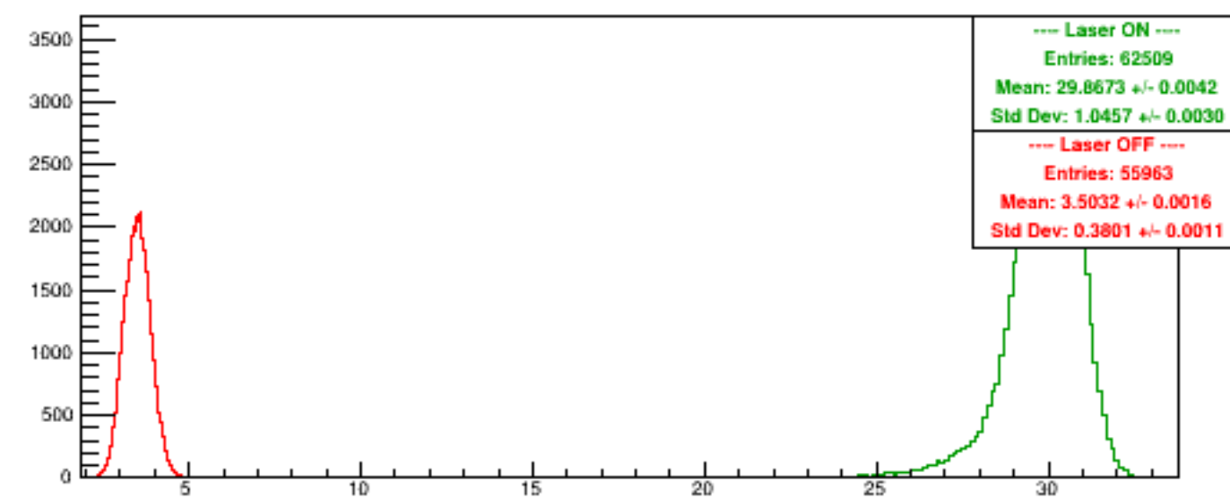
Run 5274 quartetwise, Sums0
