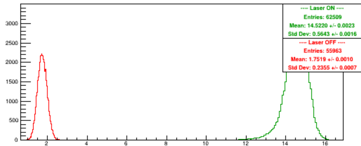
Run 5274 quartetwise, PosHelAcc0/NSamples0
