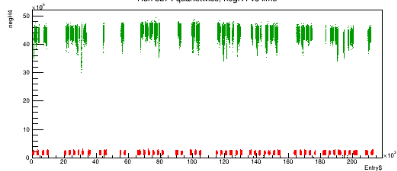
Run 5274 quartetwise, negH4 vs time
