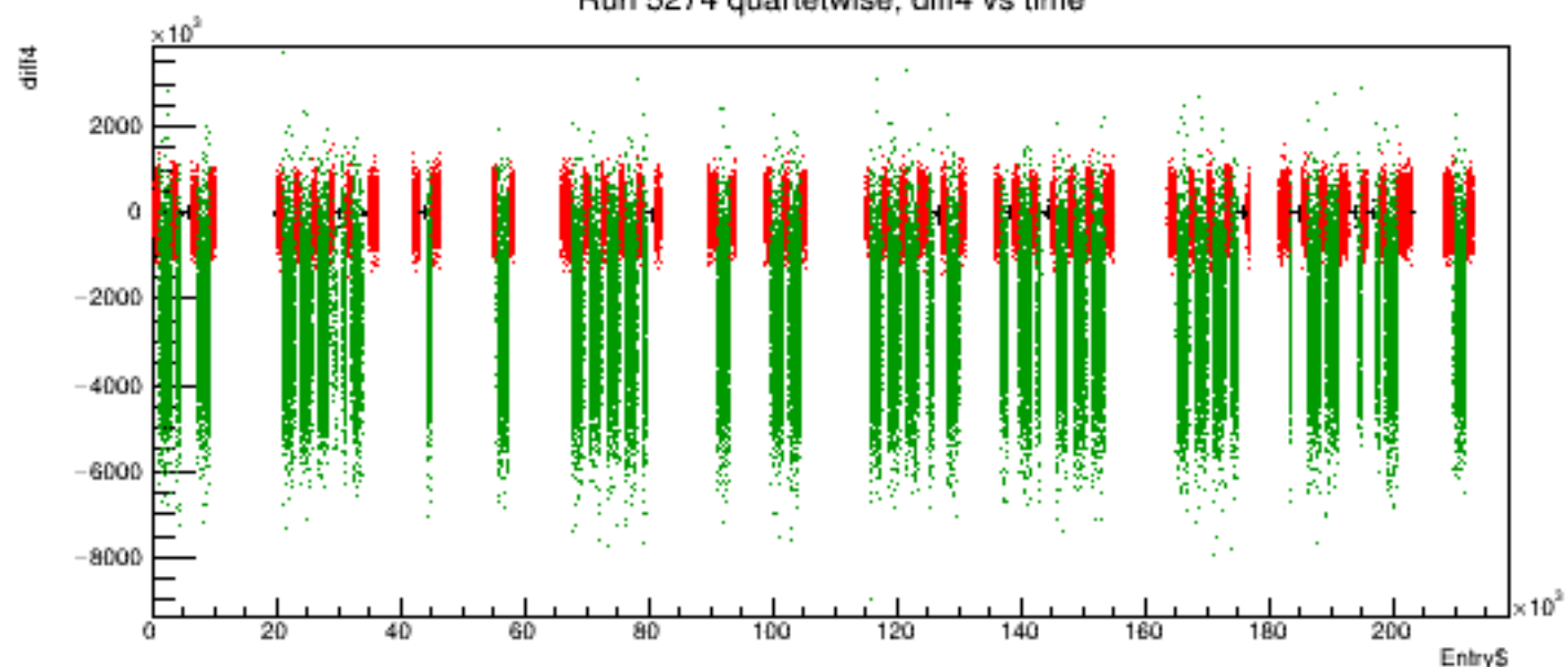
Run 5274 quartetwise, diff4 vs time
