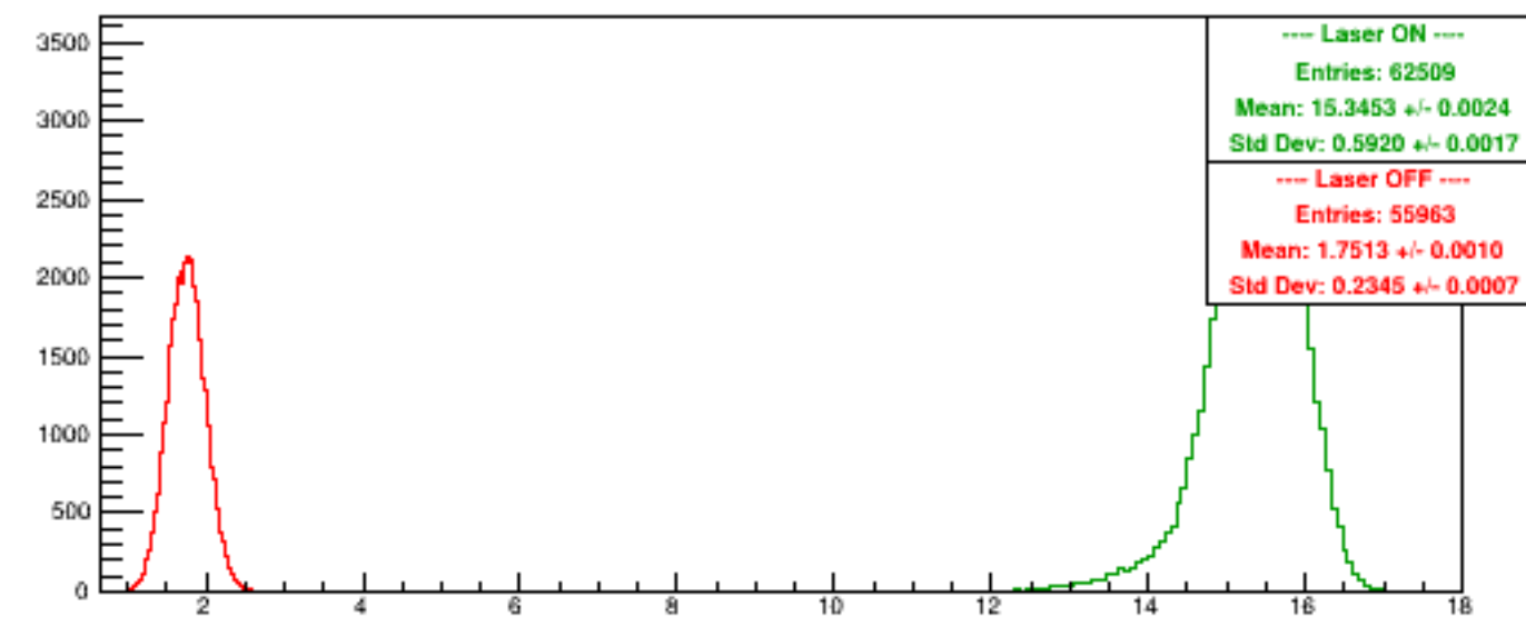
Run 5274 quartetwise, NegHelAcc0/NSamples0
