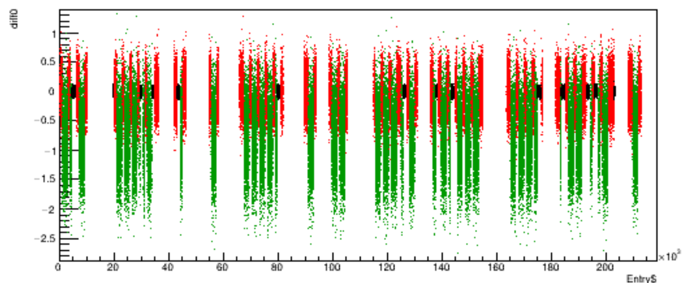
Run 5274 quartetwise, diff0 vs time
