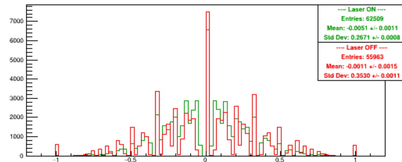
Run 5274 quartetwise, Asyms Vert Finger
