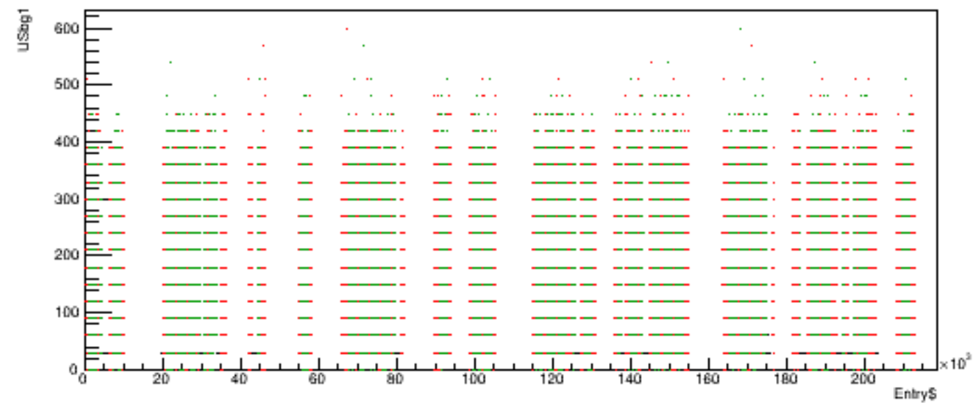
Run 5274 quartetwise, USbg1 vs time
