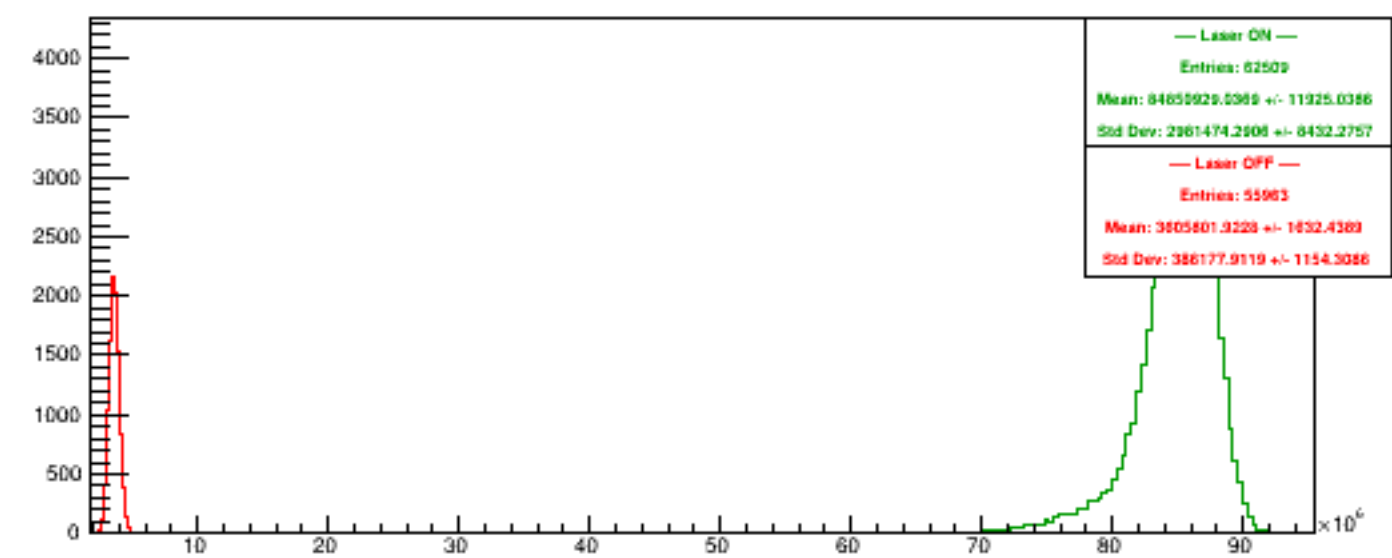
Run 5274 quartetwise, Sums4
