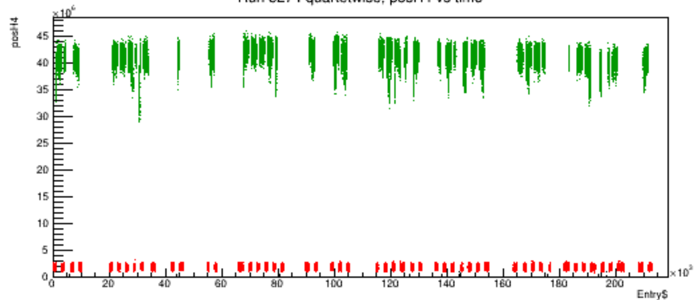
Run 5274 quartetwise, posH4 vs time
