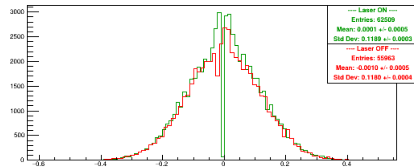
Run 5274 quartetwise, Asyms DSbg2
