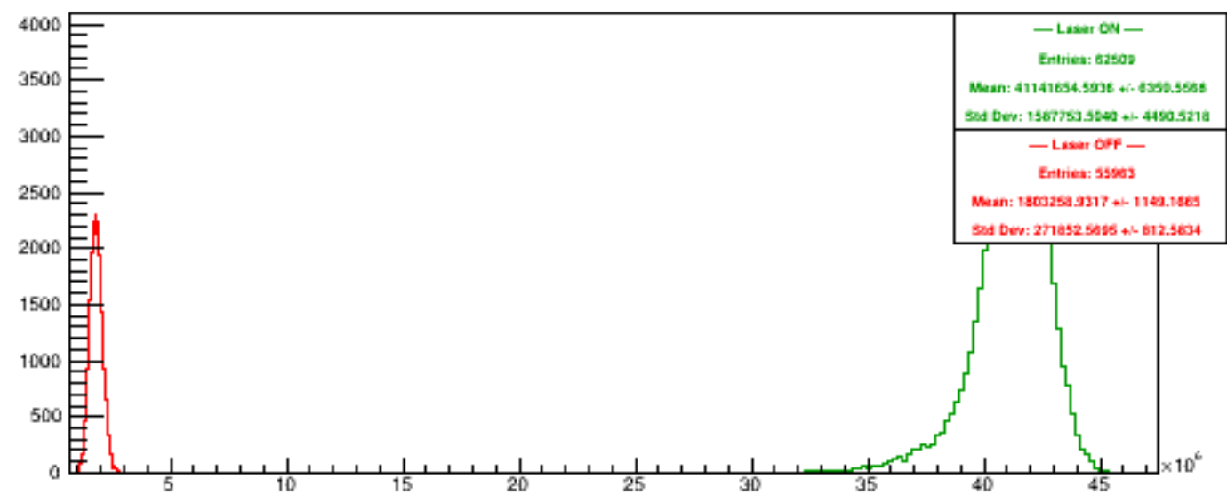
Run 5274 quartetwise, PosHelAcc4
