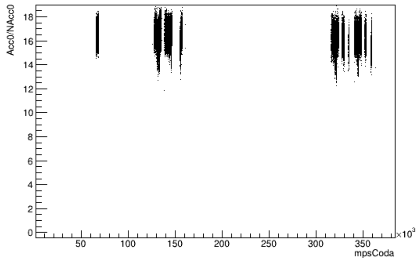
Run 5277 mpwise, Acc0 vs Time: Beam ON, Laser ON
