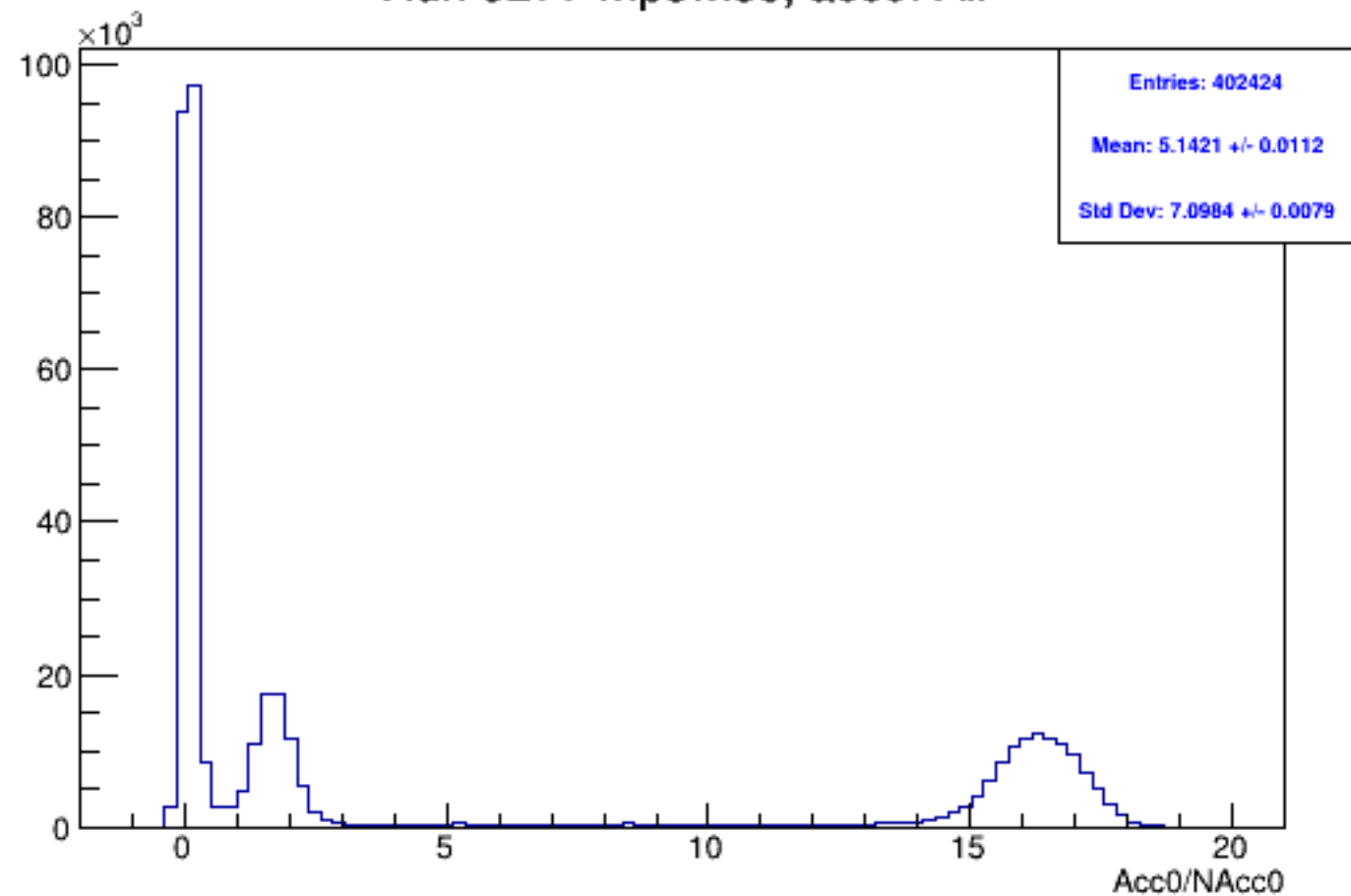
Run 5277 mpwise, acc0: All
