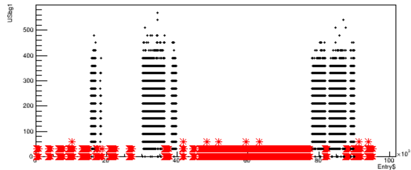
Run 5277, quartetwise: USbg1 vs time
