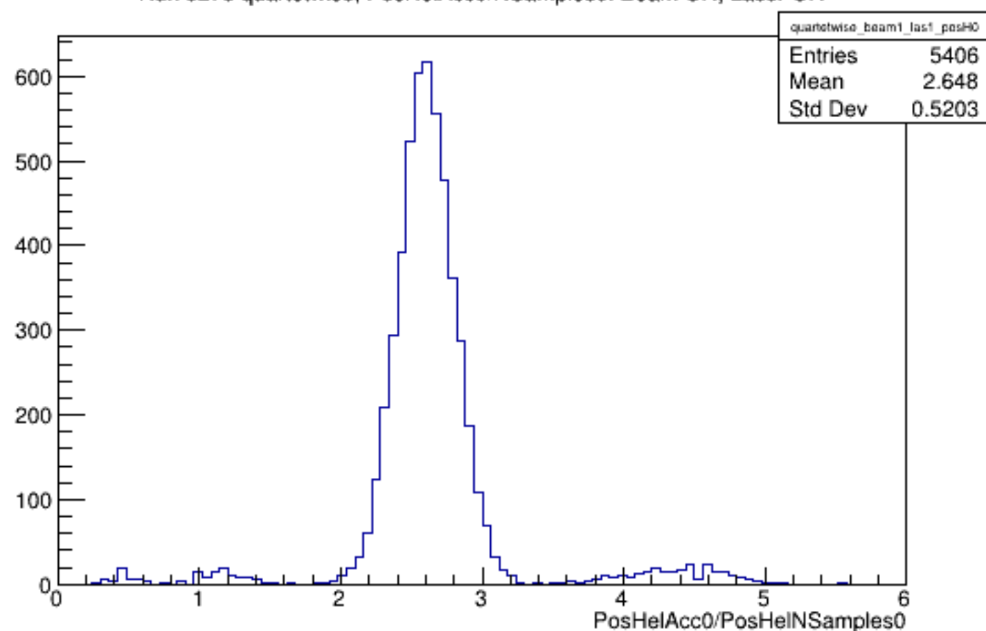
Run 5278 quartetwise, PosHelAcc0/NSamples0: Beam ON, Laser ON
