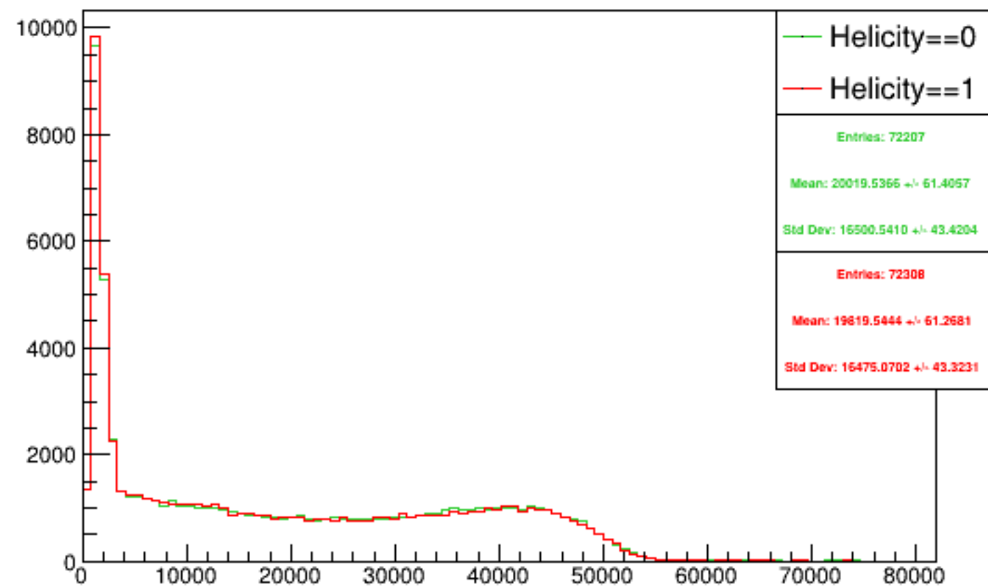
Run 5278 triggerwise, sums: Beam ON, Laser ON
