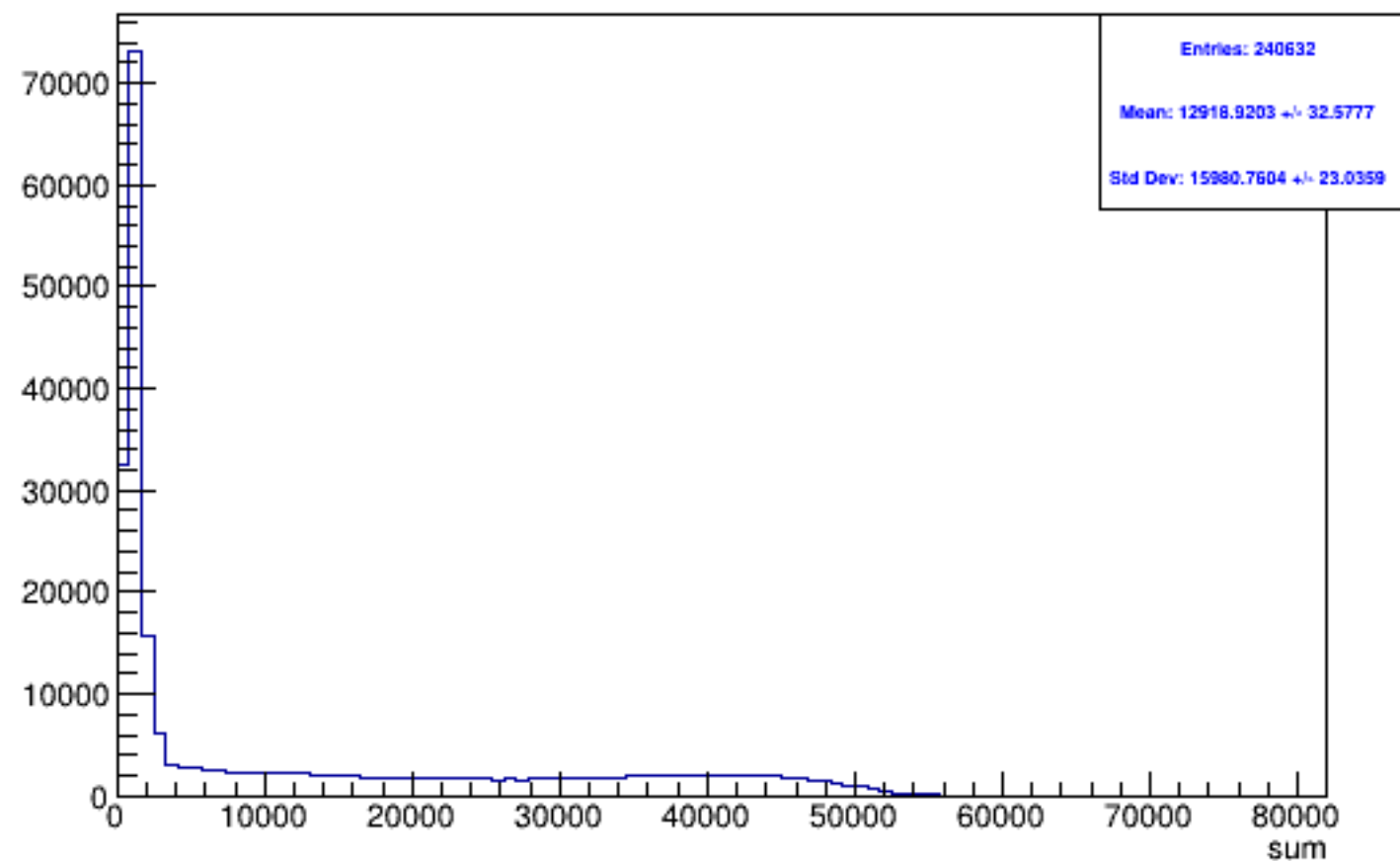
Run 5278 triggerwise, sums: All
