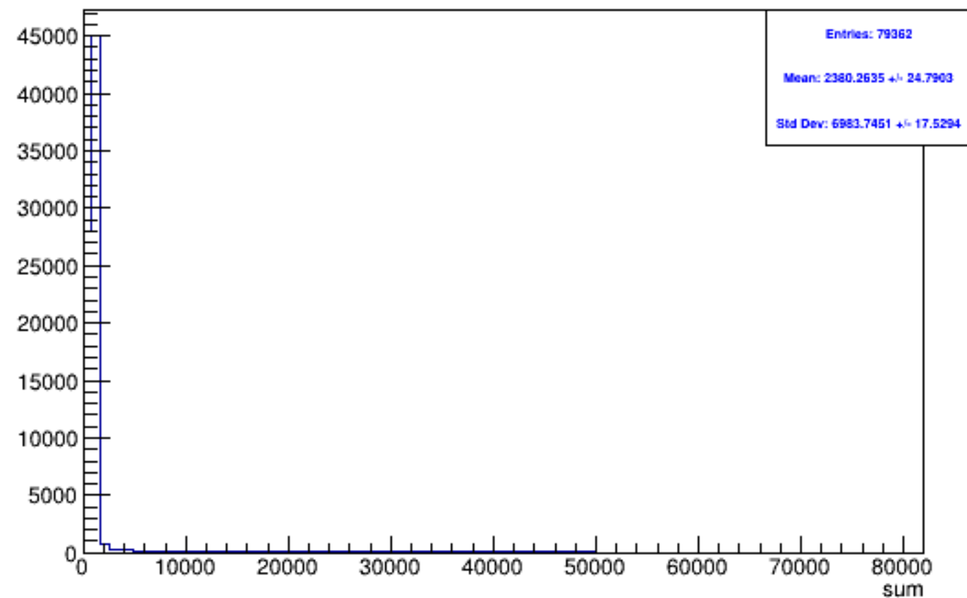
Run 5278 triggerwise, sums: Beam OFF
