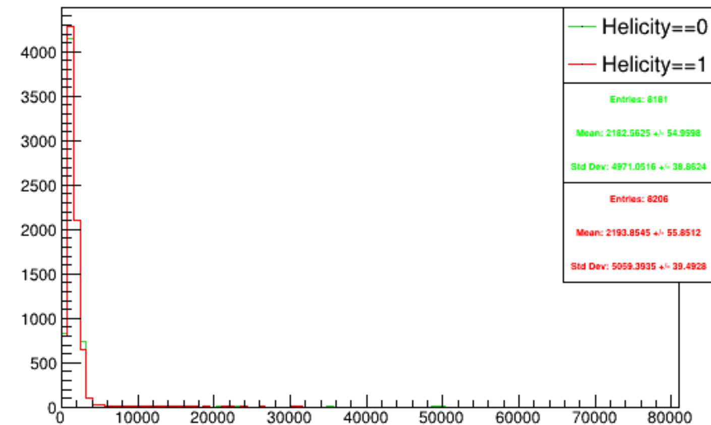
Run 5278 triggerwise, sums: Beam ON, Laser OFF
