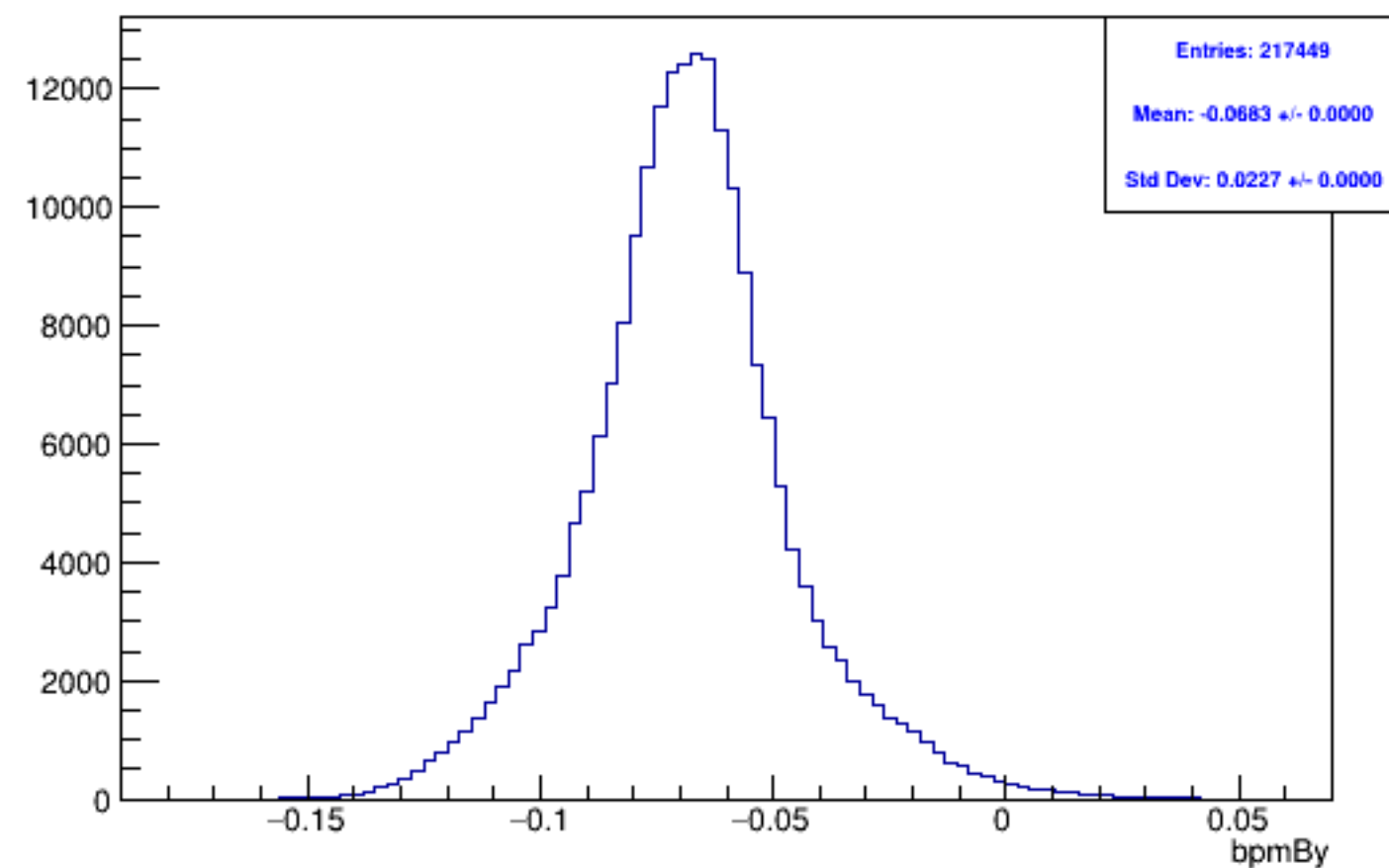
Run 5285, mpswise, bpmBy: Beam ON, Laser OFF
