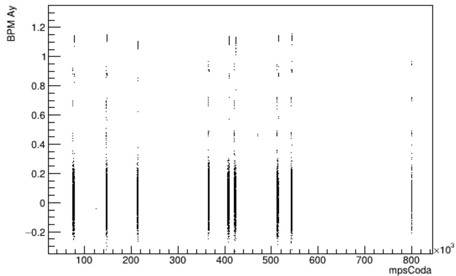
Run 5285 mpwise, beam OFF, laser ON
