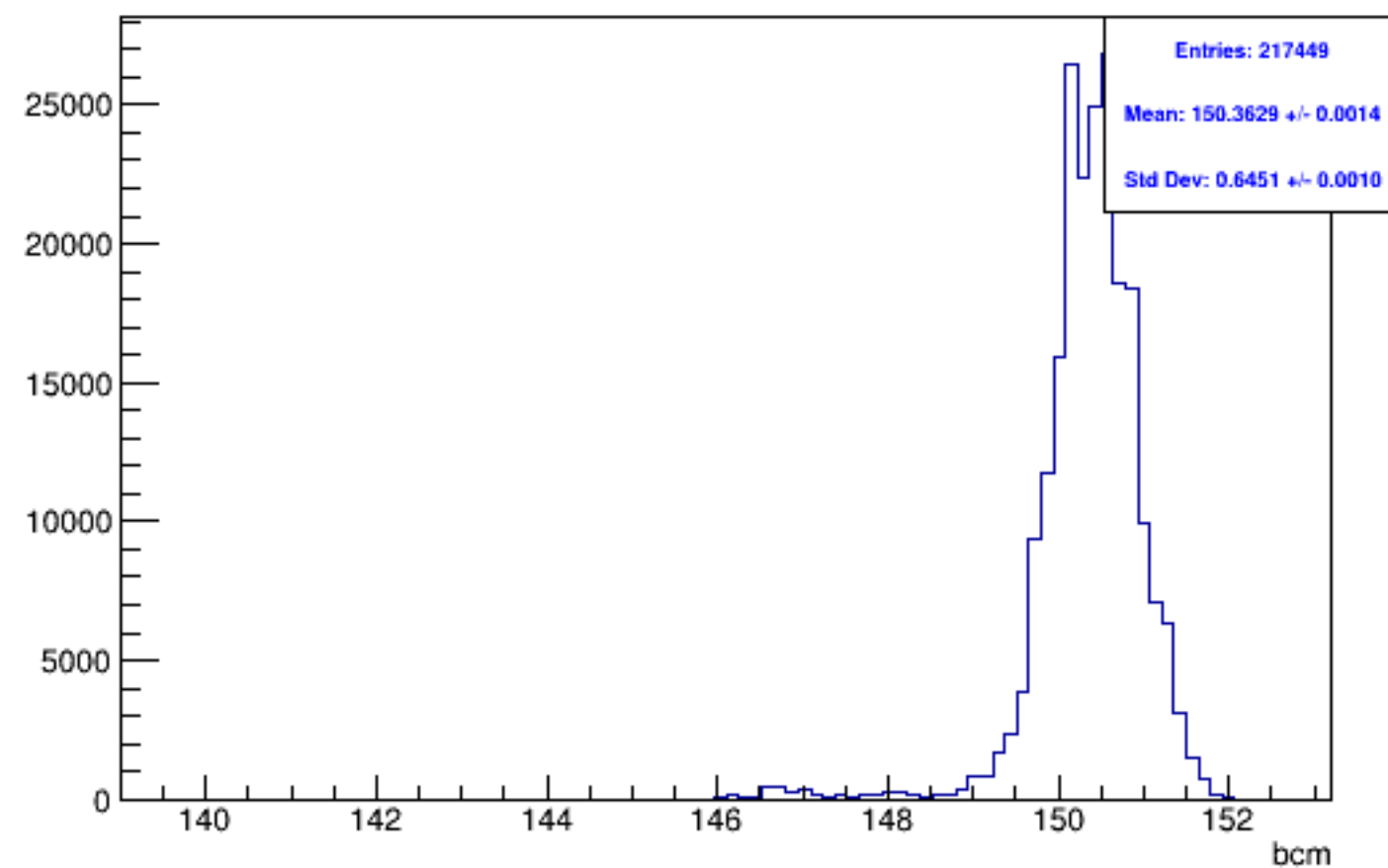
Run 5285, mpwise, BCM: Beam ON, Laser OFF
