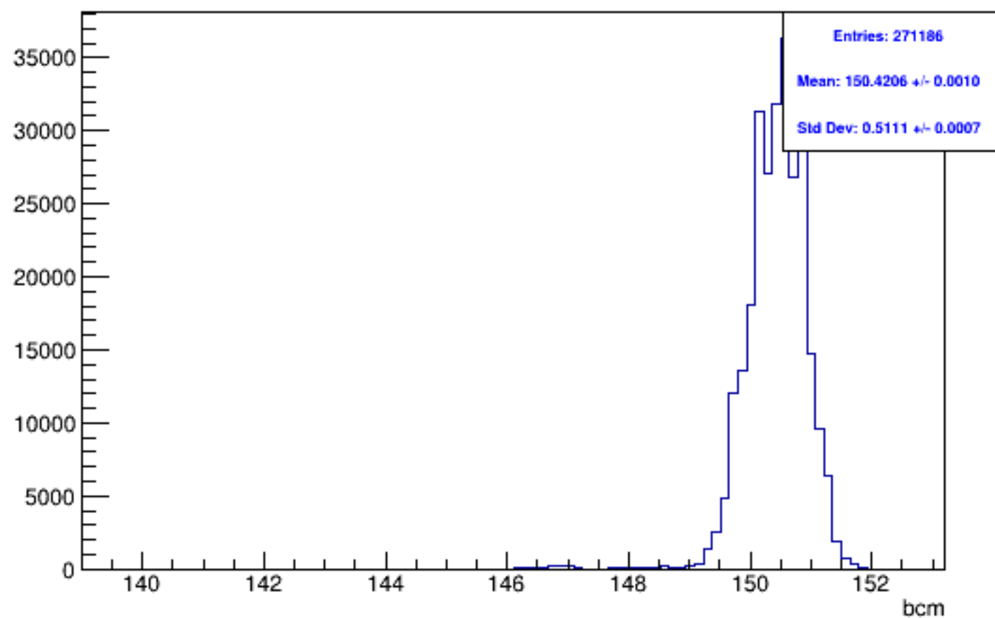
Run 5285, mpwise, BCM: Beam ON, Laser ON
