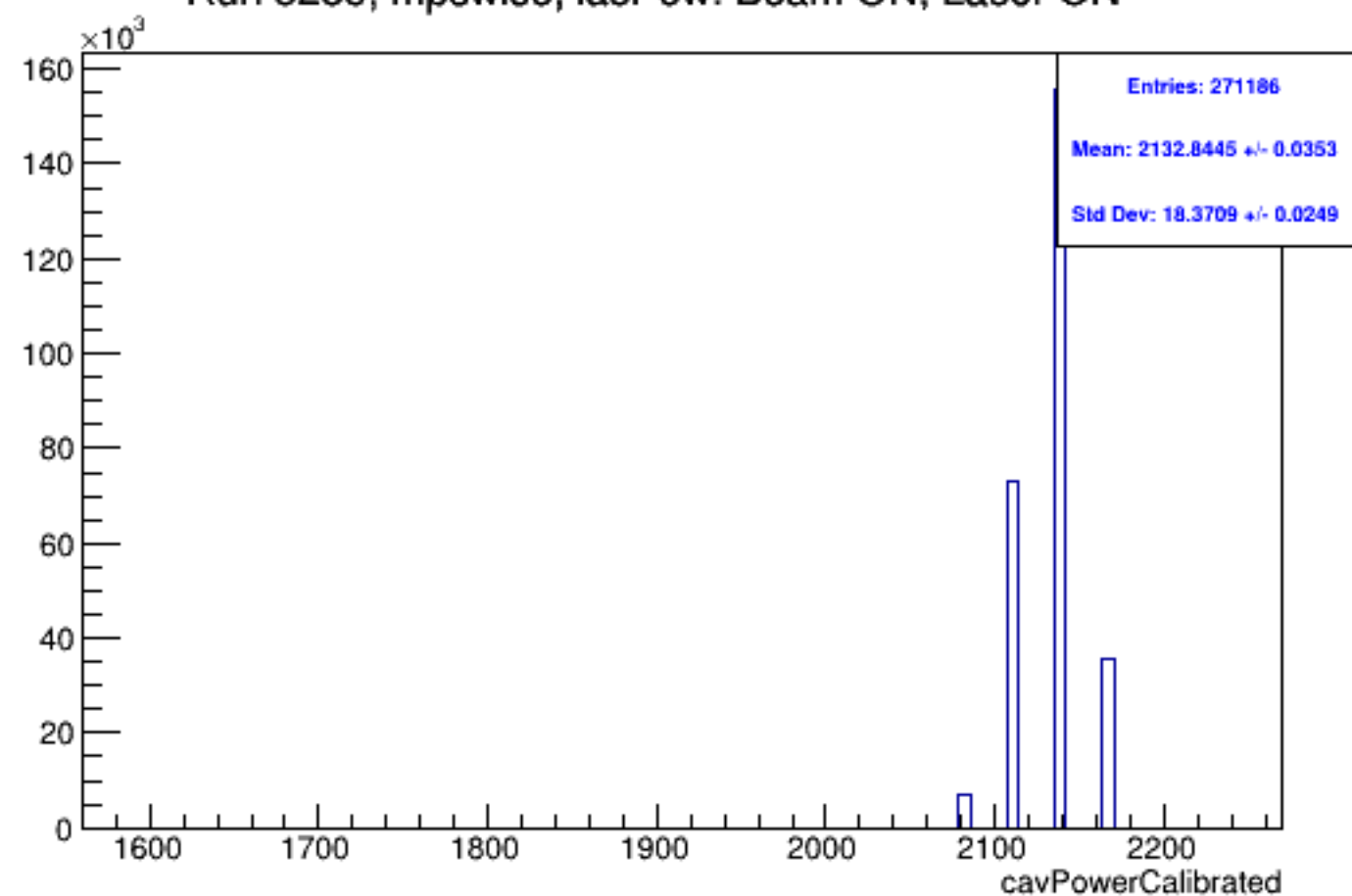
Run 5285, mpwise, lasPow: Beam ON, Laser ON
