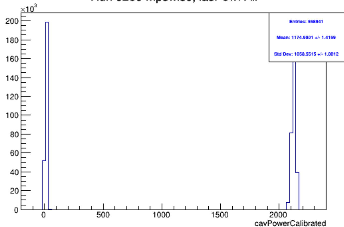
Run 5285 mpwise, lasPow: All
