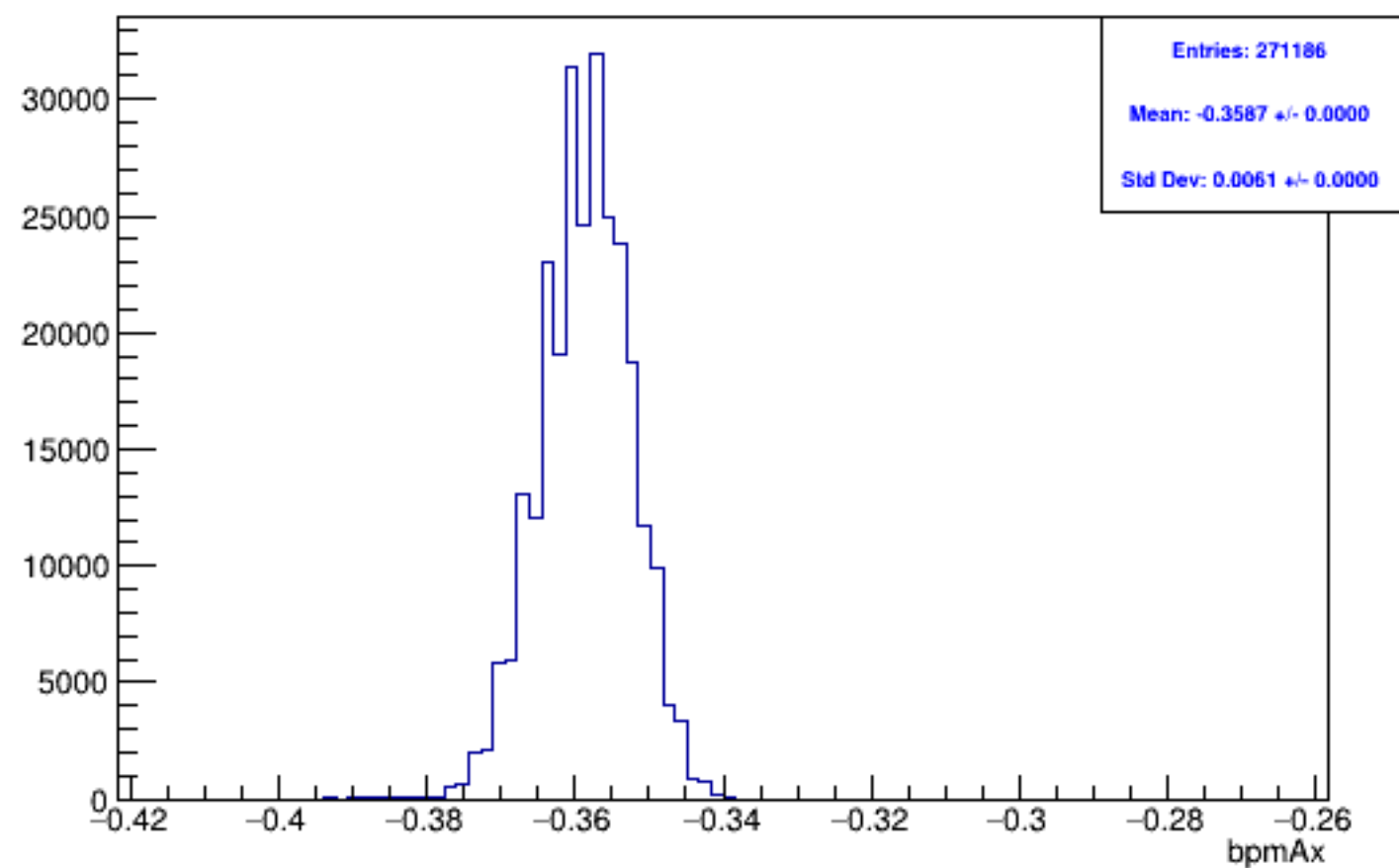
Run 5285, mpswise, bpmAx: Beam ON, Laser ON
