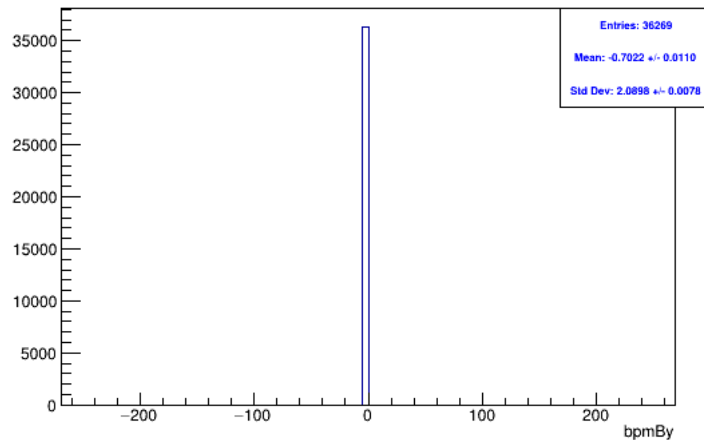
Run 5285 mpswise, bpmBy: Beam OFF
