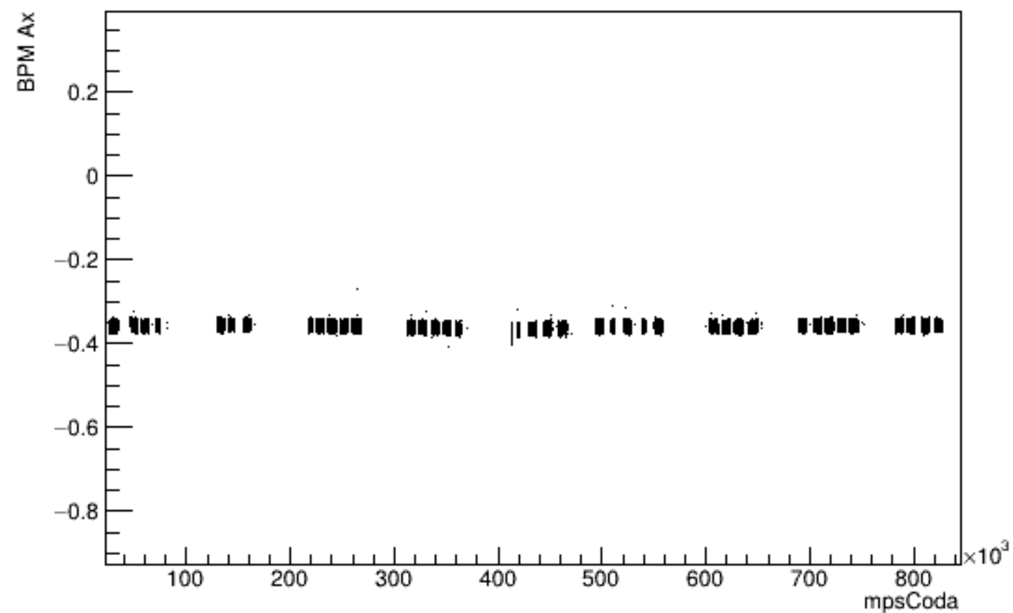
Run 5285 mpwise, beam ON, laser ON
