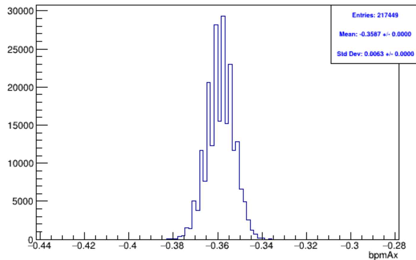
Run 5285, mpswise, bpmAx: Beam ON, Laser OFF
