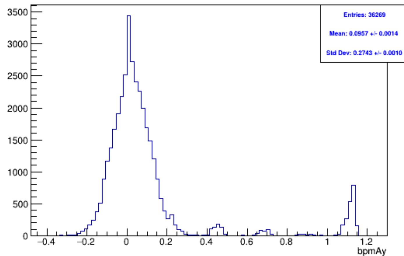
Run 5285 mpwise, bpmAy: Beam OFF
