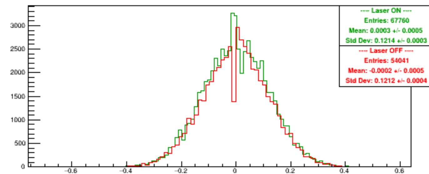
Run 5285 quartetwise, Asyms DSbg2
