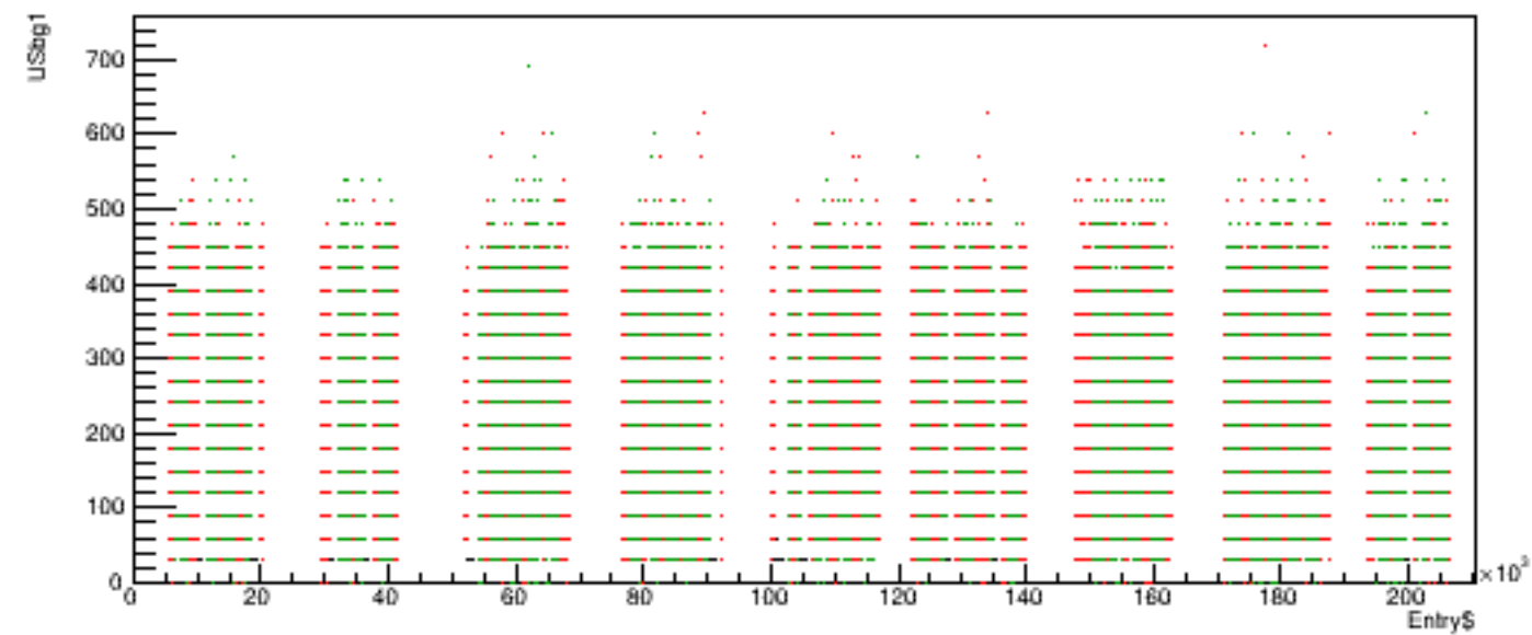
Run 5285 quartetwise, USbg1 vs time
