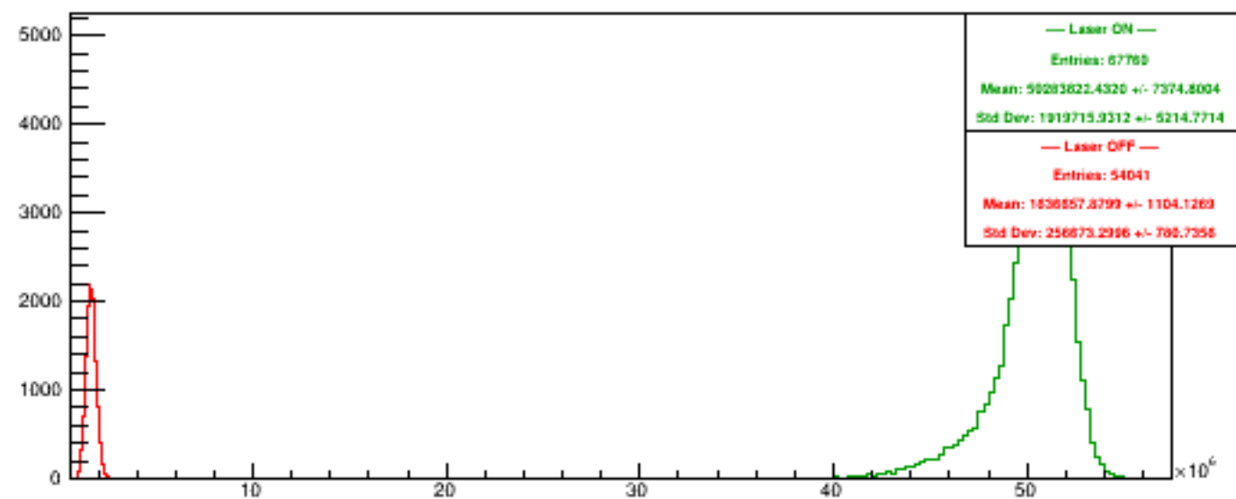
Run 5285 quartetwise, PosHelAcc4
