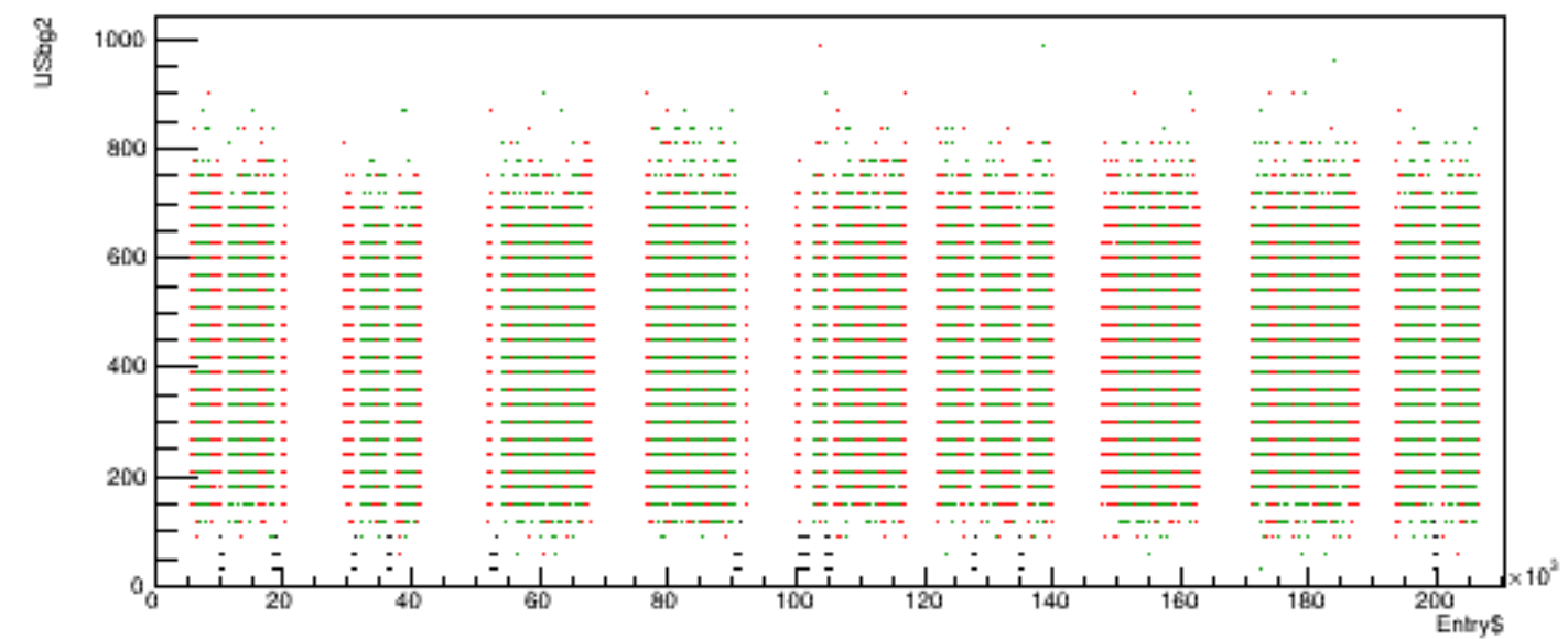
Run 5285 quartetwise, USbg2 vs time
