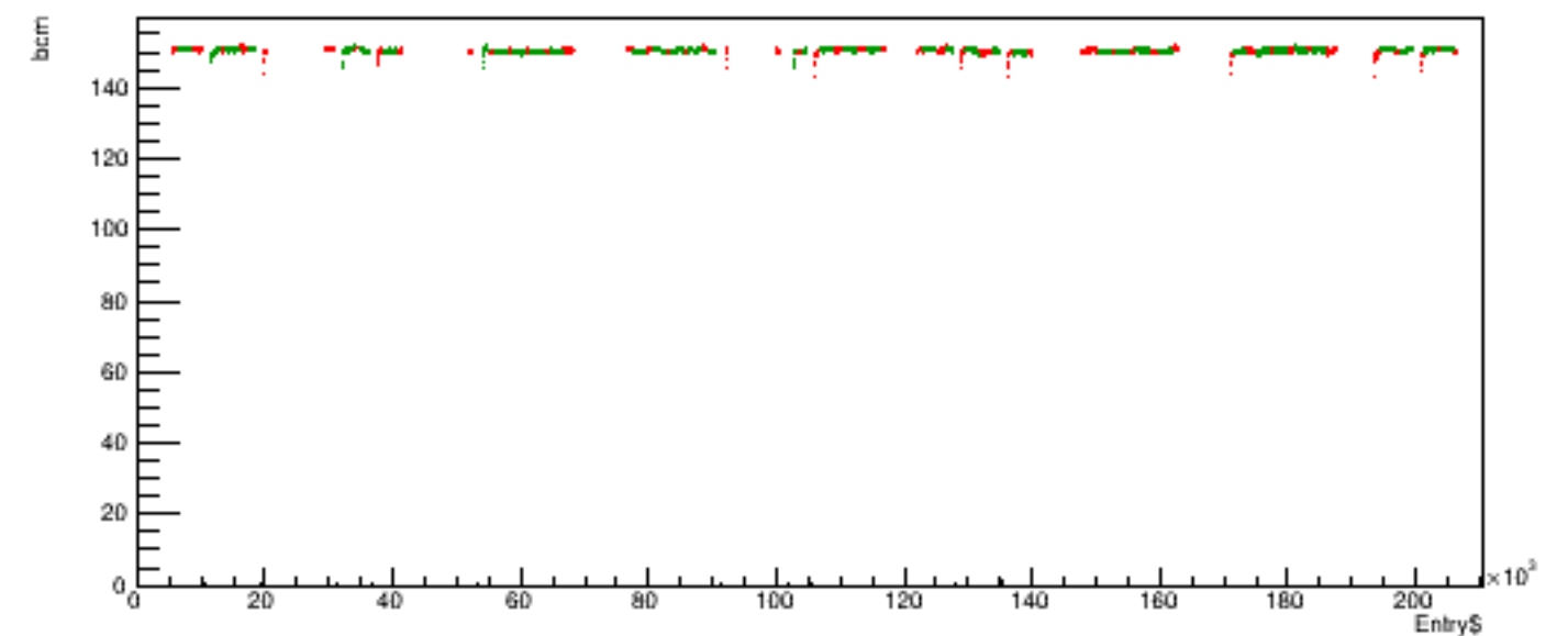
Run 5285 quartetwise, posH4 vs time
