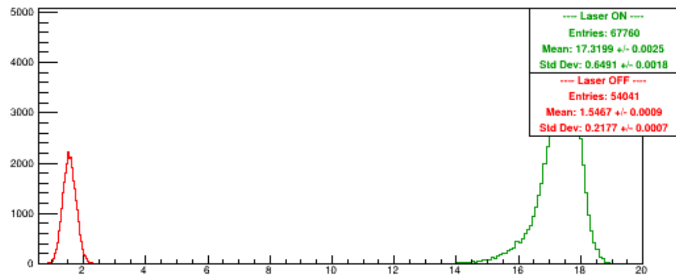
Run 5285 quartetwise, PosHelAcc0/NSamples0
