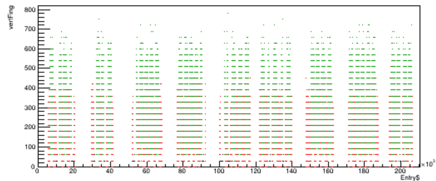
Run 5285 quartetwise, vertFing vs time
