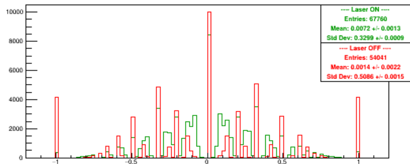
Run 5285 quartetwise, Asyms Horiz Finger
