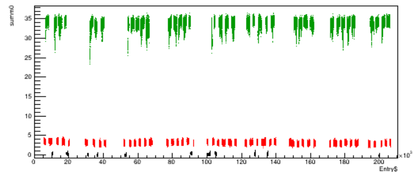
Run 5285 quartetwise, summ0 vs time
