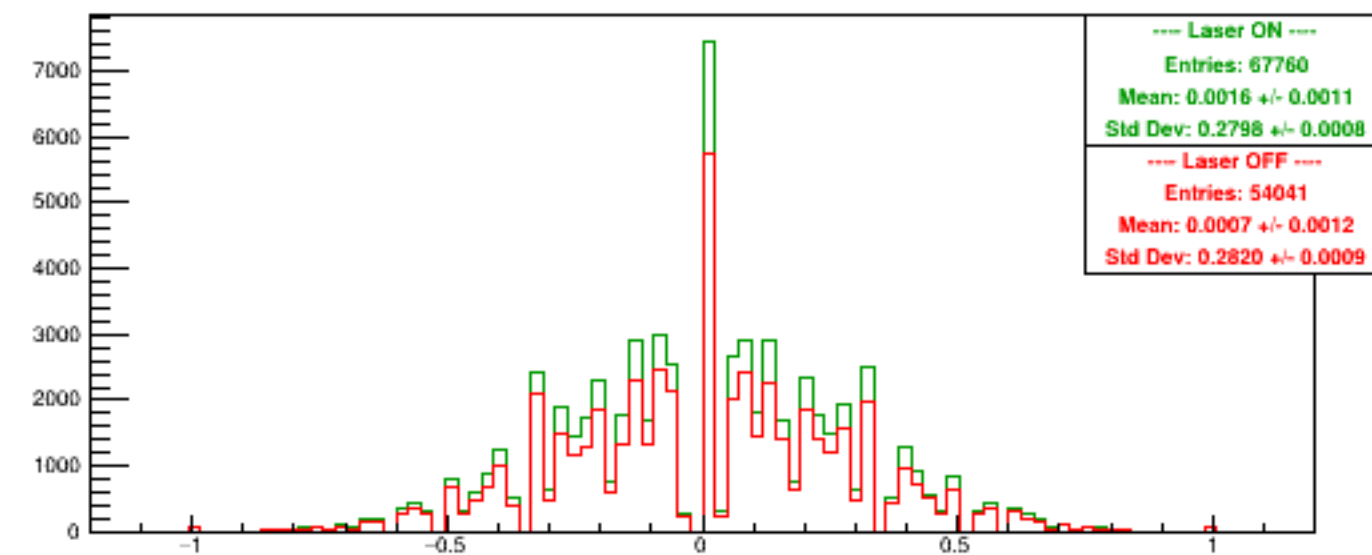
Run 5285 quartetwise, Asyms USbg2
