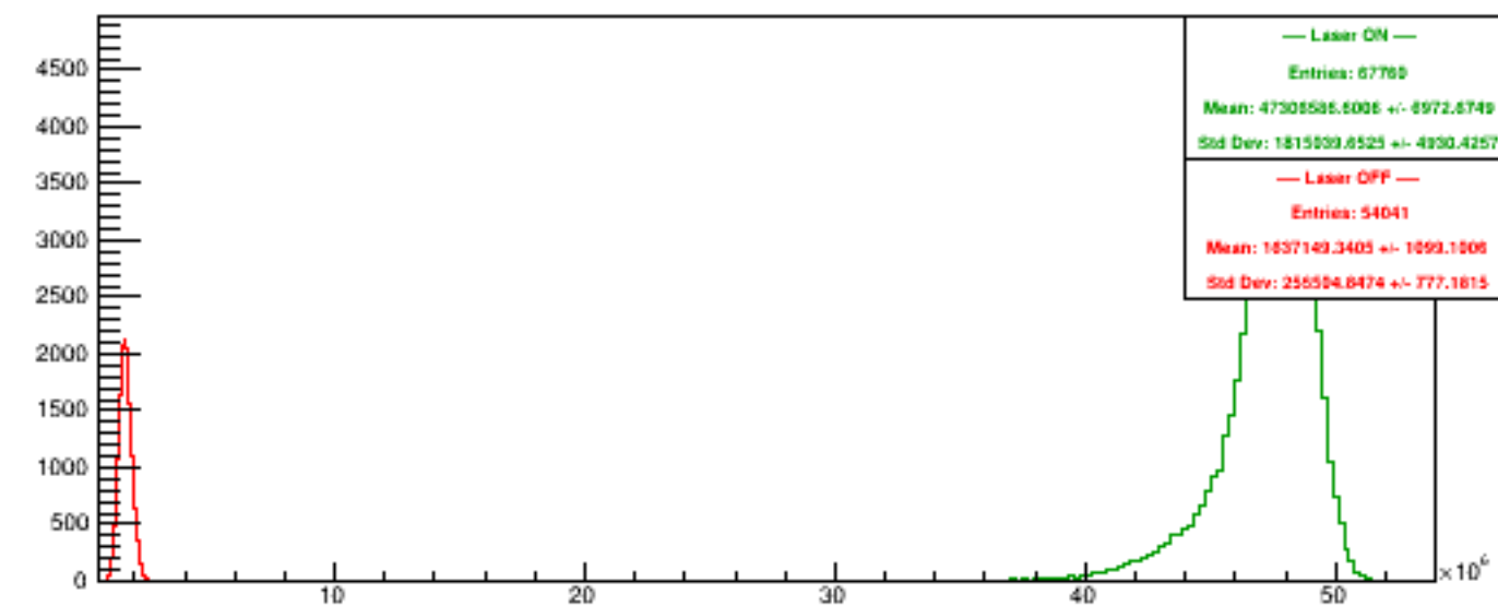
Run 5285 quartetwise, NegHelAcc4
