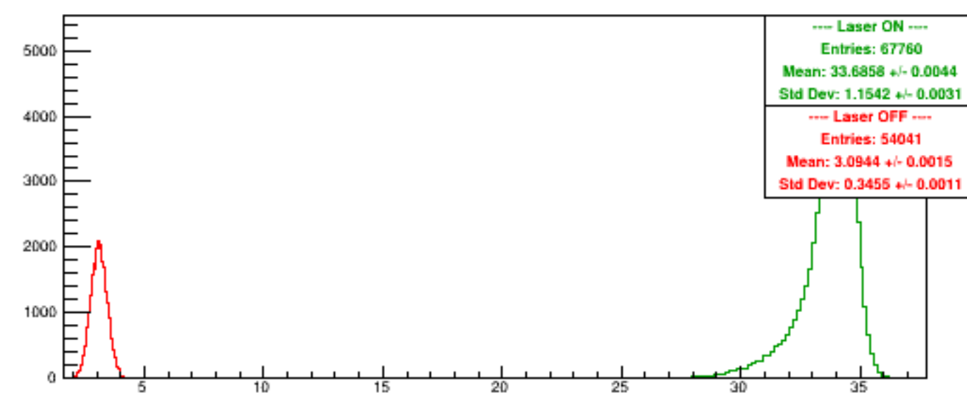
Run 5285 quartetwise, Sums0
