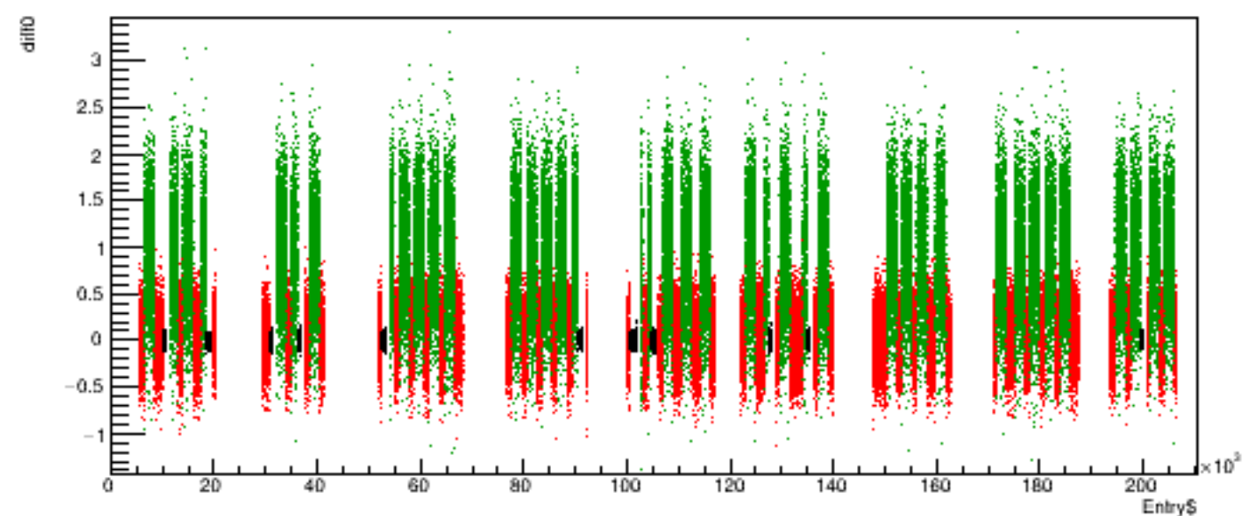
Run 5285 quartetwise, diff0 vs time
