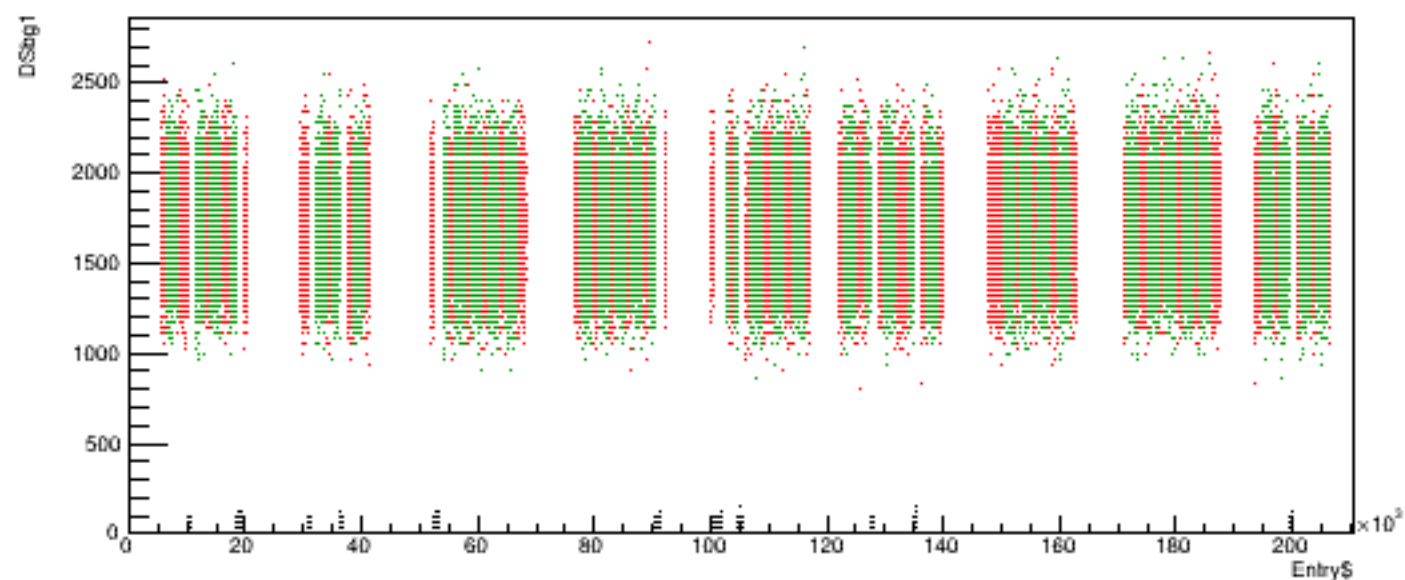
Run 5285 quartetwise, DSbg1 vs time
