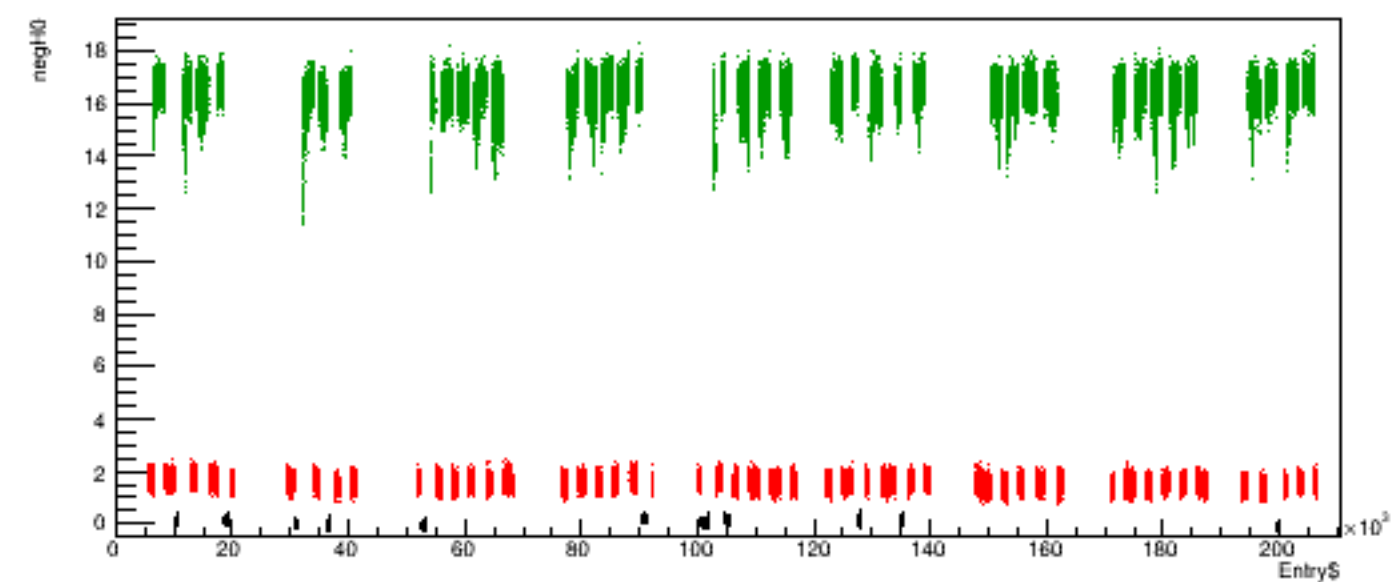
Run 5285 quartetwise, negH0 vs time
