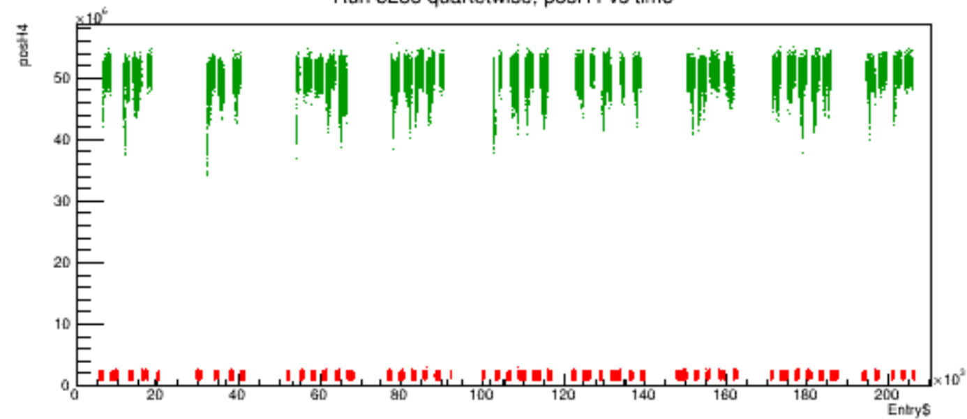
Run 5285 quartetwise, posH4 vs time
