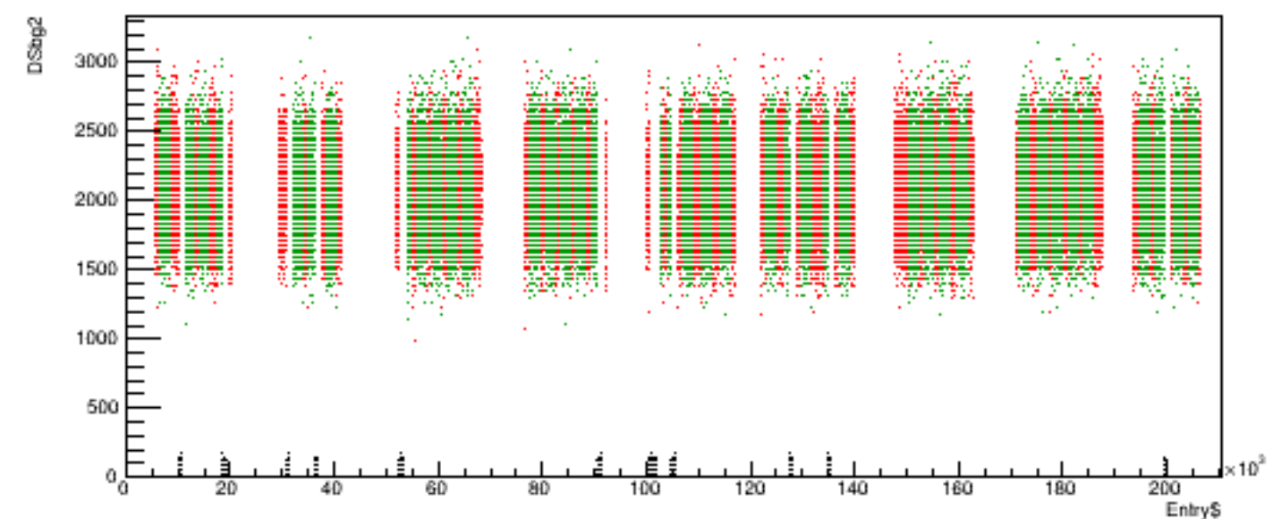
Run 5285 quartetwise, DSbg2 vs time
