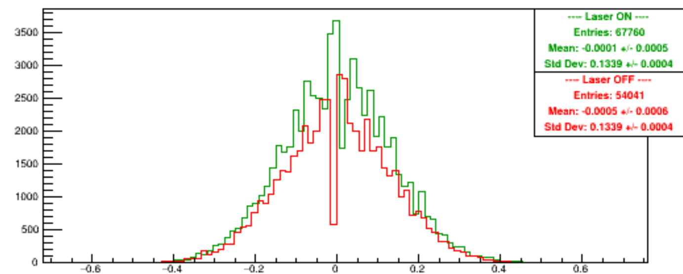
Run 5285 quartetwise, Asyms DSbg1
