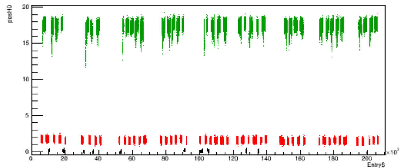
Run 5285 quartetwise, posH0 vs time
