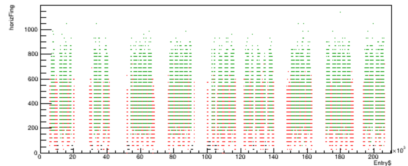
Run 5285 quartetwise, horizFing vs time
