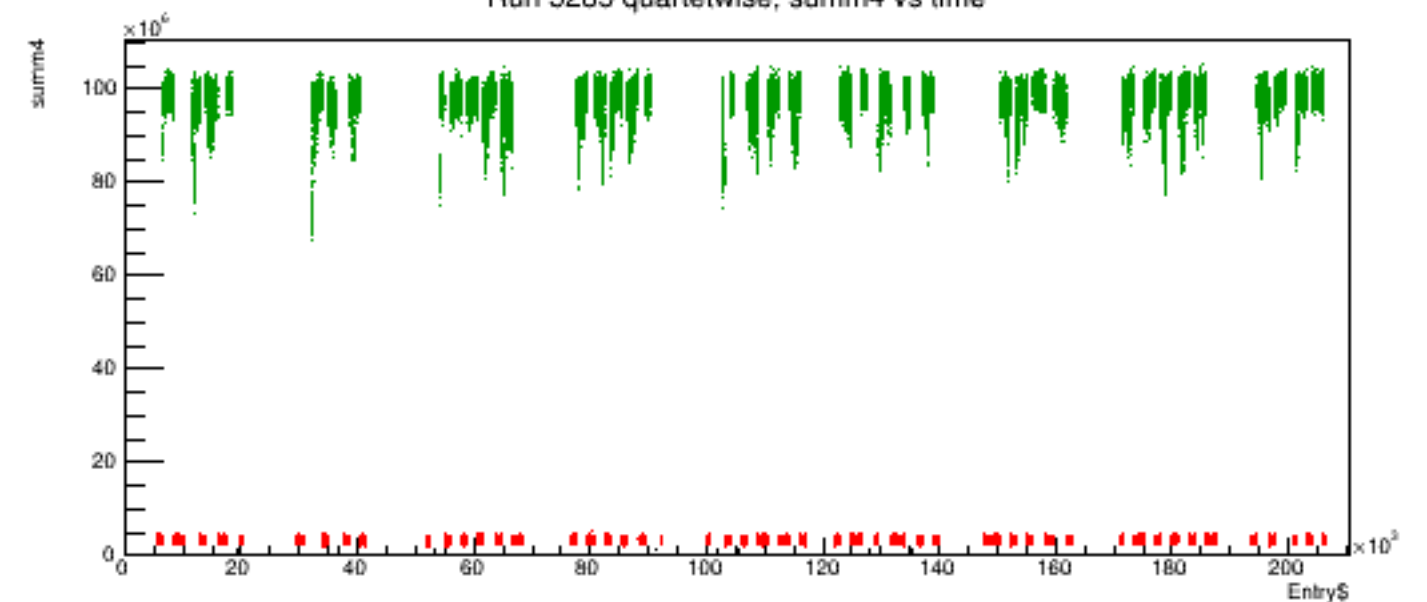
Run 5285 quartetwise, summ4 vs time
