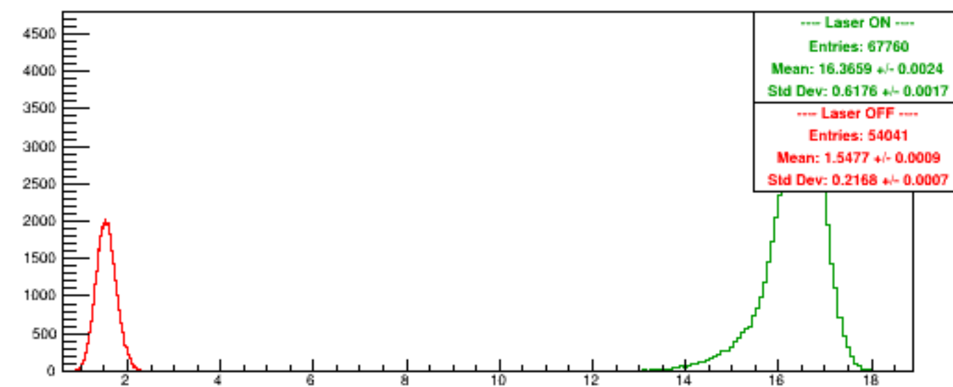
Run 5285 quartetwise, NegHelAcc0/NSamples0
