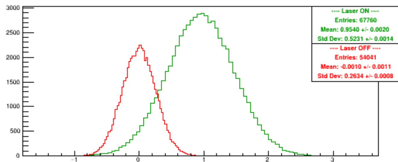
Run 5285 quartetwise, Diffs0
