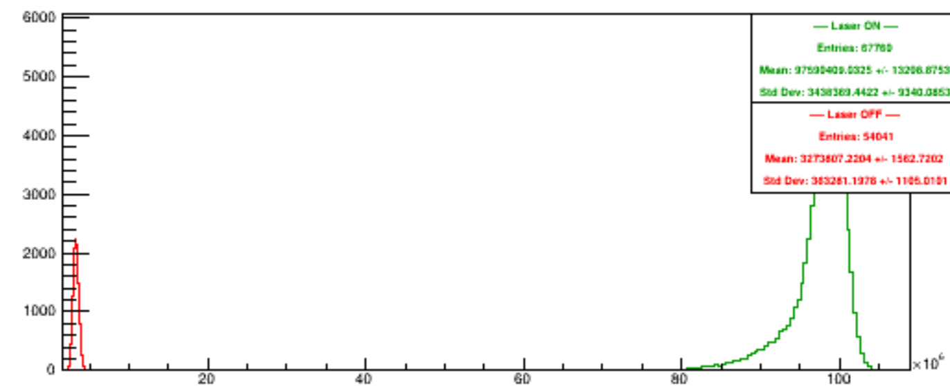
Run 5285 quartetwise, Sums4
