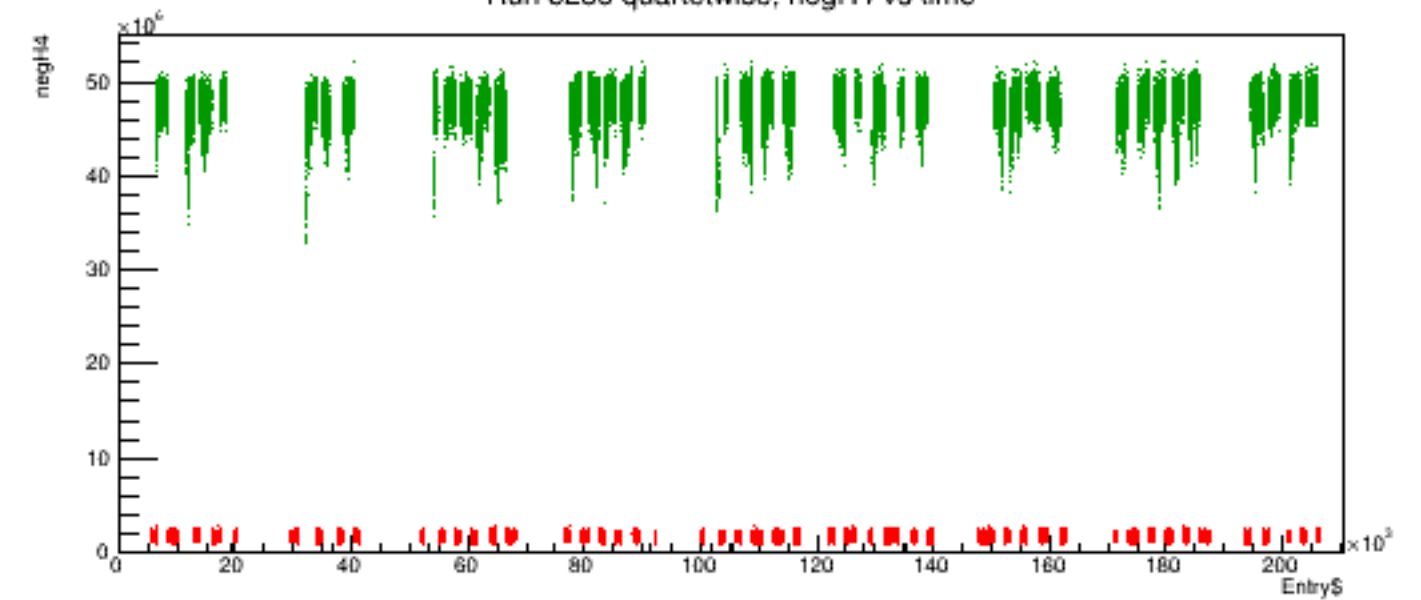
Run 5285 quartetwise, negH4 vs time
