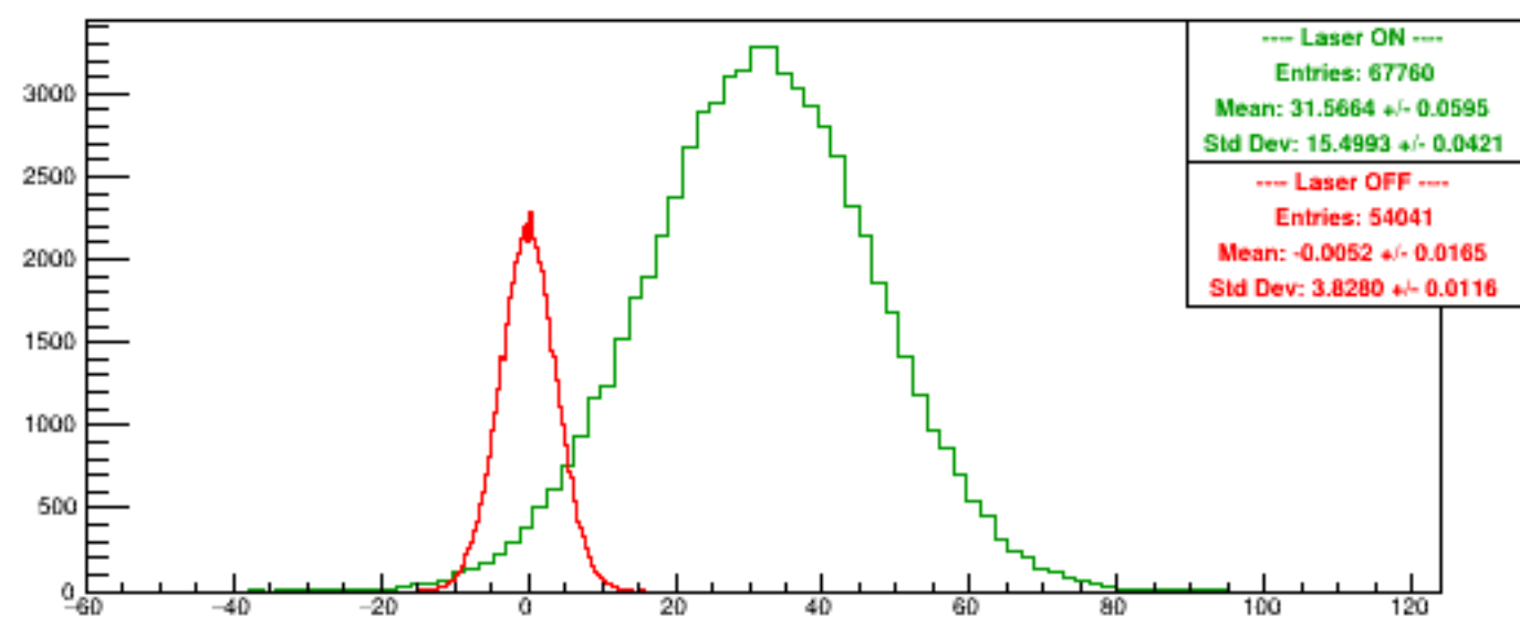
Run 5285 quartetwise, Asyms4
