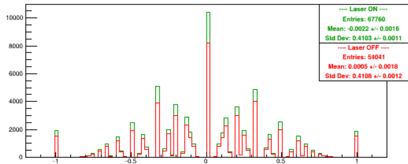
Run 5285 quartetwise, Asyms USbg1
