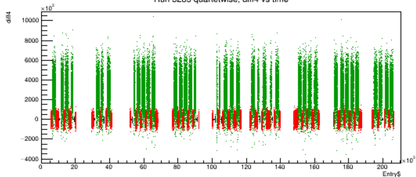
Run 5285 quartetwise, diff4 vs time
