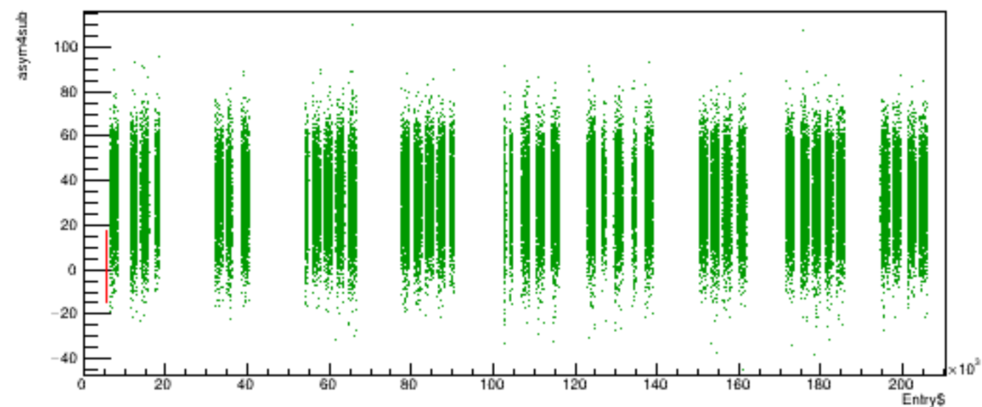
Run 5285 quartetwise, asym4sub vs time
