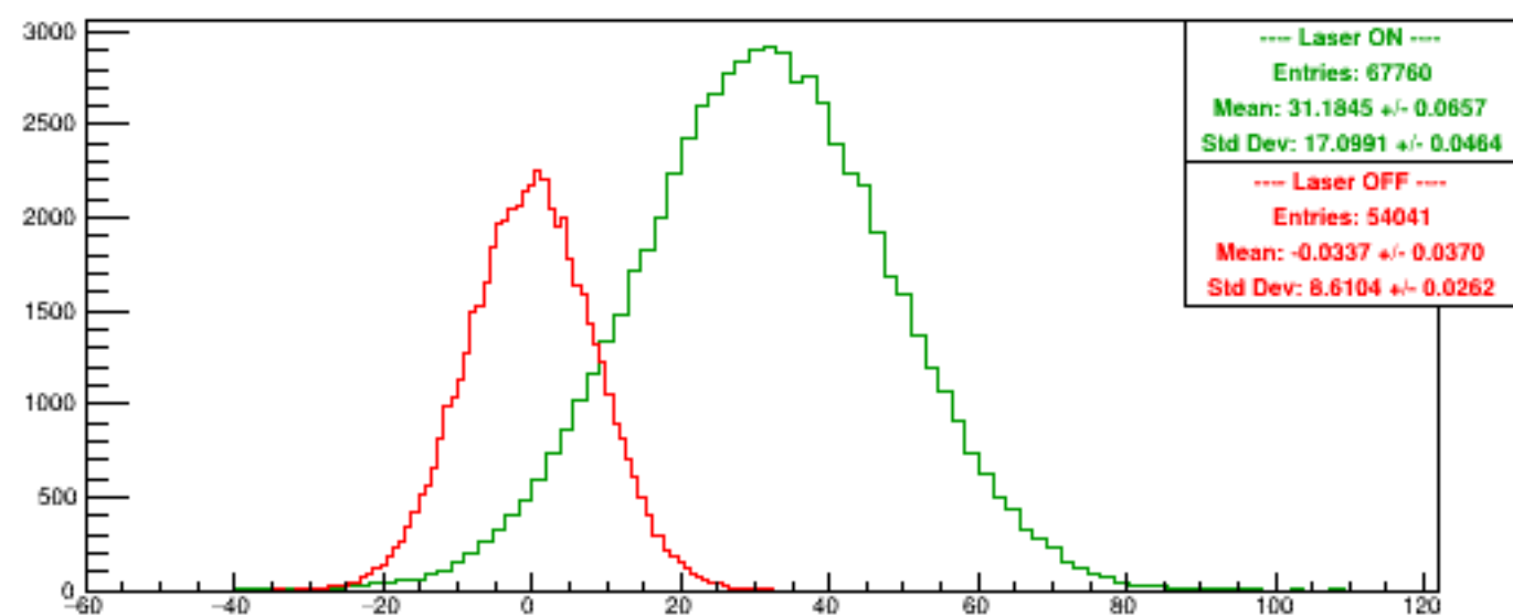
Run 5285 quartetwise, Asyms0
