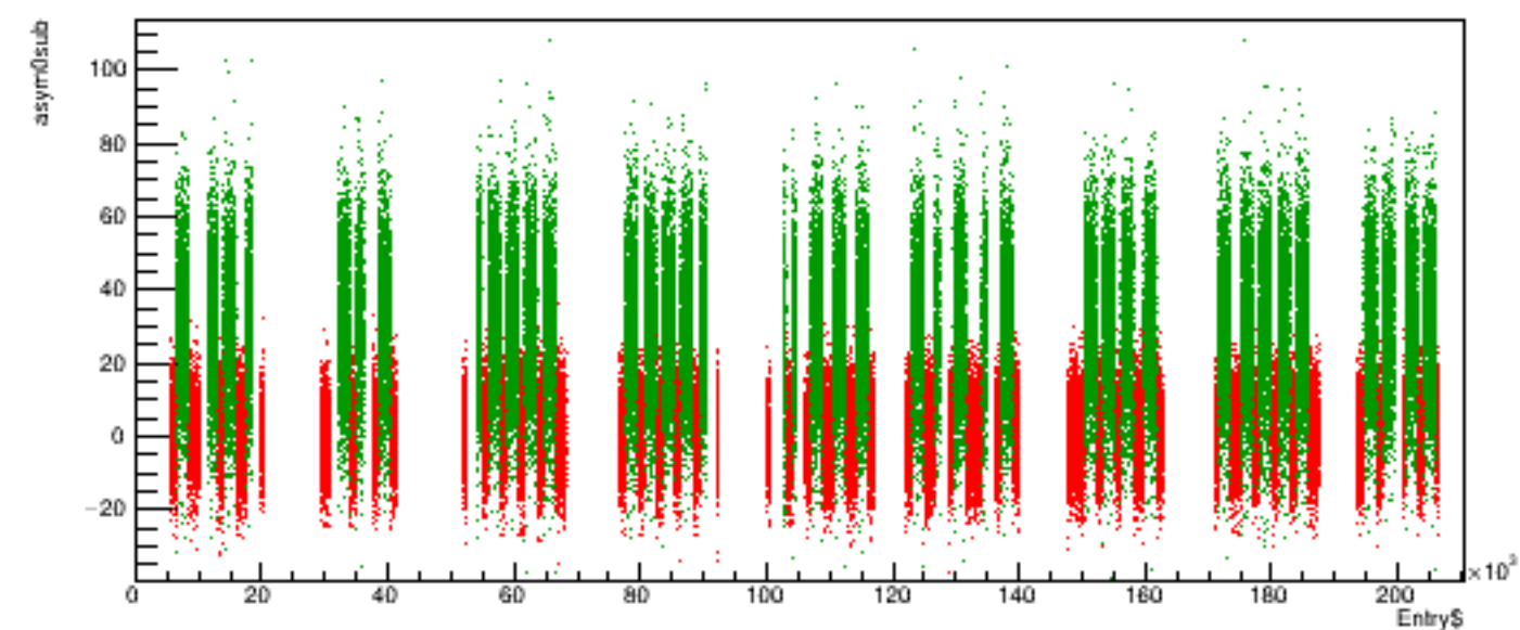
Run 5285 quartetwise, asym0sub vs time
