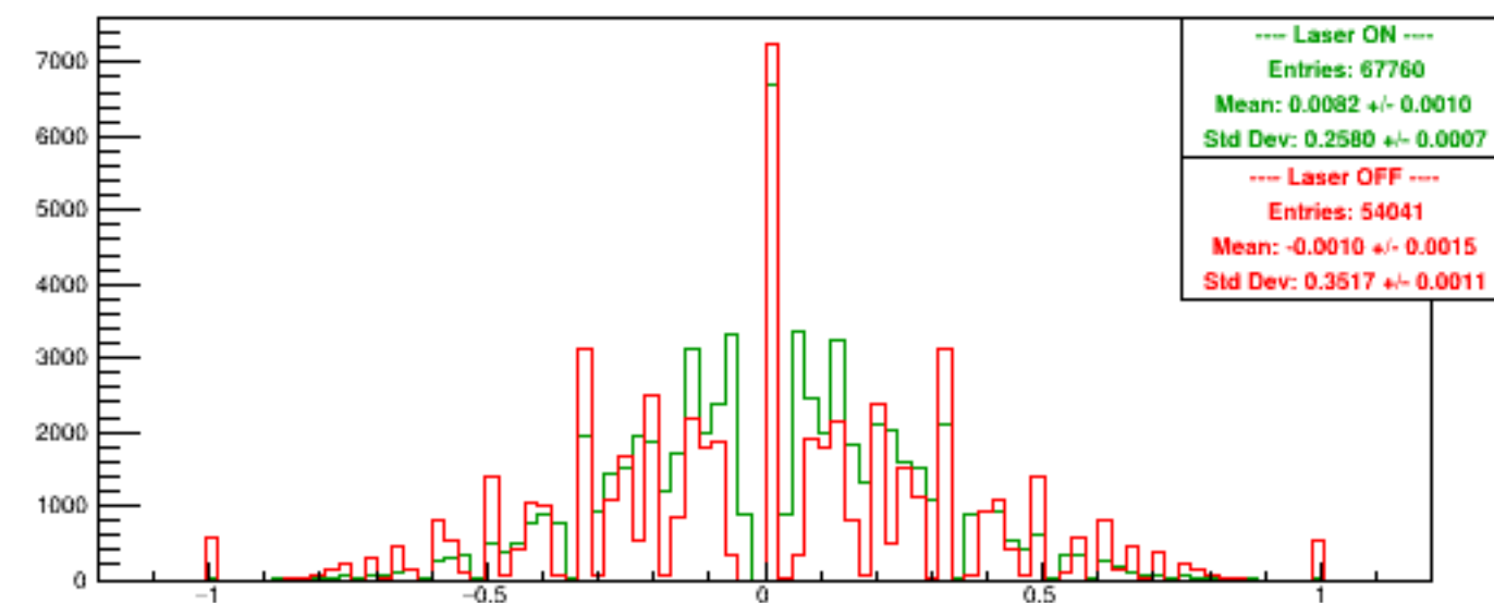
Run 5285 quartetwise, Asyms Vert Finger
