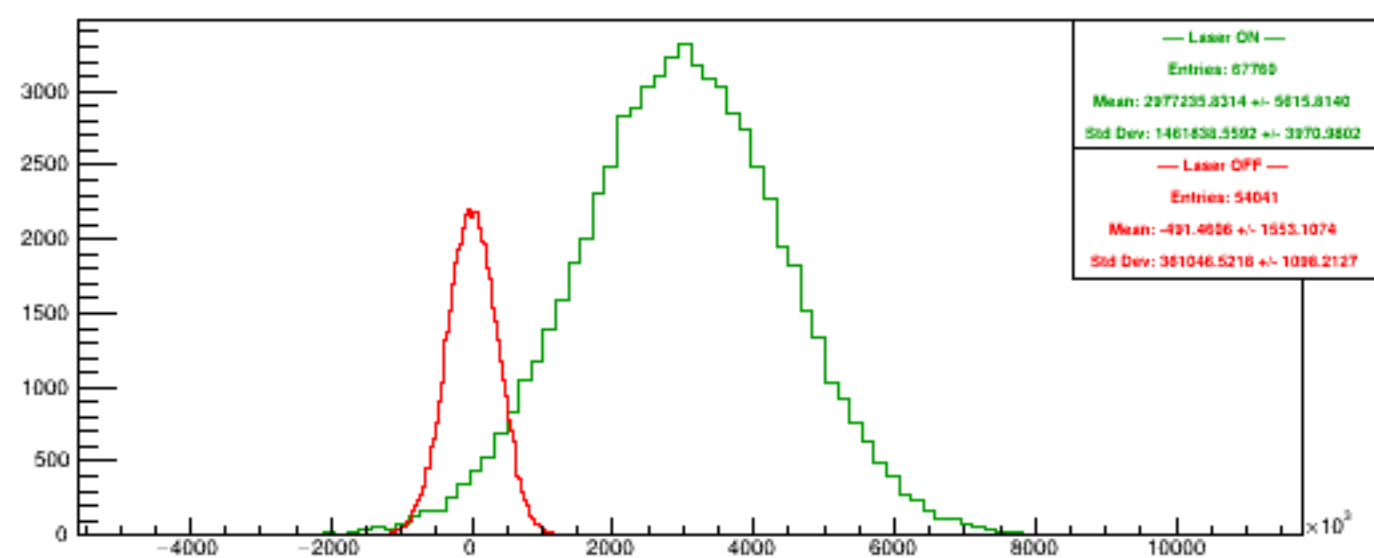
Run 5285 quartetwise, Diffs4
