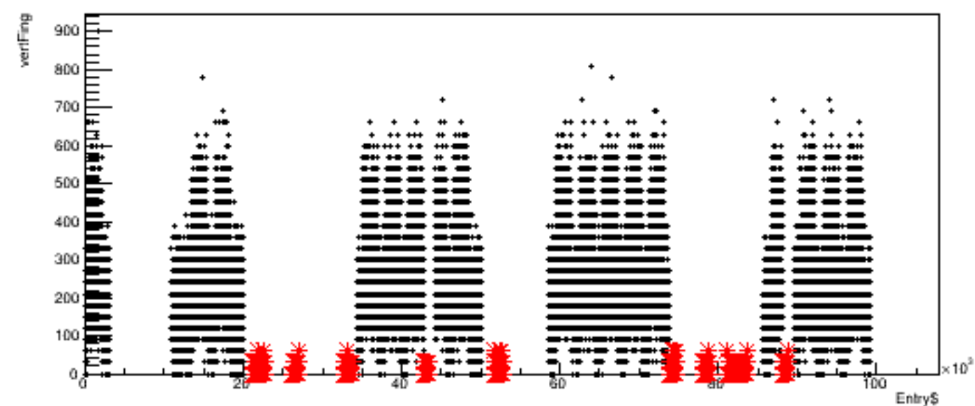
Run 5286, quartetwise: vertFing vs time
