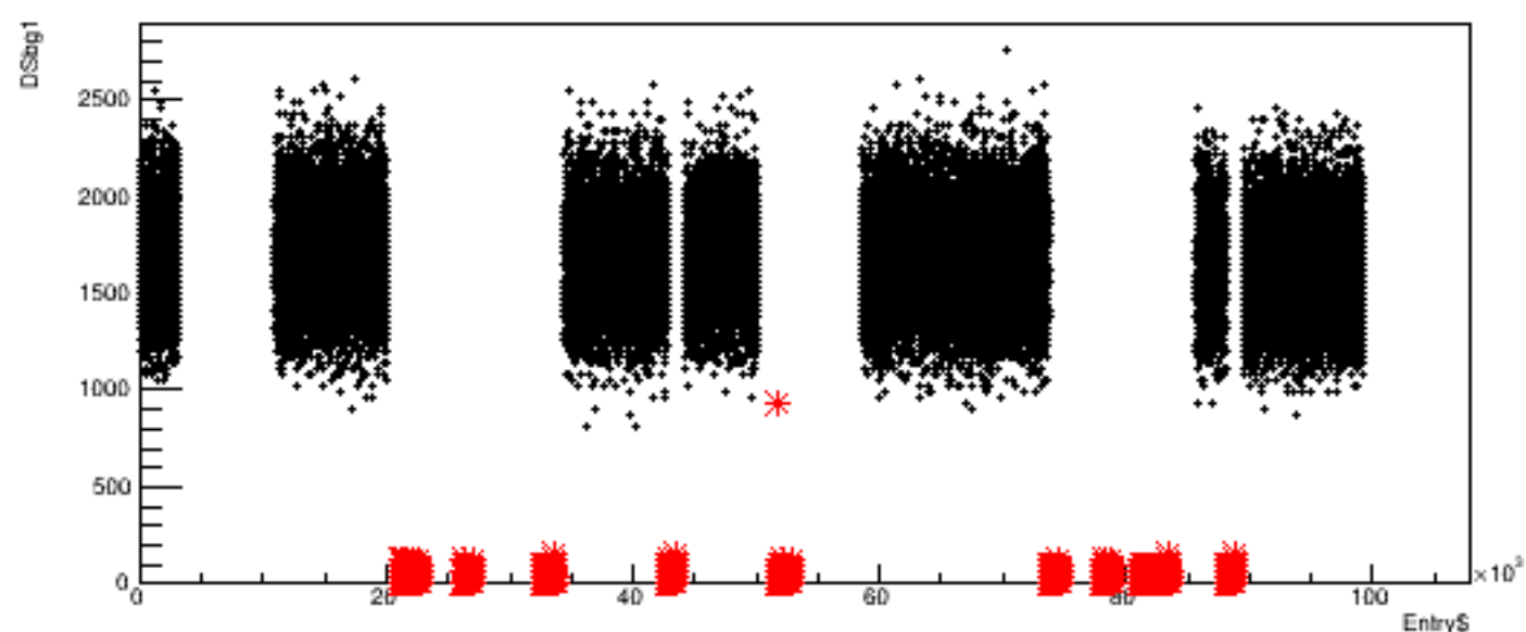
Run 5286, quartetwise: DSbg1 vs time
