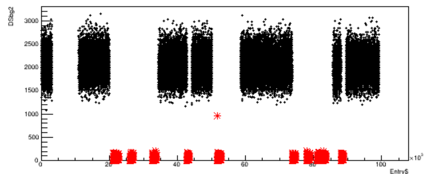
Run 5286, quartetwise: DSbg2 vs time
