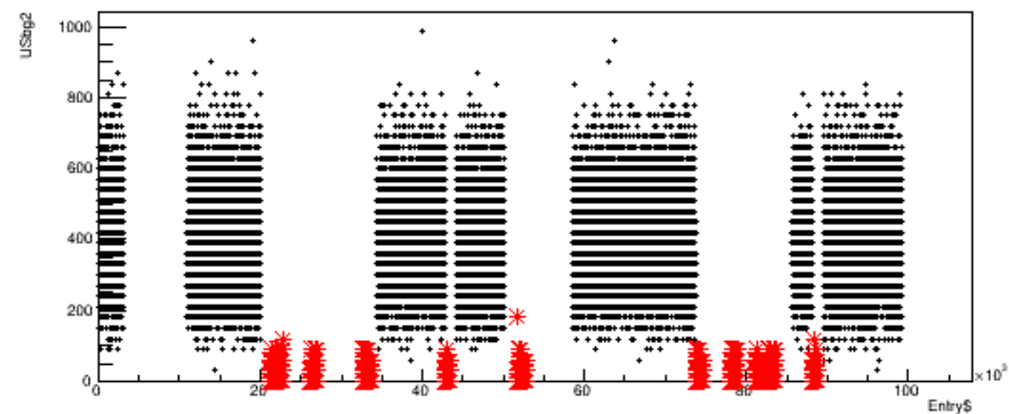
Run 5286, quartetwise: USbg2 vs time
