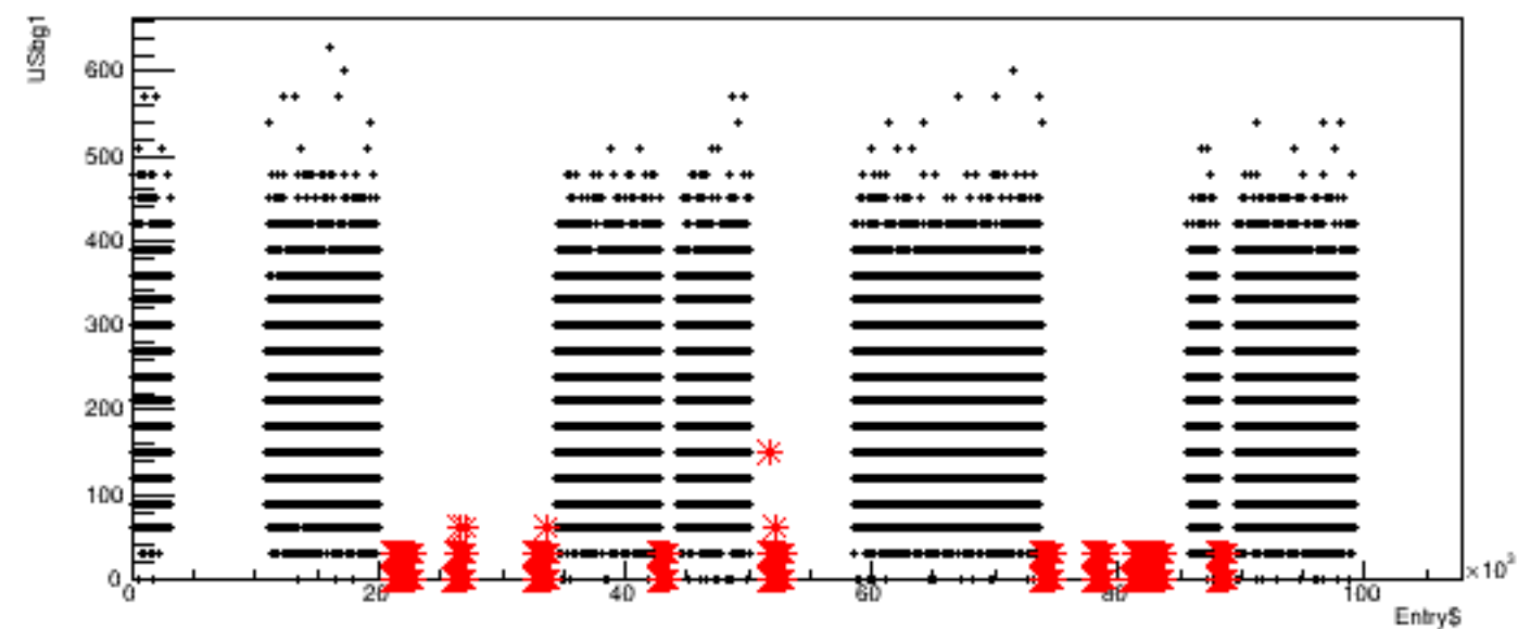
Run 5286, quartetwise: USbg1 vs time
