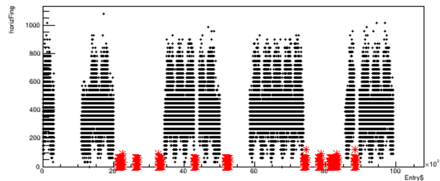
Run 5286, quartetwise: horizFing vs time
