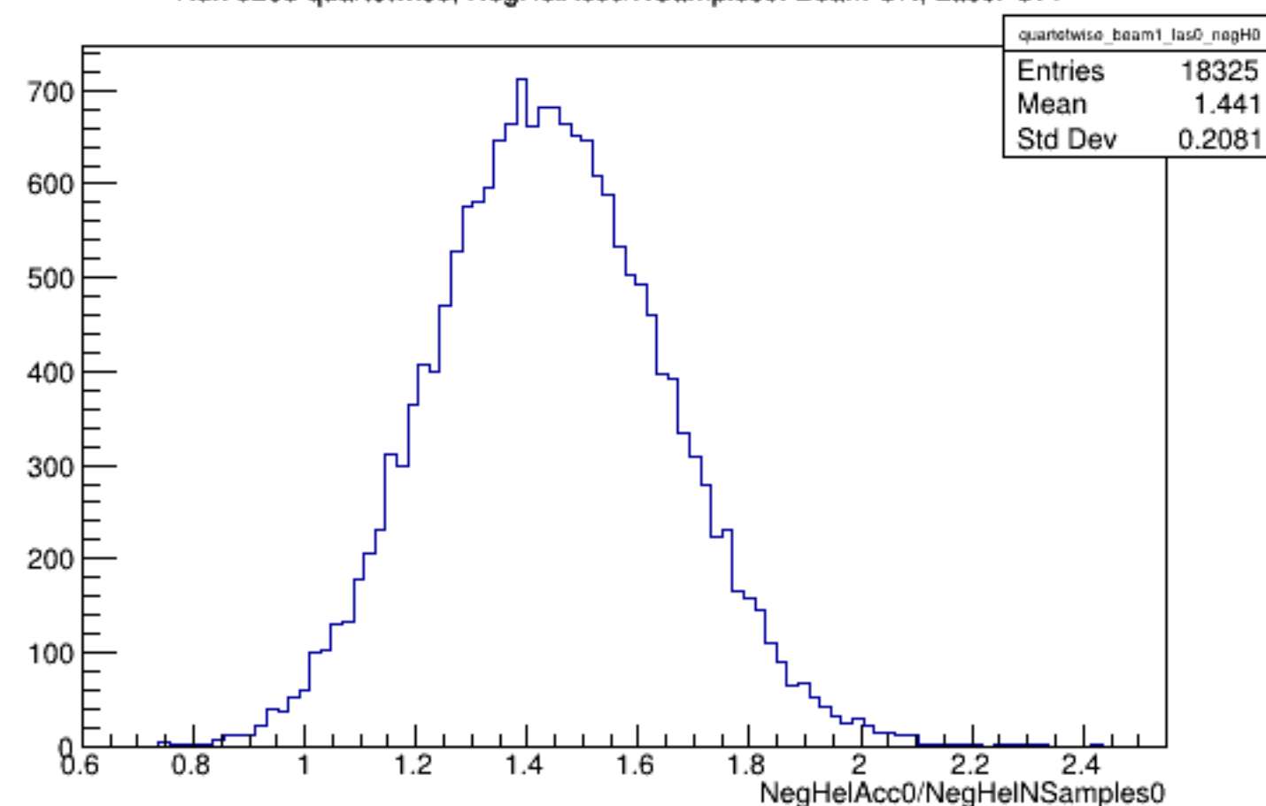
Run 5288 quartetwise, NegHelAcc0/NSamples0: Beam ON, Laser OFF
