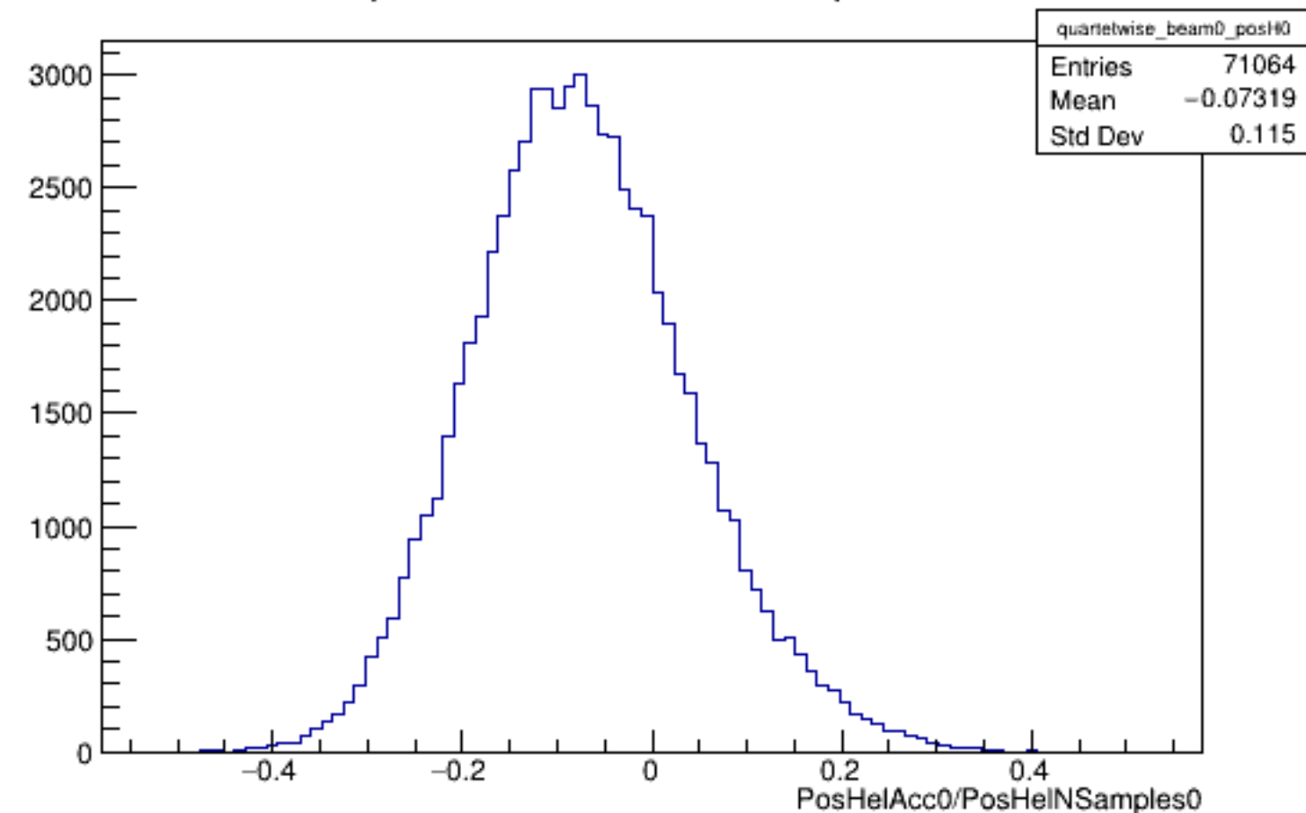
Run 5288 quartetwise, PosHelAcc0/NSamples0: Beam OFF
