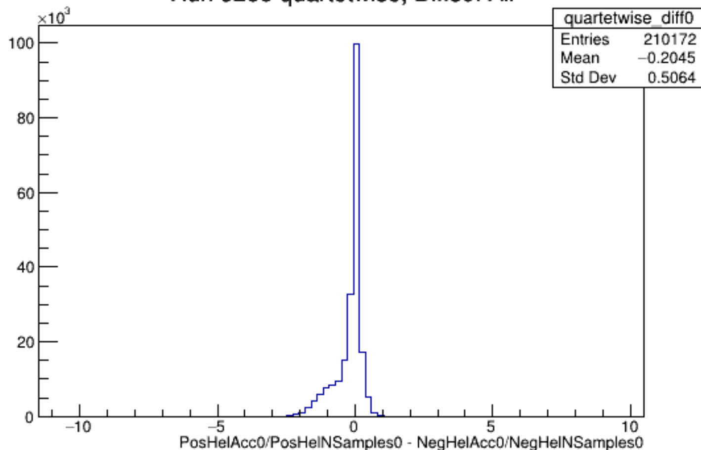
Run 5288 quartetwise, Diffs0: All
