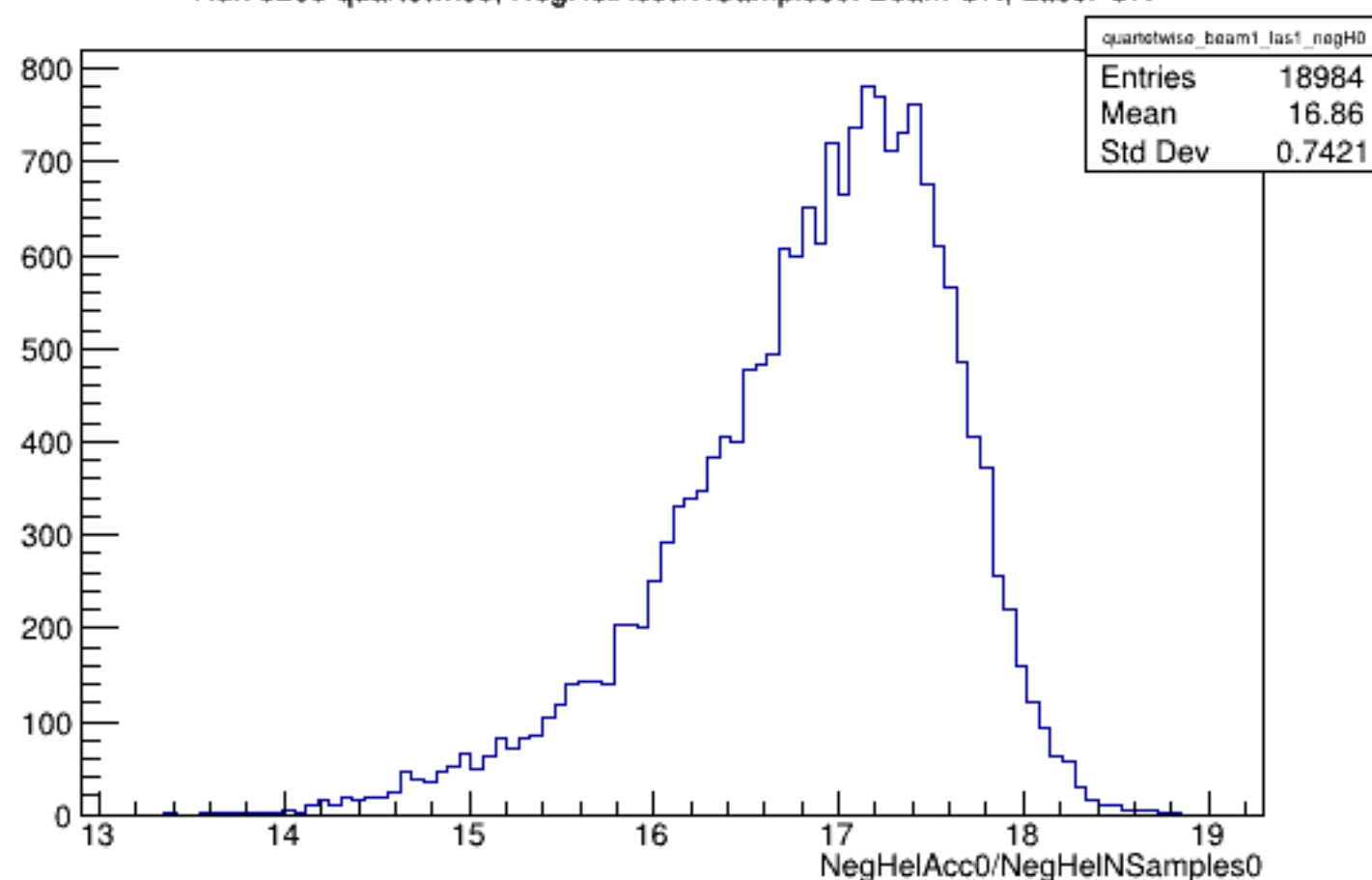
Run 5288 quartetwise, NegHelAcc0/NSamples0: Beam ON, Laser ON
