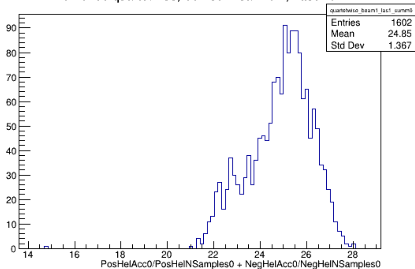
Run 5296 quartetwise, Sums0: Beam ON, Laser ON
