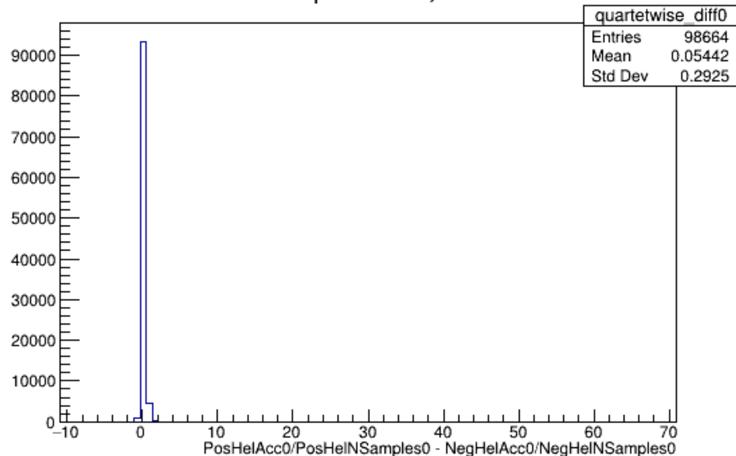
Run 5296 quartetwise, Diffs0: All
