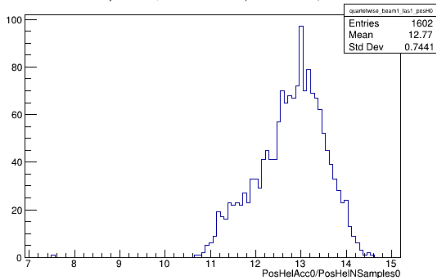
Run 5296 quartetwise, PosHelAcc0/NSamples0: Beam ON, Laser ON
