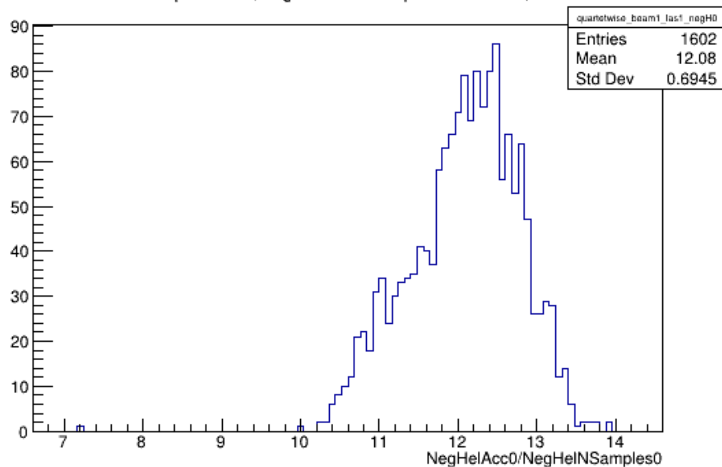
Run 5296 quartetwise, NegHelAcc0/NSamples0: Beam ON, Laser ON
