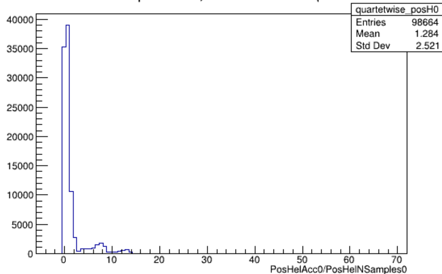
Run 5296 quartetwise, PosHelAcc0/NSamples0: All
