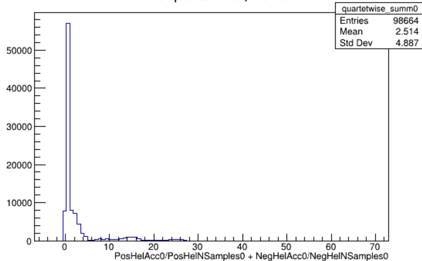
Run 5296 quartetwise, Sums0: All
