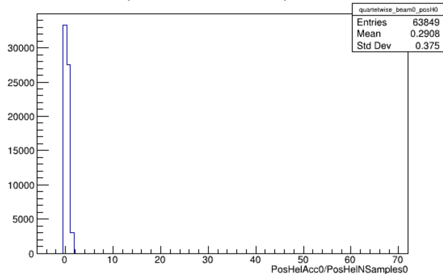
Run 5296 quartetwise, PosHelAcc0/NSamples0: Beam OFF
