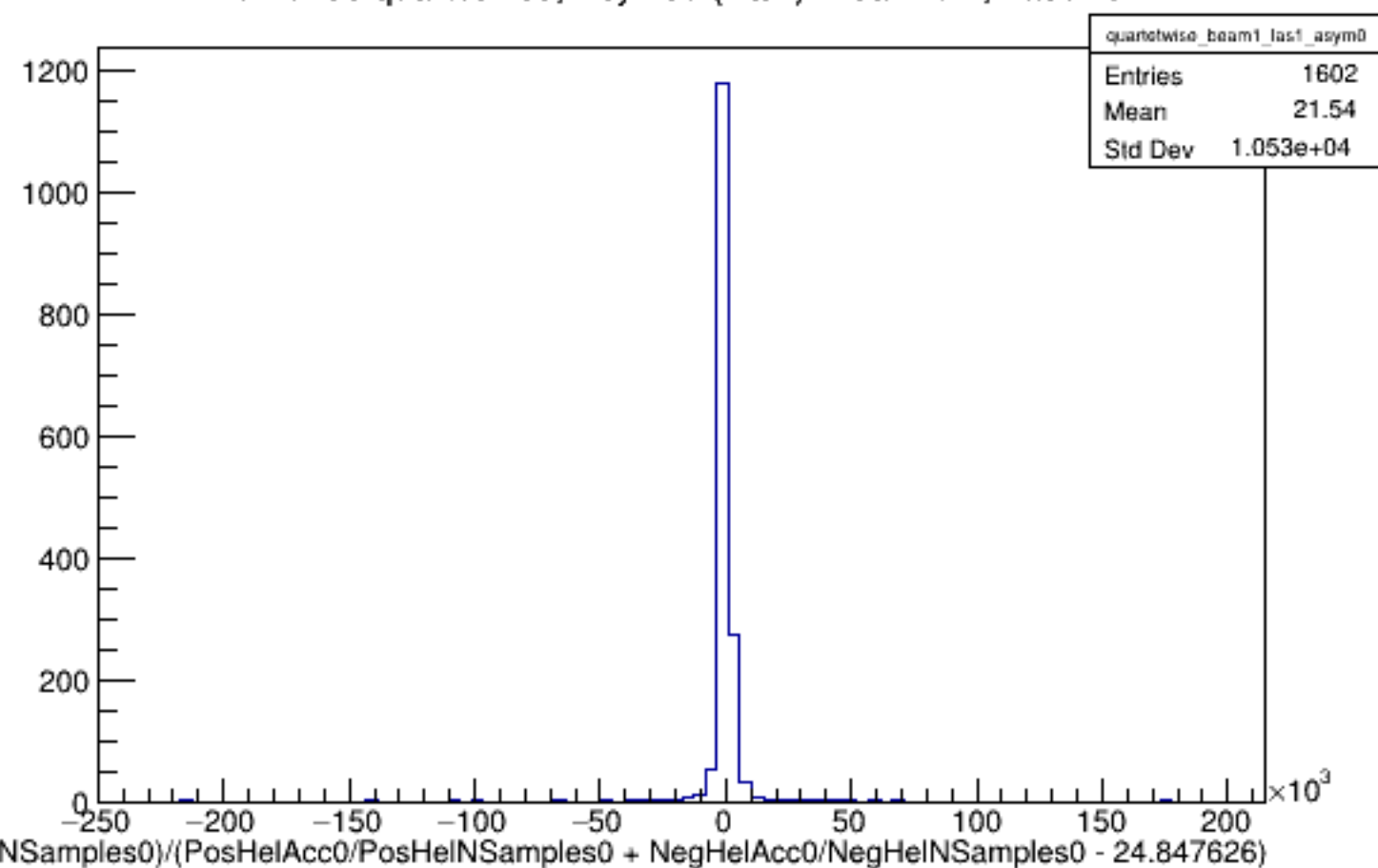
Run 5296 quartetwise, Asyms0 (Raw): Beam ON, Laser ON
