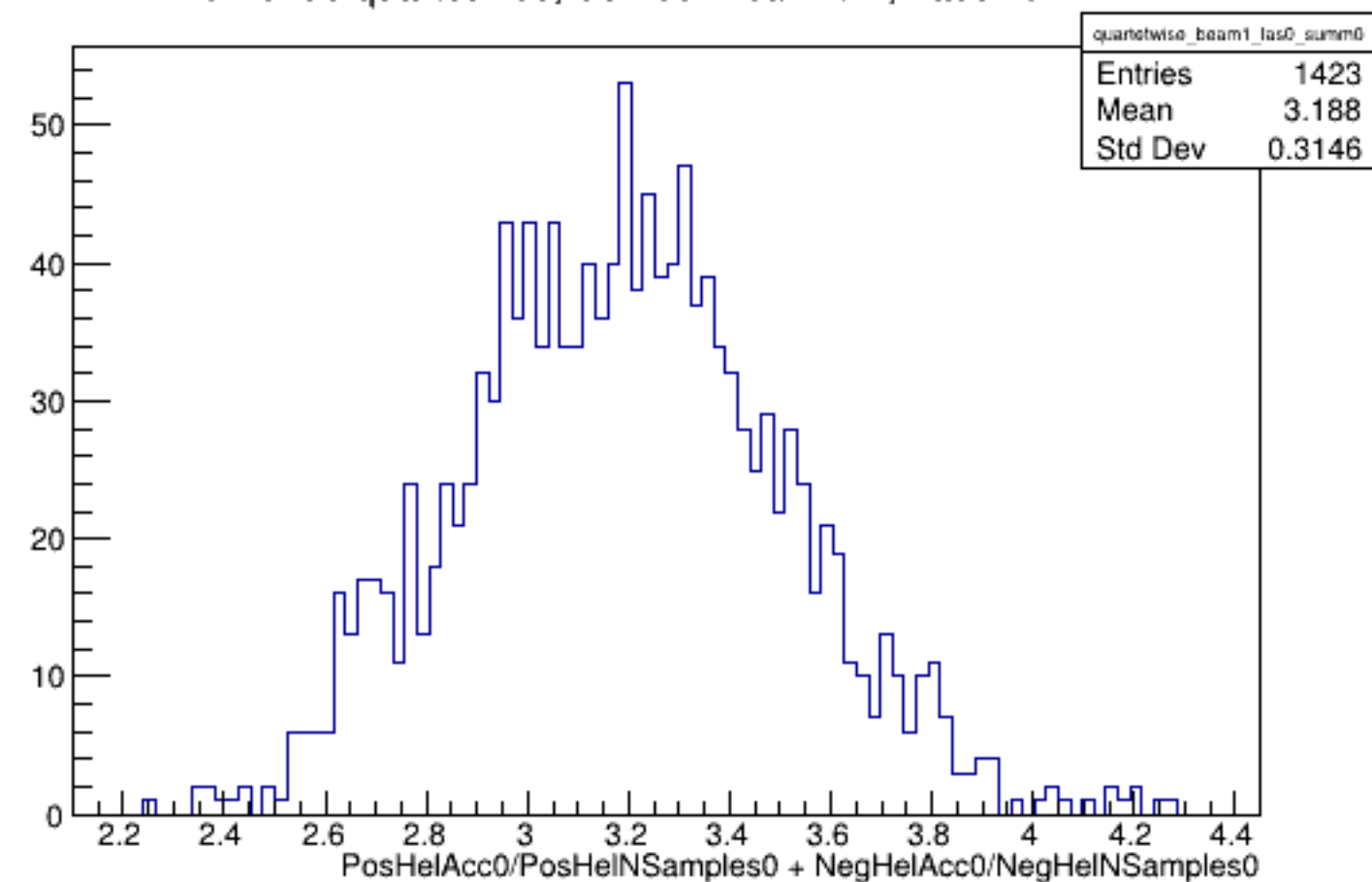
Run 5296 quartetwise, Sums0: Beam ON, Laser OFF
