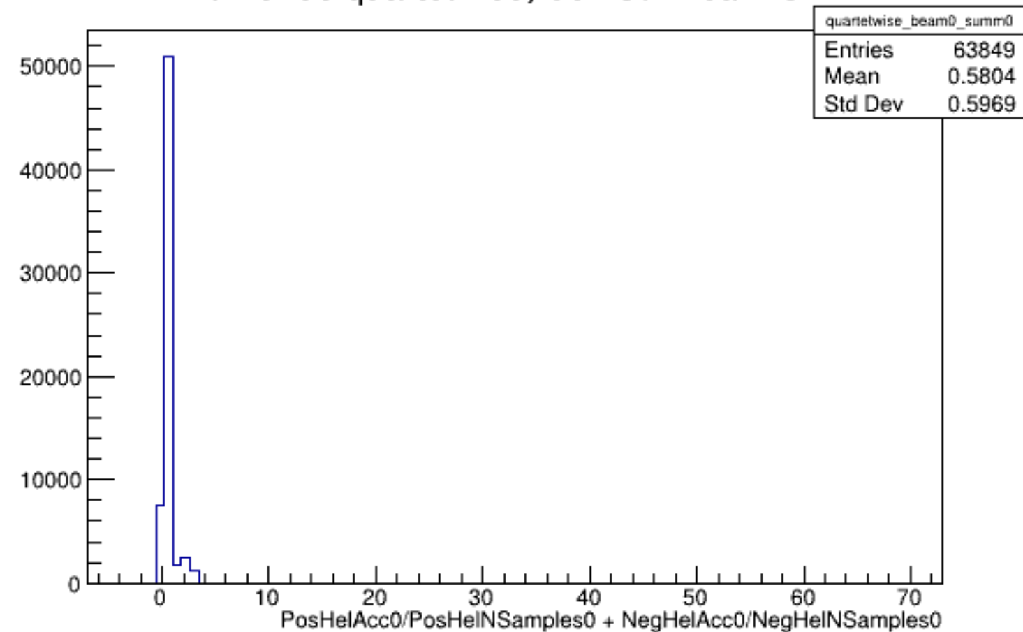
Run 5296 quartetwise, Sums0: Beam OFF
