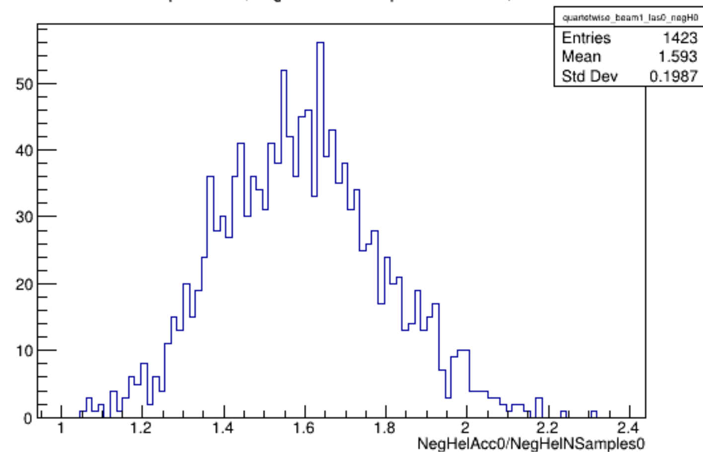
Run 5296 quartetwise, NegHelAcc0/NSamples0: Beam ON, Laser OFF
