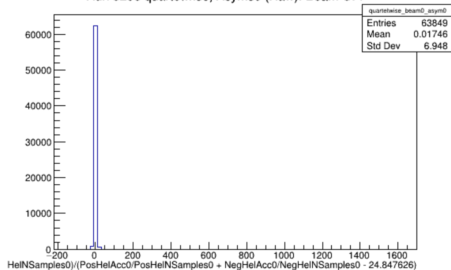
Run 5296 quartetwise, Asyms0 (Raw): Beam OFF
