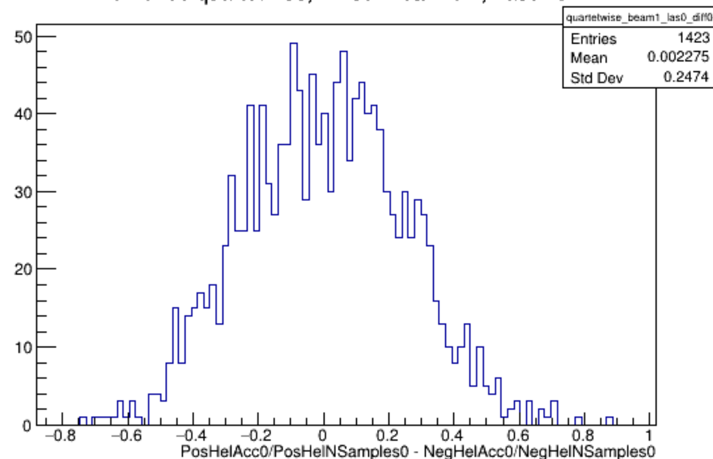
Run 5296 quartetwise, Diffs0: Beam ON, Laser OFF
