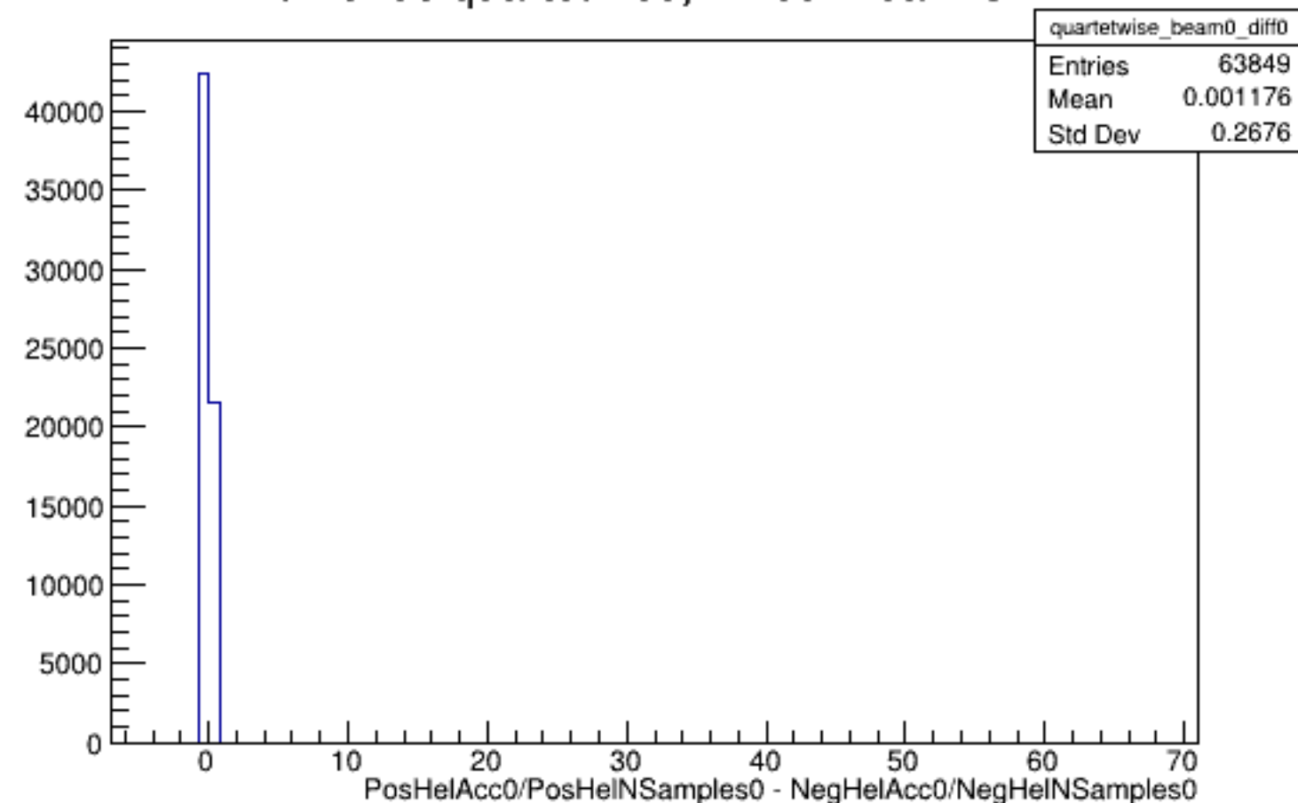
Run 5296 quartetwise, Diffs0: Beam OFF
