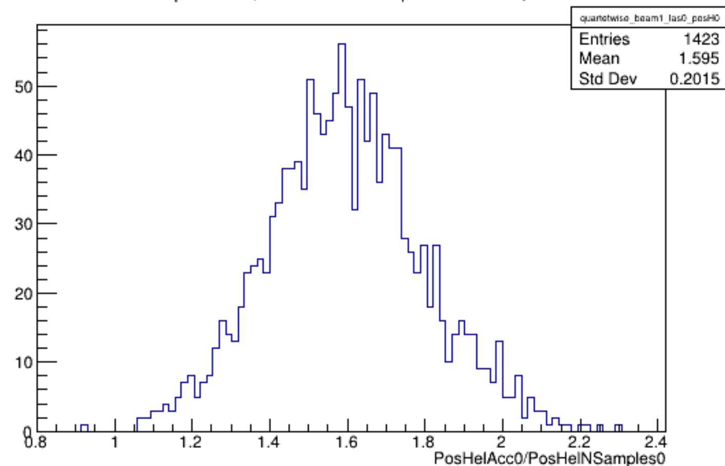
Run 5296 quartetwise, PosHelAcc0/NSamples0: Beam ON, Laser OFF
