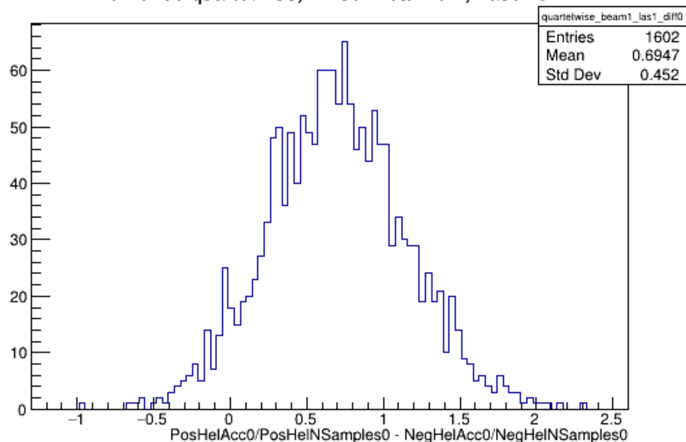
Run 5296 quartetwise, Diffs0: Beam ON, Laser ON
