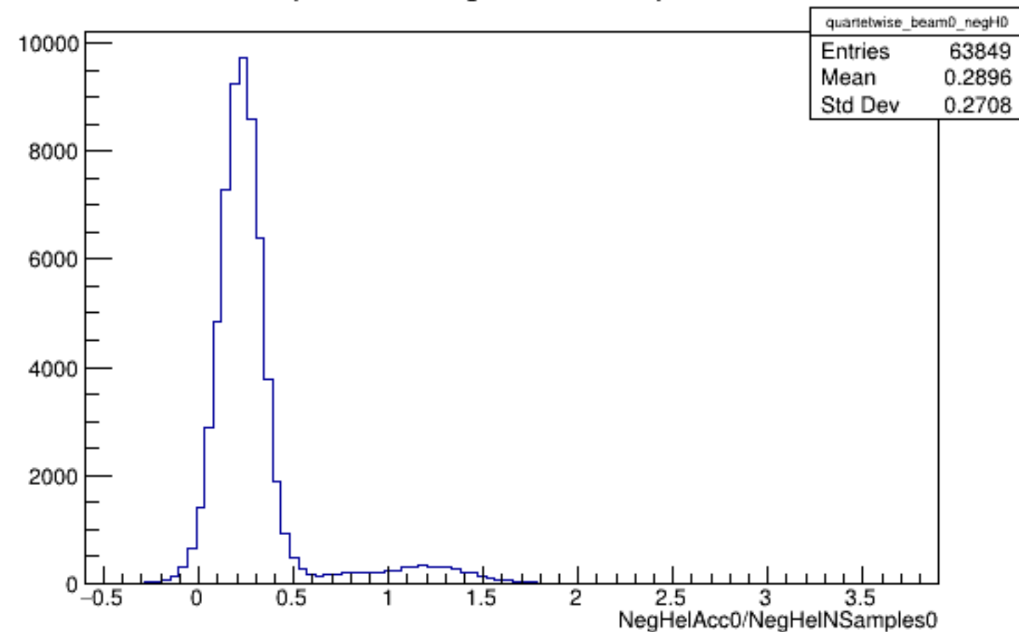
Run 5296 quartetwise, NegHelAcc0/NSamples0: Beam OFF
