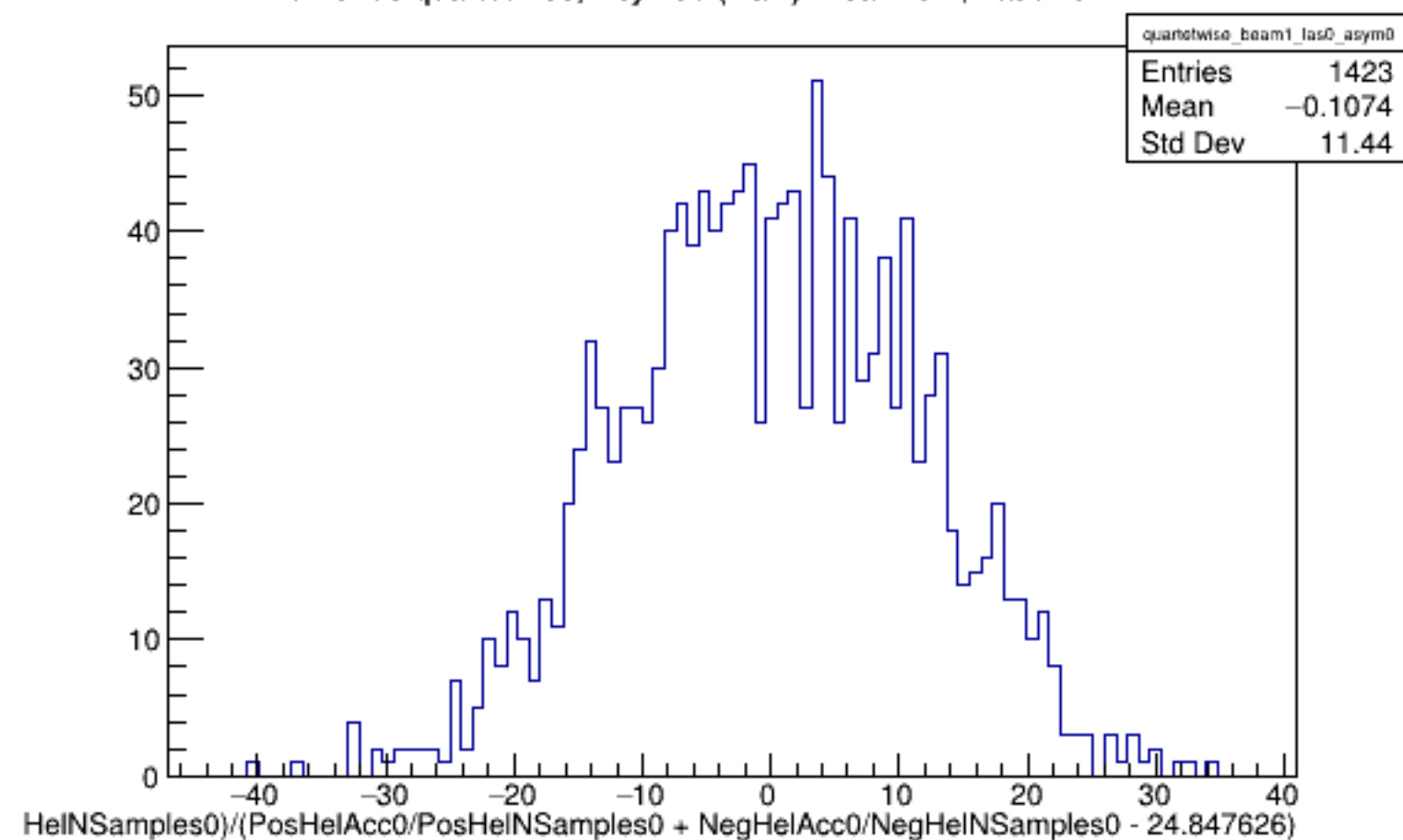
Run 5296 quartetwise, Asyms0 (Raw): Beam ON, Laser OFF
