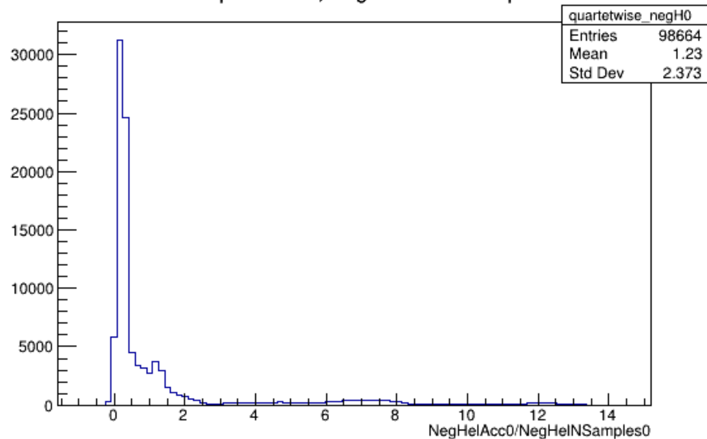
Run 5296 quartetwise, NegHelAcc0/NSamples0: All
