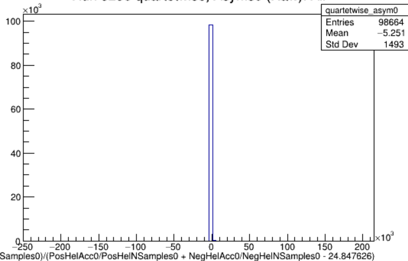
Run 5296 quartetwise, Asyms0 (Raw): All
