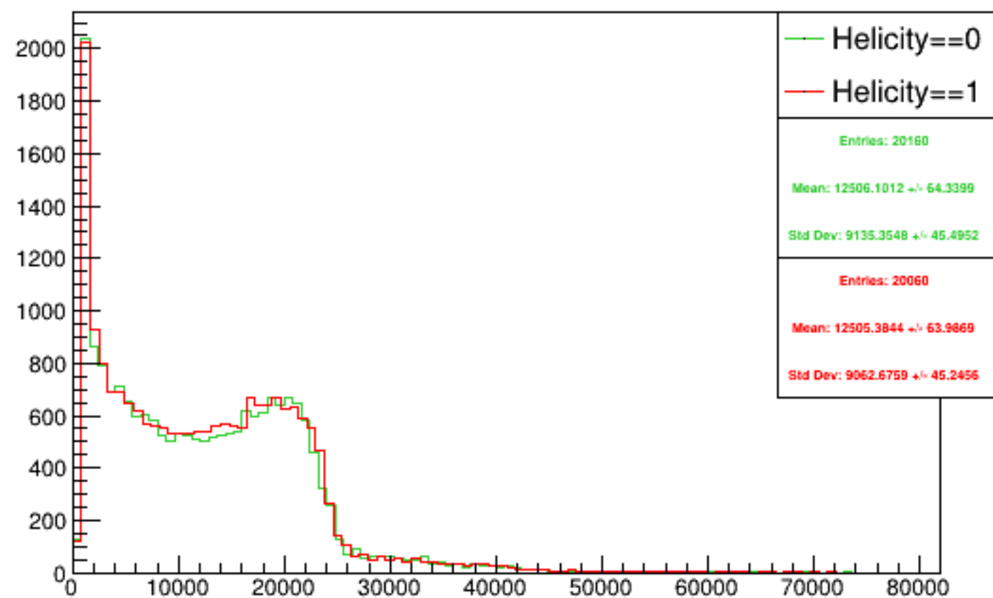
Run 5296 triggerwise, sums: Beam ON, Laser ON
