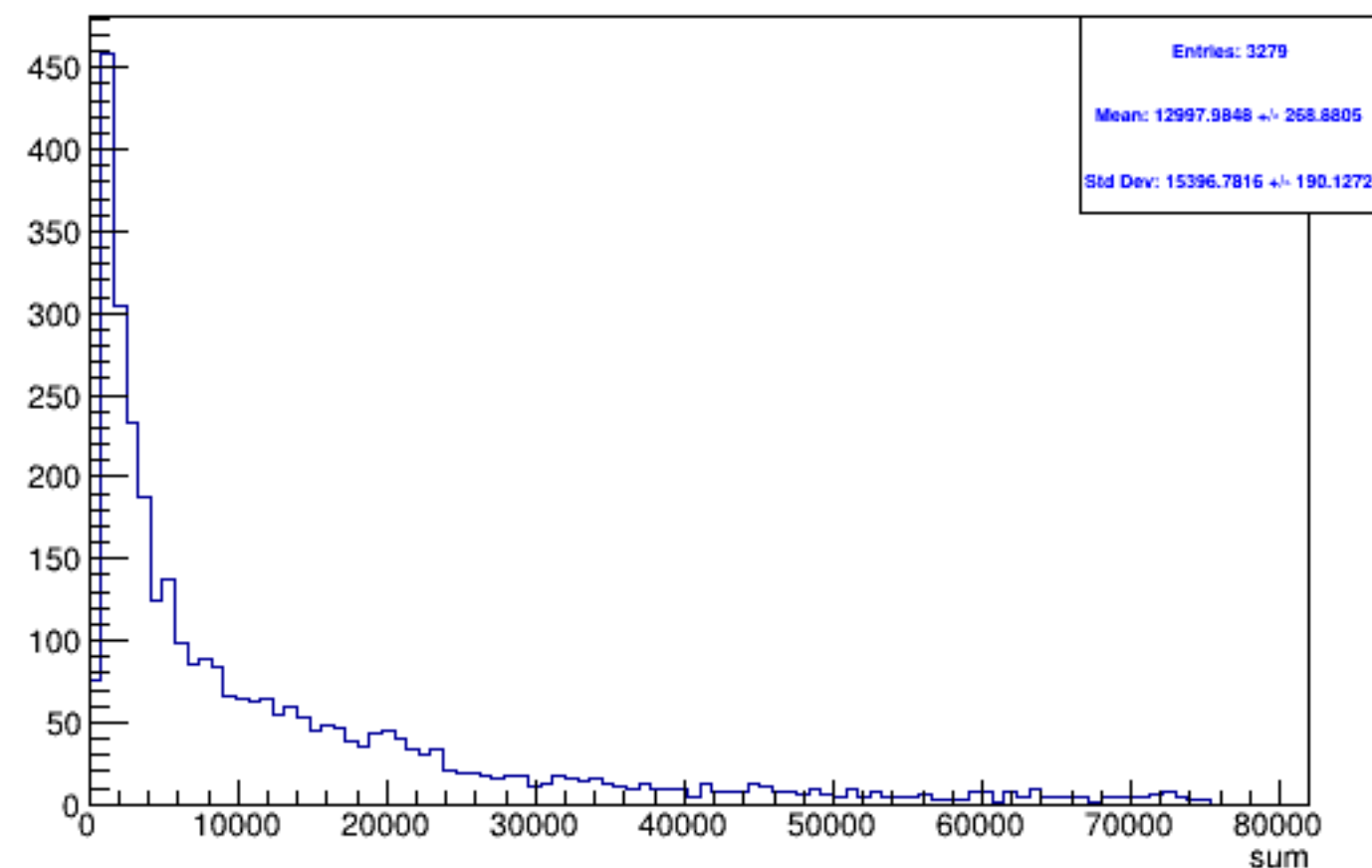
Run 5296 triggerwise, sums: Beam OFF
