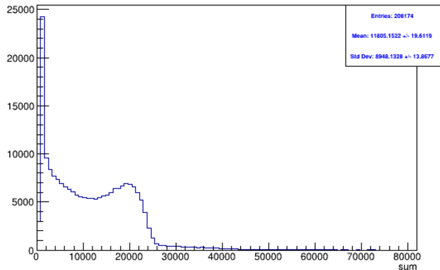
Run 5296 triggerwise, sums: All
