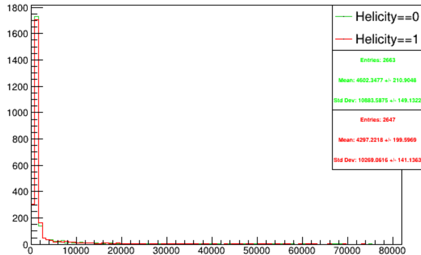
Run 5296 triggerwise, sums: Beam ON, Laser OFF
