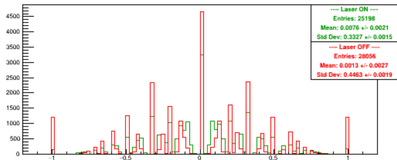
Run 5297 quartetwise, Asyms Horiz Finger
