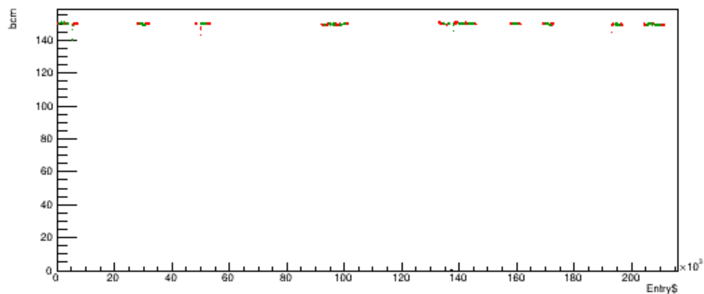
Run 5297 quartetwise, posH4 vs time
