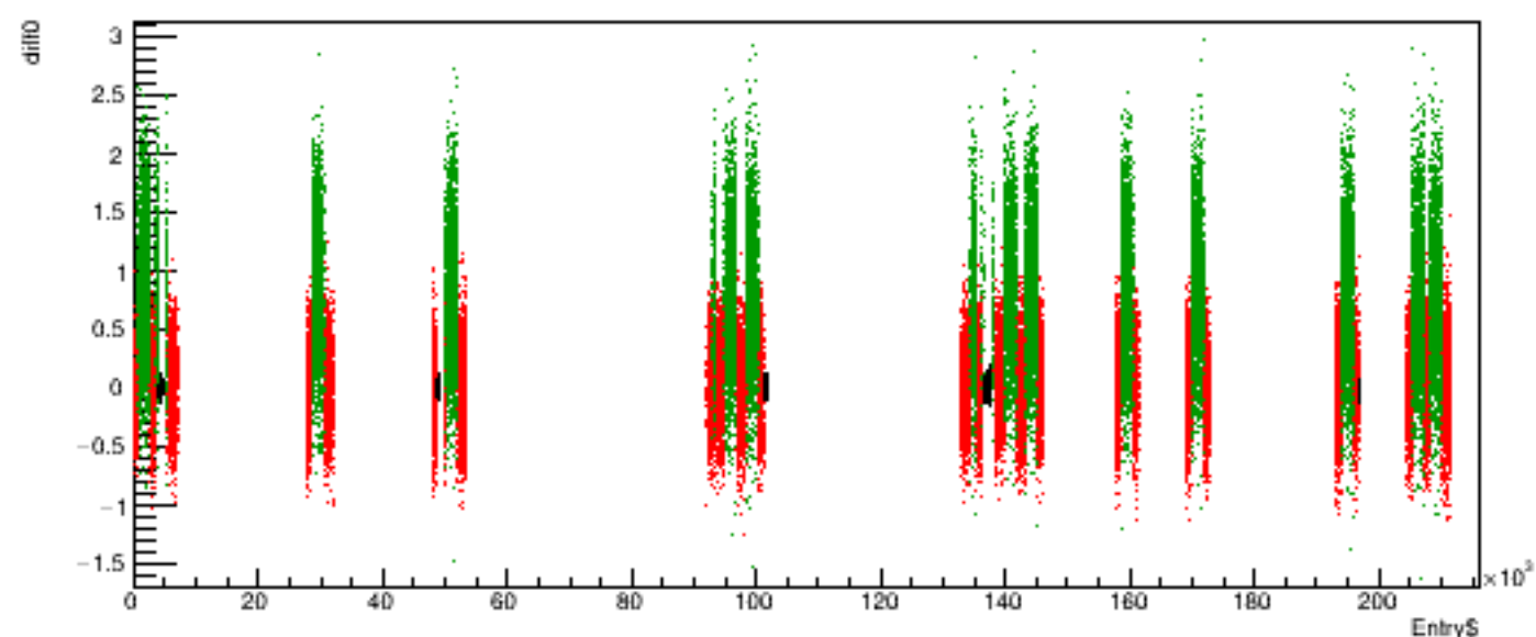
Run 5297 quartetwise, diff0 vs time
