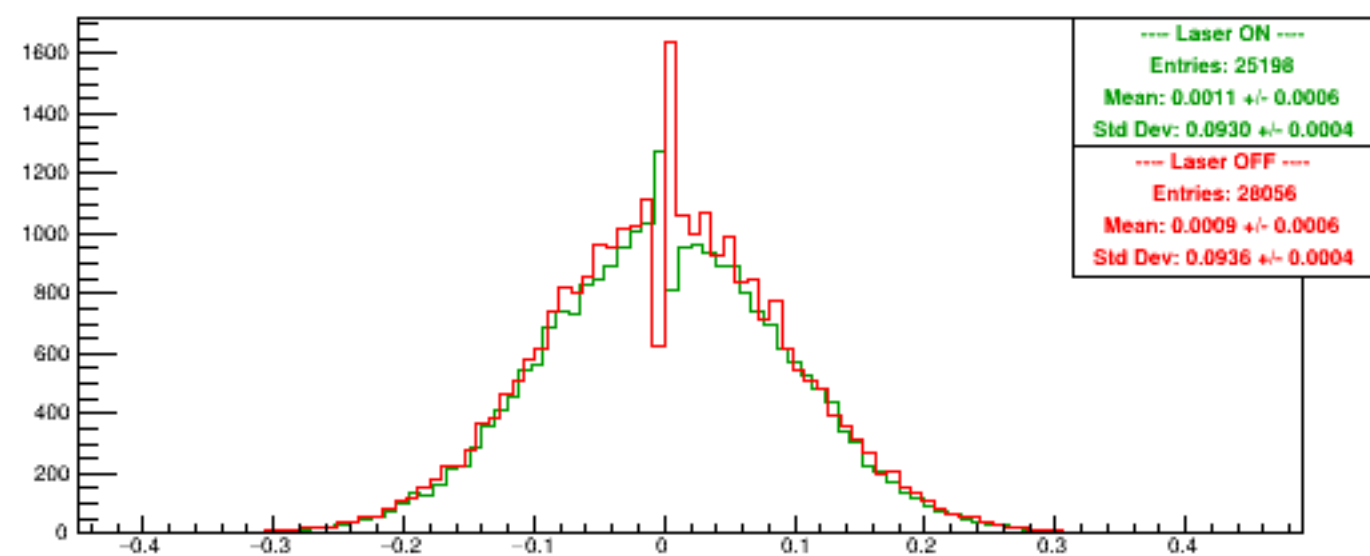
Run 5297 quartetwise, Asyms DSbg1
