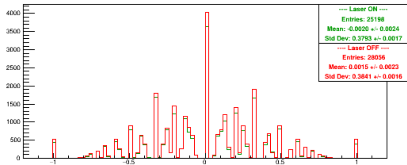
Run 5297 quartetwise, Asyms USbg1
