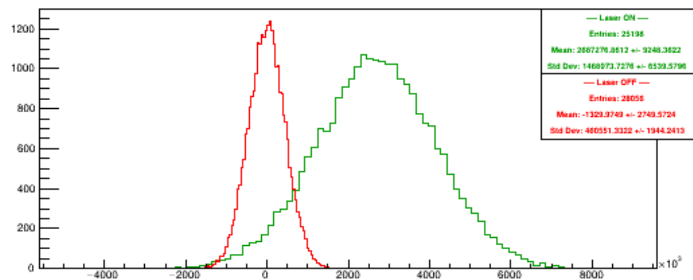
Run 5297 quartetwise, Diffs4
