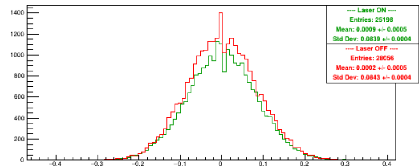
Run 5297 quartetwise, Asyms DSbg2
