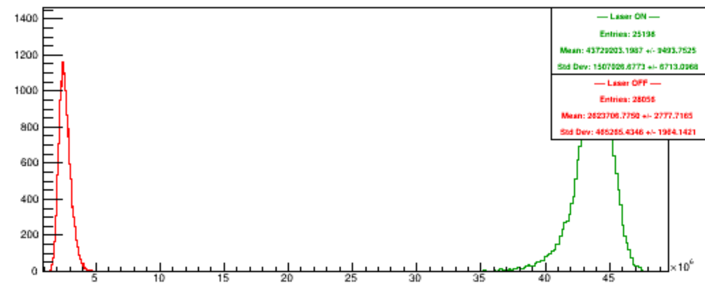
Run 5297 quartetwise, NegHelAcc4
