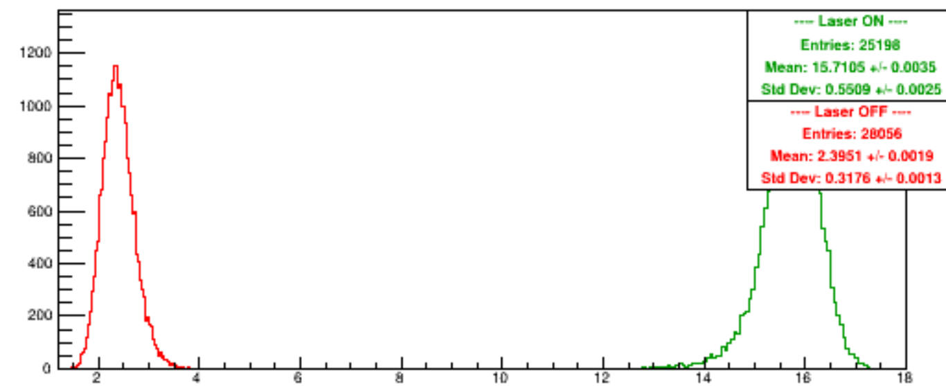
Run 5297 quartetwise, NegHelAcc0/NSamples0
