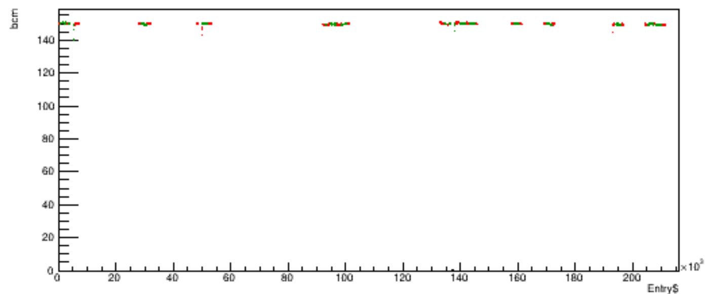
Run 5297 quartetwise, posH4 vs time
