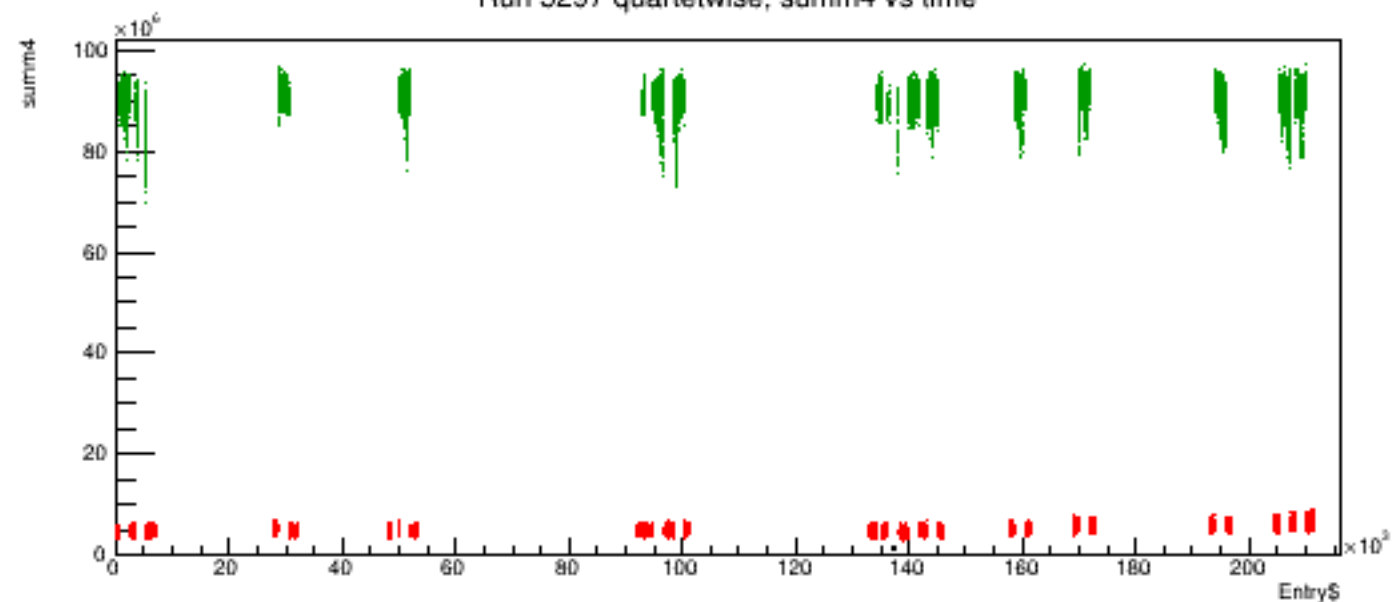
Run 5297 quartetwise, summ4 vs time
