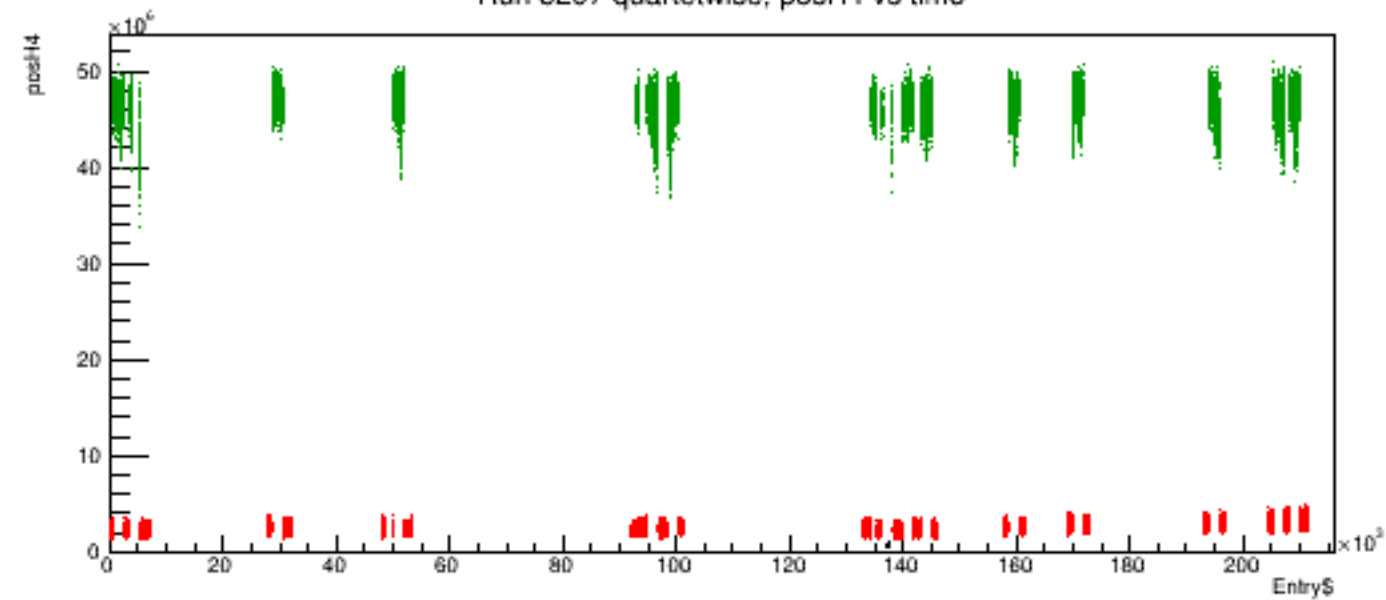
Run 5297 quartetwise, posH4 vs time
