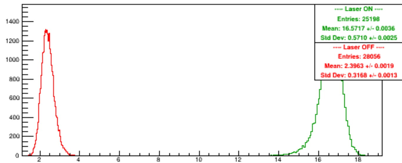
Run 5297 quartetwise, PosHelAcc0/NSamples0
