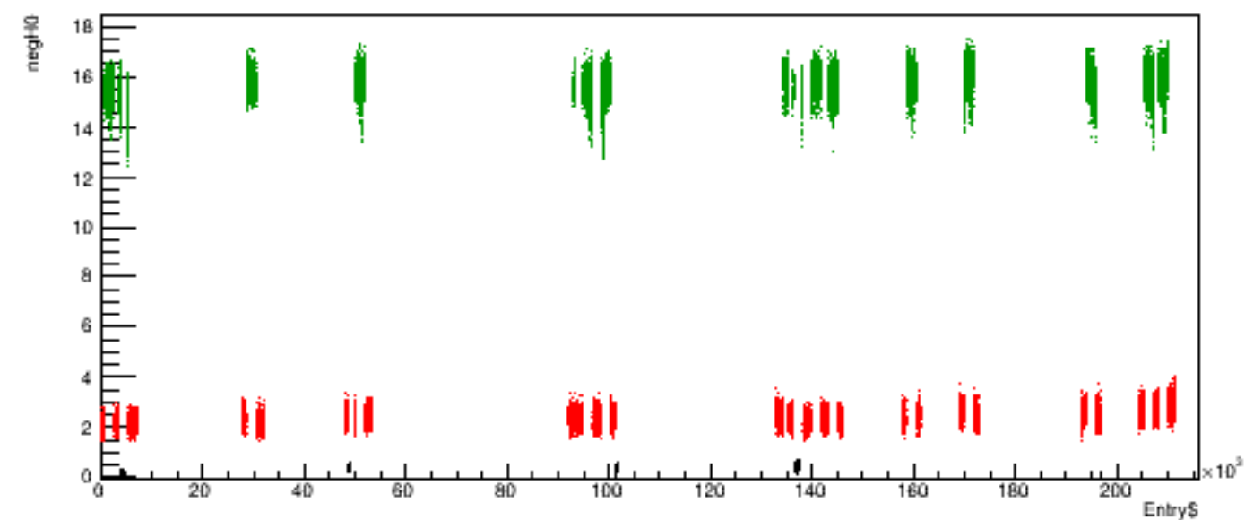
Run 5297 quartetwise, negH0 vs time
