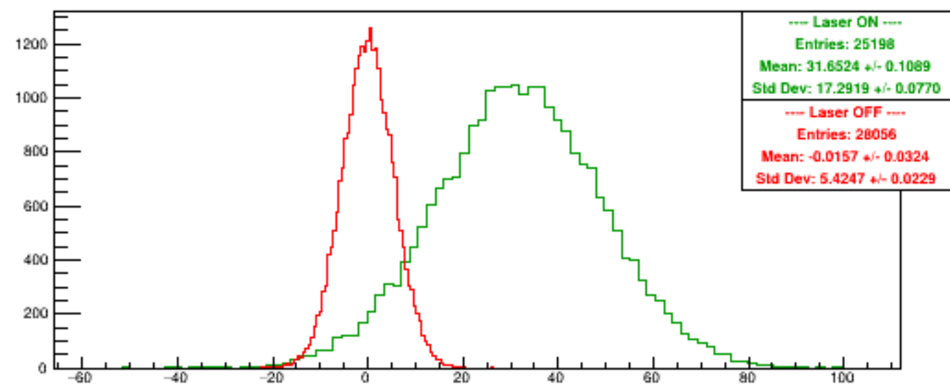
Run 5297 quartetwise, Asyms4
