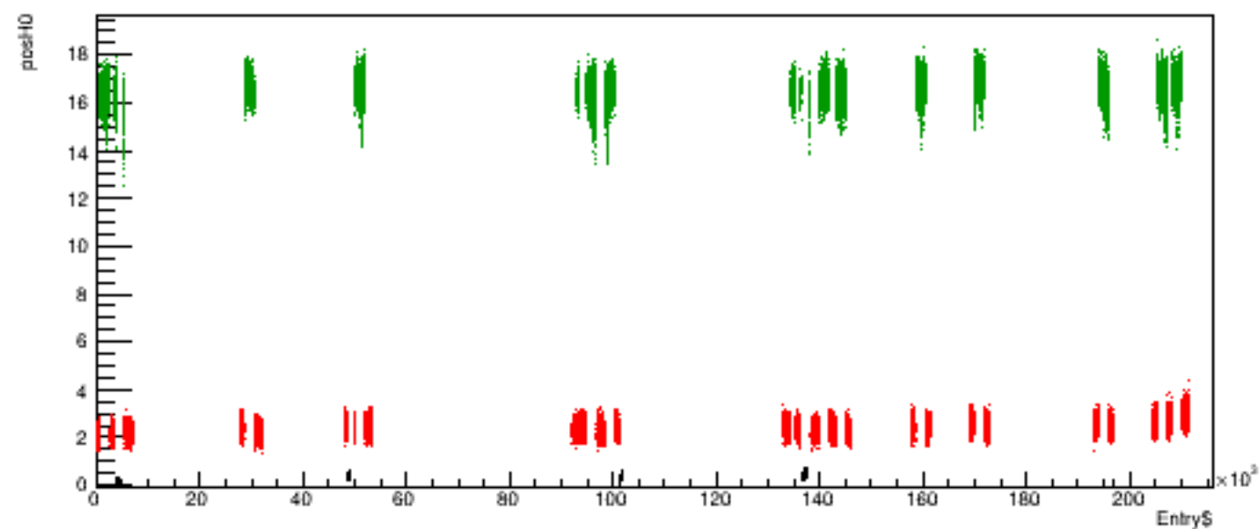
Run 5297 quartetwise, posH0 vs time
