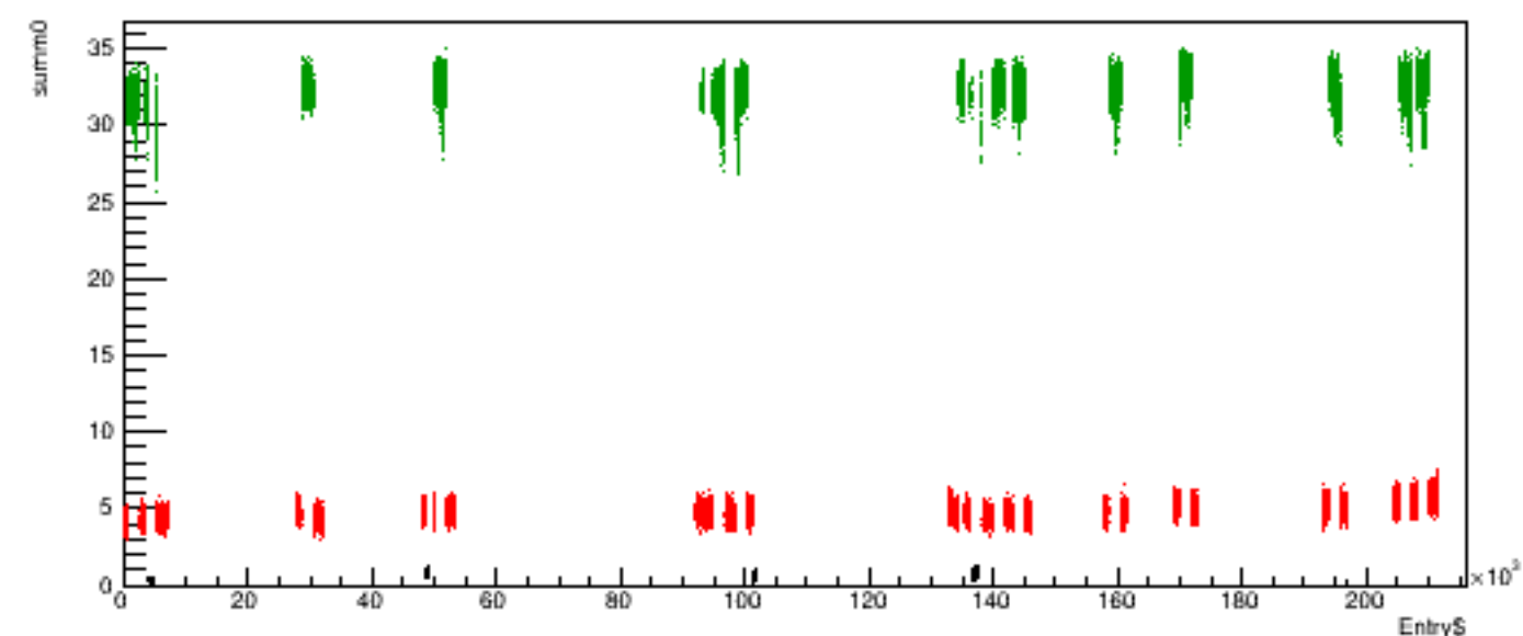
Run 5297 quartetwise, summ0 vs time
