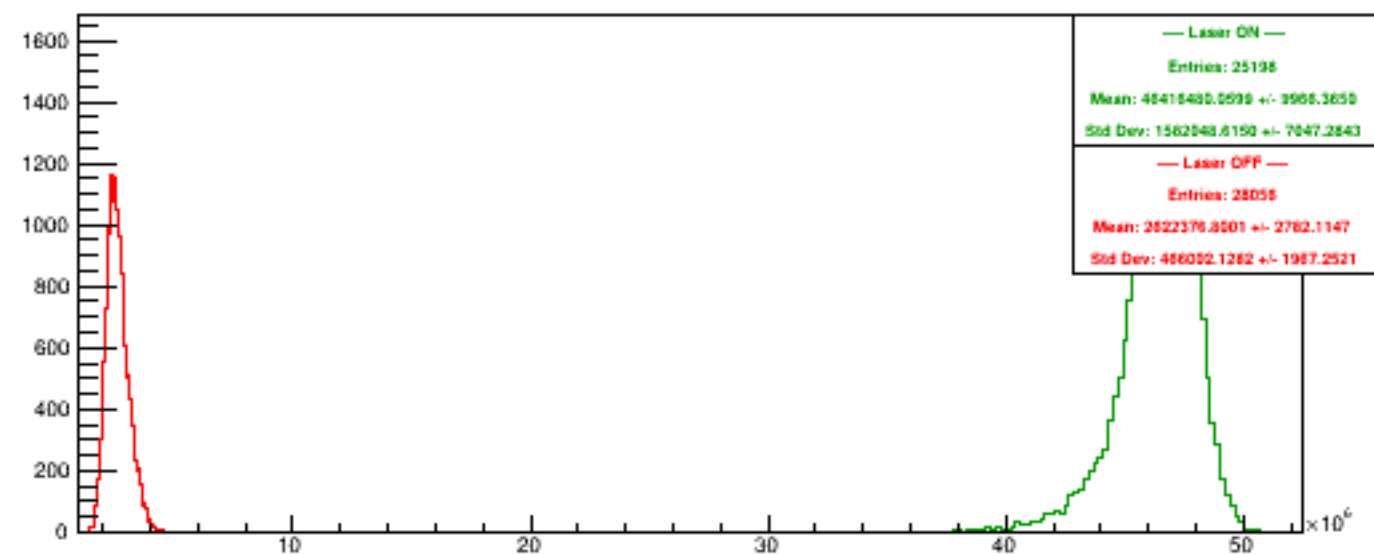
Run 5297 quartetwise, PosHelAcc4
