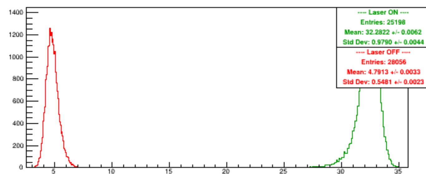
Run 5297 quartetwise, Sums0
