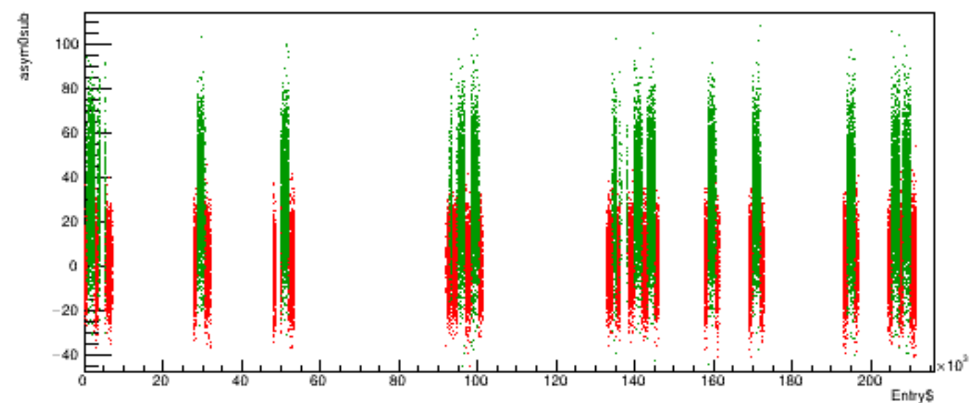
Run 5297 quartetwise, asym0sub vs time
