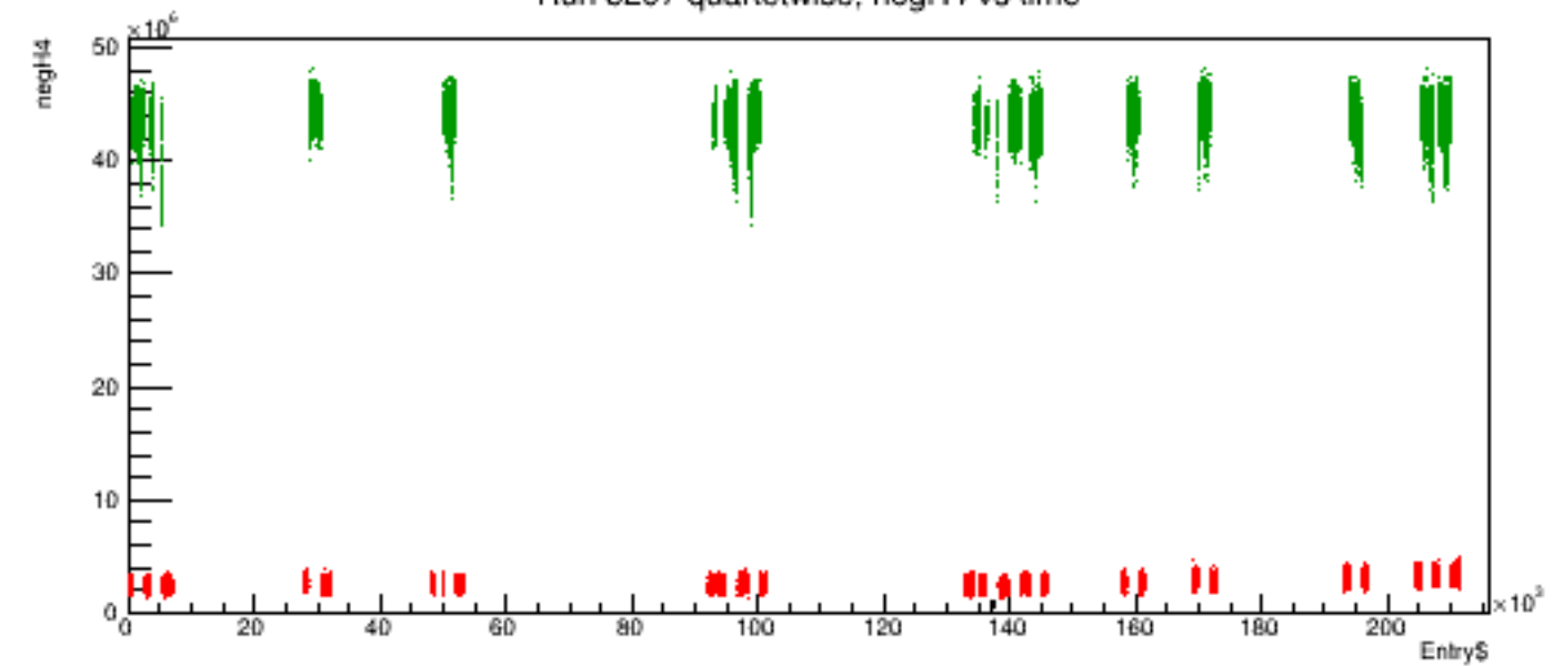
Run 5297 quartetwise, negH4 vs time
