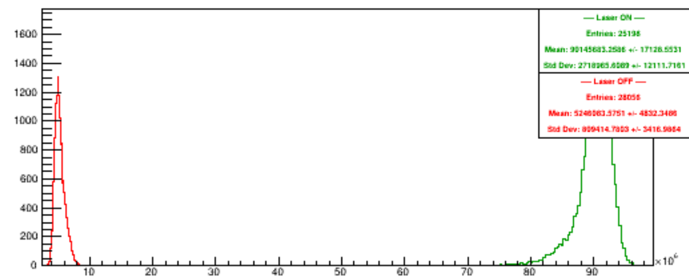
Run 5297 quartetwise, Sums4
