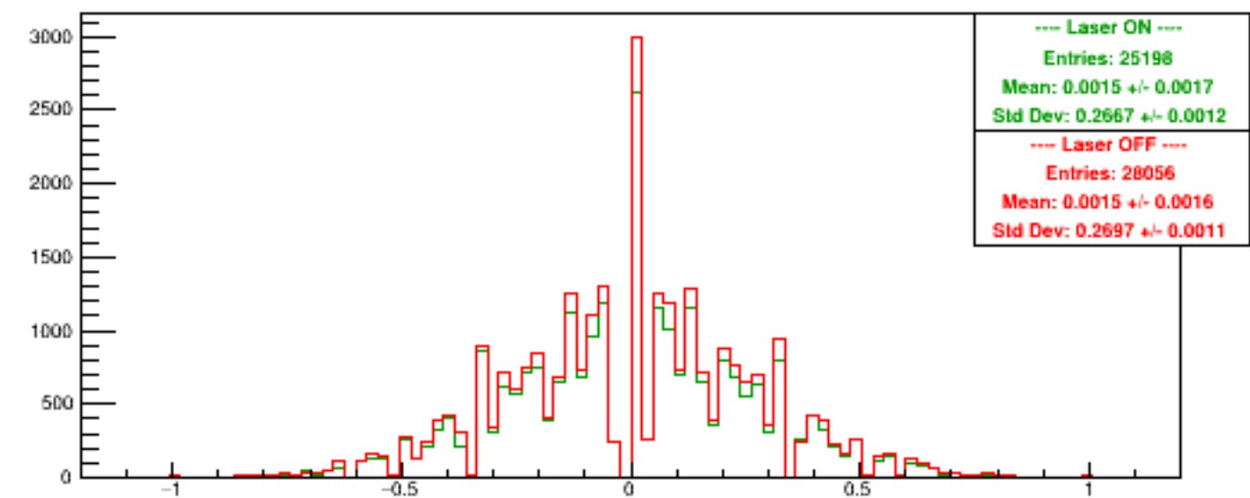
Run 5297 quartetwise, Asyms USbg2
