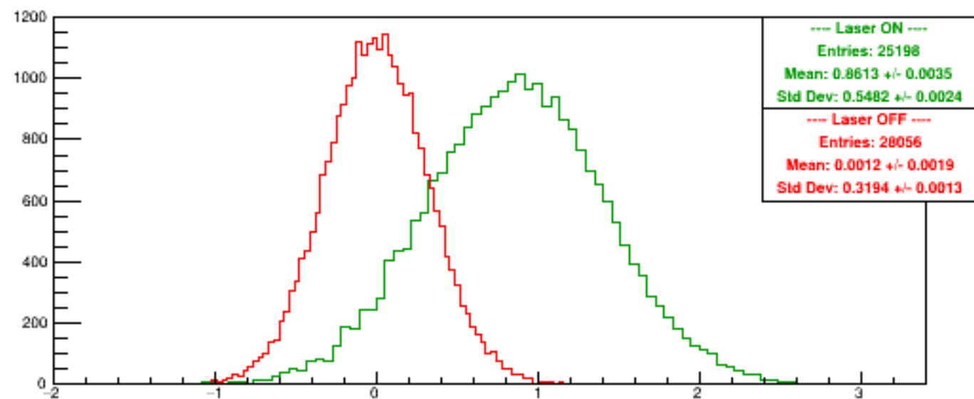
Run 5297 quartetwise, Diffs0
