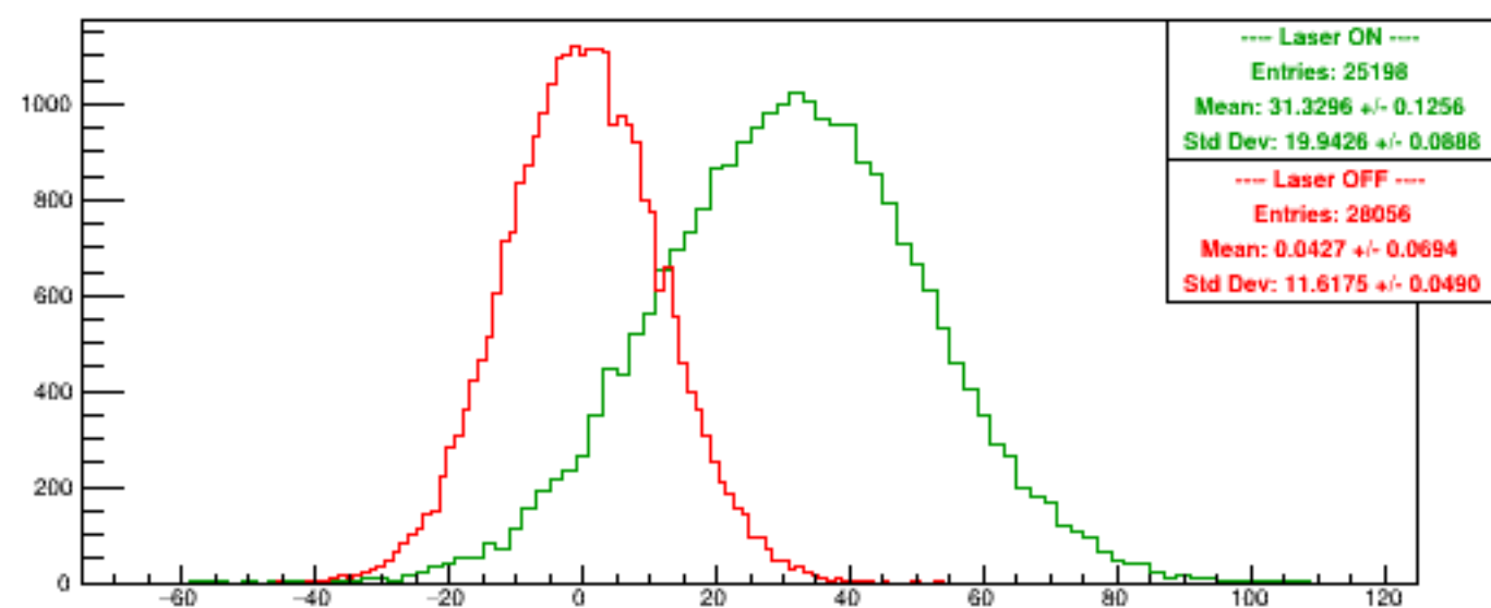
Run 5297 quartetwise, Asyms0
