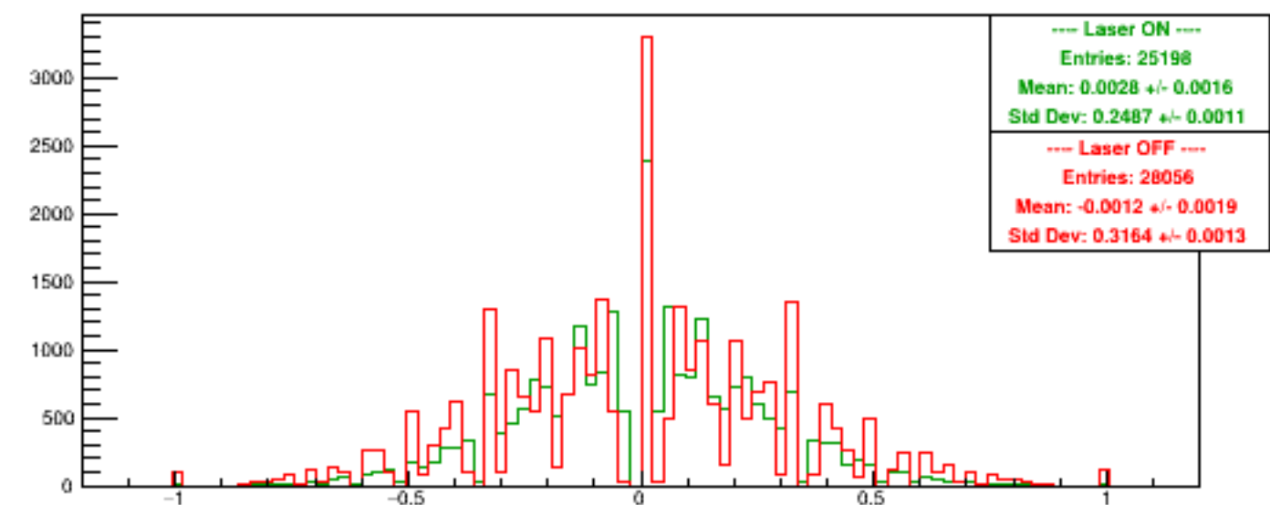
Run 5297 quartetwise, Asyms Vert Finger
