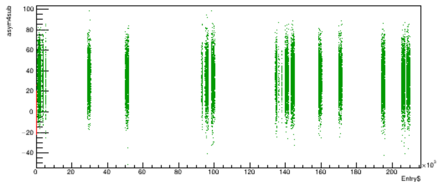
Run 5297 quartetwise, asym4sub vs time
