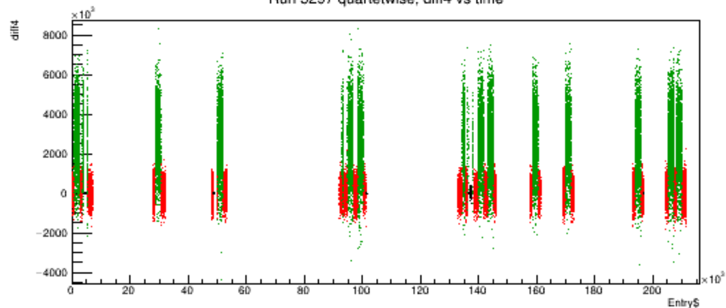
Run 5297 quartetwise, diff4 vs time
