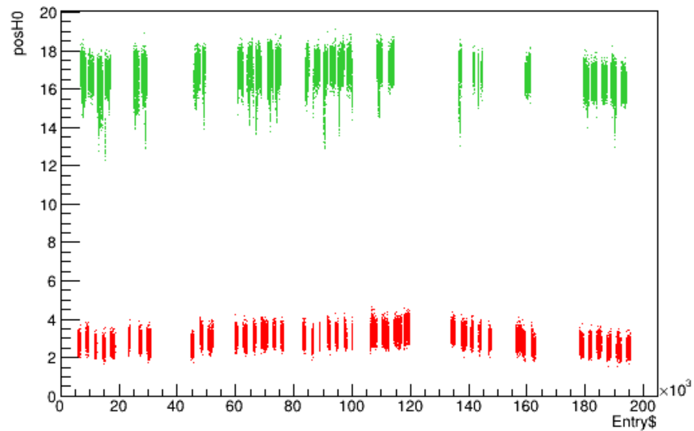
Run 5301 quartetwise, posH0 vs time
