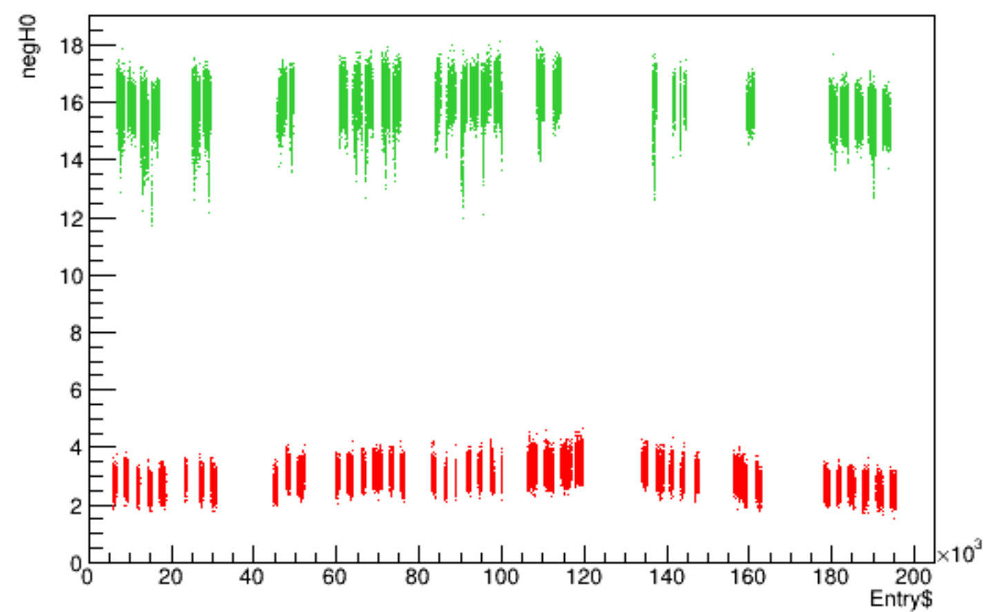
Run 5301 quartetwise, negH0 vs time
