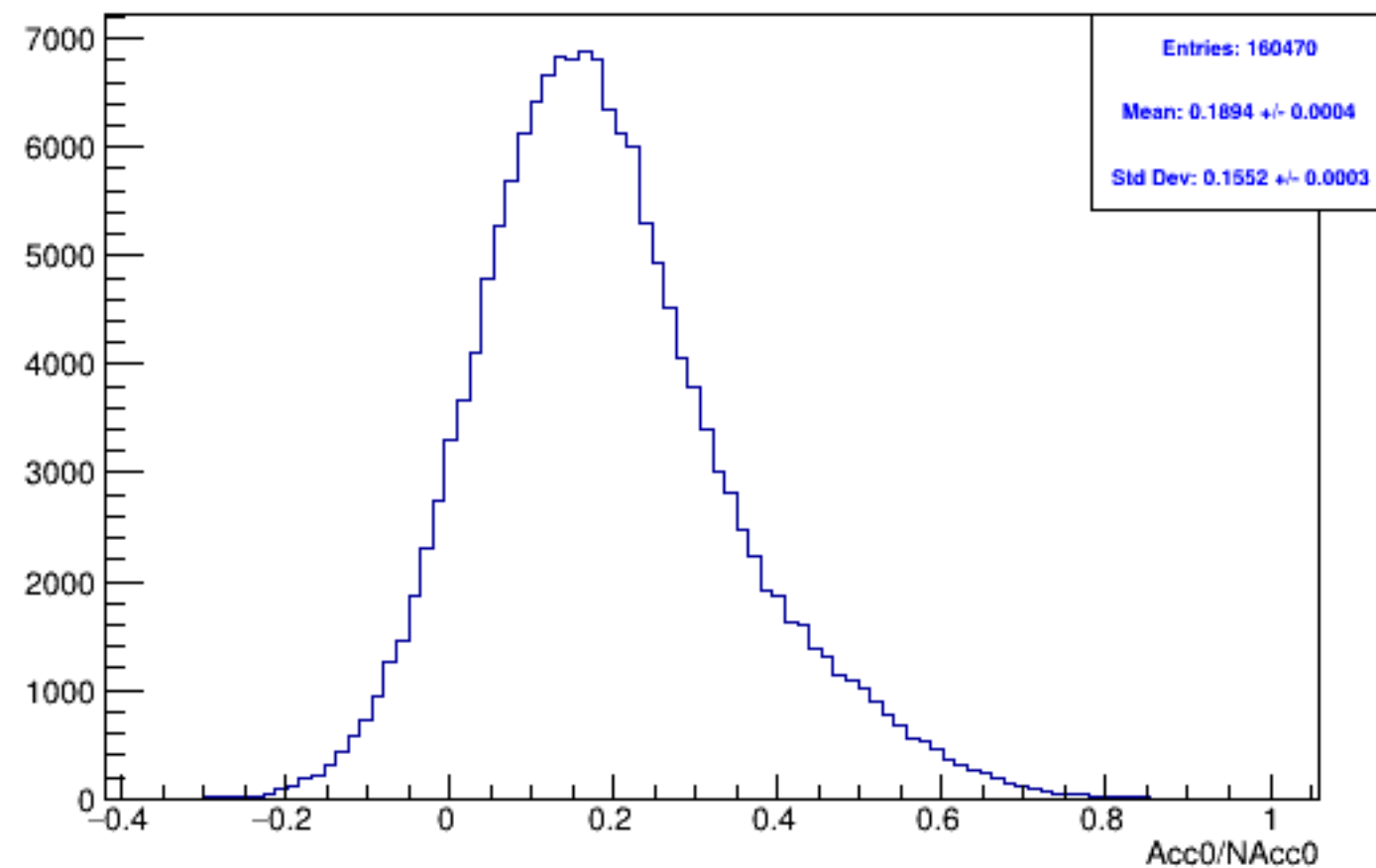
Run 5302 mpwise, acc0: Beam OFF
