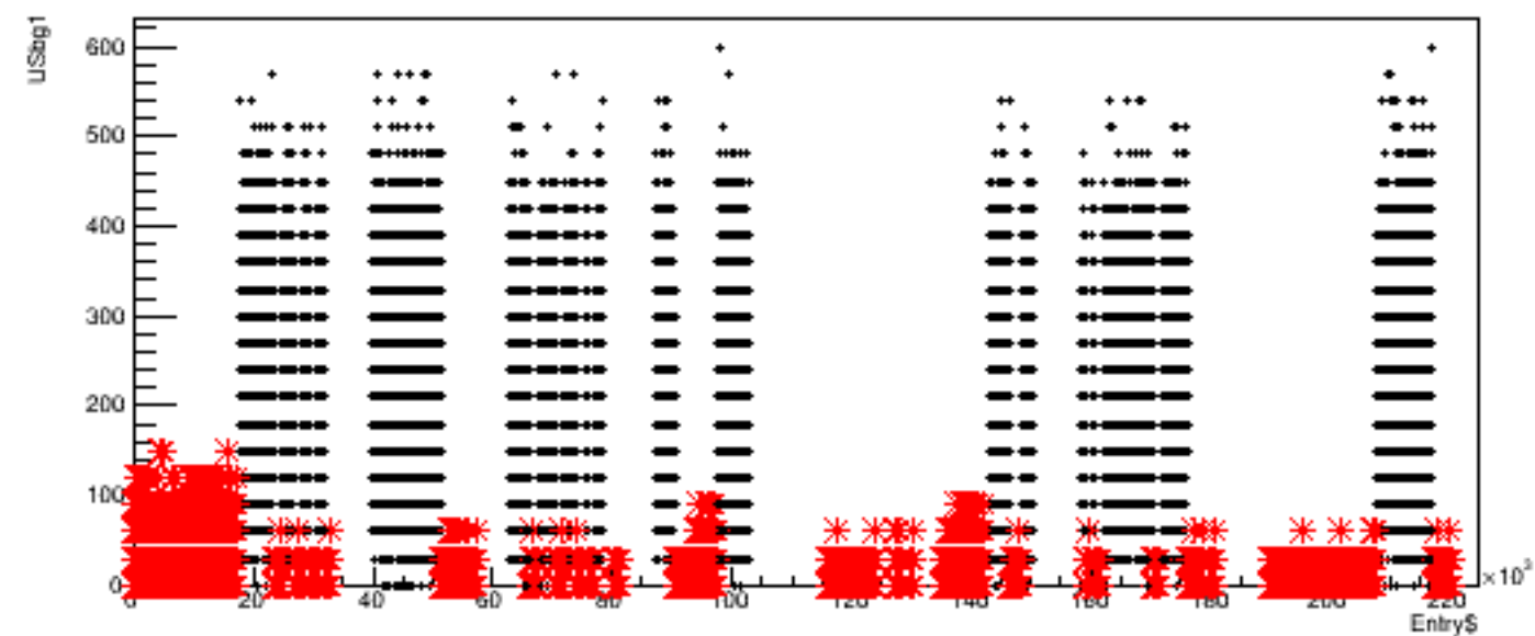
Run 5305, quartetwise: USbg1 vs time
