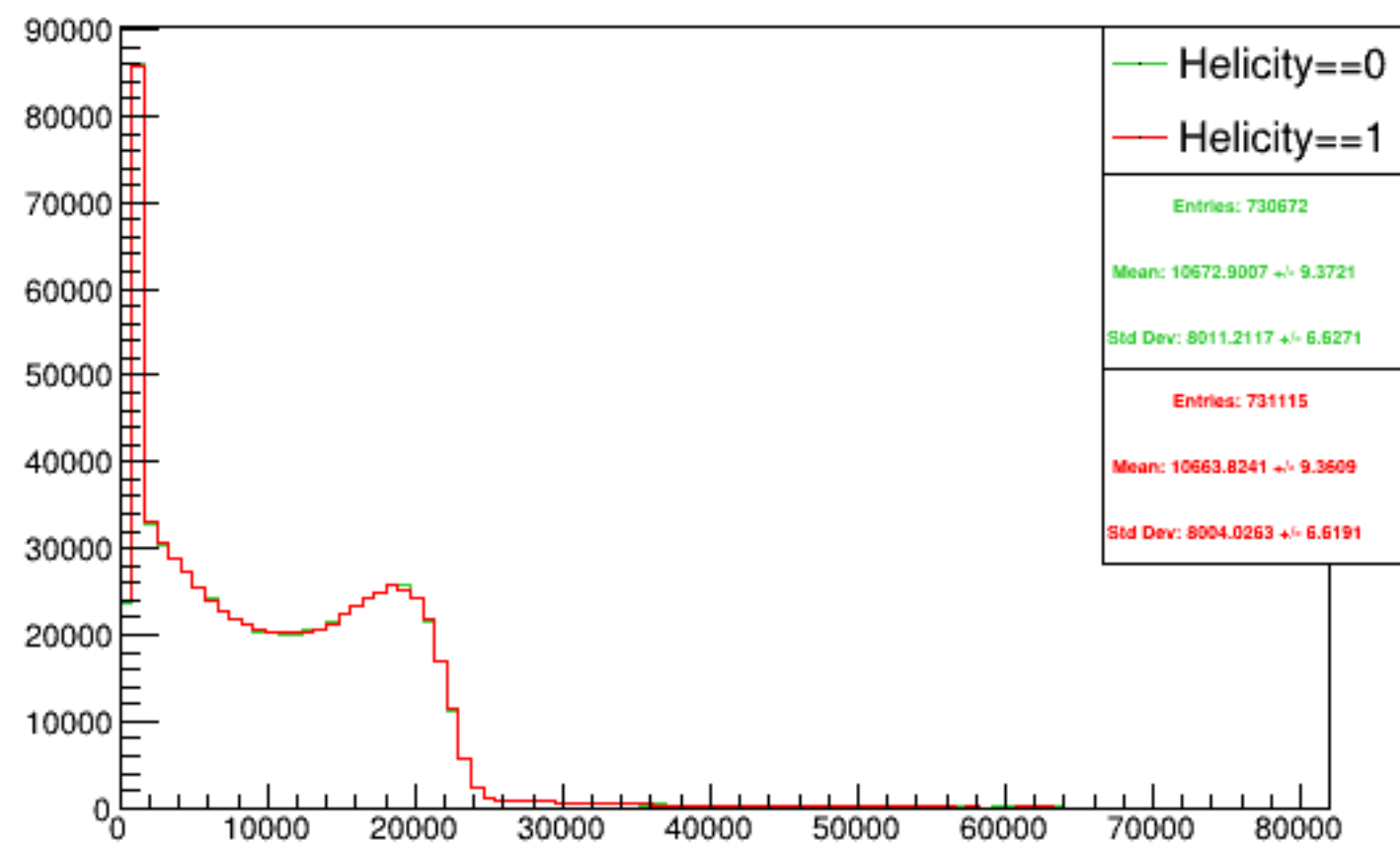
Run 5305 triggerwise, sums: Beam ON, Laser ON
