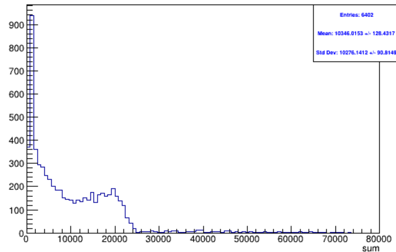
Run 5305 triggerwise, sums: Beam OFF
