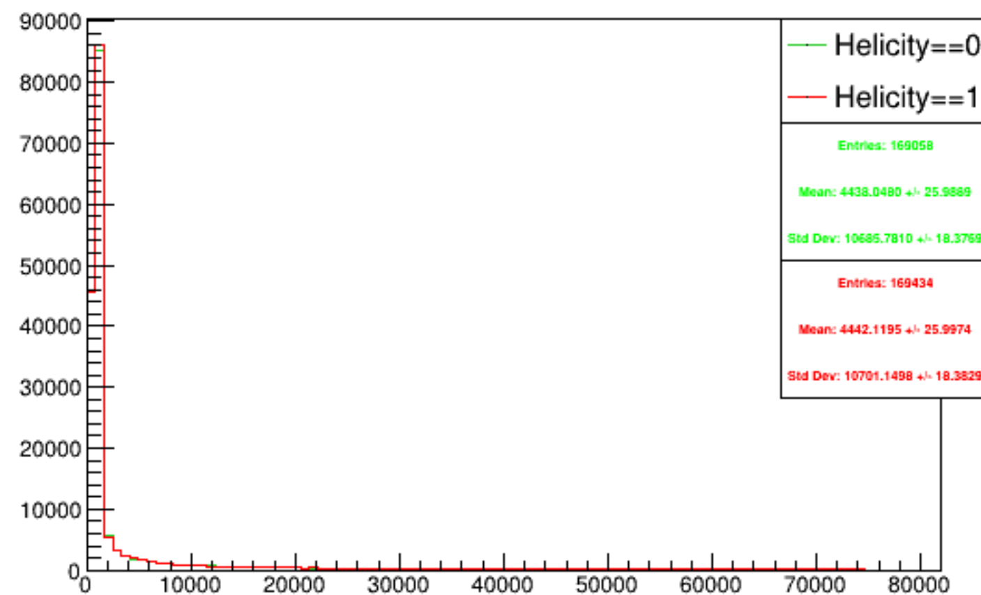
Run 5305 triggerwise, sums: Beam ON, Laser OFF
