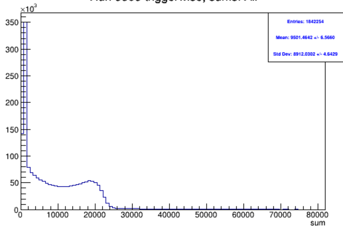
Run 5305 triggerwise, sums: All
