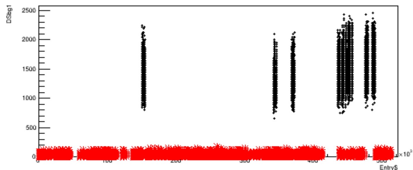
Run 5316, quartetwise: DSbg1 vs time
