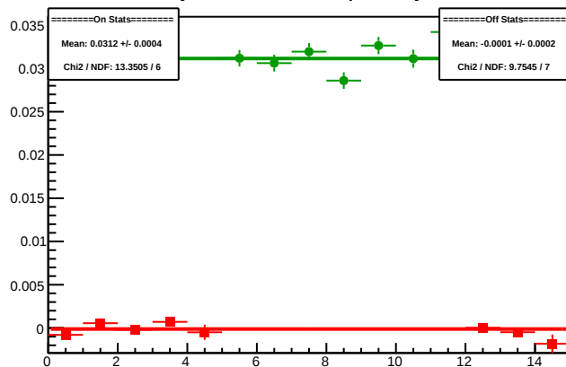
Cycle 5319.7: Multiplet Asyms
