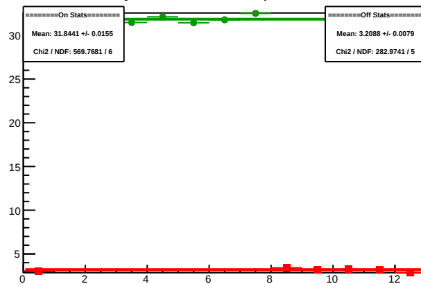
Cycle 5319.12: Multiplet Sums
