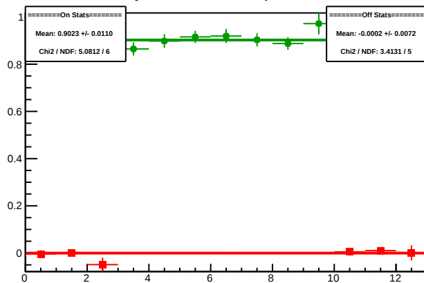
Cycle 5319.8: Multiplet Diffs
