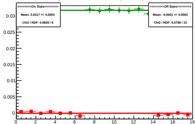
Cycle 5319.20: Multiplet Asyms
