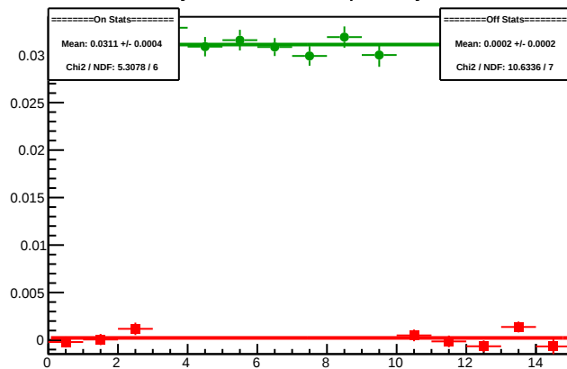
Cycle 5319.1: Multiplet Asyms
