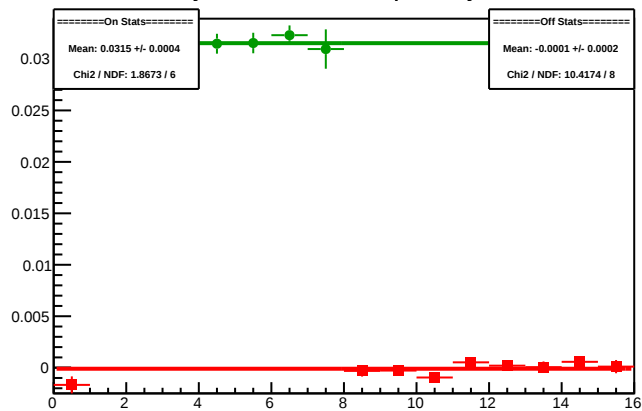
Cycle 5319.13: Multiplet Asyms
