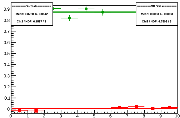
Cycle 5319.18: Multiplet Diffs
