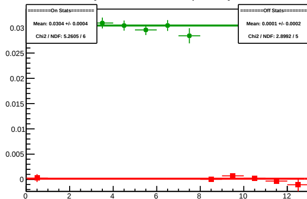
Cycle 5319.12: Multiplet Asyms
