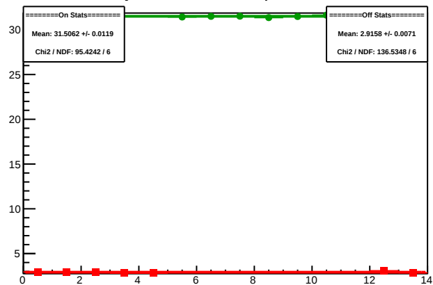
Cycle 5319.17: Multiplet Sums
