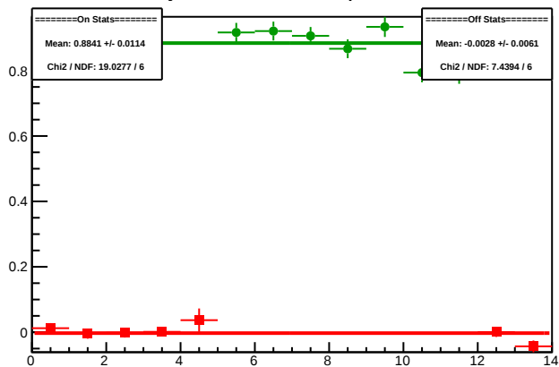
Cycle 5319.17: Multiplet Diffs
