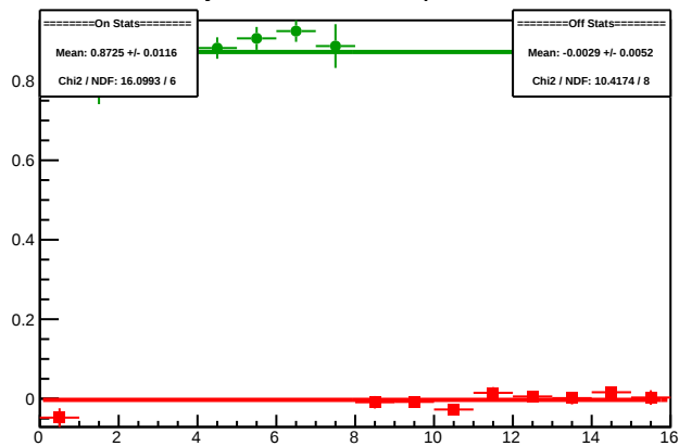
Cycle 5319.13: Multiplet Diffs
