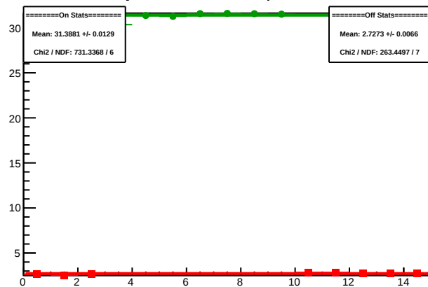
Cycle 5319.15: Multiplet Sums
