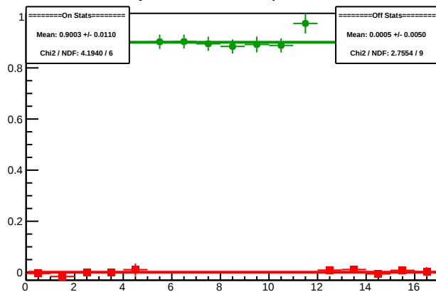
Cycle 5319.6: Multiplet Diffs
