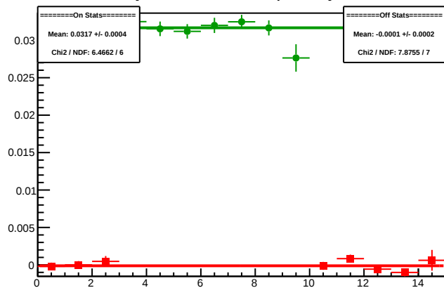
Cycle 5319.15: Multiplet Asyms
