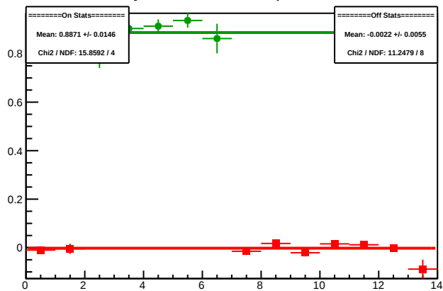
Cycle 5319.10: Multiplet Diffs
