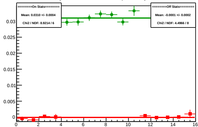
Cycle 5319.16: Multiplet Asyms
