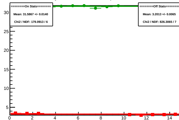
Cycle 5319.4: Multiplet Sums
