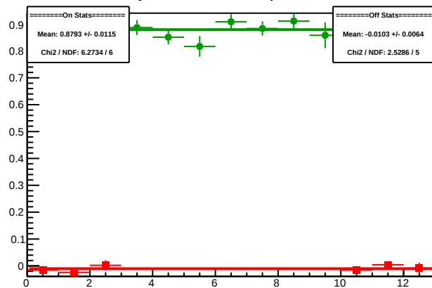
Cycle 5319.3: Multiplet Diffs
