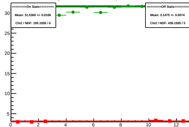
Cycle 5319.2: Multiplet Sums
