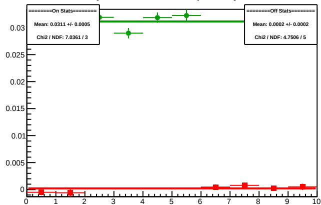
Cycle 5319.18: Multiplet Asyms
