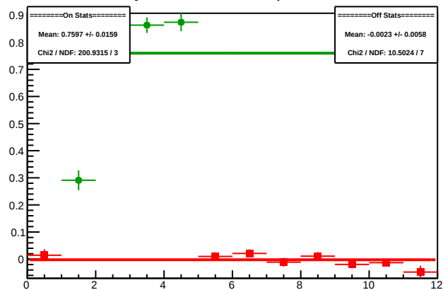
Cycle 5319.14: Multiplet Diffs
