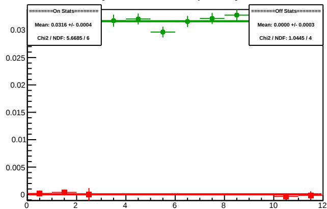
Cycle 5319.9: Multiplet Asyms
