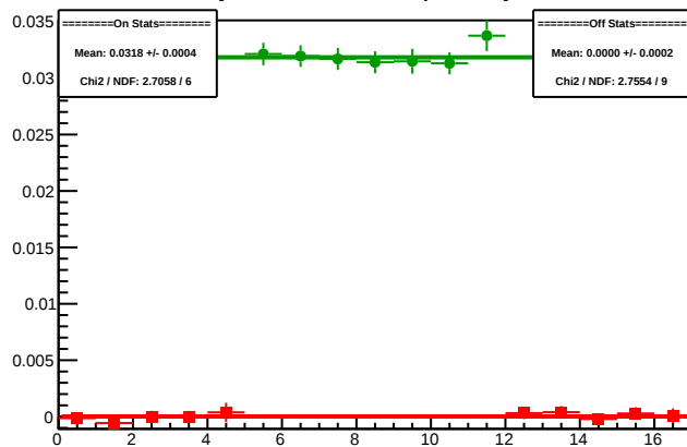
Cycle 5319.6: Multiplet Asyms
