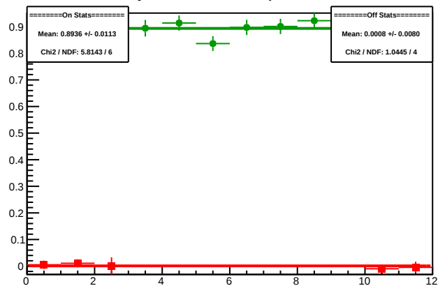
Cycle 5319.9: Multiplet Diffs
