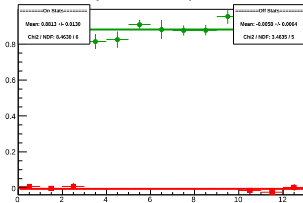
Cycle 5319.2: Multiplet Diffs
