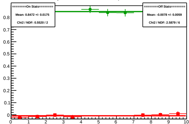
Cycle 5319.21: Multiplet Diffs
