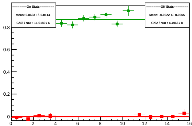
Cycle 5319.16: Multiplet Diffs
