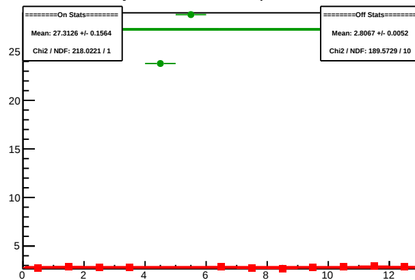
Cycle 5319.19: Multiplet Sums
