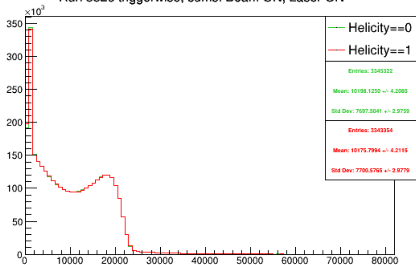
Run 5326 triggerwise, sums: Beam ON, Laser ON
