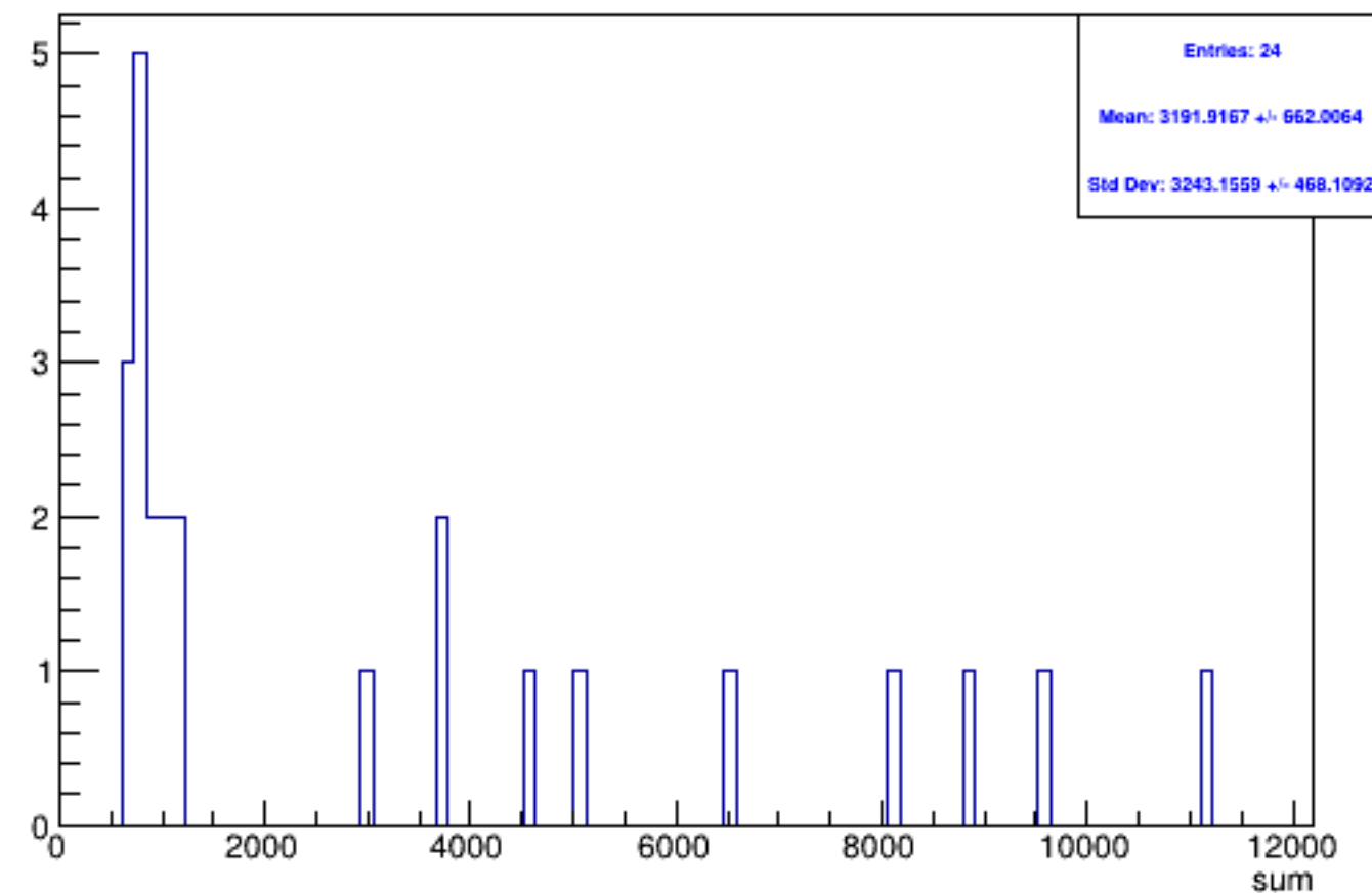
Run 5326 triggerwise, sums: Beam OFF
