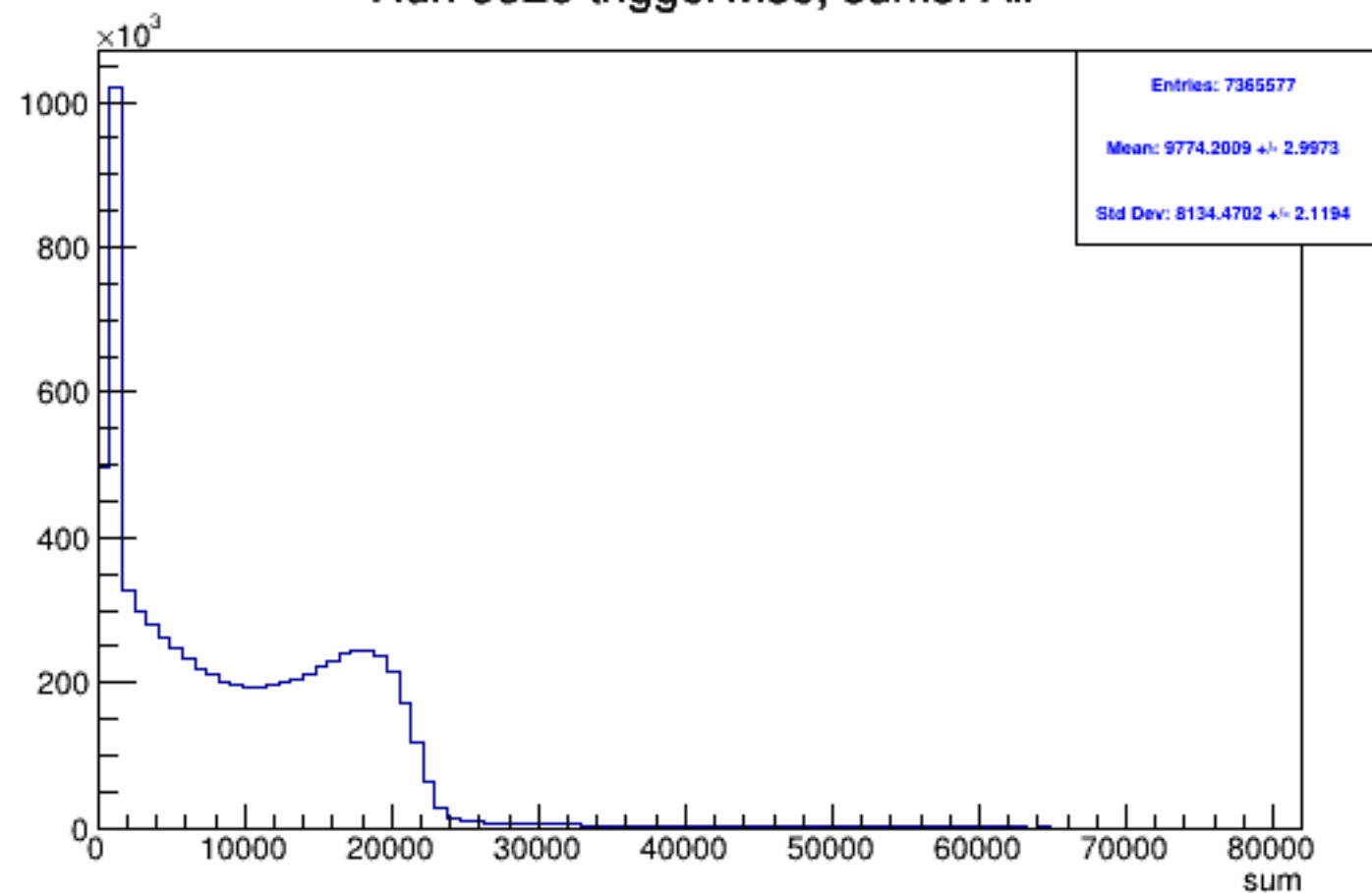
Run 5326 triggerwise, sums: All
