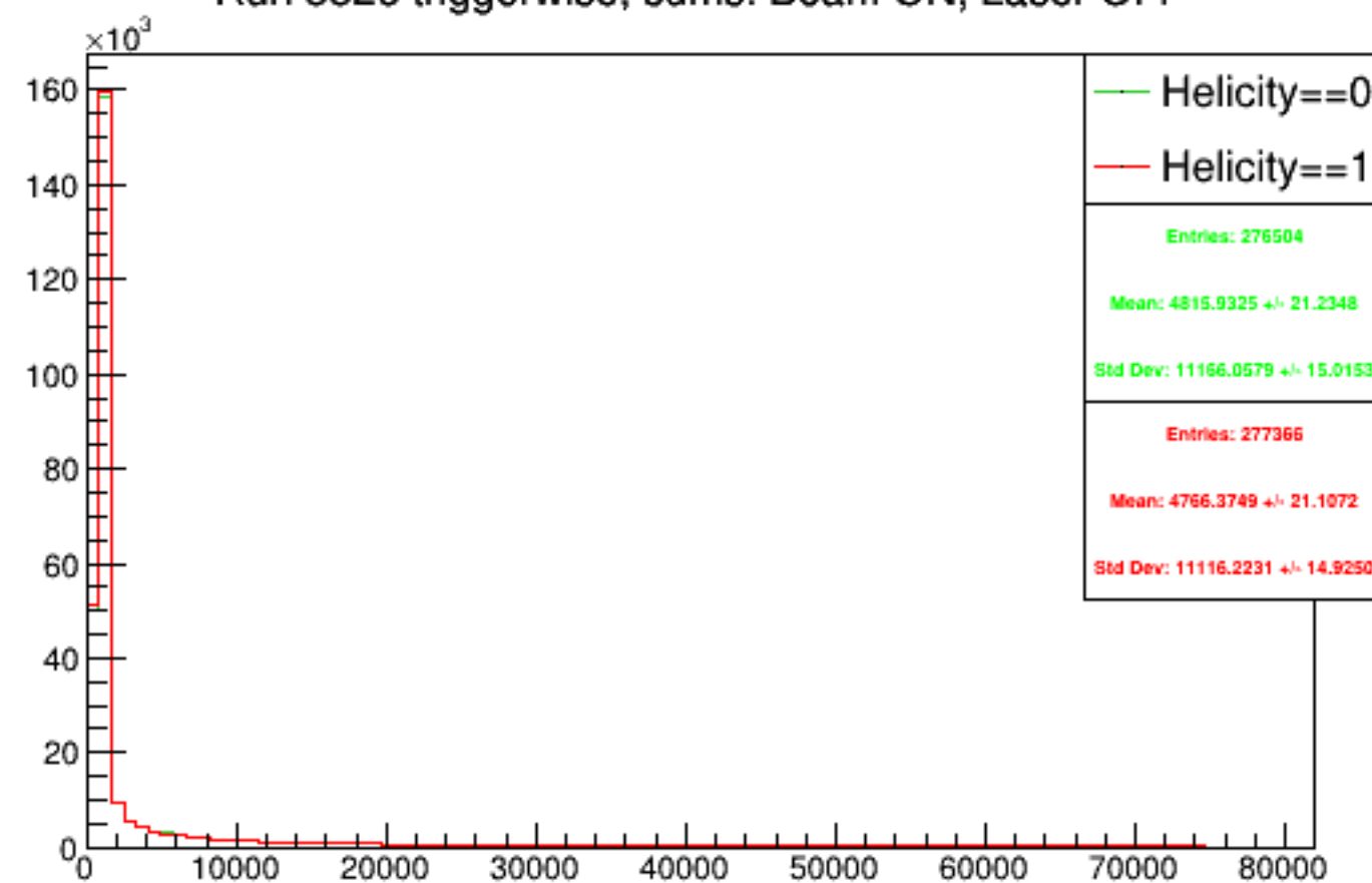
Run 5326 triggerwise, sums: Beam ON, Laser OFF
