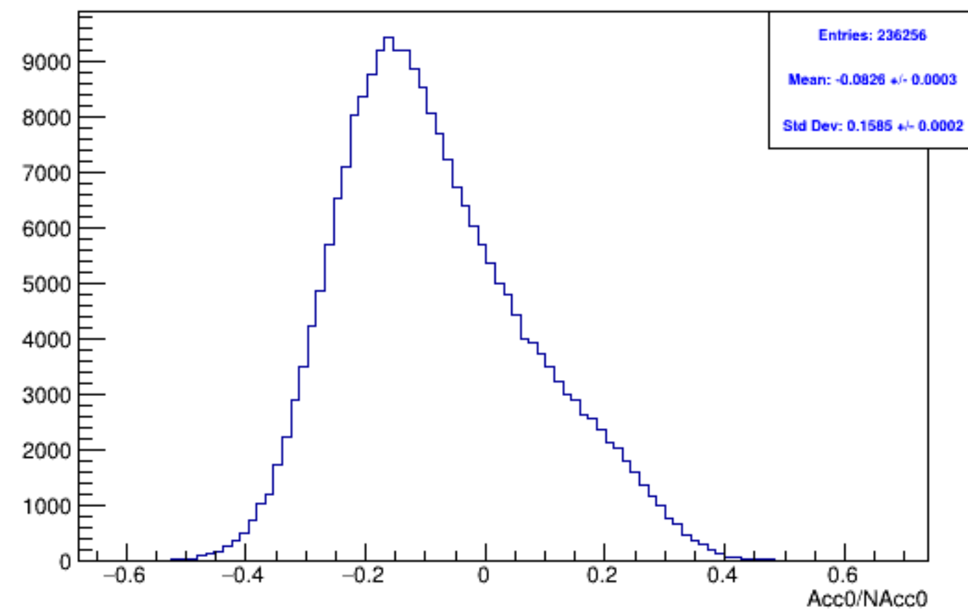
Run 5327 mpwise, acc0: Beam OFF
