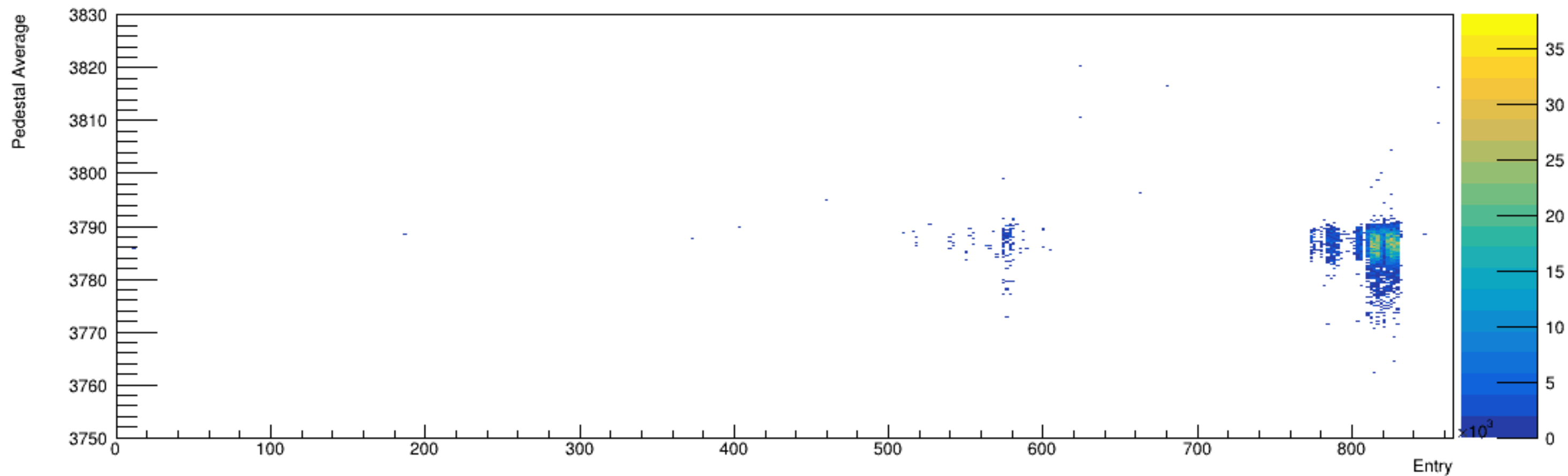
Run 5333, snapshots: Pedestal vs. Time
