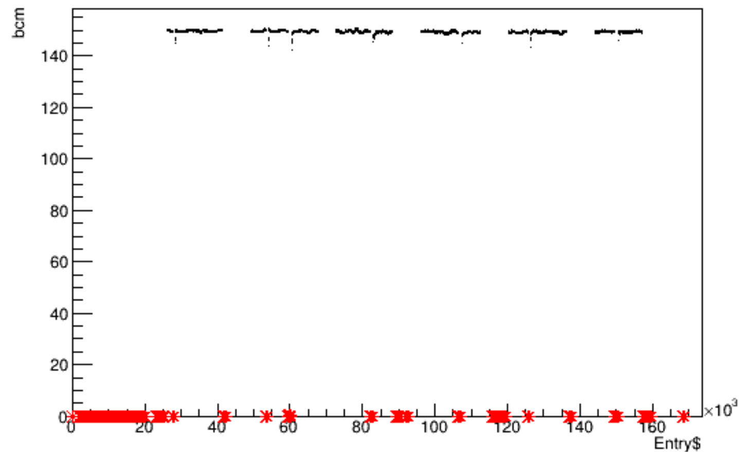
Run 5342 quartetwise, bcm vs time
