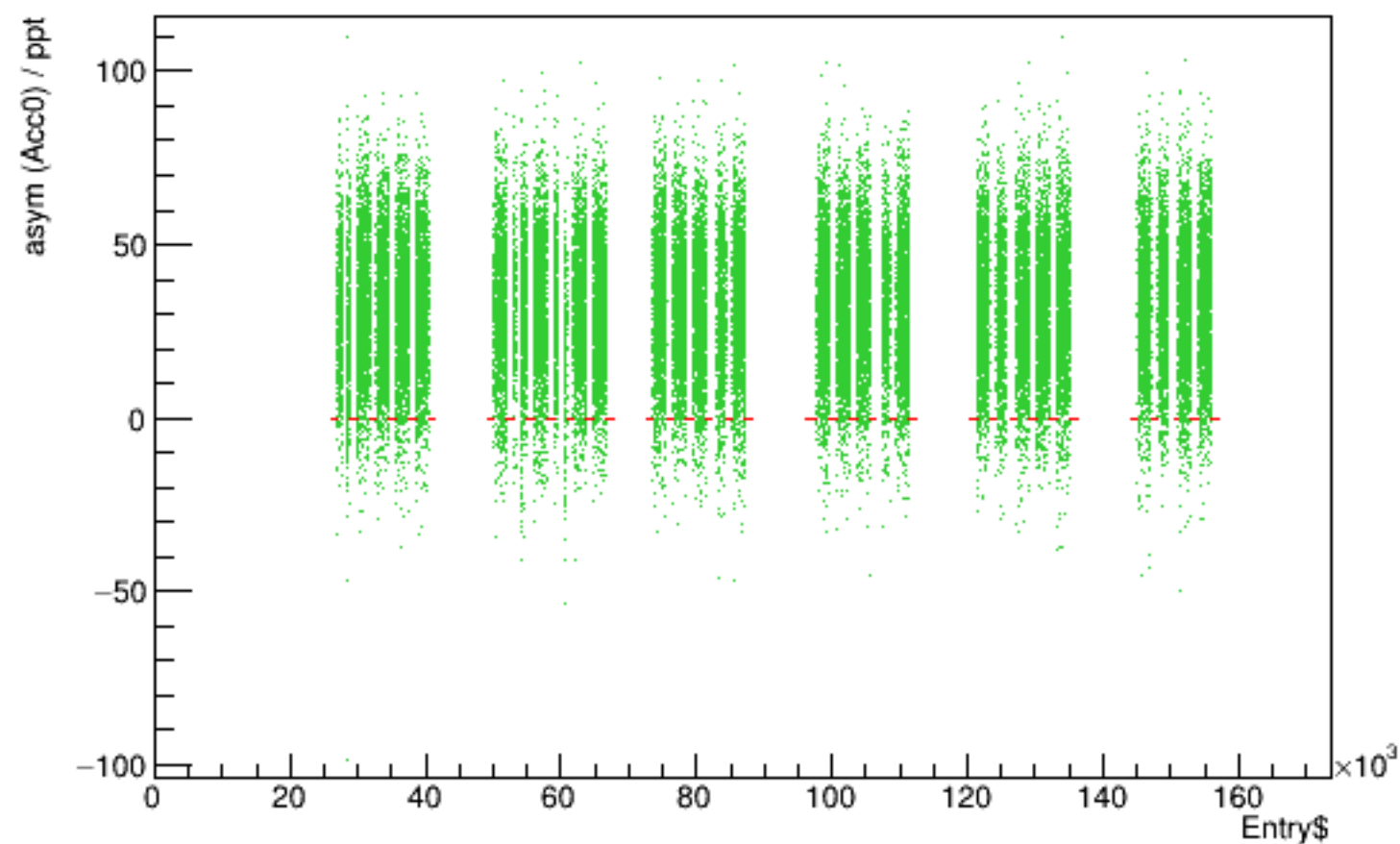
Run 5342 quartetwise, asym0sub vs time
