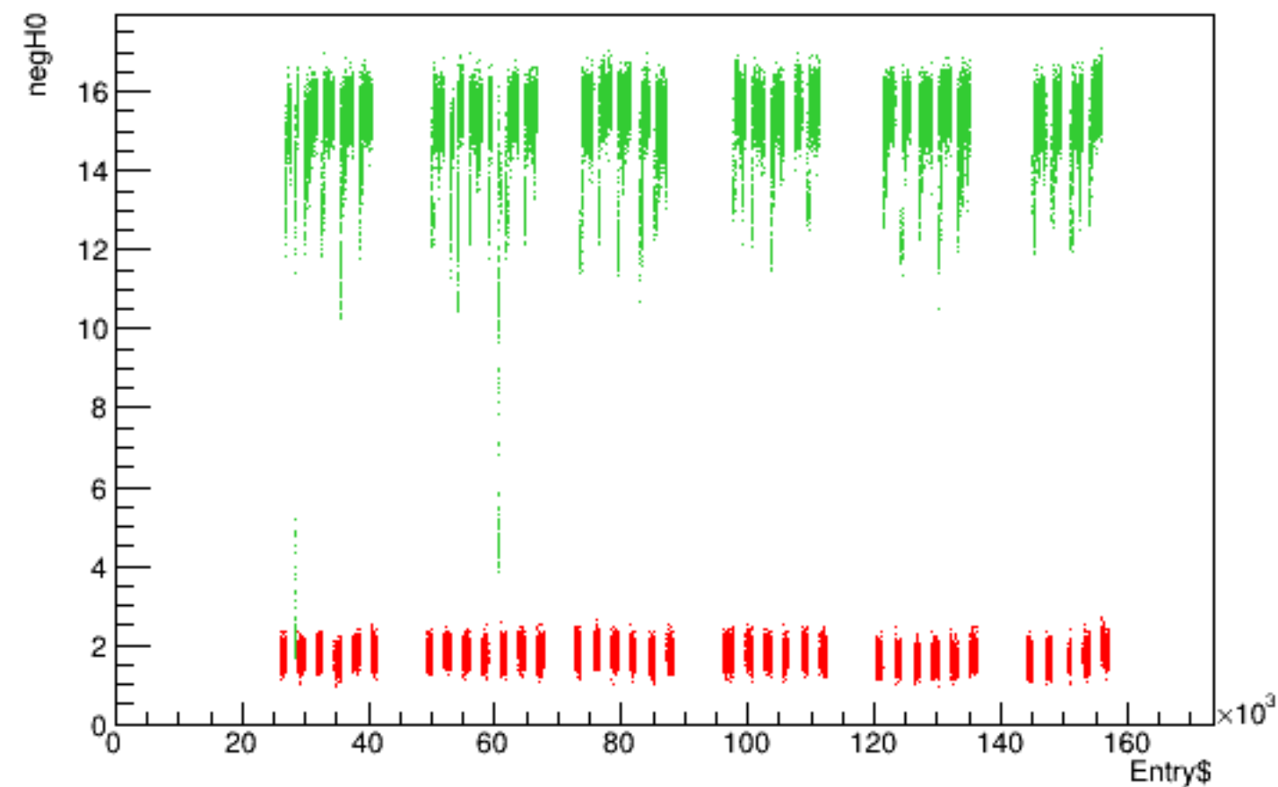
Run 5342 quartetwise, negH0 vs time
