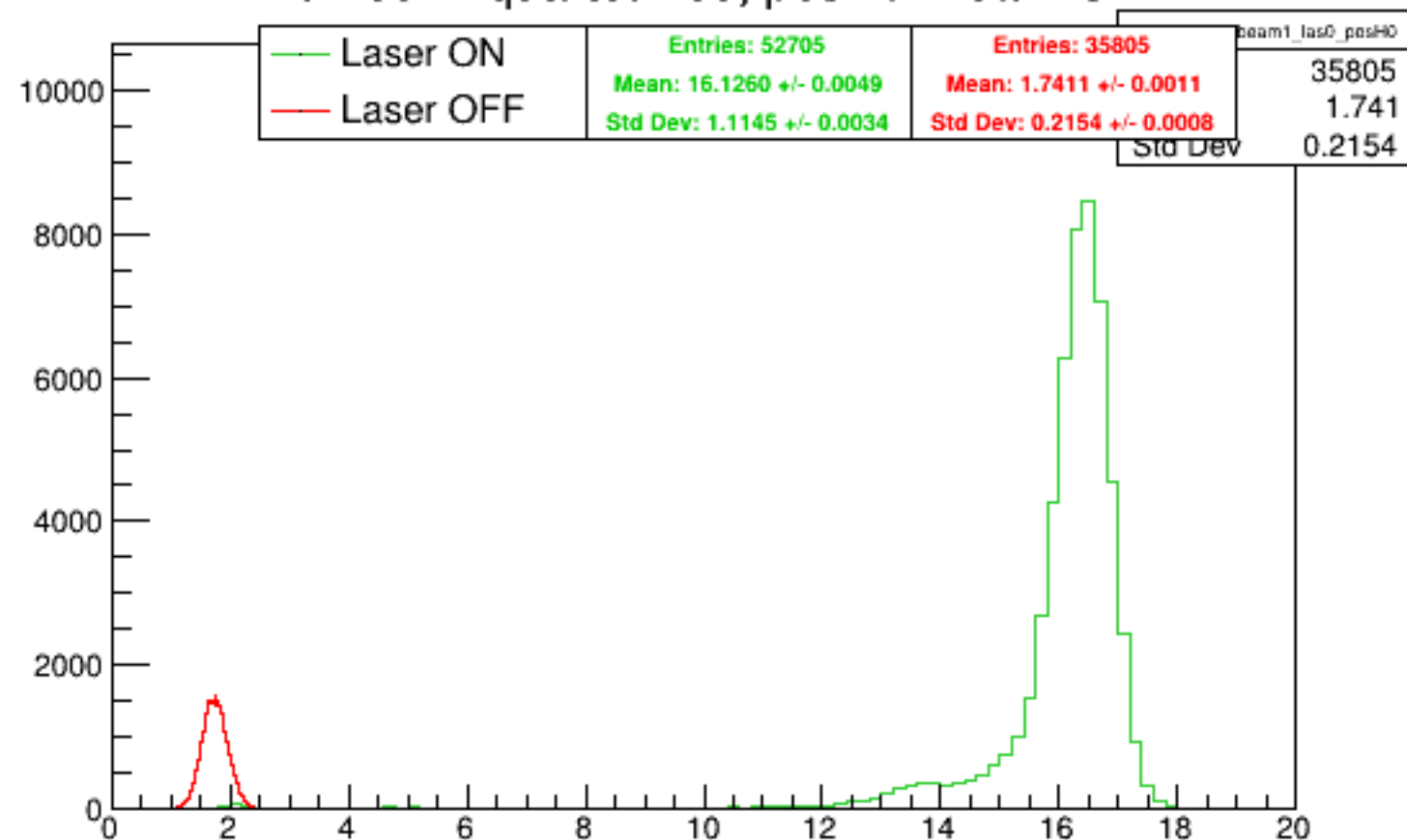
Run 5342 quartetwise, posH0: Beam ON
