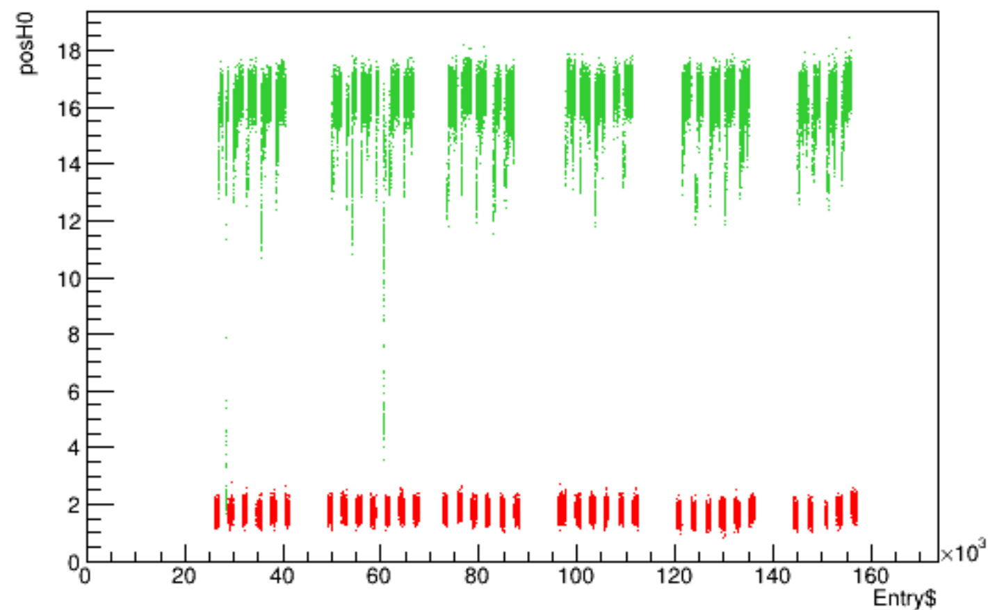
Run 5342 quartetwise, posH0 vs time
