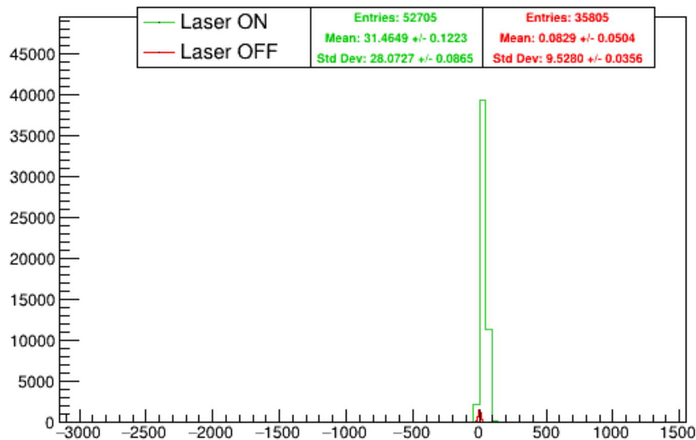
Run 5342 quartetwise, asym0sub: Beam ON
