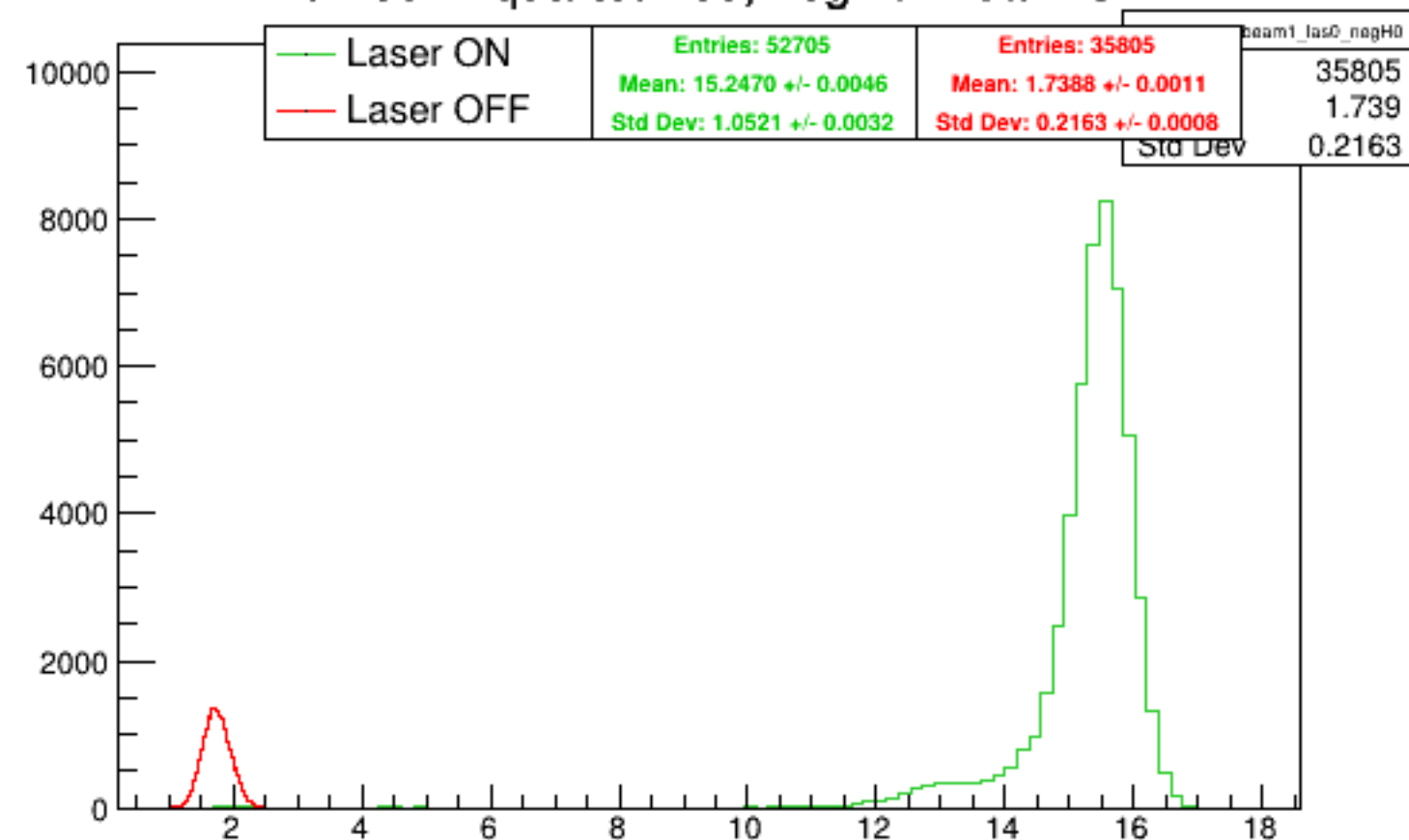
Run 5342 quartetwise, negH0: Beam ON
