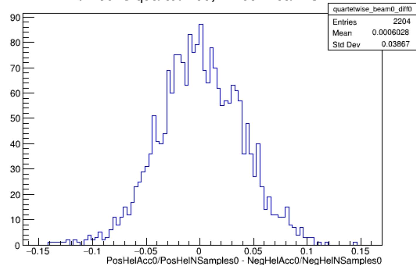
Run 5343 quartetwise, Diffs0: Beam OFF
