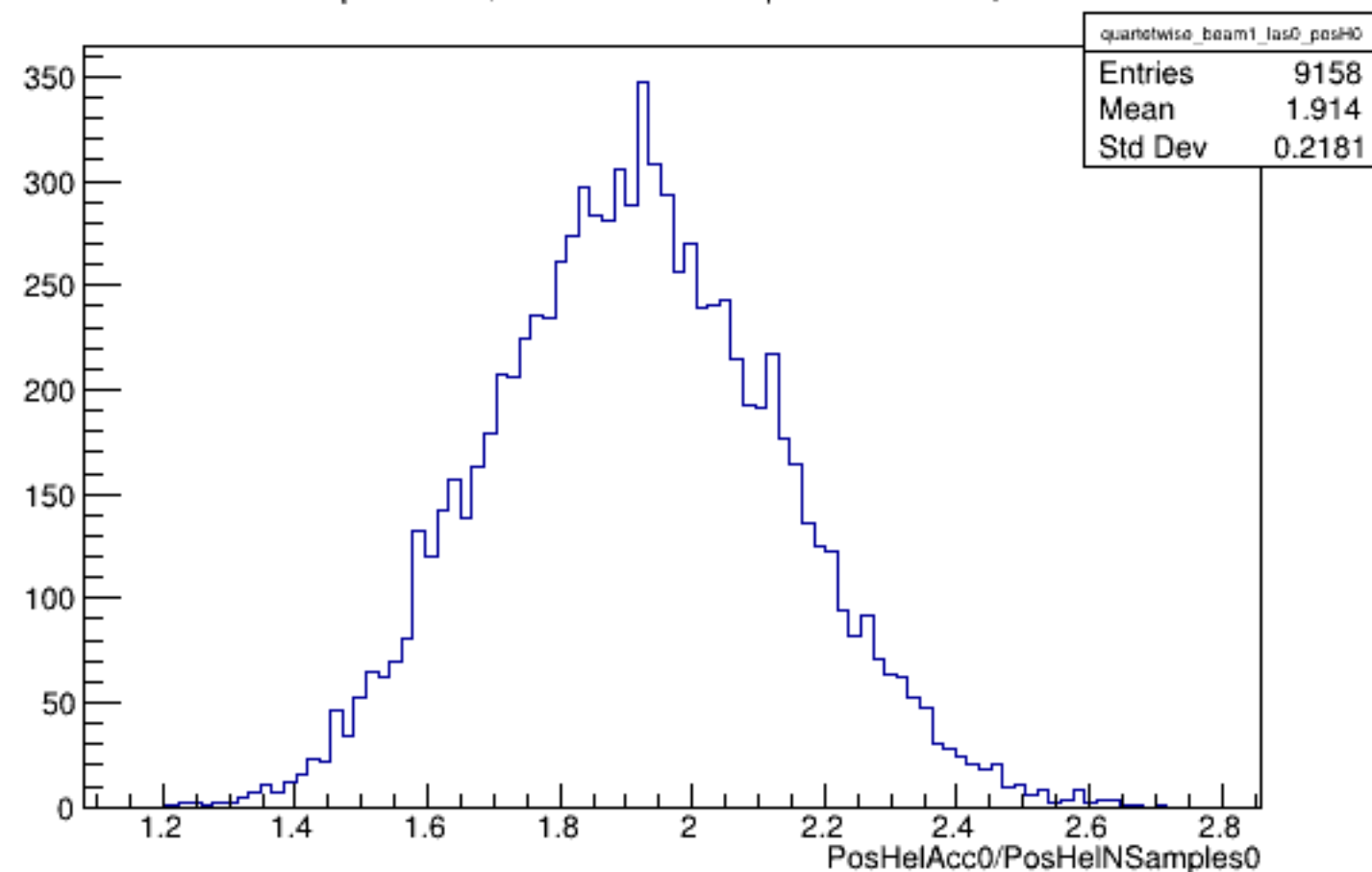
Run 5343 quartetwise, PosHelAcc0/NSamples0: Beam ON, Laser OFF
