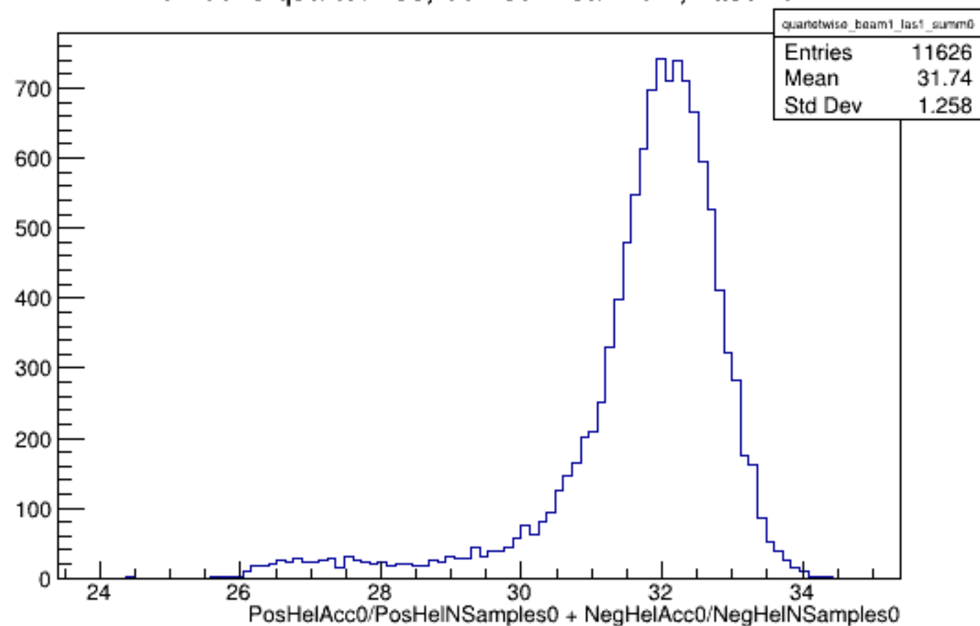
Run 5343 quartetwise, Sums0: Beam ON, Laser ON
