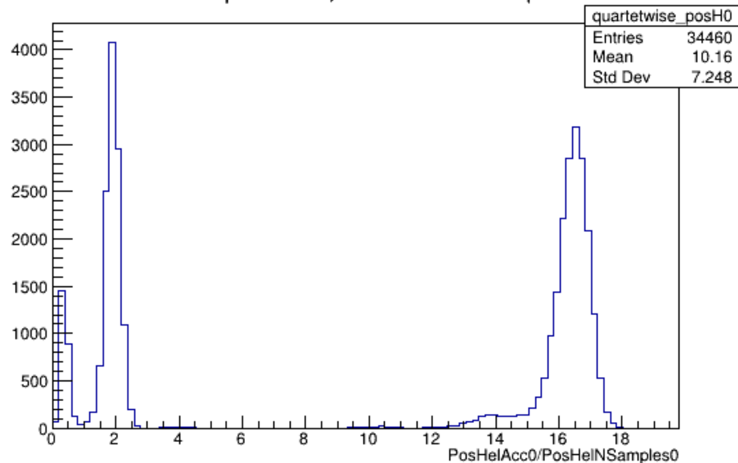
Run 5343 quartetwise, PosHelAcc0/NSamples0: All
