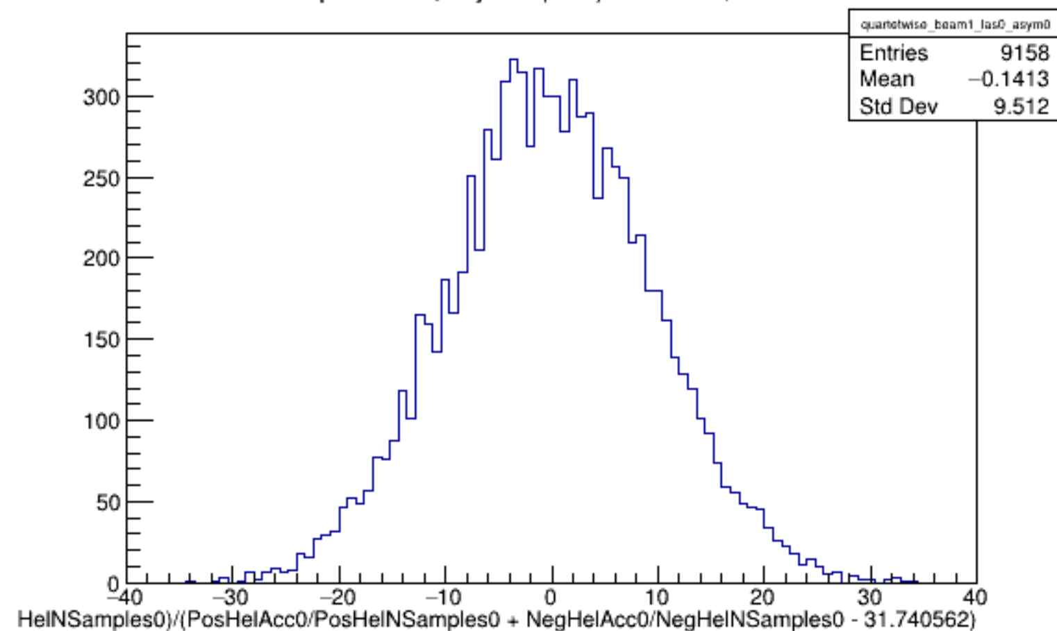
Run 5343 quartetwise, Asyms0 (Raw): Beam ON, Laser OFF
