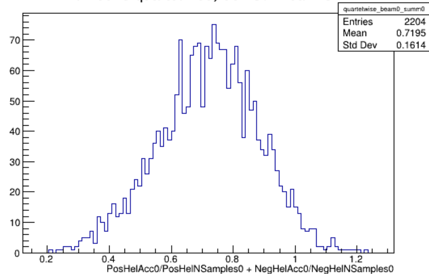
Run 5343 quartetwise, Sums0: Beam OFF
