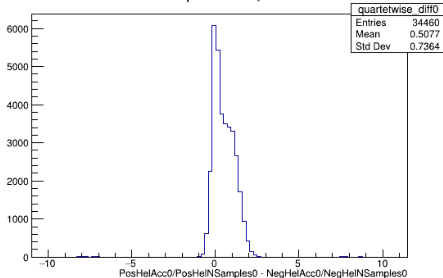
Run 5343 quartetwise, Diffs0: All
