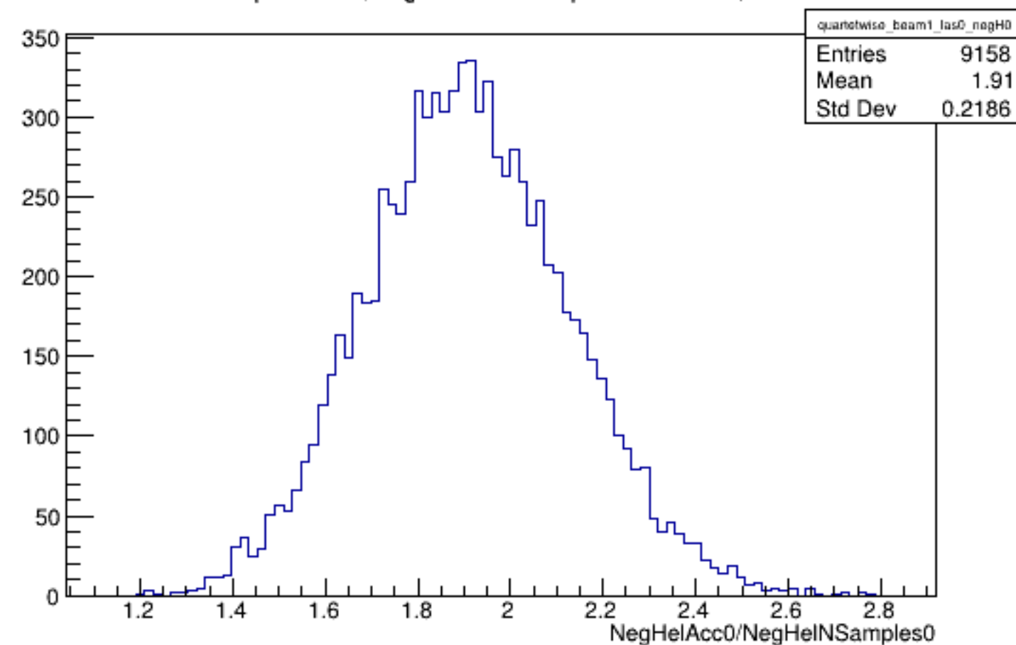
Run 5343 quartetwise, NegHelAcc0/NSamples0: Beam ON, Laser OFF
