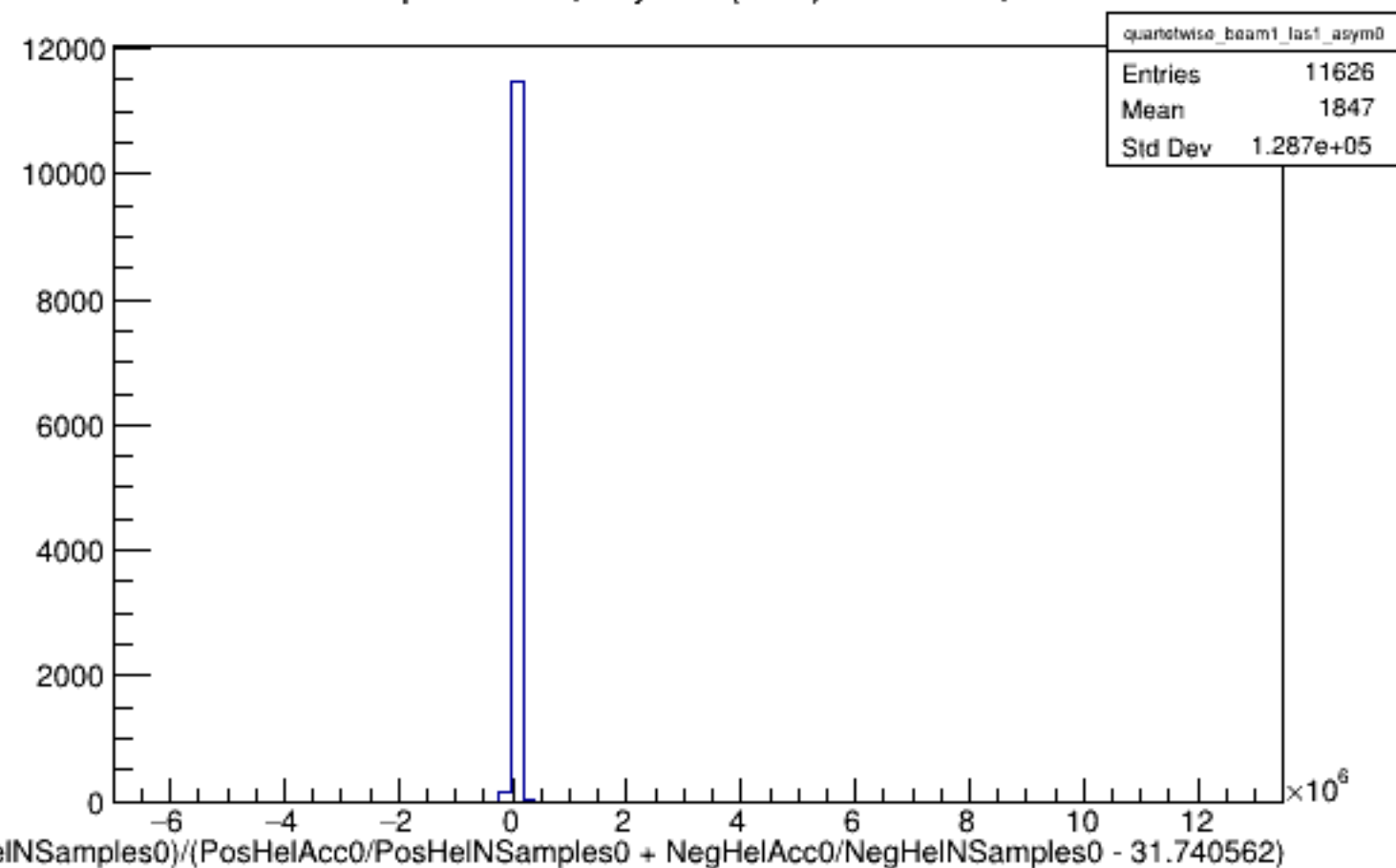
Run 5343 quartetwise, Asyms0 (Raw): Beam ON, Laser ON
