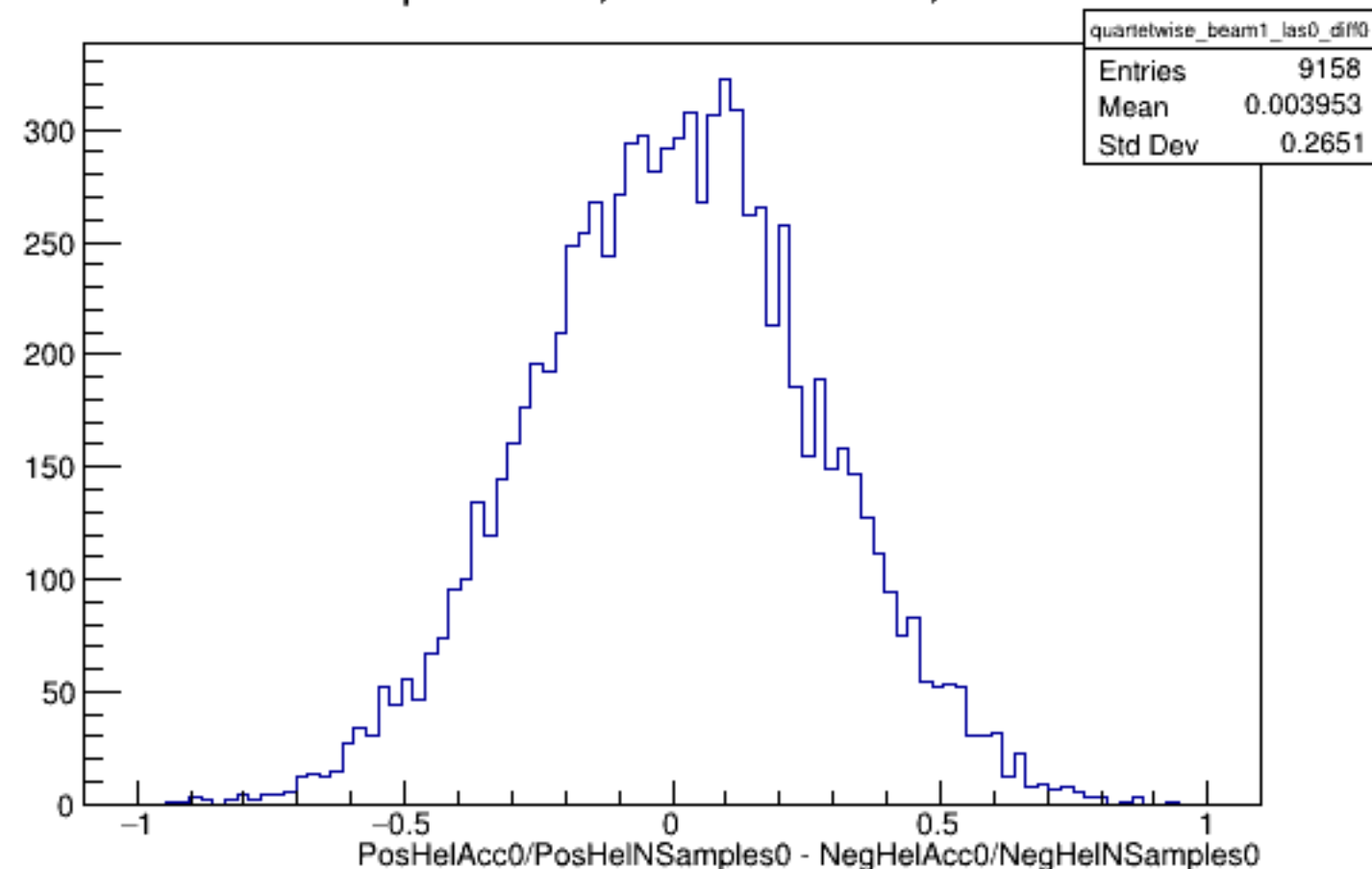
Run 5343 quartetwise, Diffs0: Beam ON, Laser OFF
