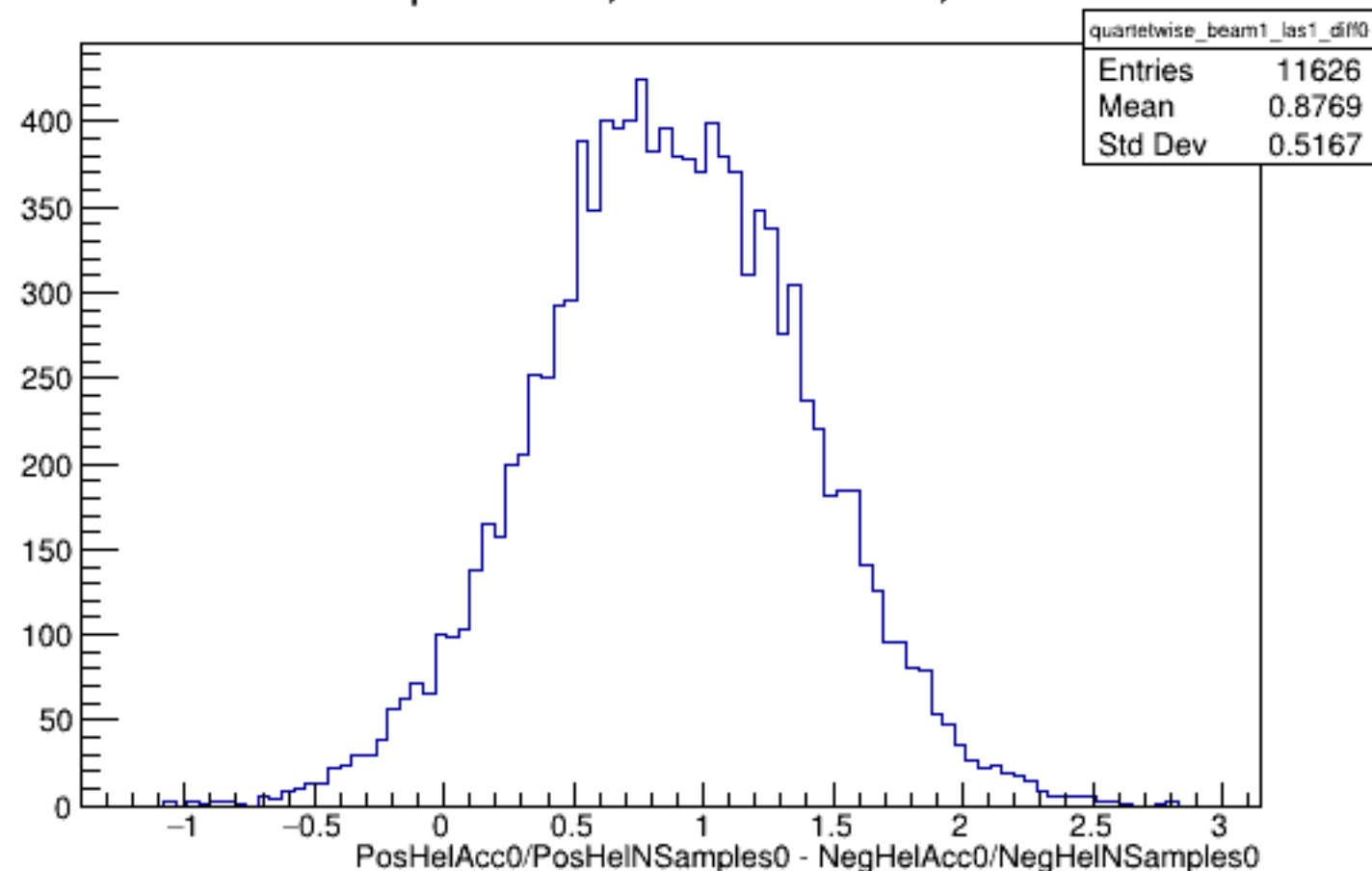
Run 5343 quartetwise, Diffs0: Beam ON, Laser ON
