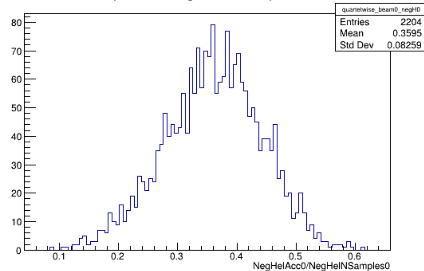
Run 5343 quartetwise, NegHelAcc0/NSamples0: Beam OFF
