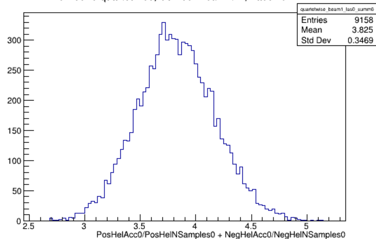
Run 5343 quartetwise, Sums0: Beam ON, Laser OFF
