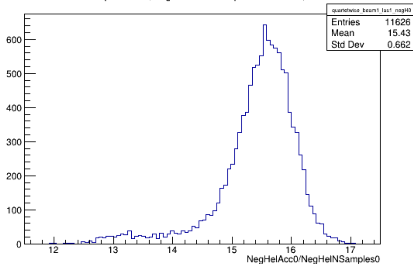
Run 5343 quartetwise, NegHelAcc0/NSamples0: Beam ON, Laser ON
