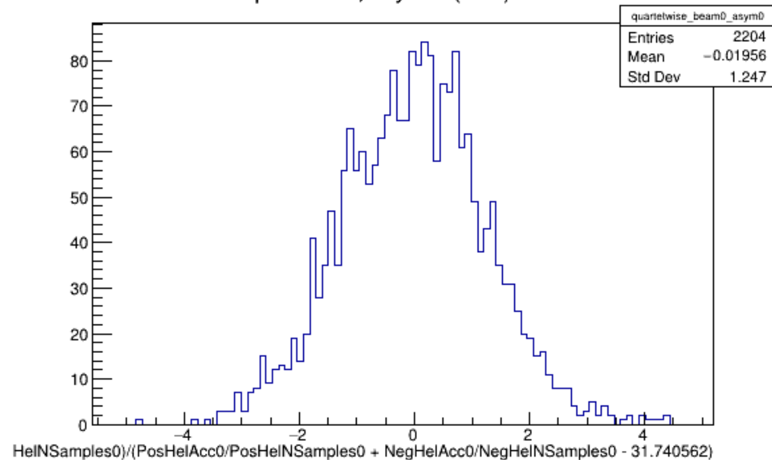
Run 5343 quartetwise, Asyms0 (Raw): Beam OFF
