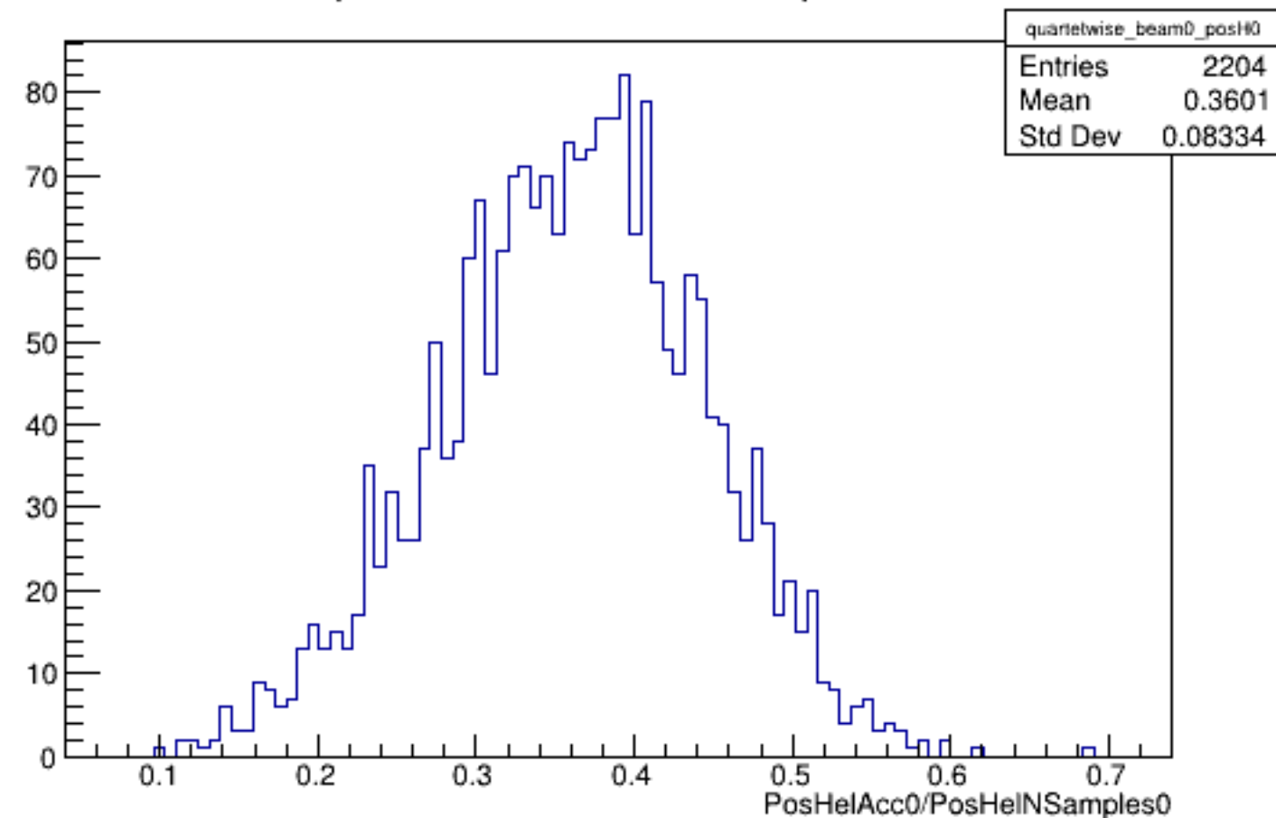
Run 5343 quartetwise, PosHelAcc0/NSamples0: Beam OFF
