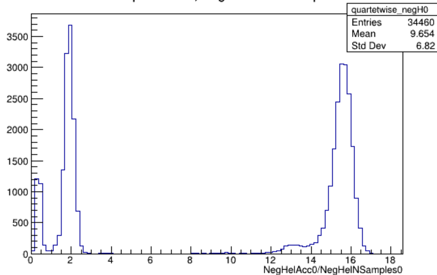
Run 5343 quartetwise, NegHelAcc0/NSamples0: All
