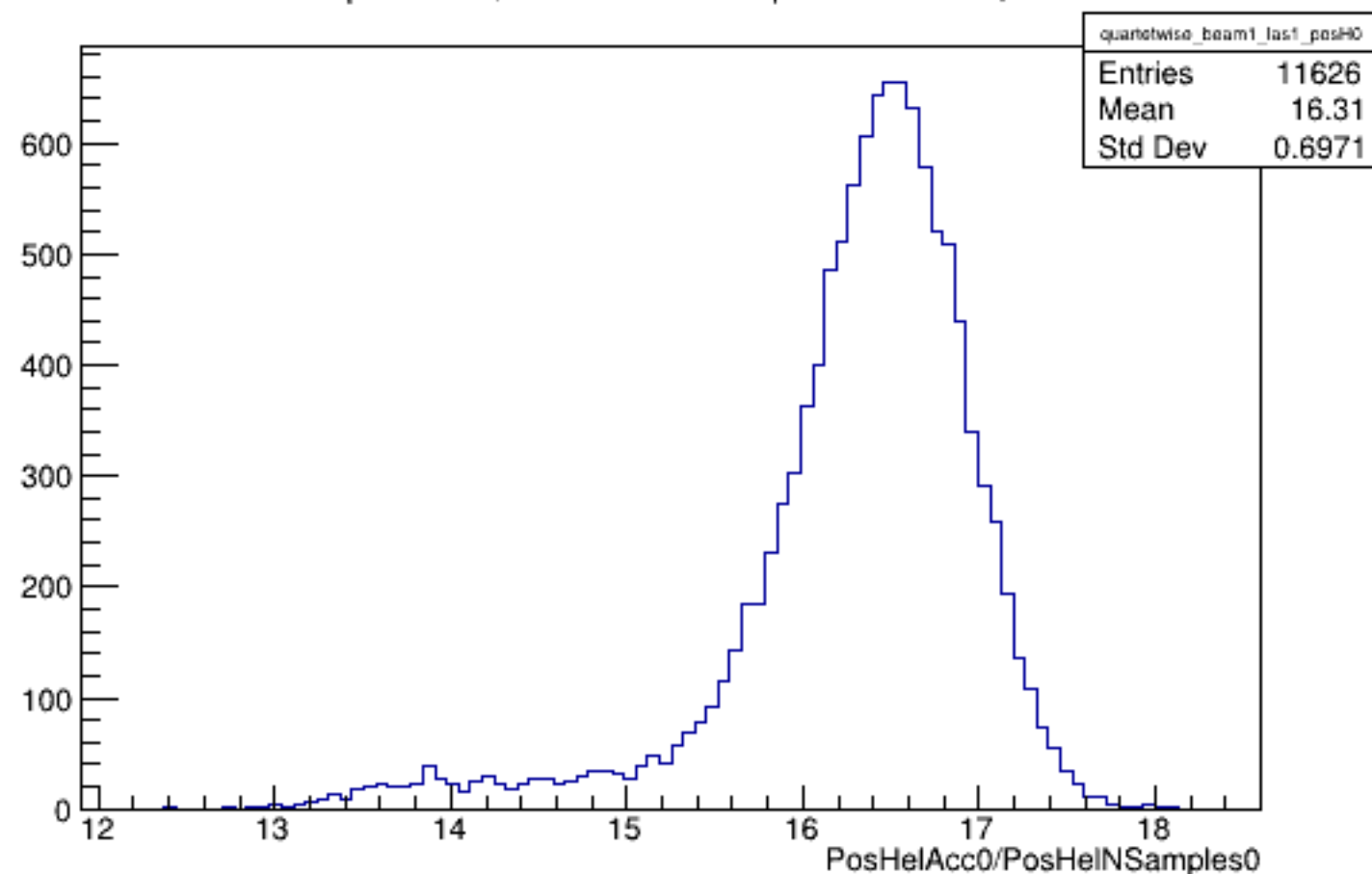
Run 5343 quartetwise, PosHelAcc0/NSamples0: Beam ON, Laser ON
