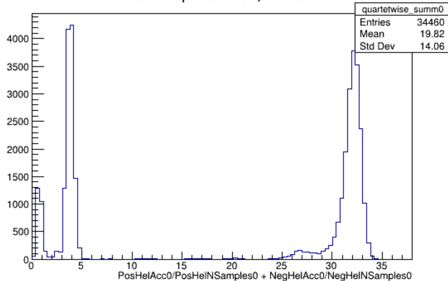
Run 5343 quartetwise, Sums0: All
