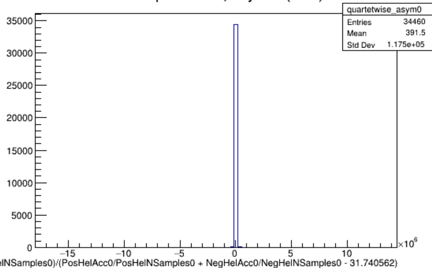
Run 5343 quartetwise, Asyms0 (Raw): All
