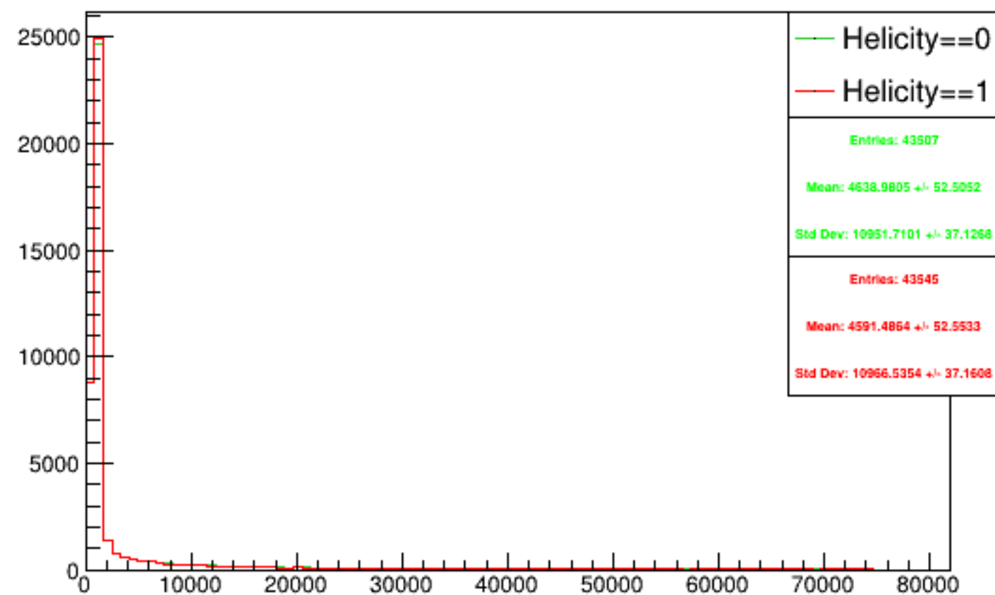
Run 5344 triggerwise, sums: Beam ON, Laser OFF
