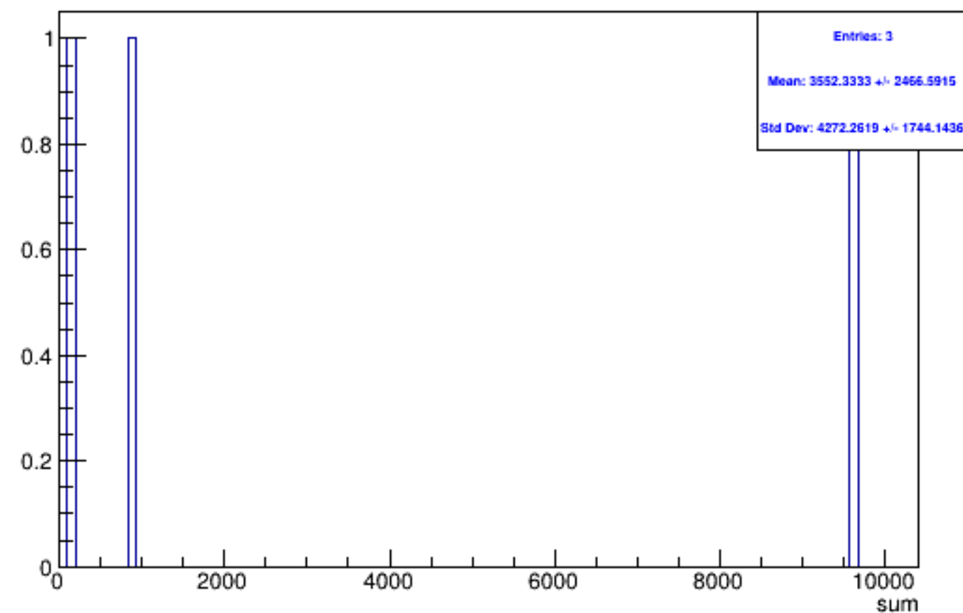
Run 5344 triggerwise, sums: Beam OFF
