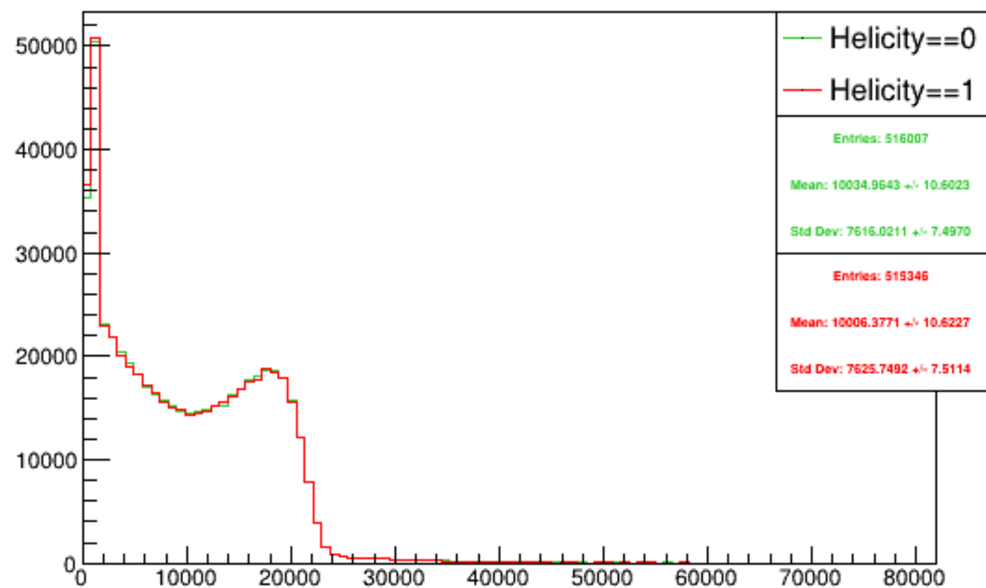
Run 5344 triggerwise, sums: Beam ON, Laser ON
