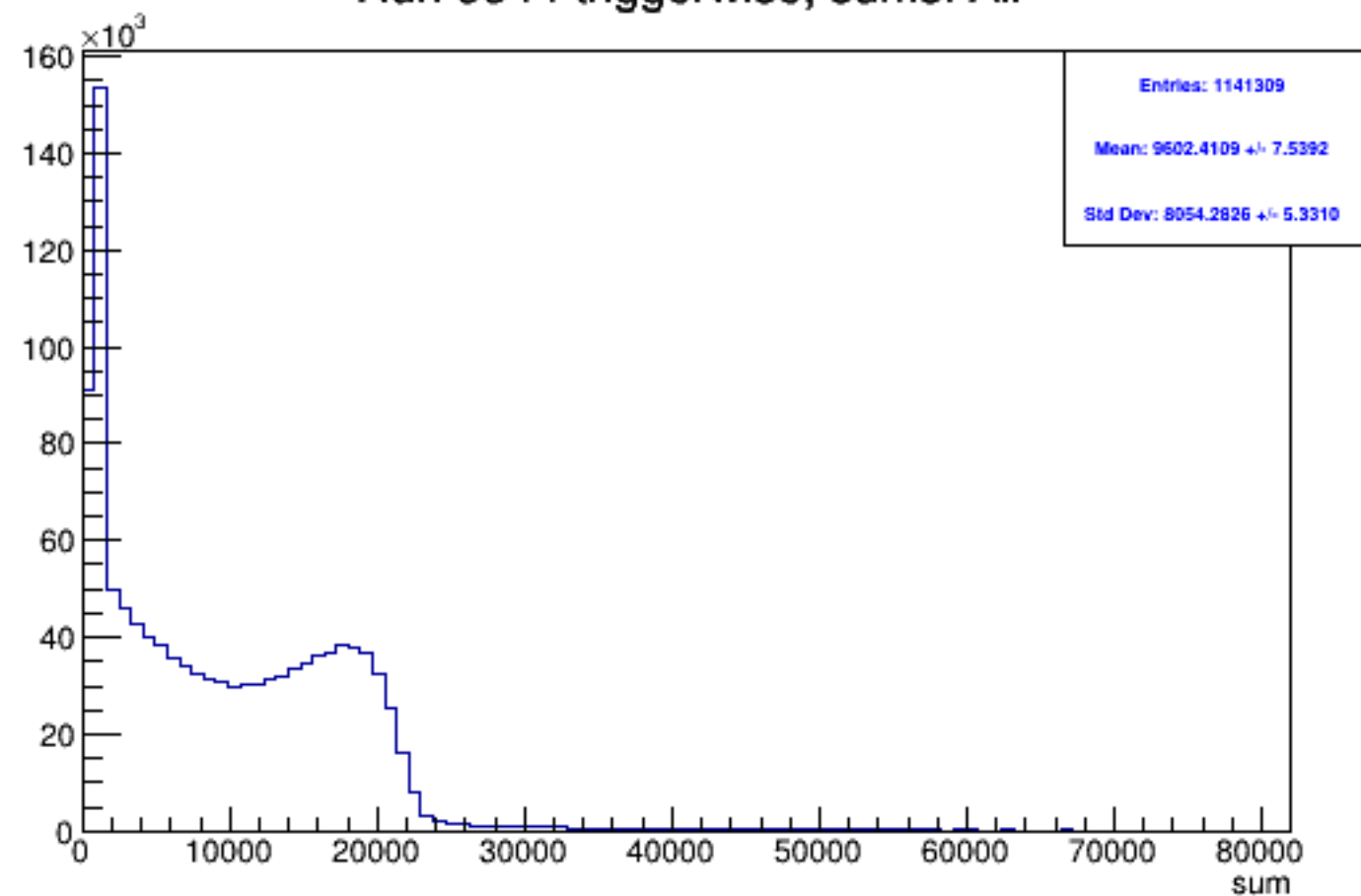
Run 5344 triggerwise, sums: All
