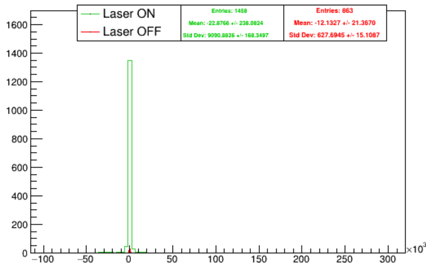
Run 5354 quartetwise, asym0sub: Beam ON
