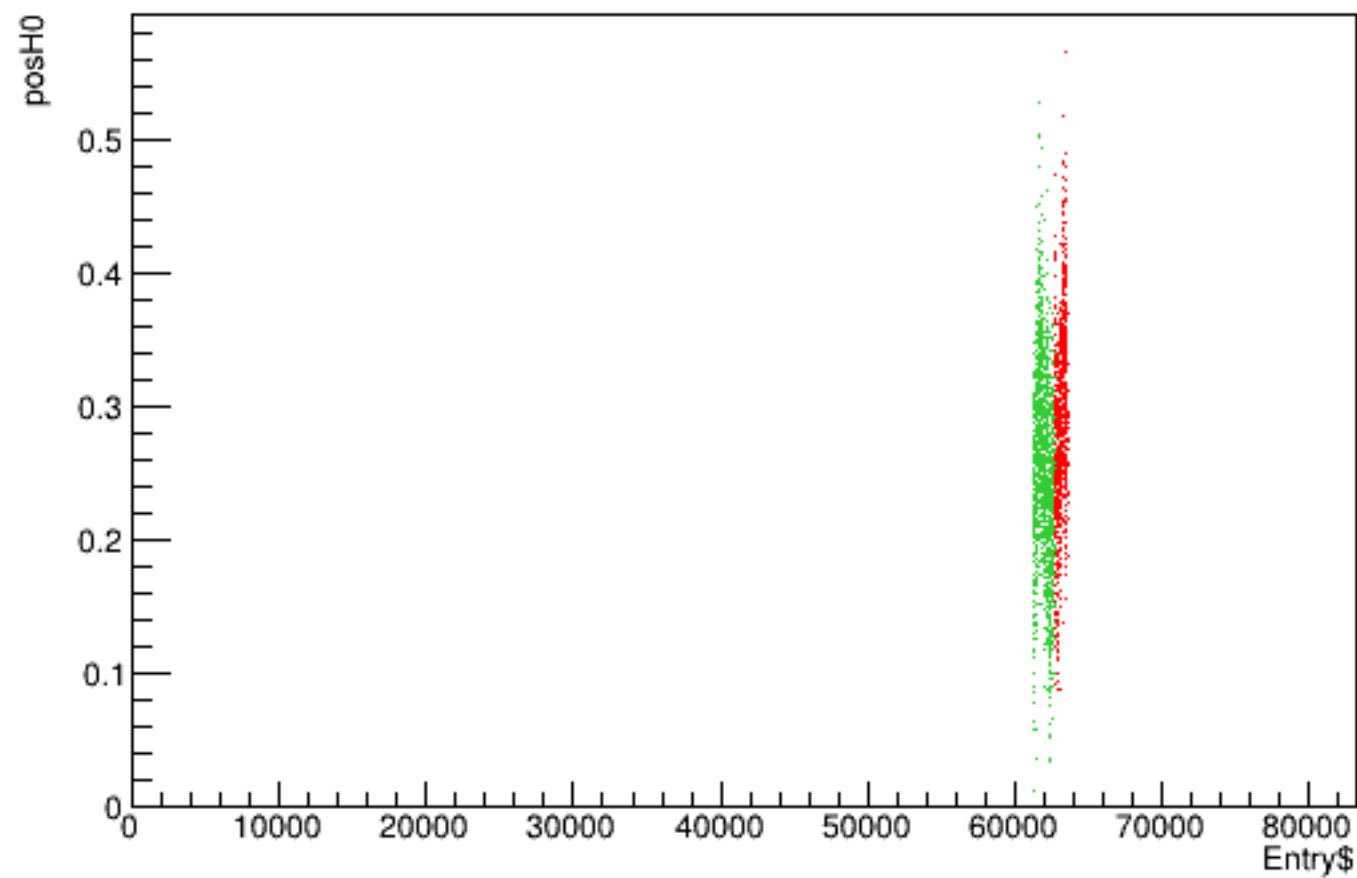
Run 5354 quartetwise, posH0 vs time
