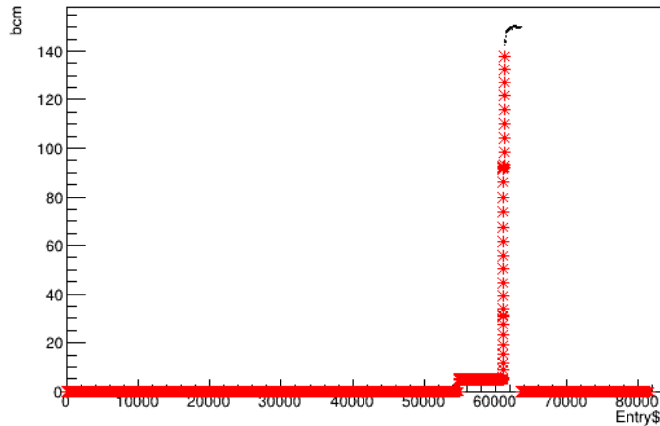
Run 5354 quartetwise, bcm vs time
