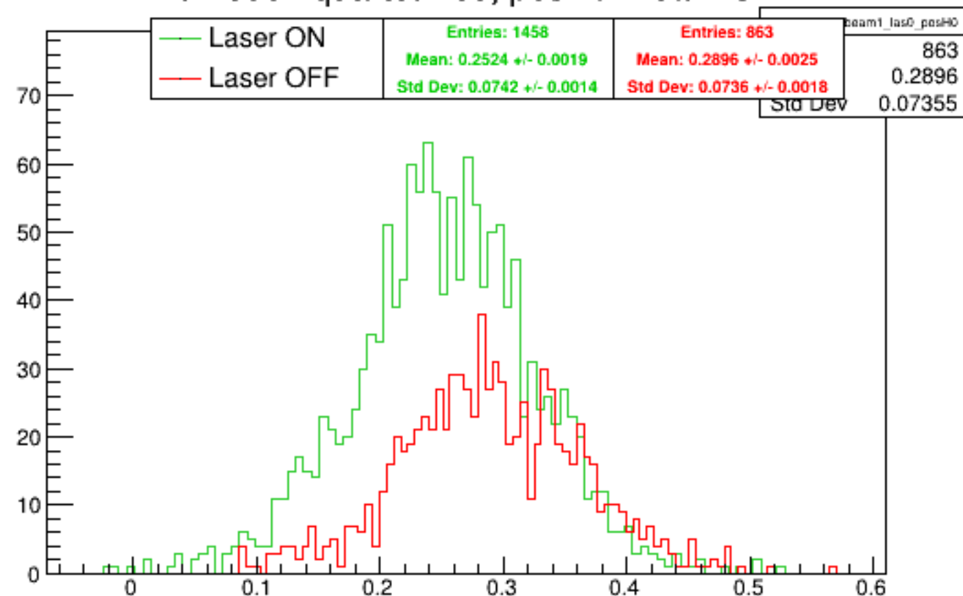
Run 5354 quartetwise, posH0: Beam ON
