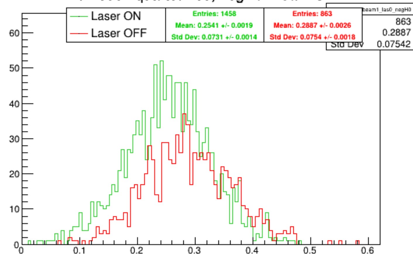
Run 5354 quartetwise, negH0: Beam ON
