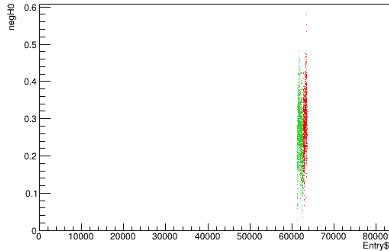
Run 5354 quartetwise, negH0 vs time
