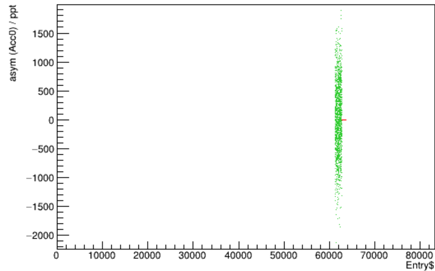
Run 5354 quartetwise, asym0sub vs time
