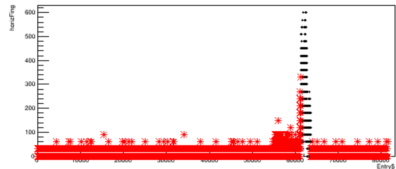
Run 5354, quartetwise: horizFing vs time
