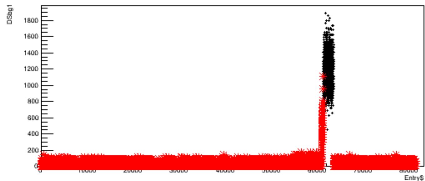
Run 5354, quartetwise: DSbg1 vs time
