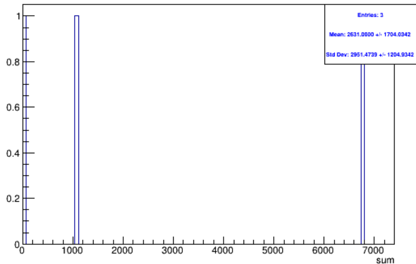
Run 5354 triggerwise, sums: All
