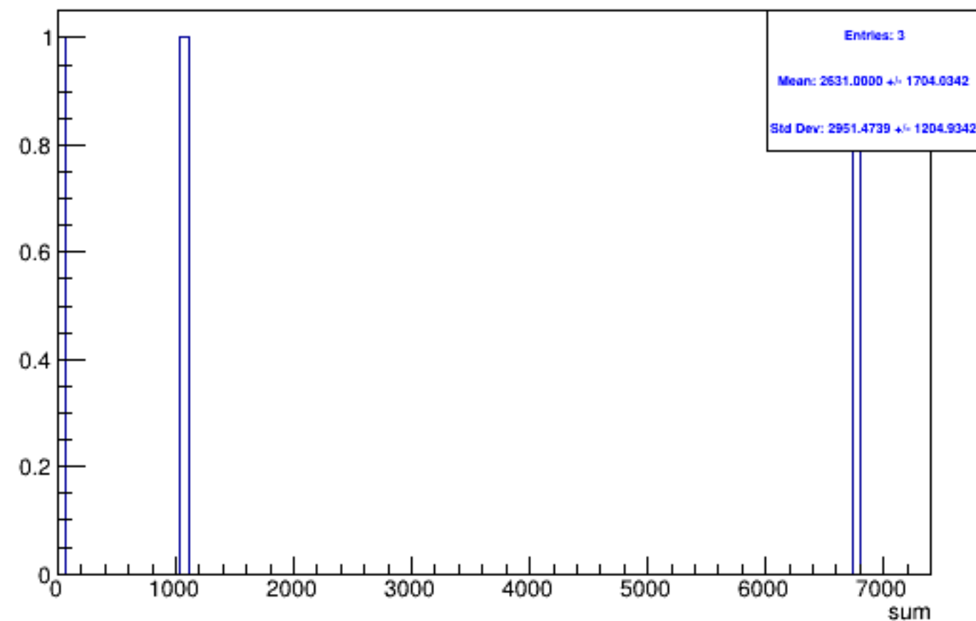
Run 5354 triggerwise, sums: Beam OFF
