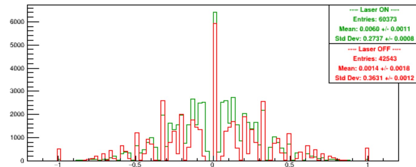
Run 5359 quartetwise, Asyms Vert Finger
