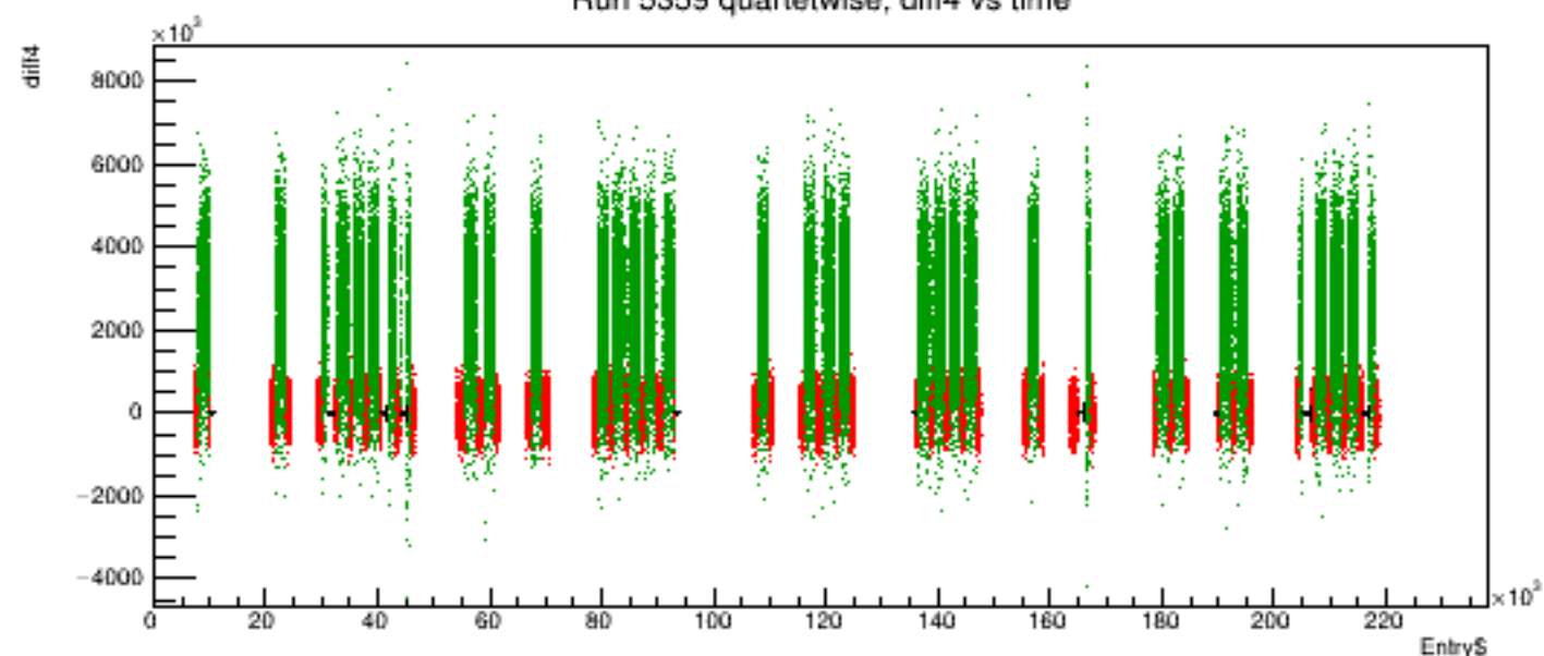
Run 5359 quartetwise, diff4 vs time
