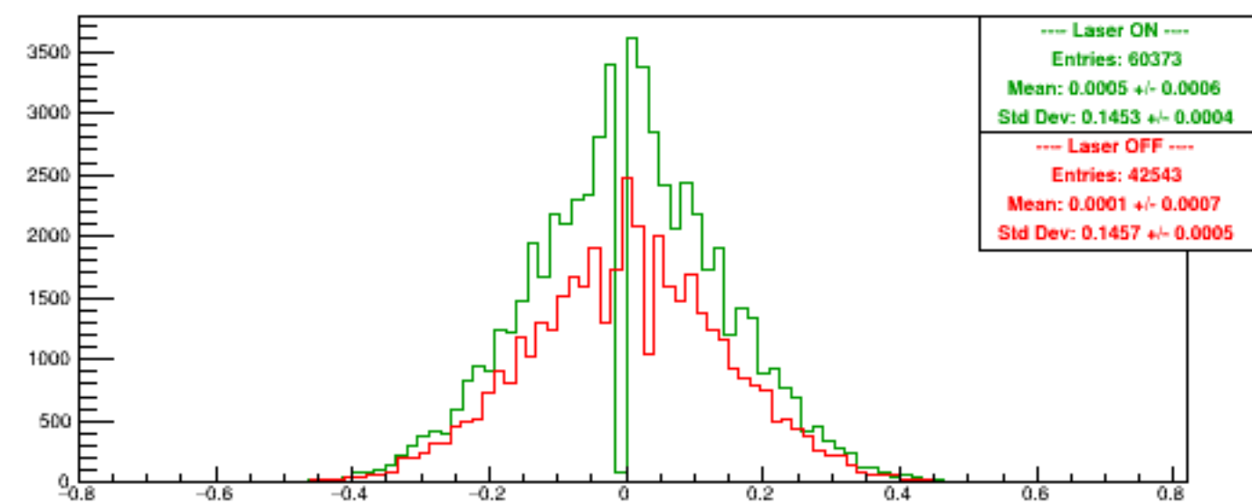
Run 5359 quartetwise, Asyms DSbg1
