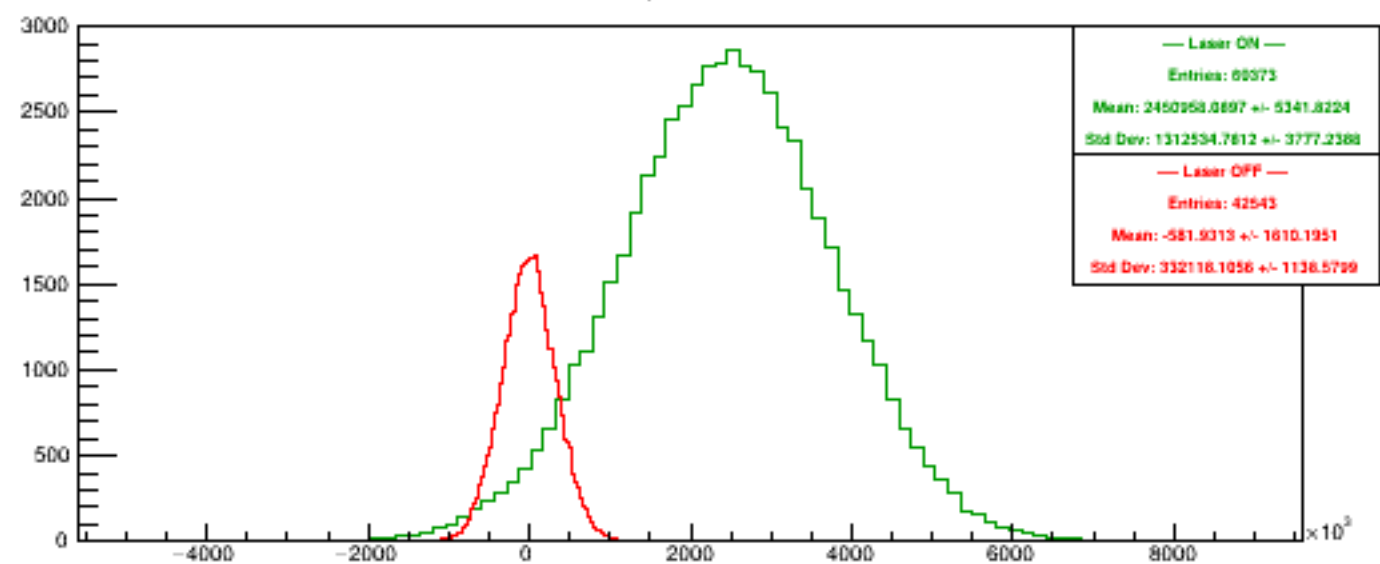
Run 5359 quartetwise, Diffs4
