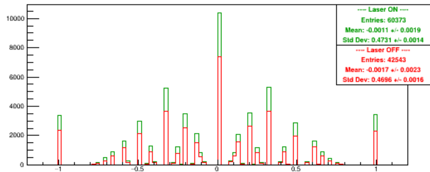
Run 5359 quartetwise, Asyms USbg1
