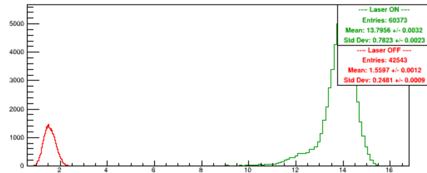
Run 5359 quartetwise, NegHelAcc0/NSamples0
