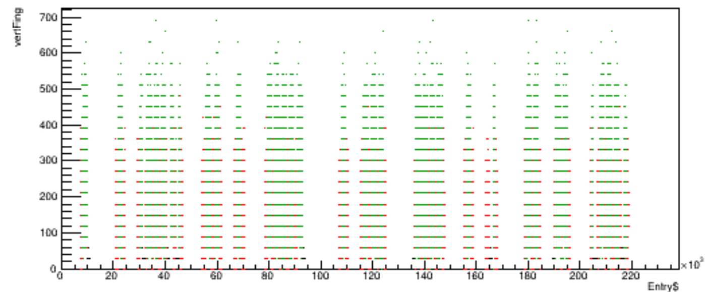
Run 5359 quartetwise, vertFing vs time
