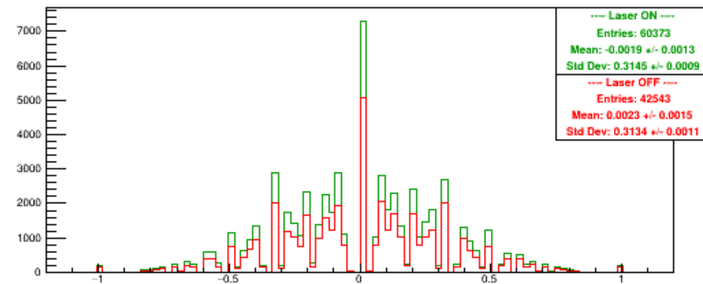
Run 5359 quartetwise, Asyms USbg2
