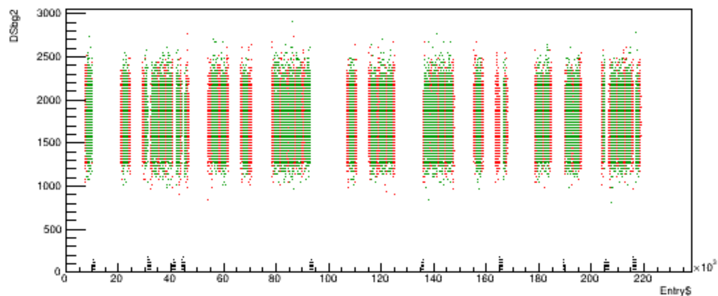
Run 5359 quartetwise, DSbg2 vs time
