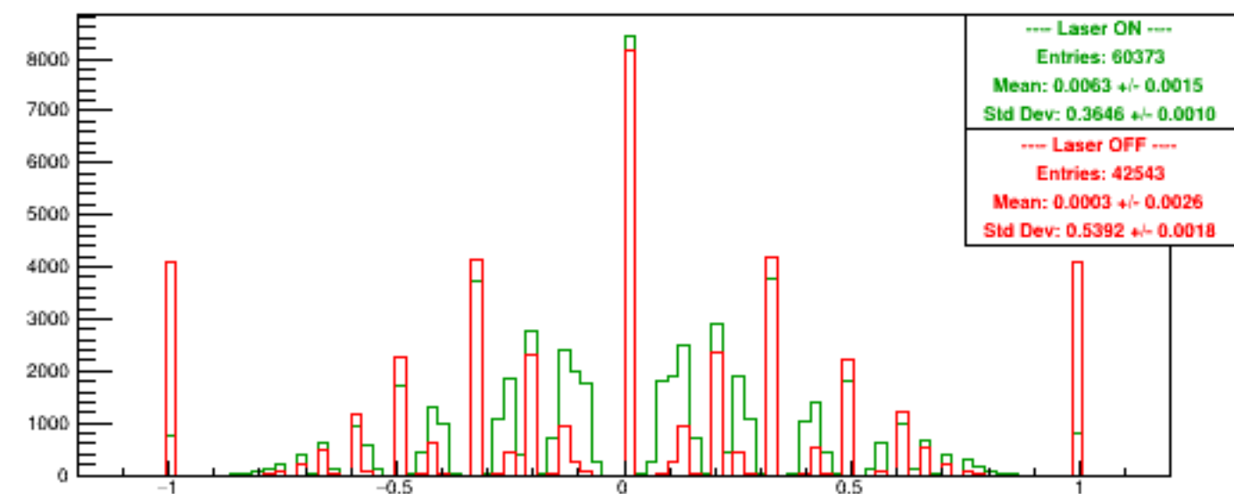
Run 5359 quartetwise, Asyms Horiz Finger
