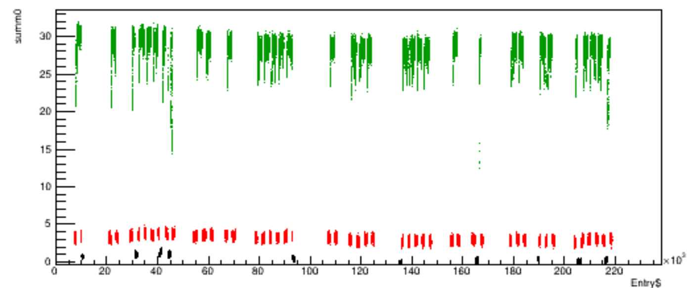
Run 5359 quartetwise, summ0 vs time
