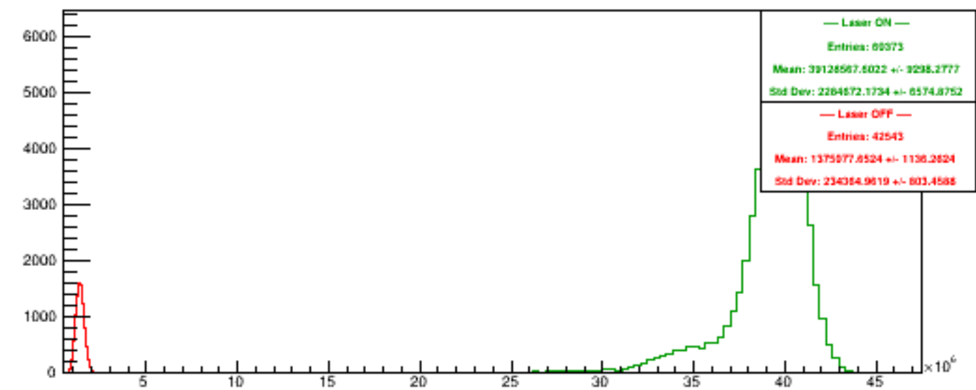
Run 5359 quartetwise, NegHelAcc4
