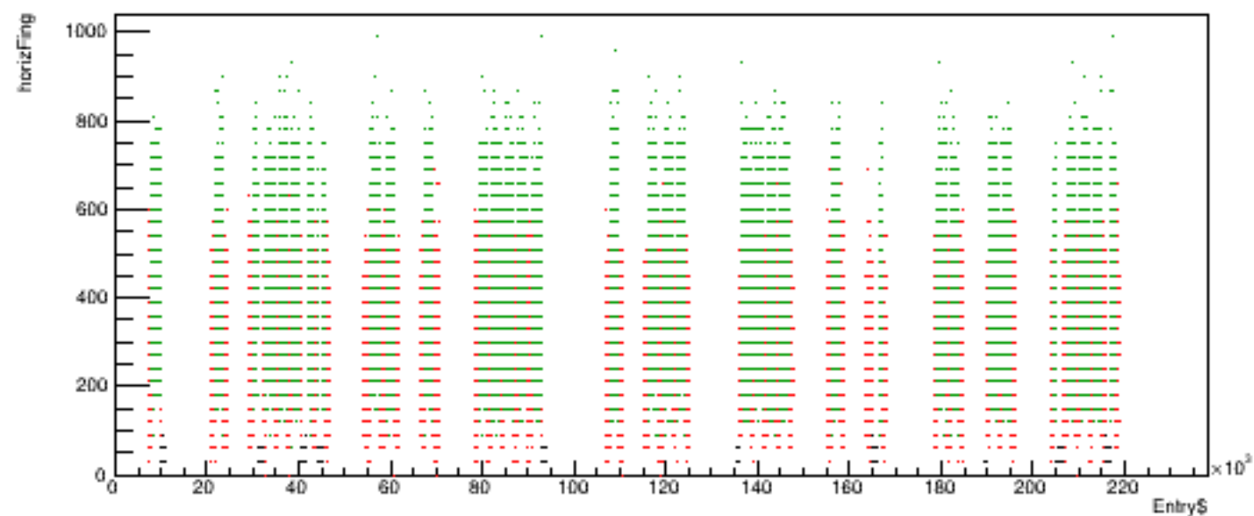
Run 5359 quartetwise, horizFing vs time
