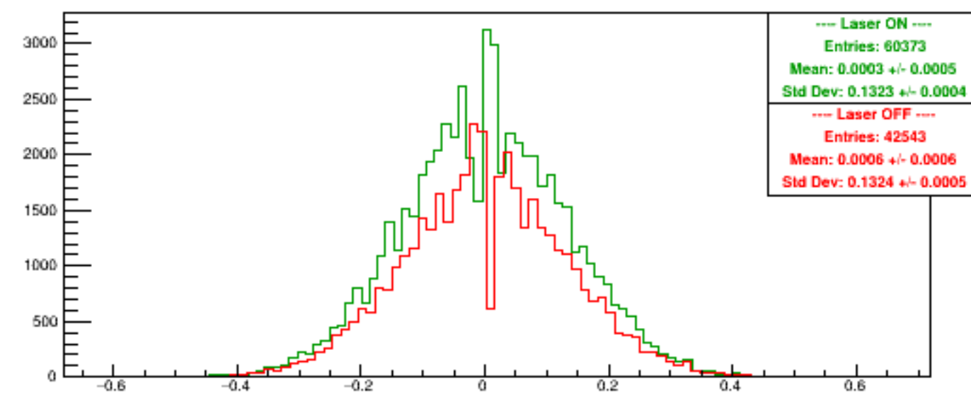
Run 5359 quartetwise, Asyms DSbg2
