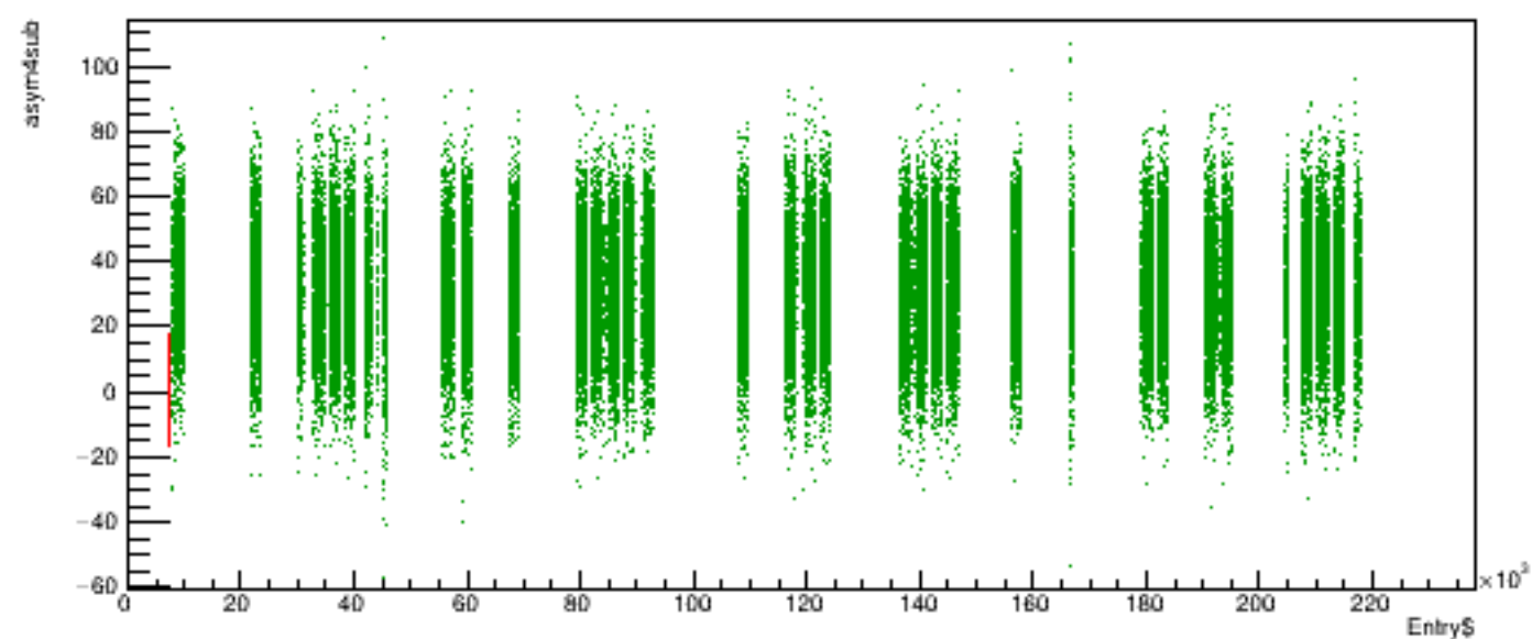
Run 5359 quartetwise, asym4sub vs time
