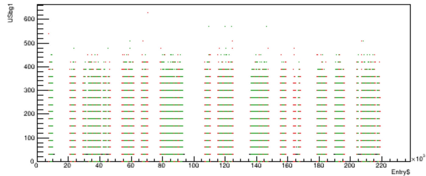
Run 5359 quartetwise, USbg1 vs time
