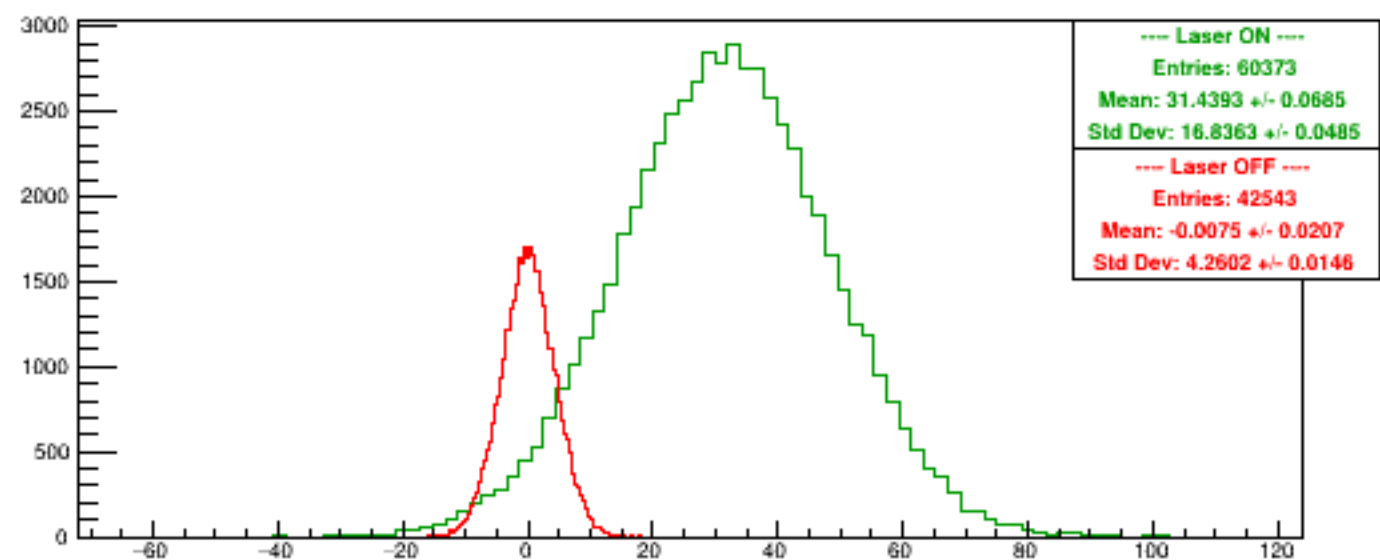
Run 5359 quartetwise, Asyms4
