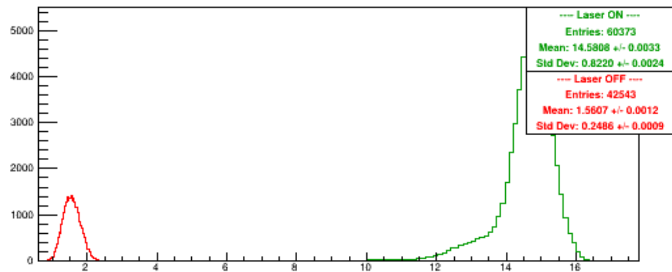
Run 5359 quartetwise, PosHelAcc0/NSamples0
