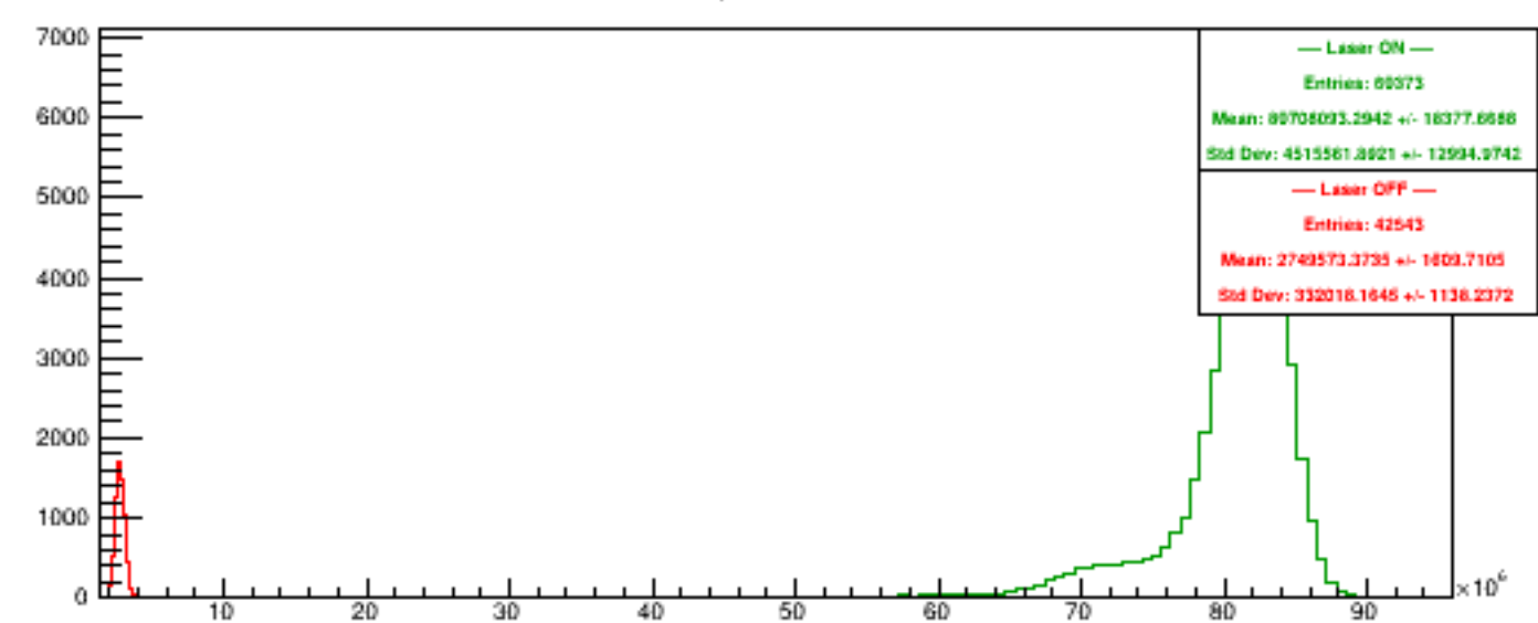
Run 5359 quartetwise, Sums4
