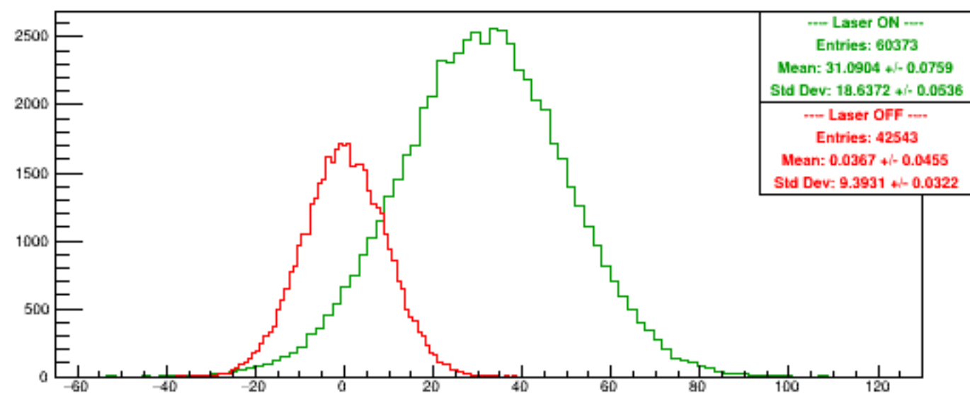
Run 5359 quartetwise, Asyms0
