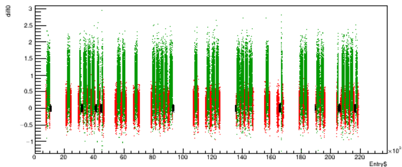
Run 5359 quartetwise, diff0 vs time
