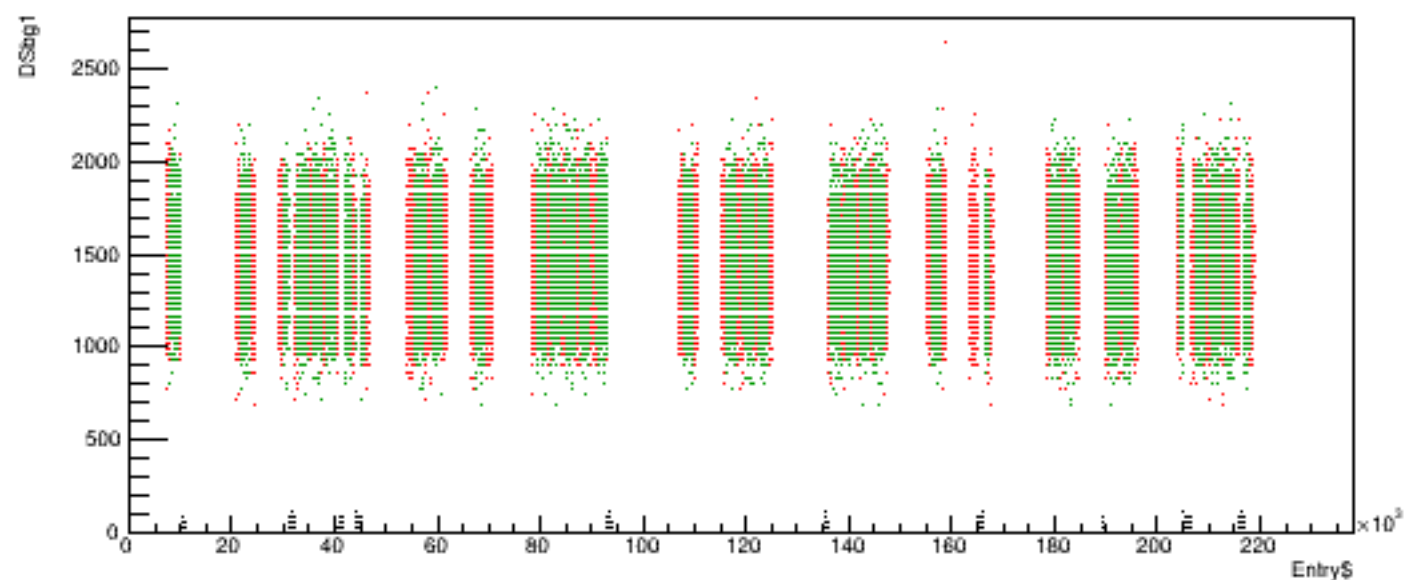
Run 5359 quartetwise, DSbg1 vs time
