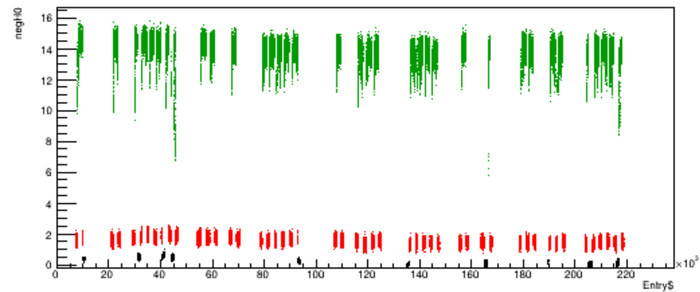
Run 5359 quartetwise, negH0 vs time
