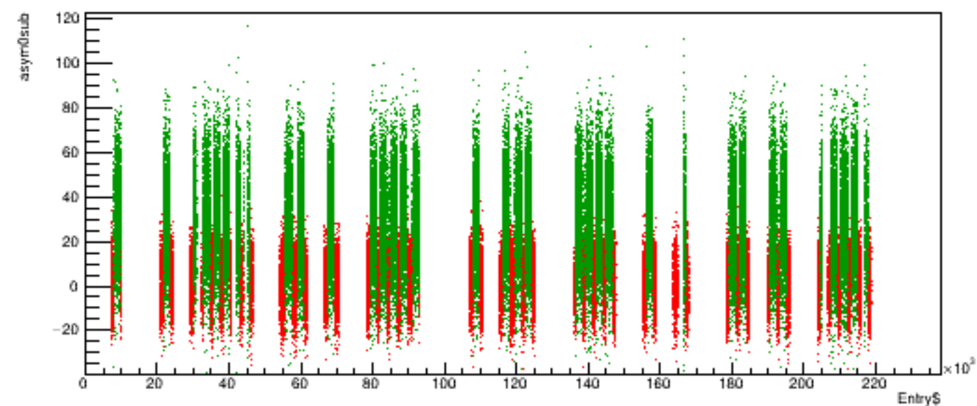
Run 5359 quartetwise, asym0sub vs time
