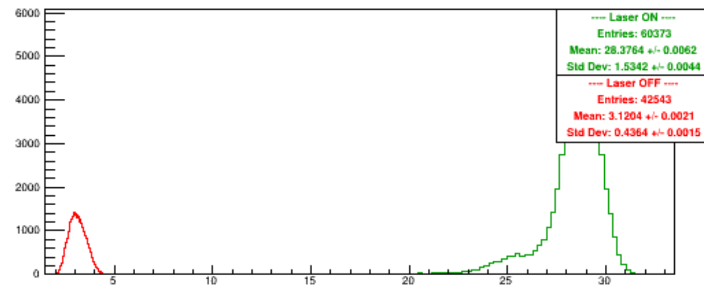
Run 5359 quartetwise, Sums0
