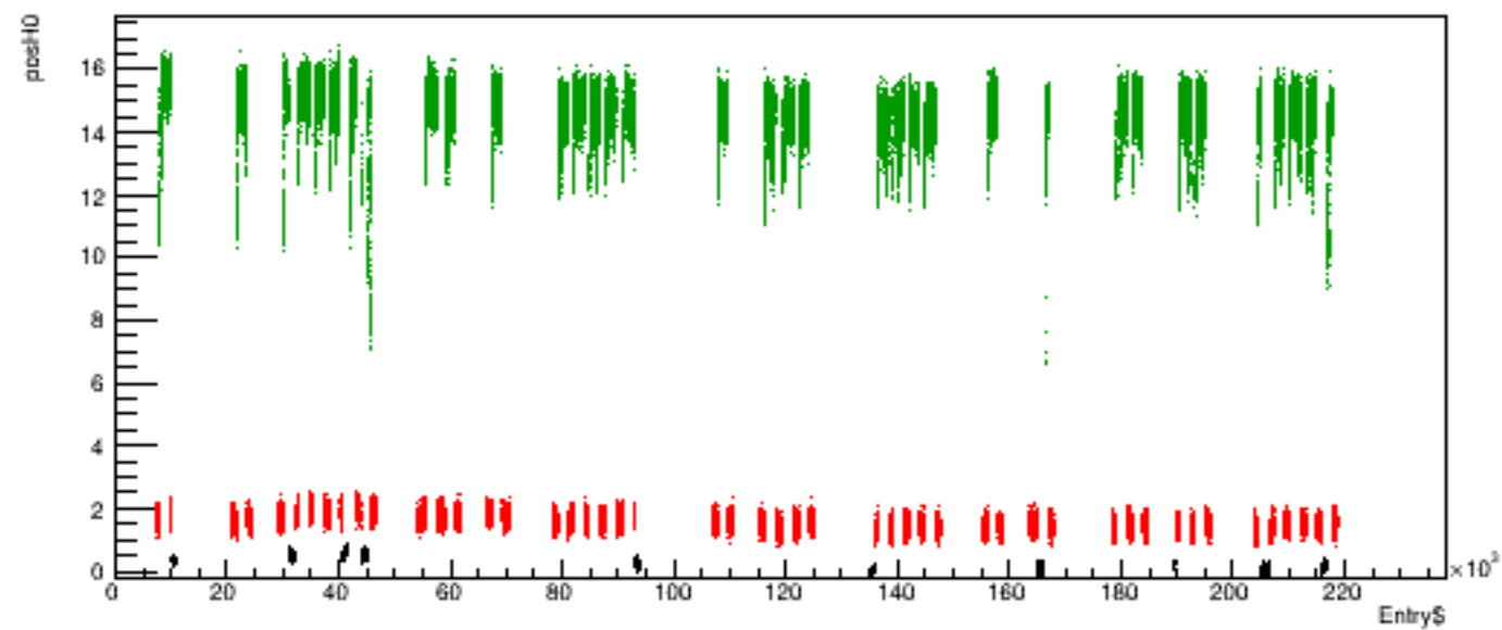
Run 5359 quartetwise, posH0 vs time
