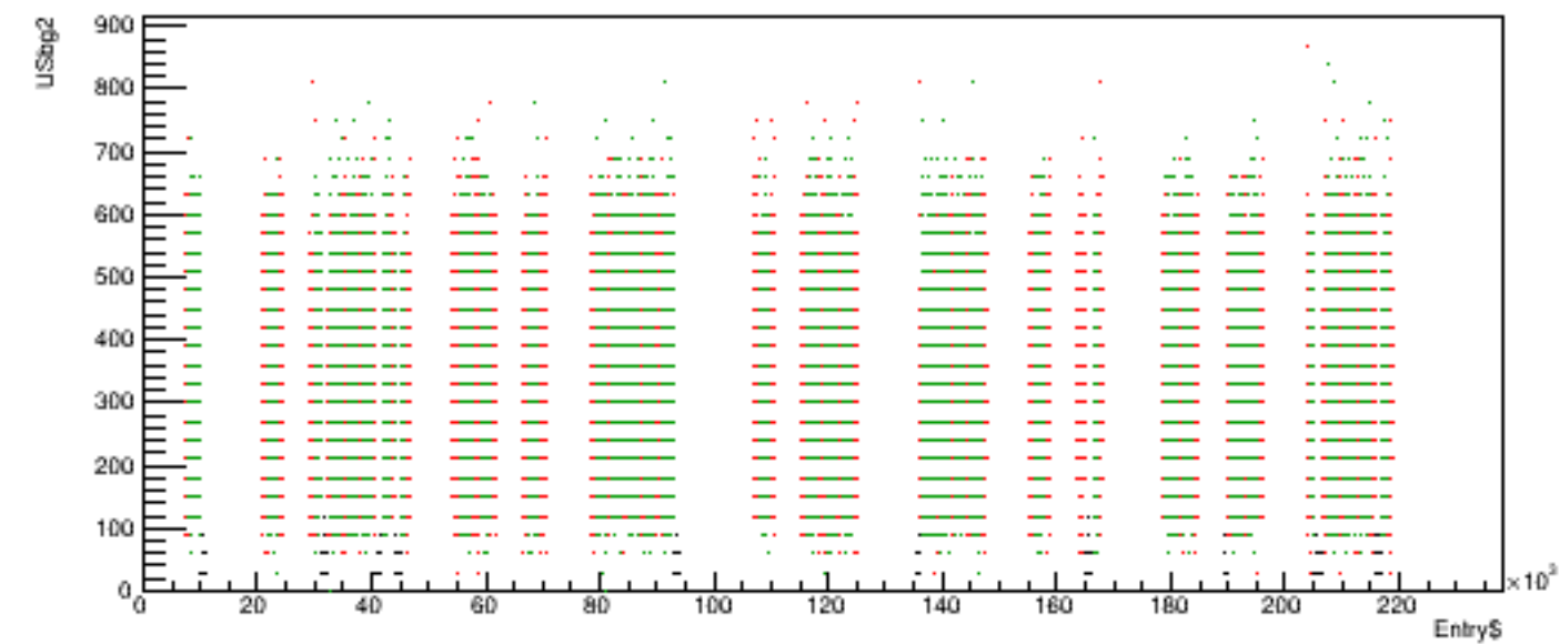
Run 5359 quartetwise, USbg2 vs time
