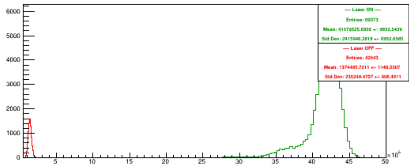
Run 5359 quartetwise, PosHelAcc4
