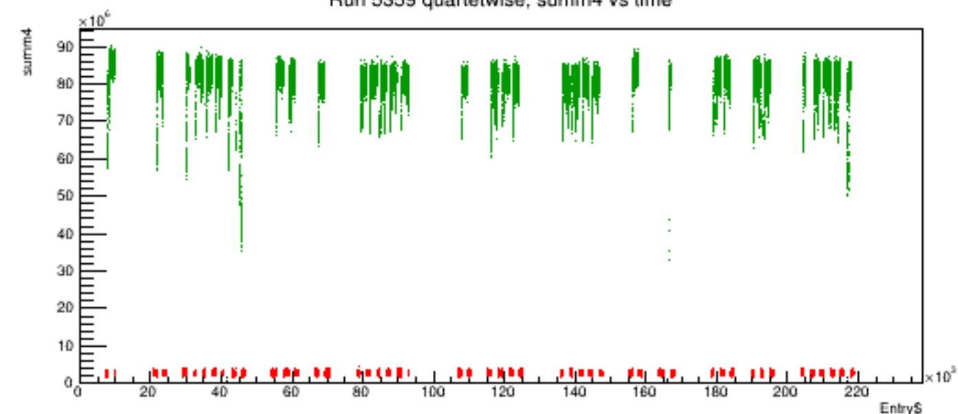
Run 5359 quartetwise, summ4 vs time
