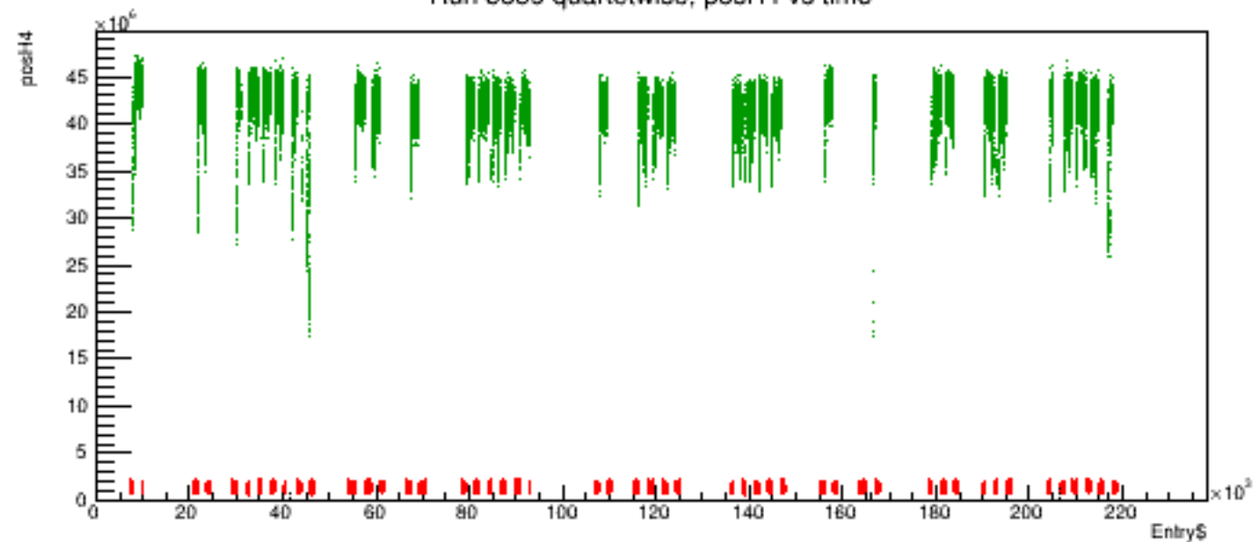
Run 5359 quartetwise, posH4 vs time
