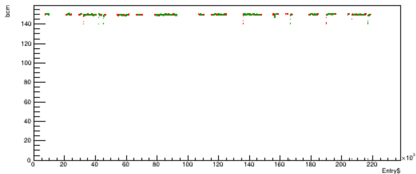
Run 5359 quartetwise, posH4 vs time
