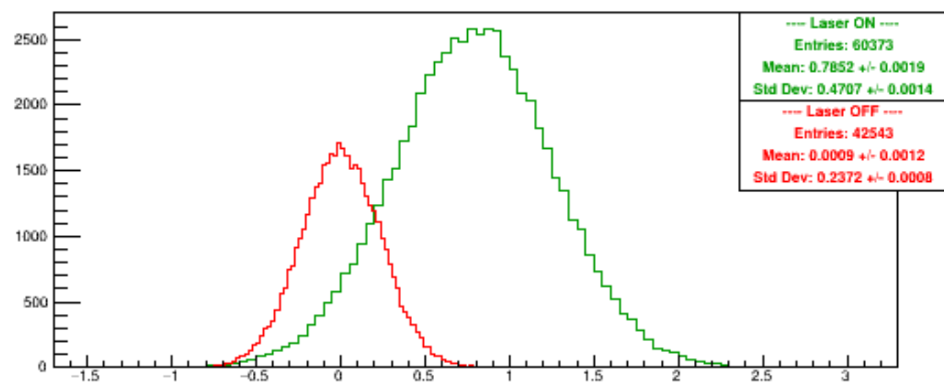
Run 5359 quartetwise, Diffs0
