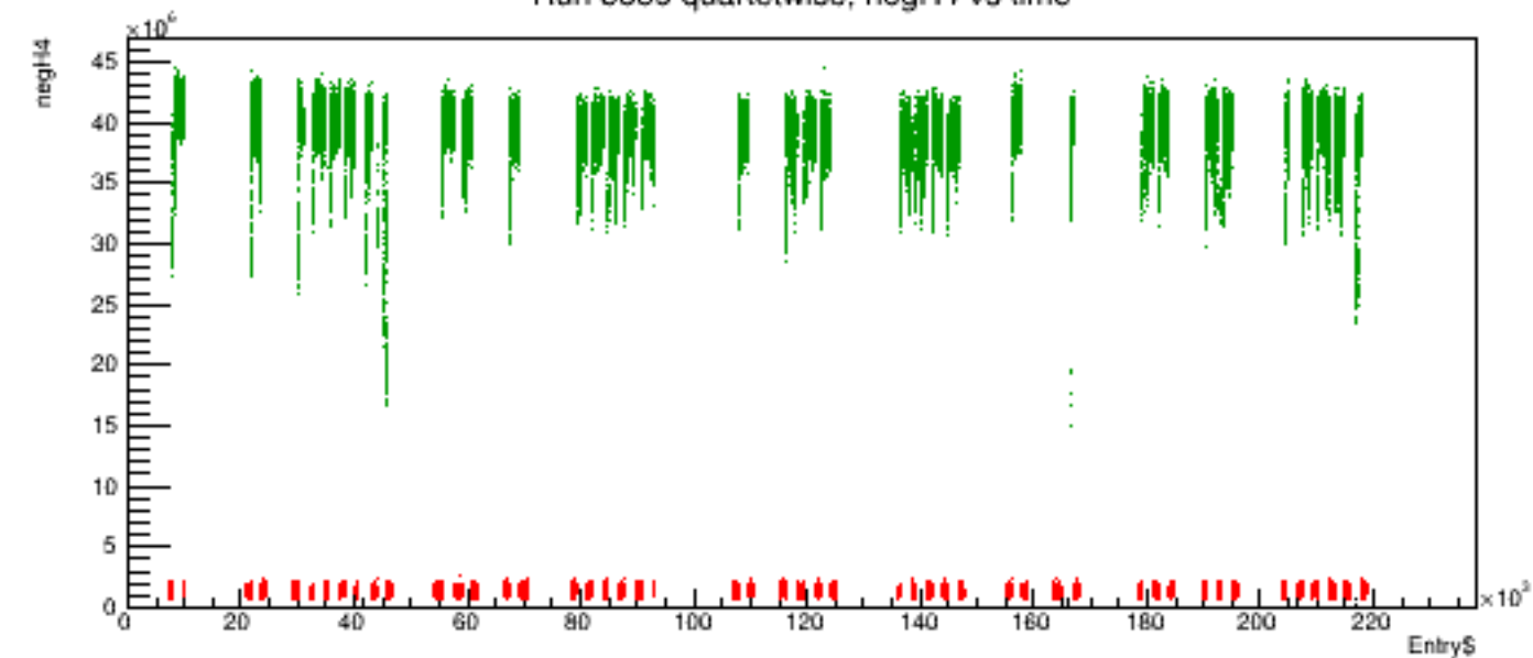
Run 5359 quartetwise, negH4 vs time
