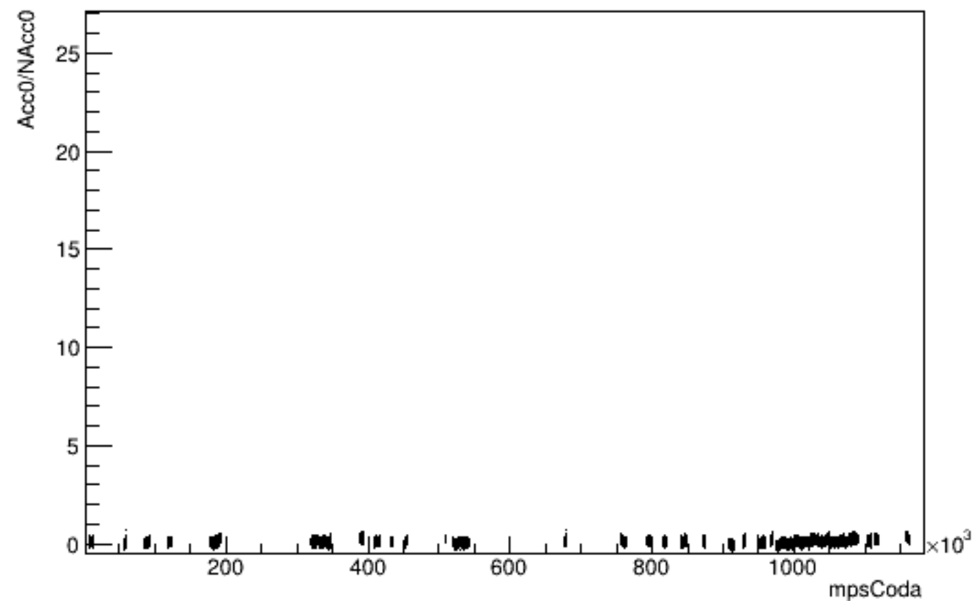
Run 5360 mpwise, Acc0 vs Time: Beam OFF
