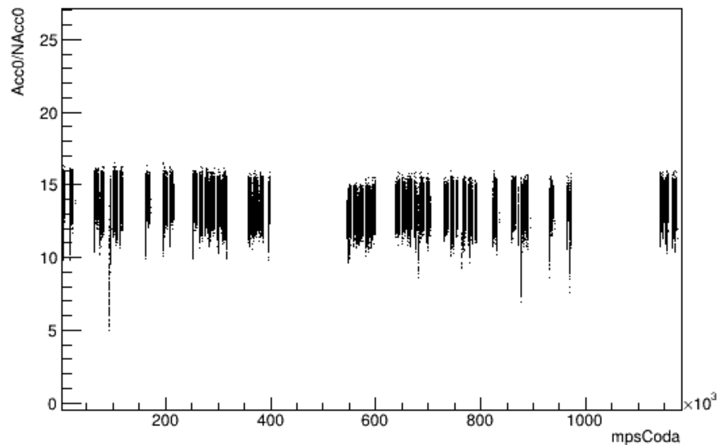
Run 5360 mpwise, Acc0 vs Time: Beam ON, Laser ON
