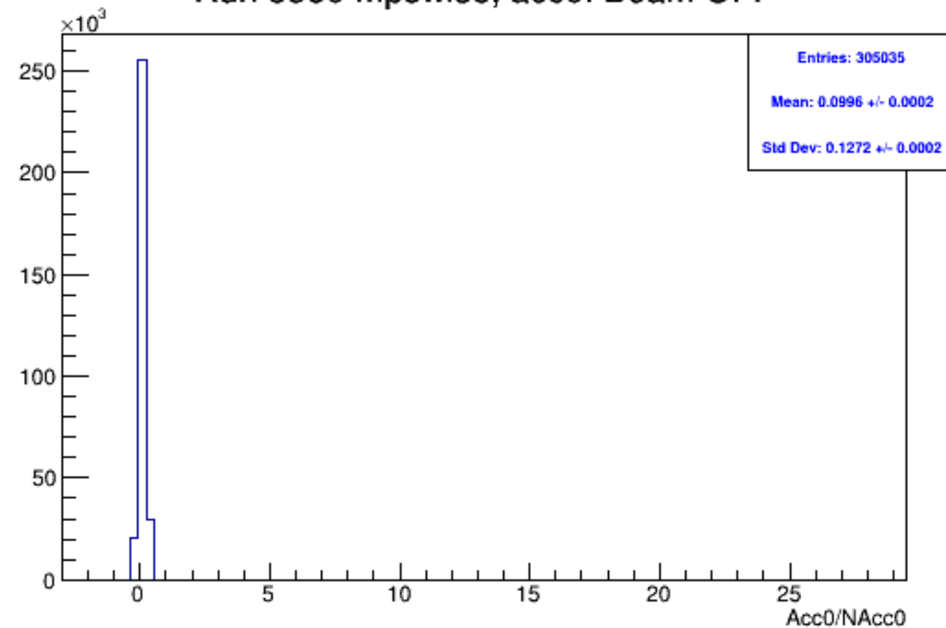
Run 5360 mpwise, acc0: Beam OFF
