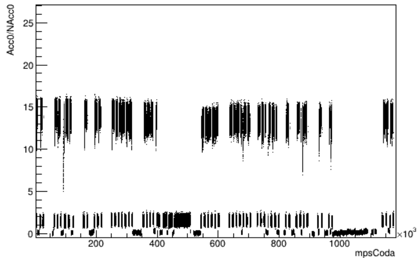
Run 5360 mpwise, Acc0 vs Time: All
