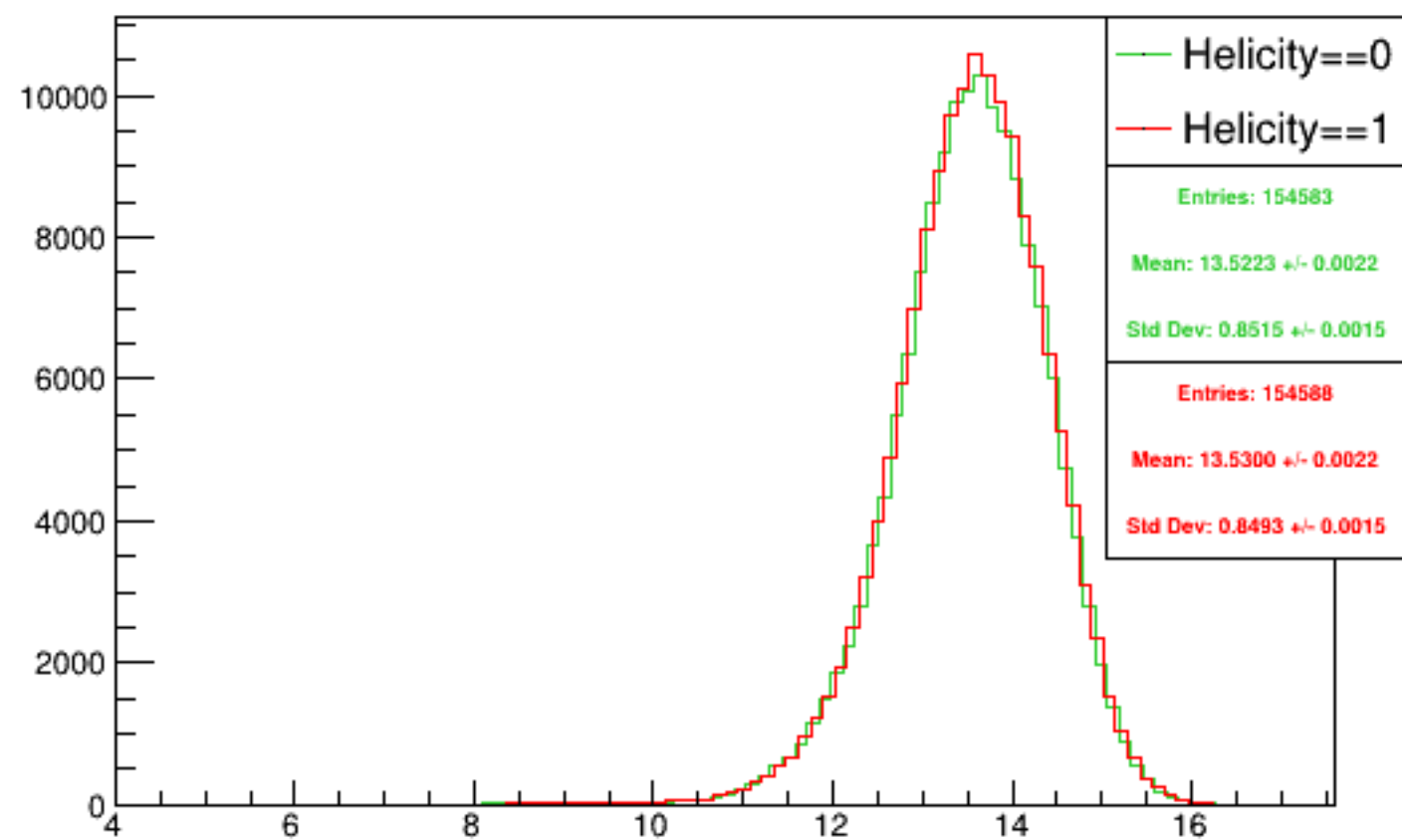
Run 5360 mpwise, acc0: Beam ON, Laser ON
