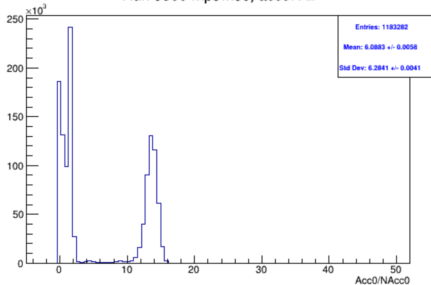
Run 5360 mpwise, acc0: All
