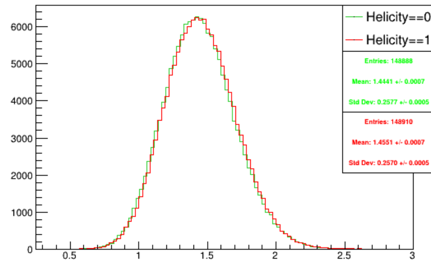
Run 5360 mpwise, acc0: Beam ON, Laser OFF
