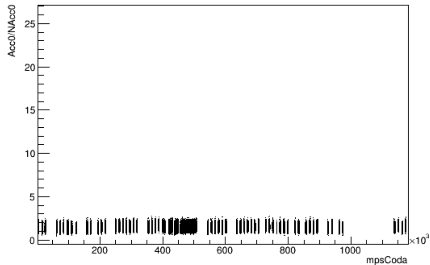
Run 5360 mpwise, Acc0 vs Time: Beam ON, Laser OFF
