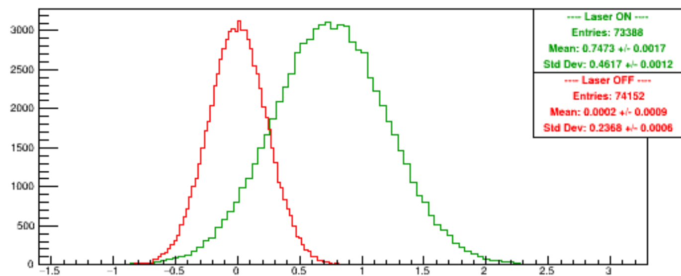
Run 5360 quartetwise, Diffs0
