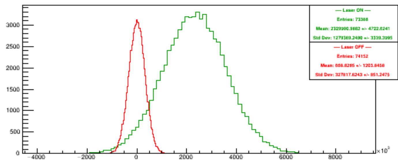
Run 5360 quartetwise, Diffs4
