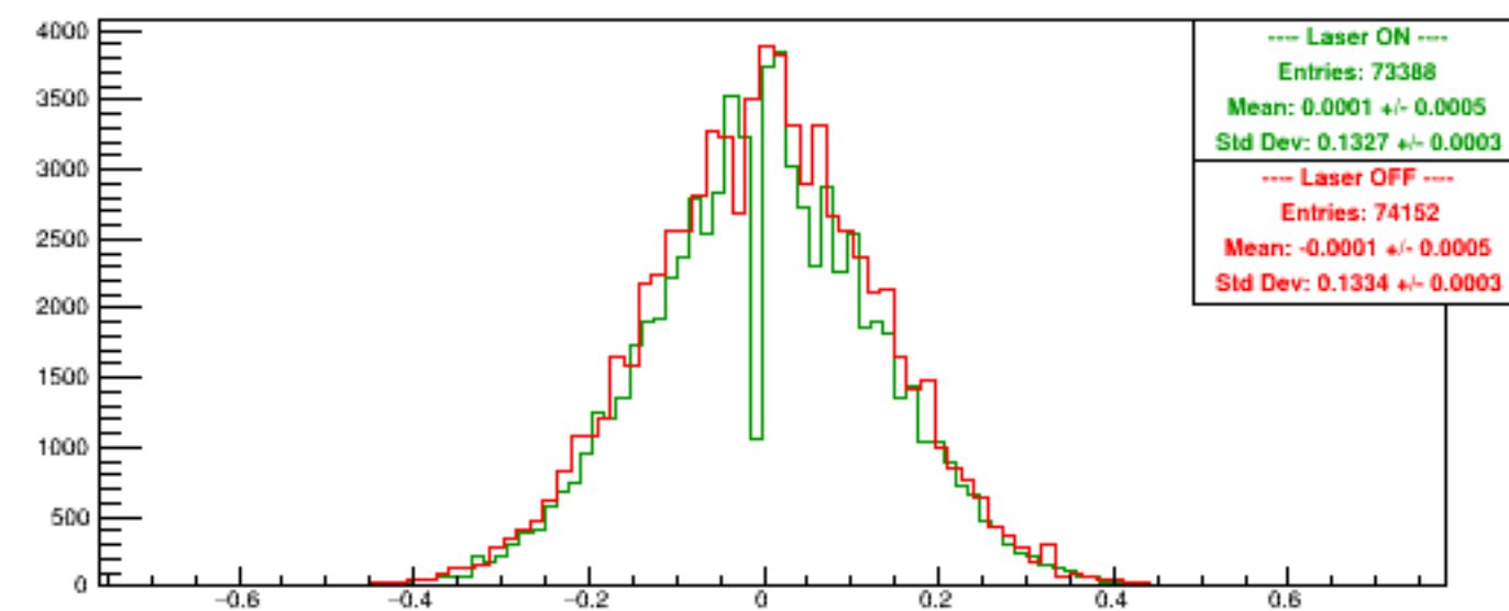
Run 5360 quartetwise, Asyms DSbg2
