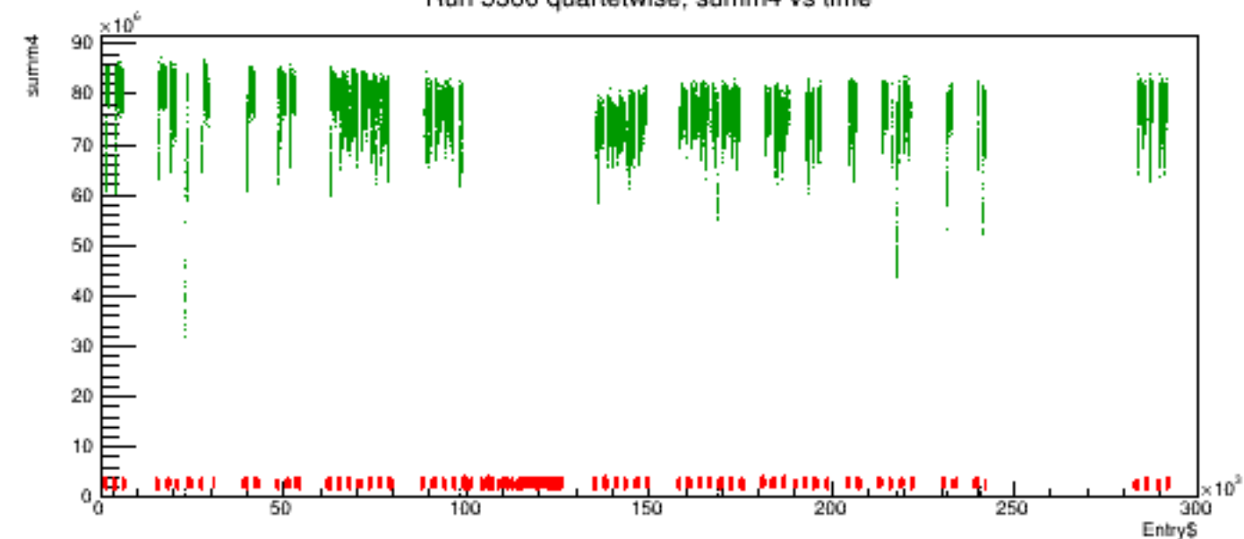
Run 5360 quartetwise, summ4 vs time
