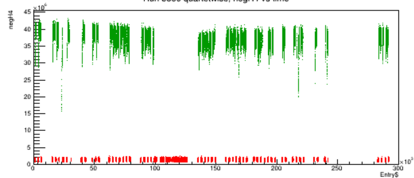
Run 5360 quartetwise, negH4 vs time
