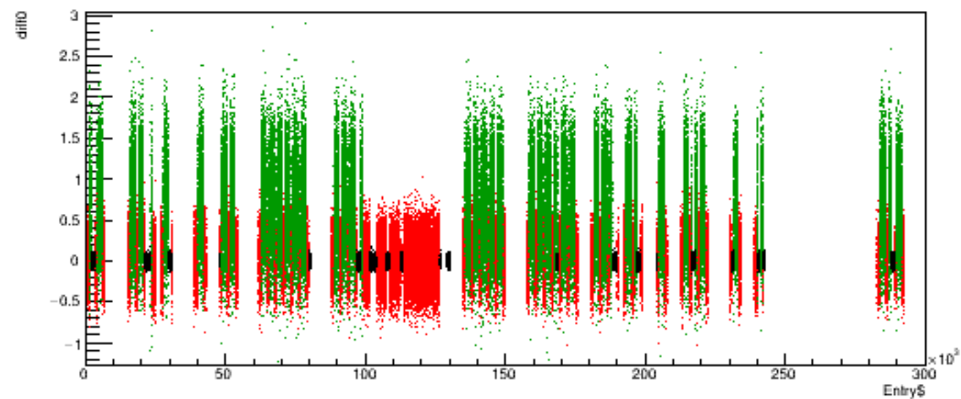
Run 5360 quartetwise, diff0 vs time
