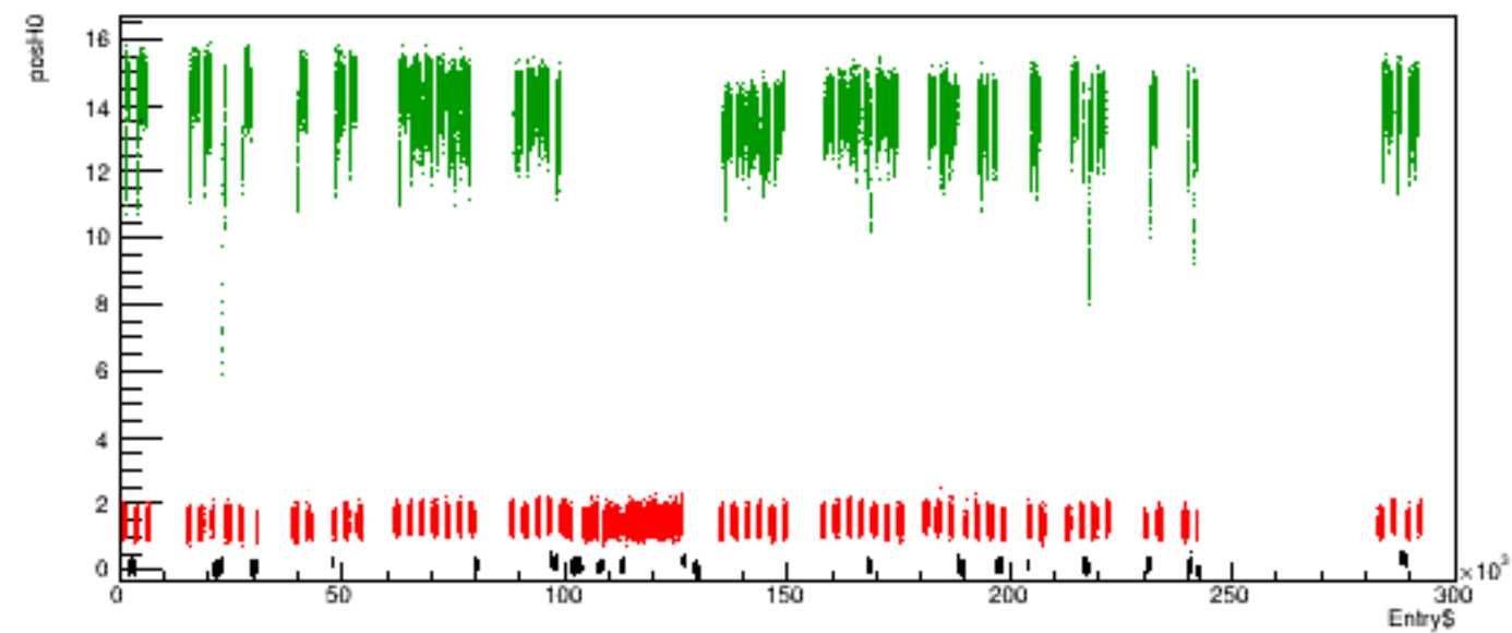
Run 5360 quartetwise, posH0 vs time
