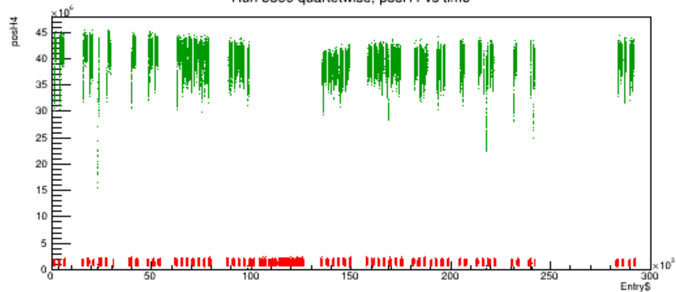
Run 5360 quartetwise, posH4 vs time
