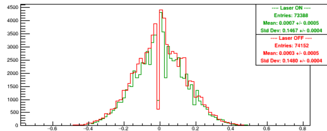
Run 5360 quartetwise, Asyms DSbg1
