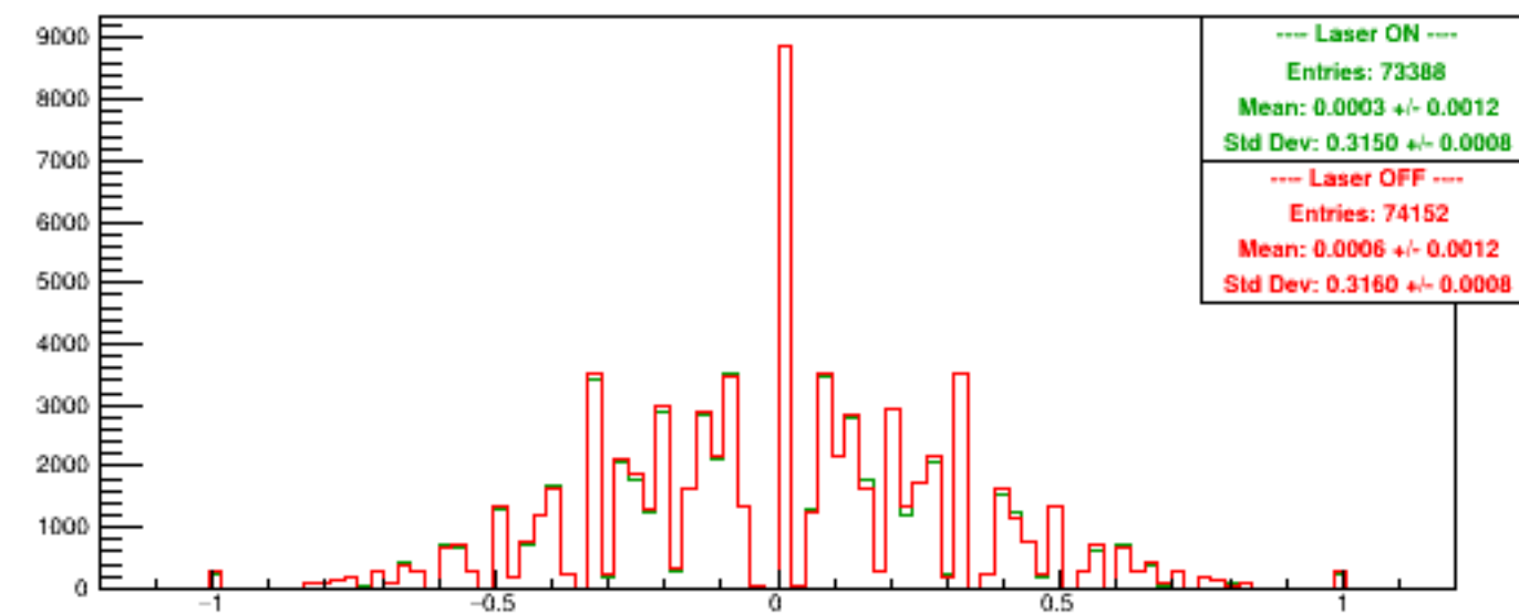
Run 5360 quartetwise, Asyms USbg2
