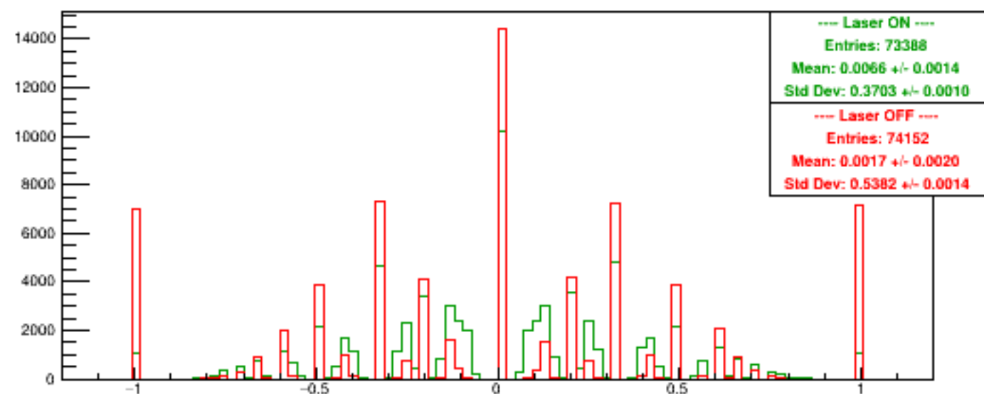
Run 5360 quartetwise, Asyms Horiz Finger
