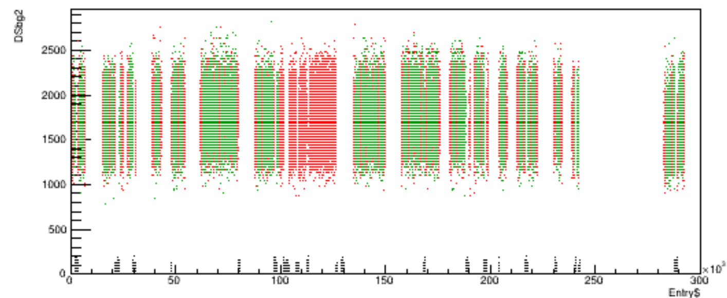
Run 5360 quartetwise, DSbg2 vs time
