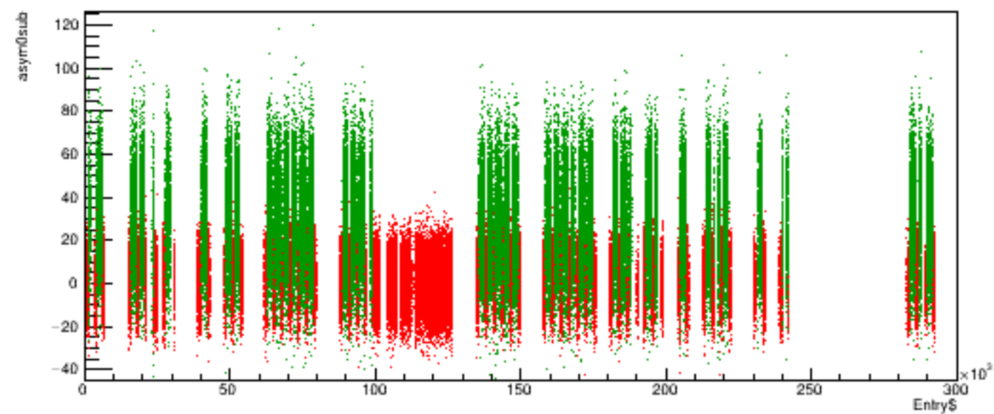
Run 5360 quartetwise, asym0sub vs time
