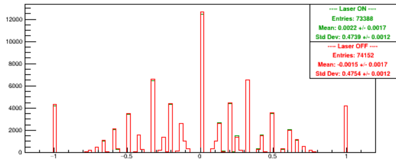
Run 5360 quartetwise, Asyms USbg1
