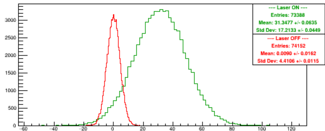
Run 5360 quartetwise, Asyms4
