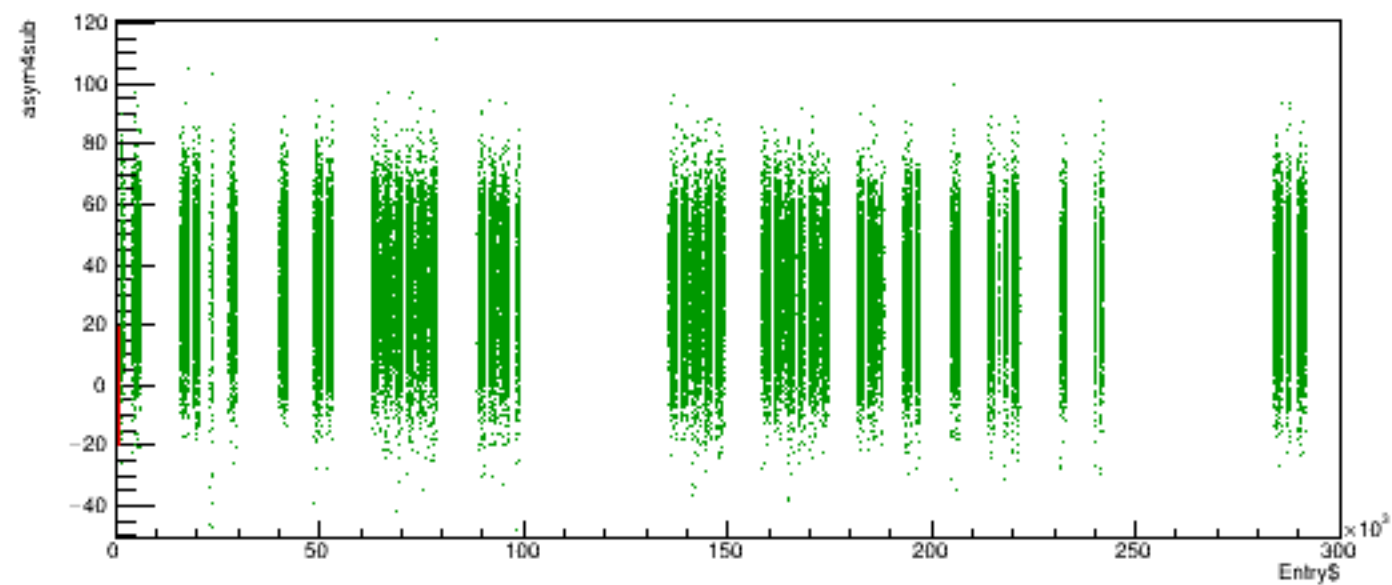
Run 5360 quartetwise, asym4sub vs time
