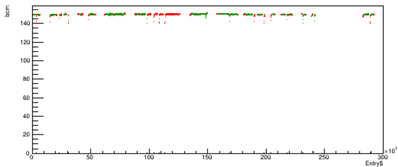
Run 5360 quartetwise, posH4 vs time
