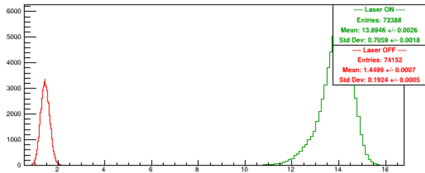
Run 5360 quartetwise, PosHelAcc0/NSamples0
