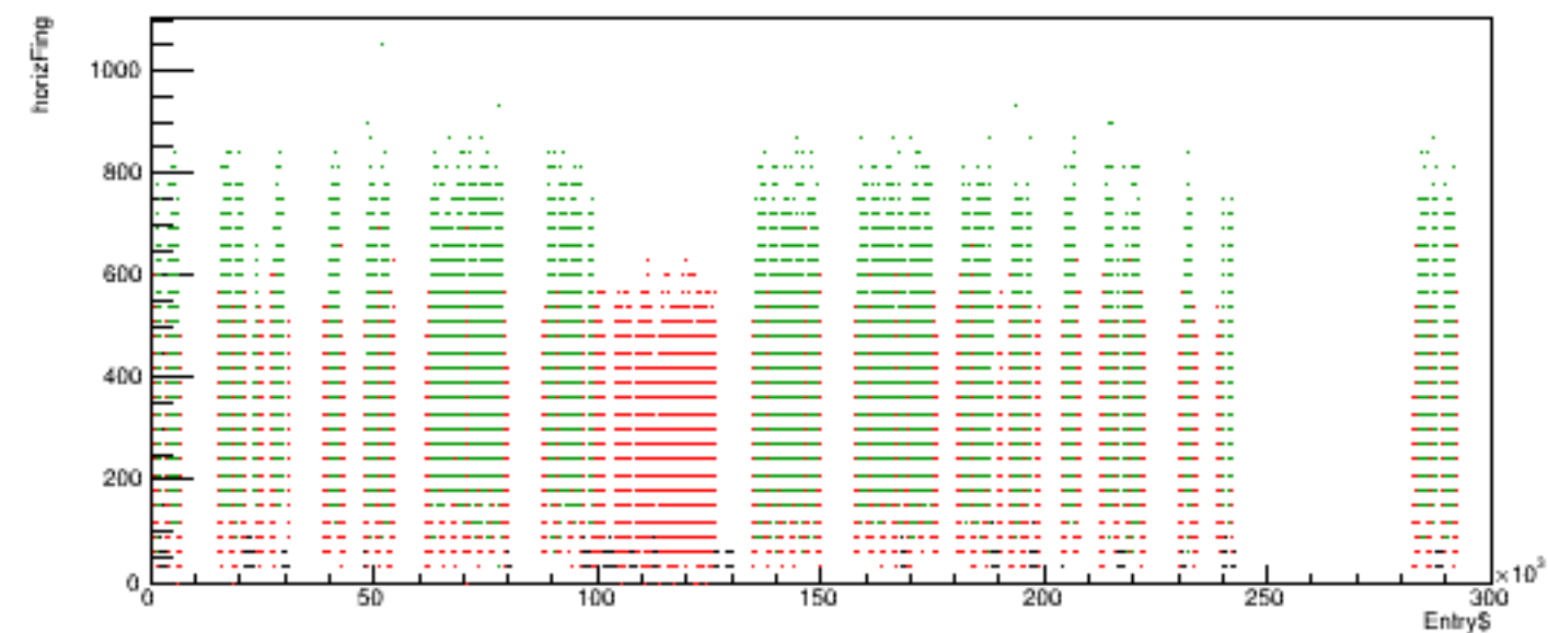
Run 5360 quartetwise, horizFing vs time
