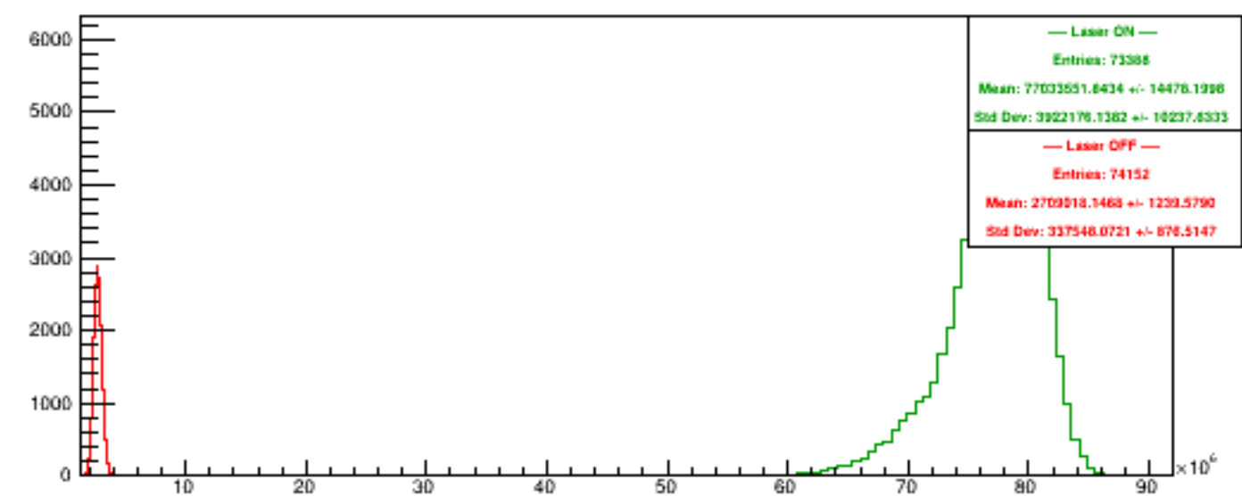
Run 5360 quartetwise, Sums4
