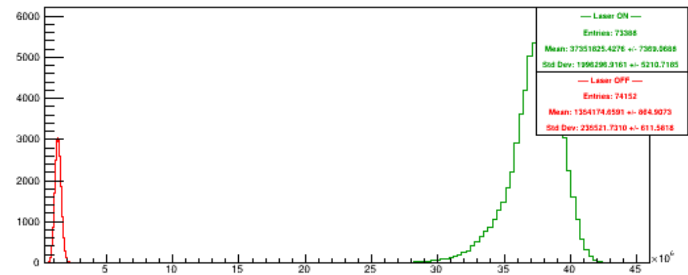
Run 5360 quartetwise, NegHelAcc4
