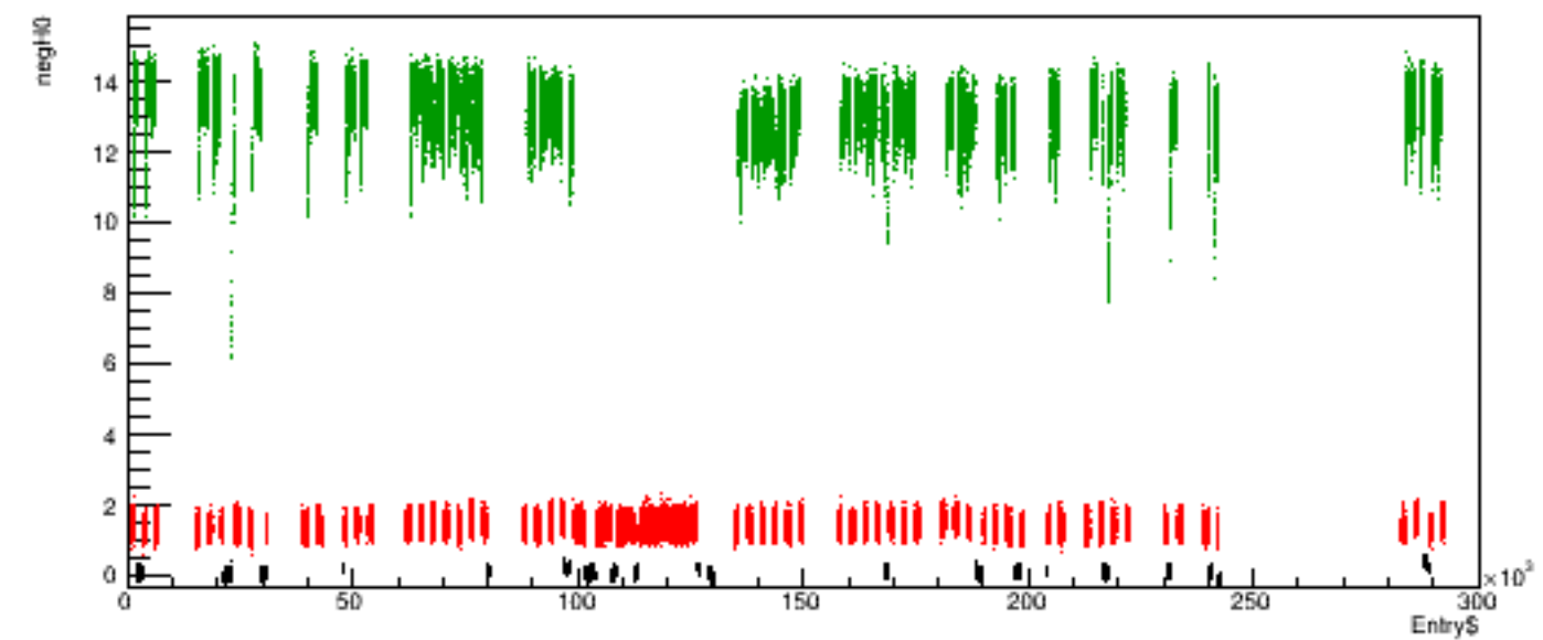
Run 5360 quartetwise, negH0 vs time
