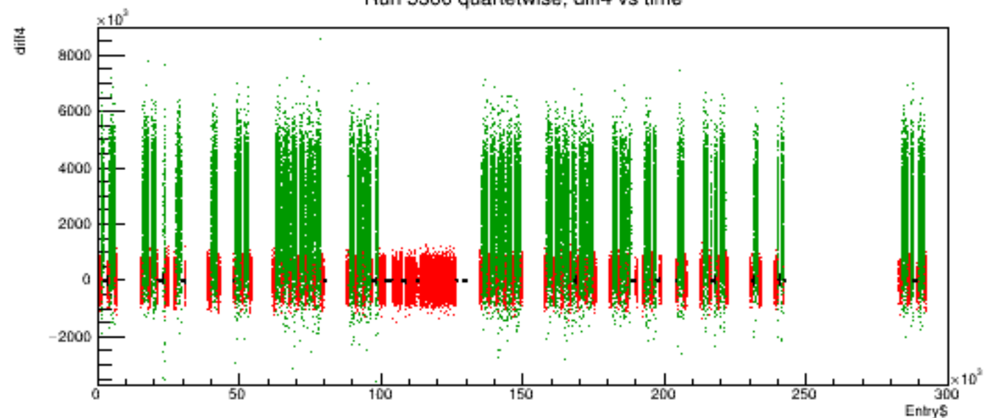
Run 5360 quartetwise, diff4 vs time
