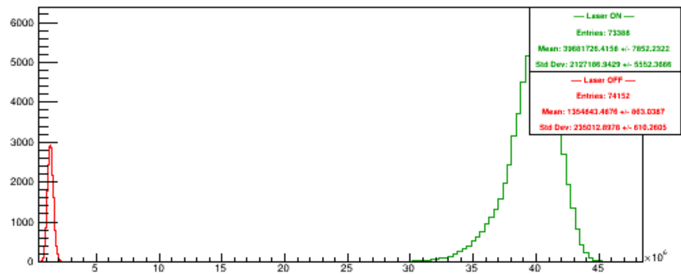
Run 5360 quartetwise, PosHelAcc4
