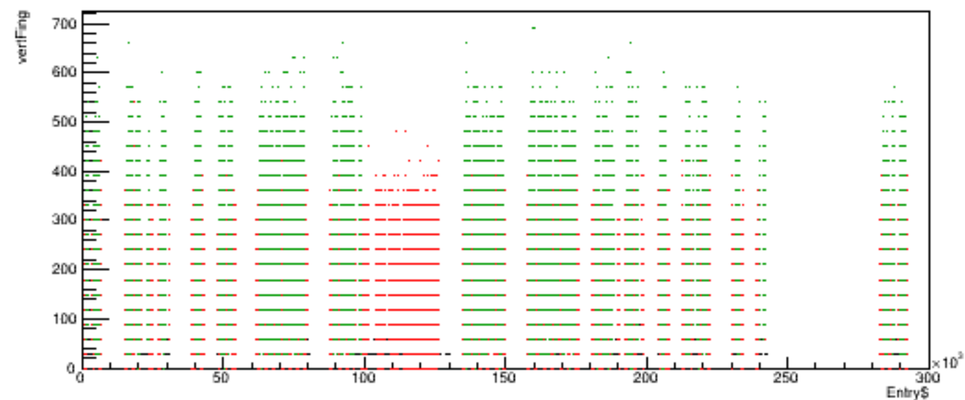
Run 5360 quartetwise, vertFing vs time
