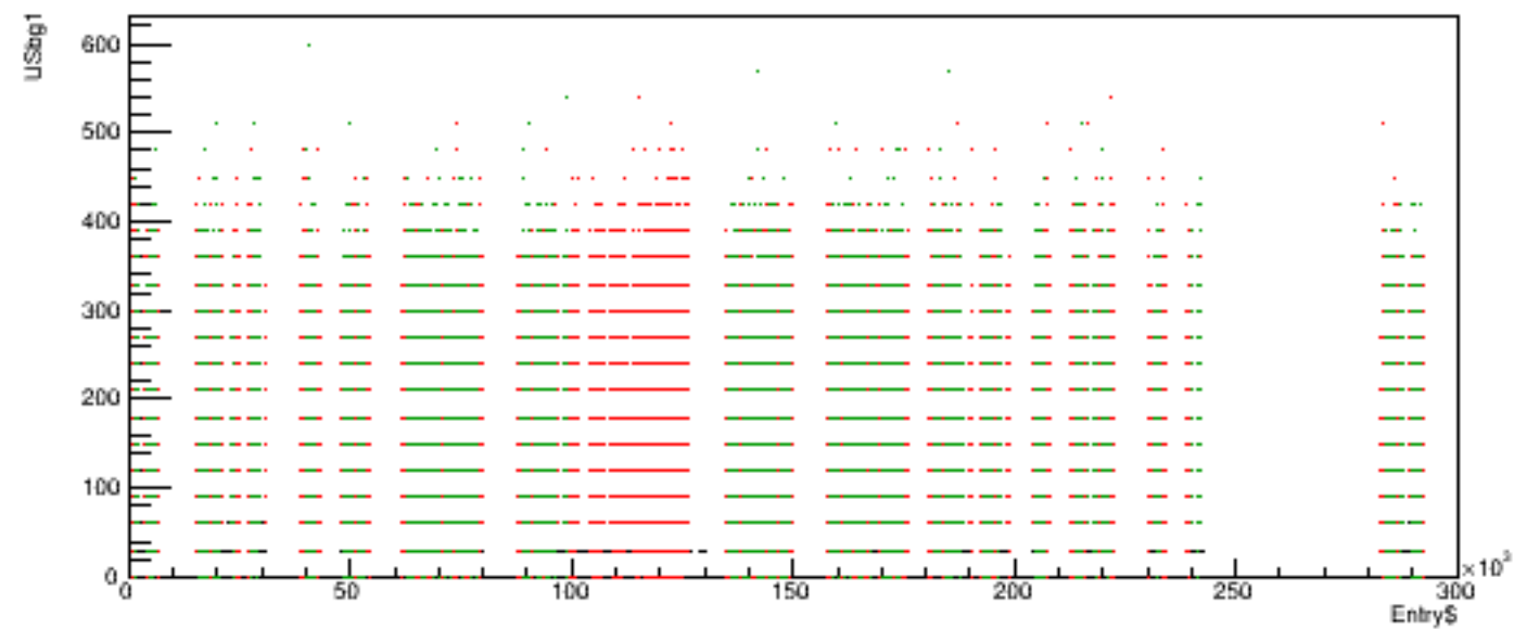
Run 5360 quartetwise, USbg1 vs time
