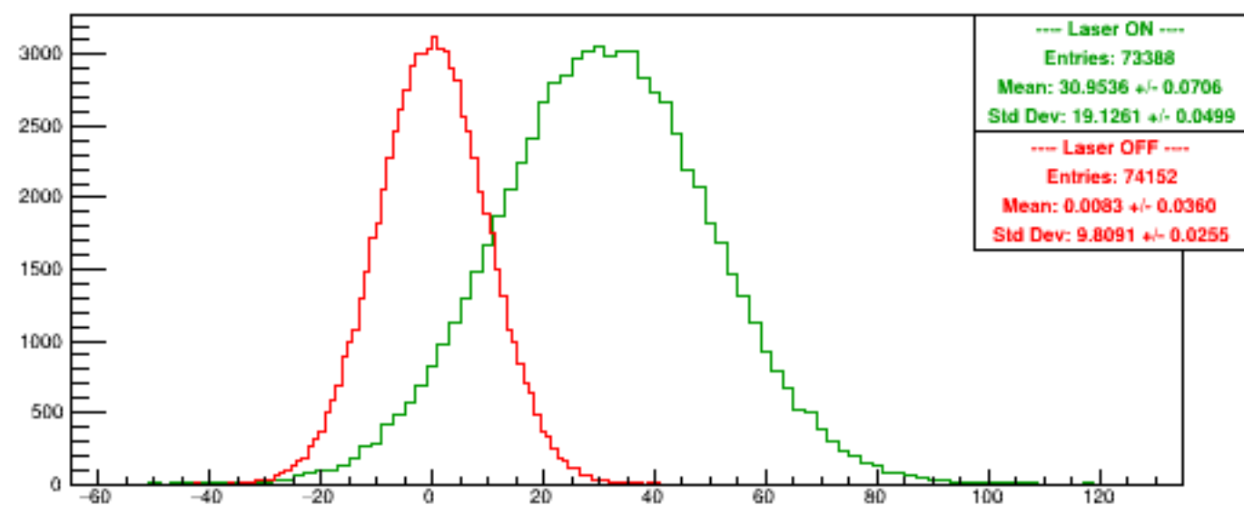
Run 5360 quartetwise, Asyms0
