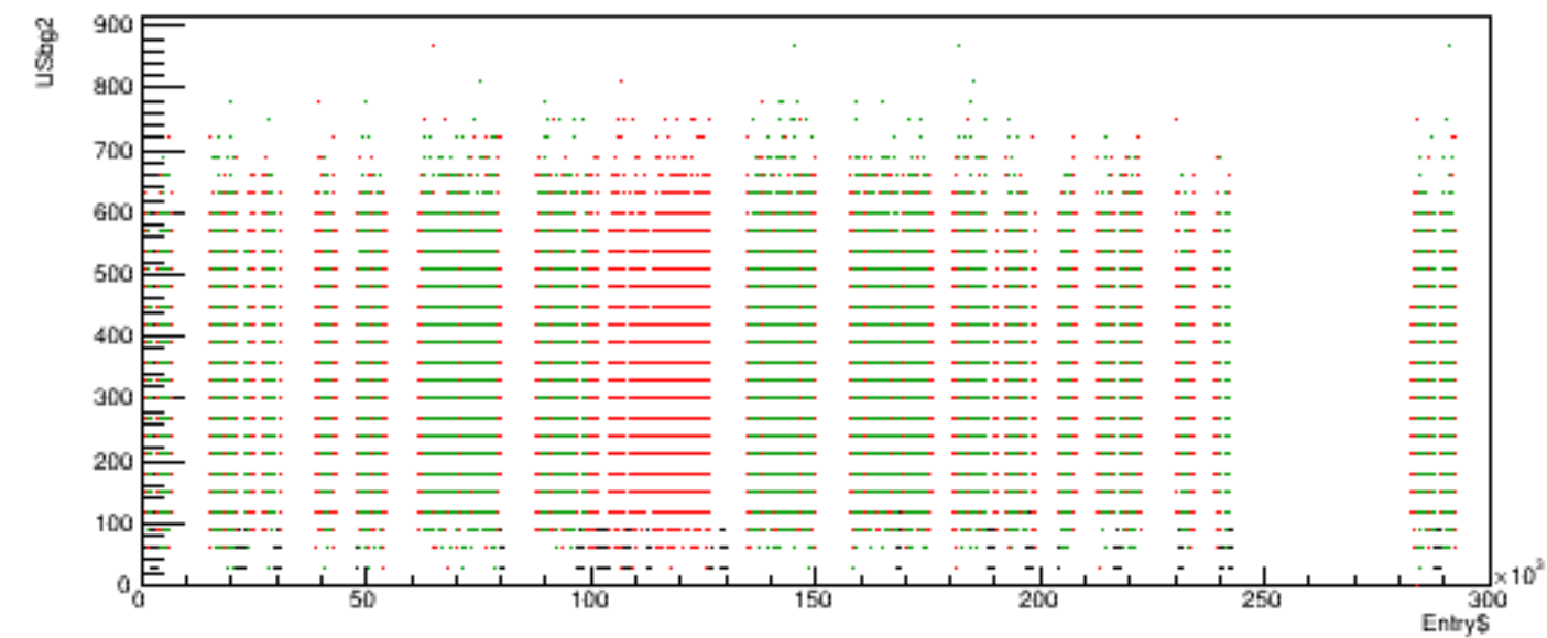
Run 5360 quartetwise, USbg2 vs time
