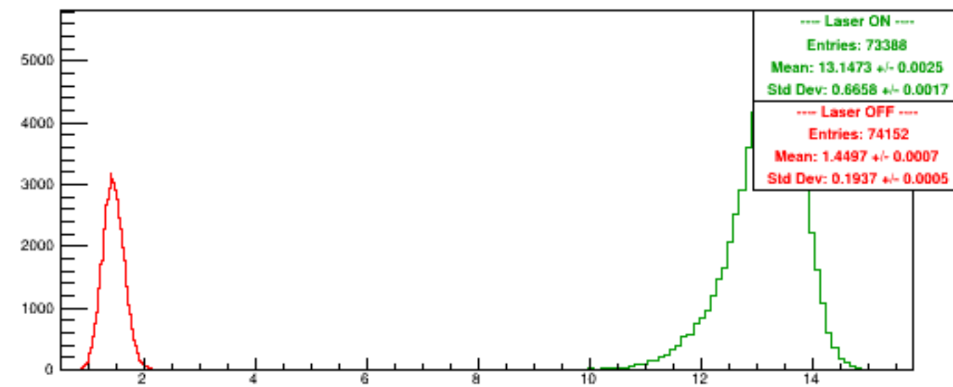
Run 5360 quartetwise, NegHelAcc0/NSamples0
