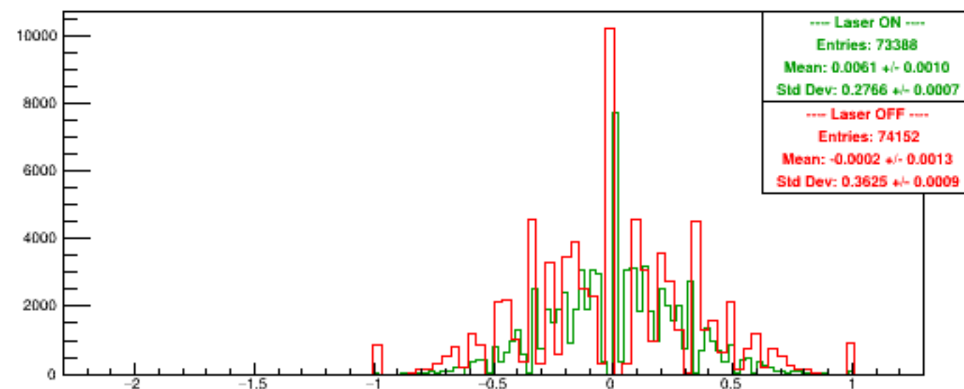
Run 5360 quartetwise, Asyms Vert Finger
