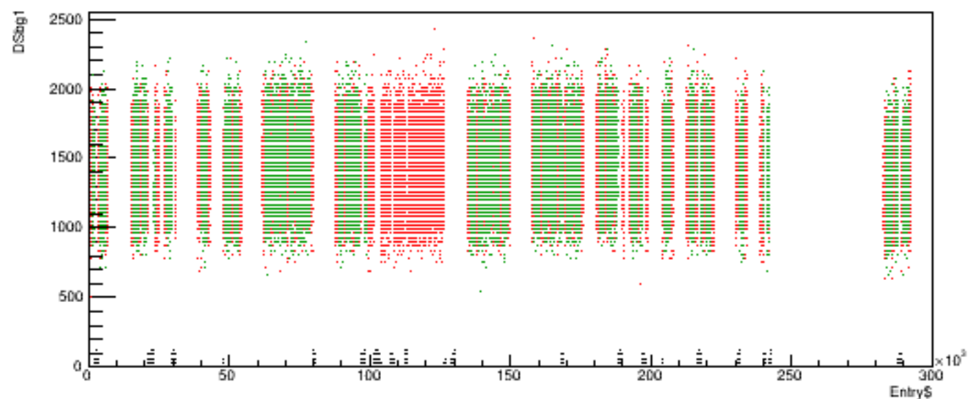
Run 5360 quartetwise, DSbg1 vs time
