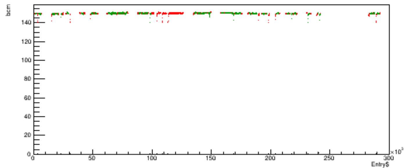
Run 5360 quartetwise, posH4 vs time
