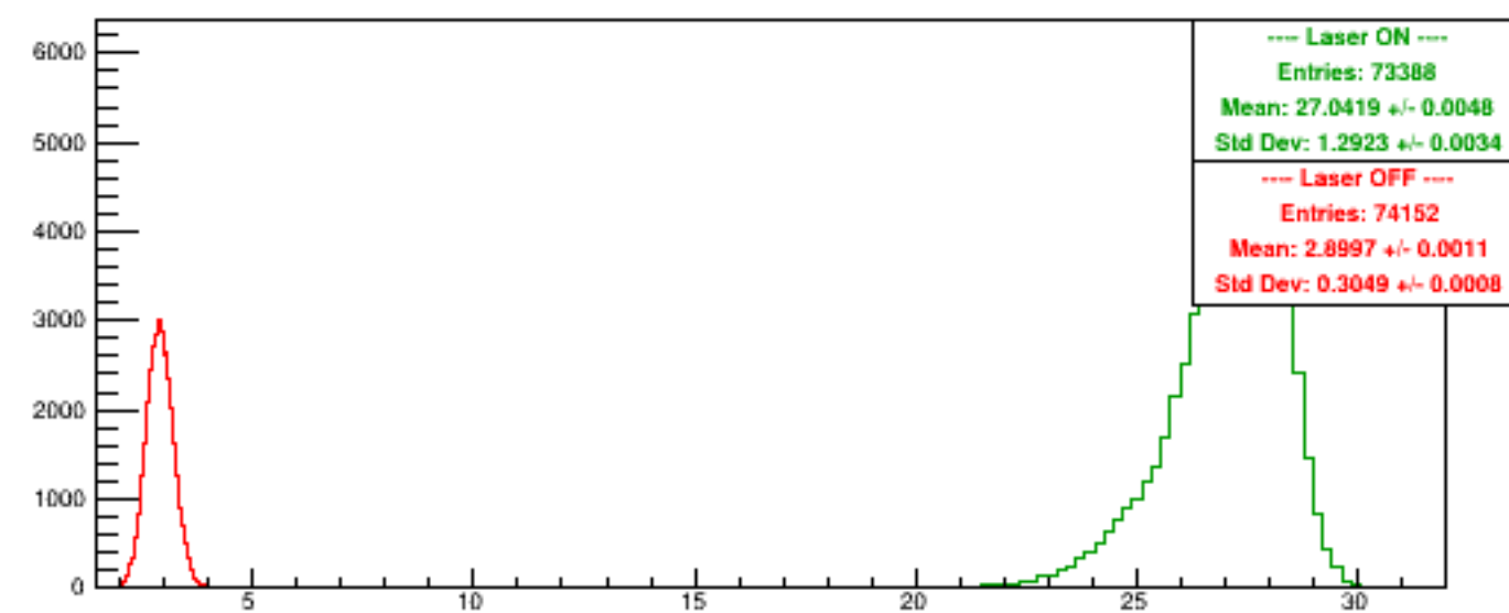
Run 5360 quartetwise, Sums0
