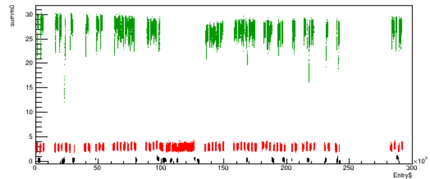
Run 5360 quartetwise, summ0 vs time
