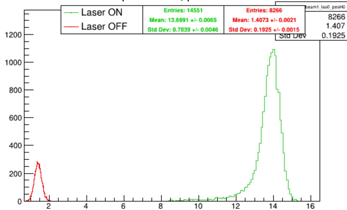
Run 5361 quartetwise, posH0: Beam ON
