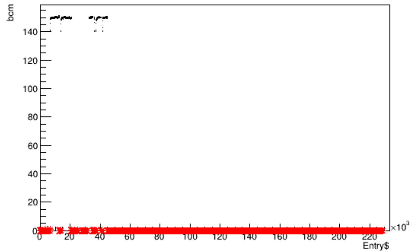
Run 5361 quartetwise, bcm vs time
