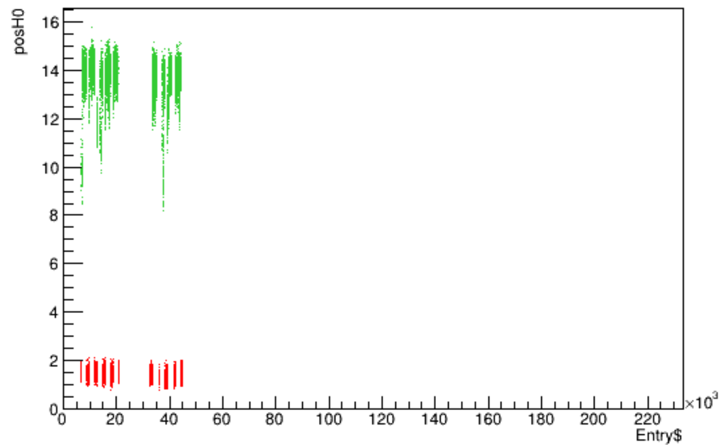
Run 5361 quartetwise, posH0 vs time
