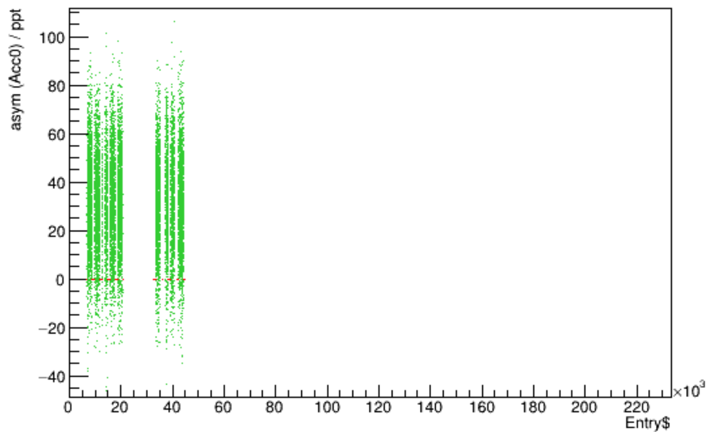
Run 5361 quartetwise, asym0sub vs time
