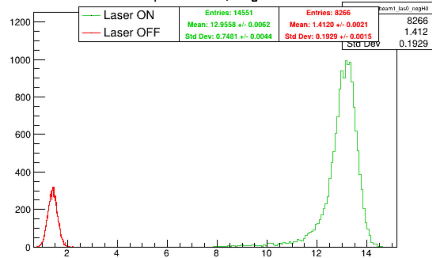
Run 5361 quartetwise, negH0: Beam ON
