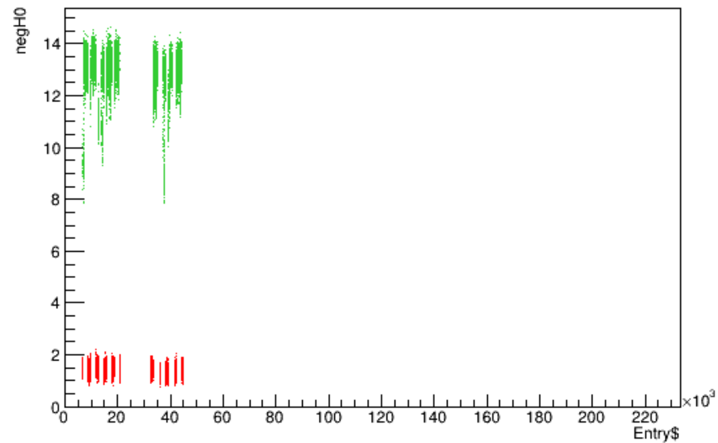
Run 5361 quartetwise, negH0 vs time
