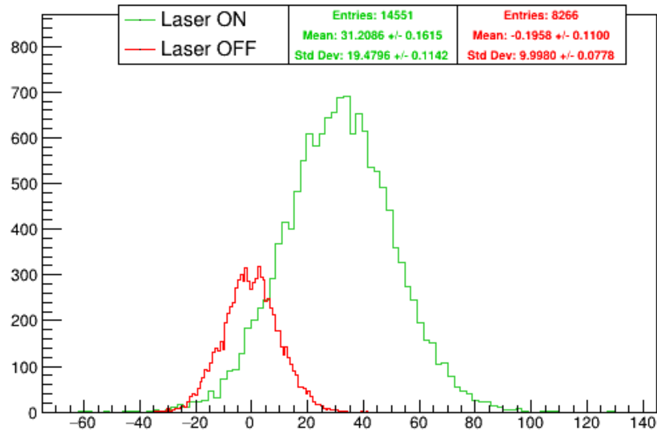
Run 5361 quartetwise, asym0sub: Beam ON
