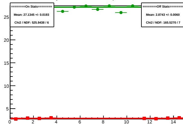
Cycle 5361.4: Multiplet Sums
