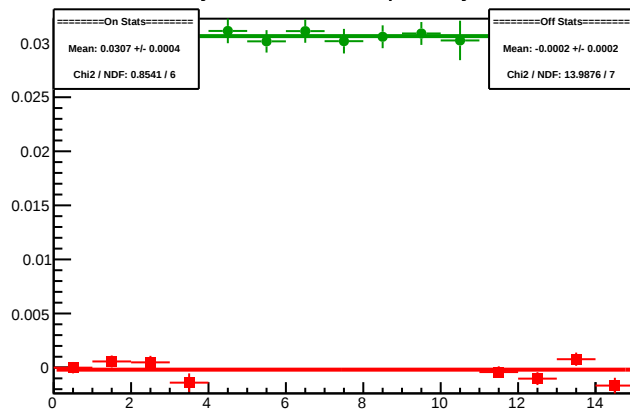
Cycle 5361.2: Multiplet Asyms
