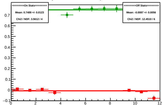
Cycle 5361.8: Multiplet Diffs
