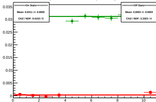
Cycle 5361.6: Multiplet Asyms
