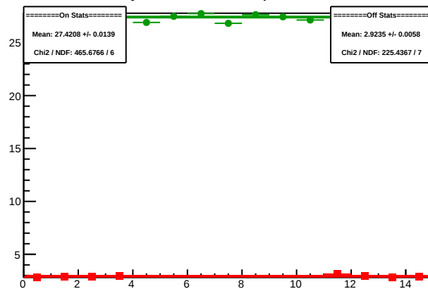
Cycle 5361.2: Multiplet Sums
