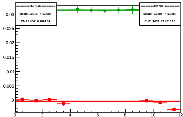
Cycle 5361.8: Multiplet Asyms
