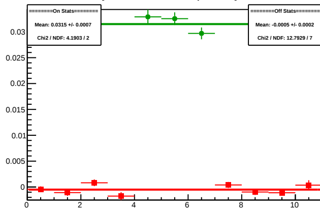
Cycle 5361.3: Multiplet Asyms
