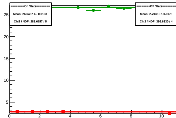
Cycle 5361.6: Multiplet Sums
