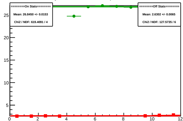
Cycle 5361.8: Multiplet Sums
