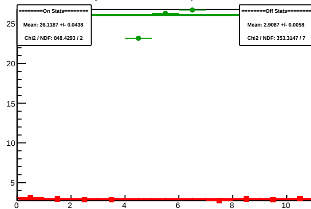
Cycle 5361.3: Multiplet Sums
