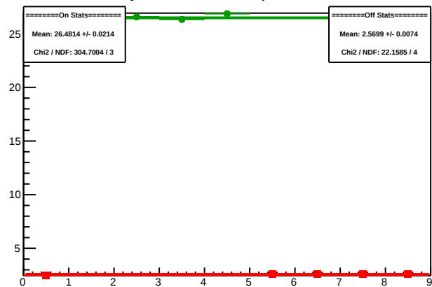
Cycle 5361.7: Multiplet Sums
