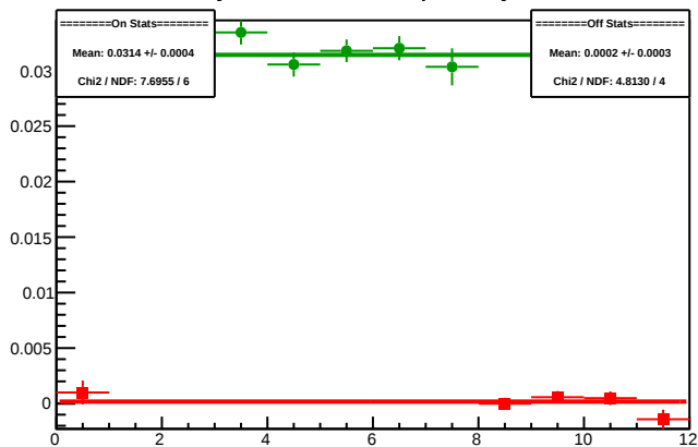
Cycle 5361.1: Multiplet Asyms
