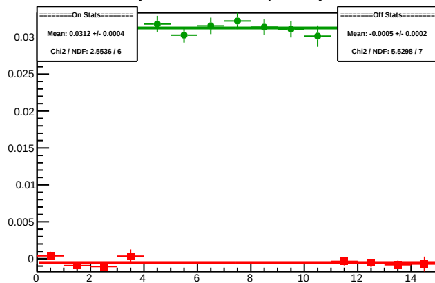
Cycle 5361.4: Multiplet Asyms
