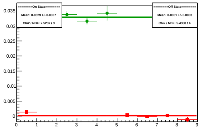
Cycle 5361.7: Multiplet Asyms
