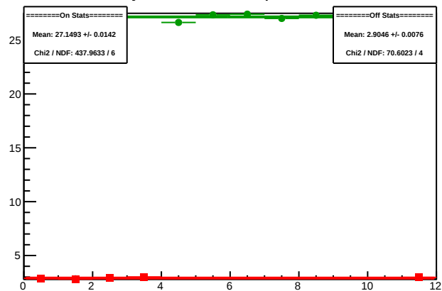
Cycle 5361.5: Multiplet Sums
