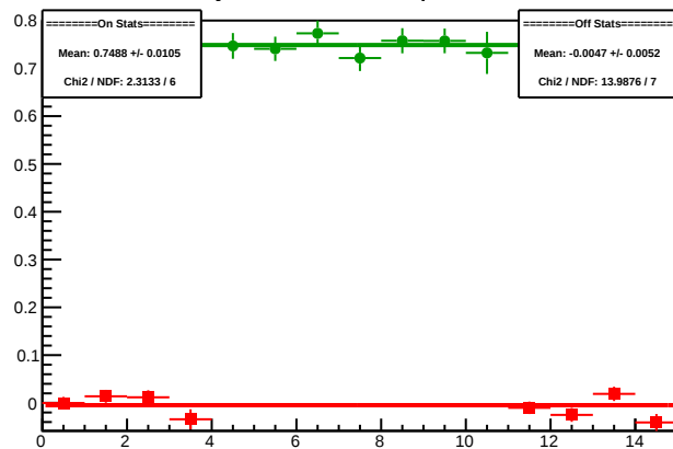
Cycle 5361.2: Multiplet Diffs
