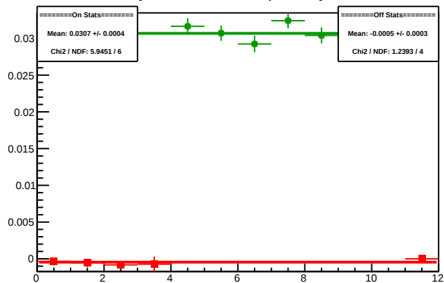
Cycle 5361.5: Multiplet Asyms
