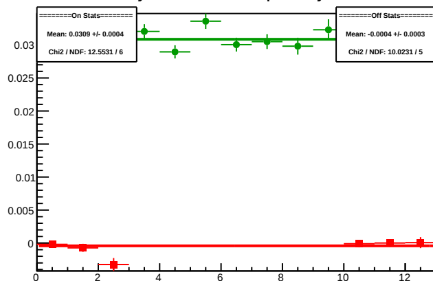
Cycle 5361.9: Multiplet Asyms
