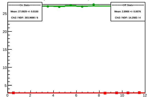
Cycle 5361.1: Multiplet Sums
