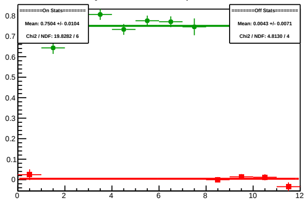
Cycle 5361.1: Multiplet Diffs
