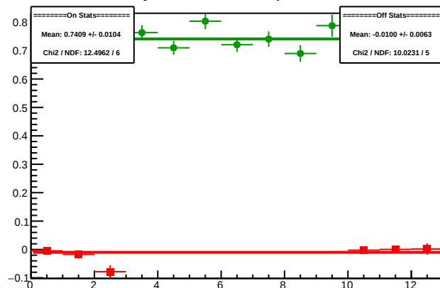
Cycle 5361.9: Multiplet Diffs
