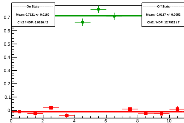
Cycle 5361.3: Multiplet Diffs
