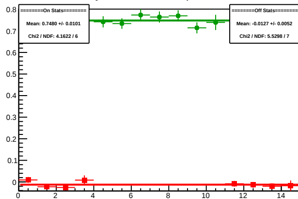
Cycle 5361.4: Multiplet Diffs
