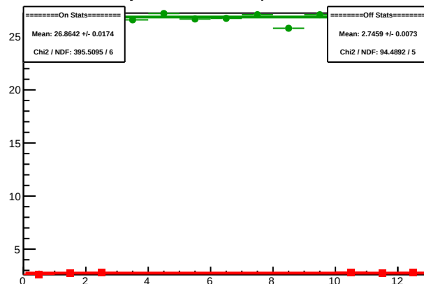
Cycle 5361.9: Multiplet Sums
