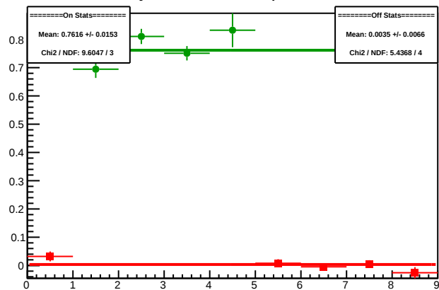
Cycle 5361.7: Multiplet Diffs
