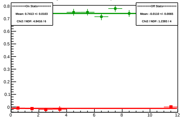
Cycle 5361.5: Multiplet Diffs
