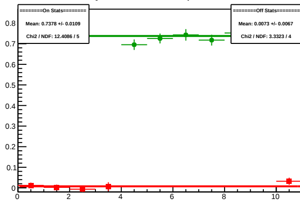
Cycle 5361.6: Multiplet Diffs
