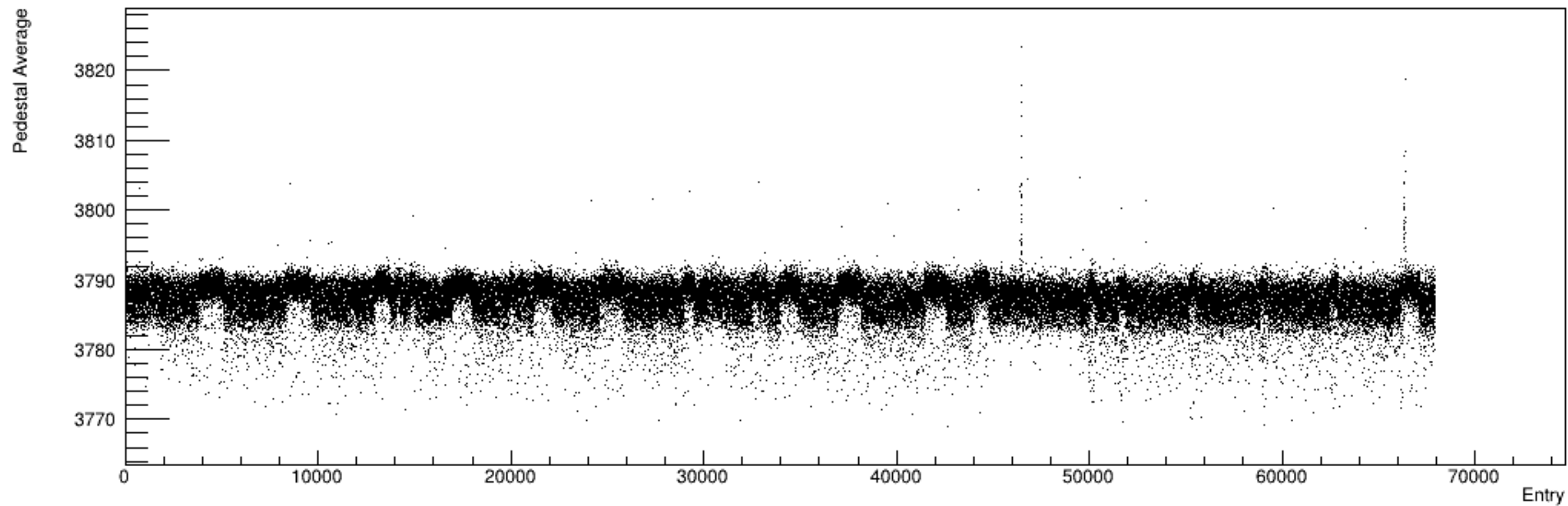
Run 5369, snapshots: Pedestal vs. Time
