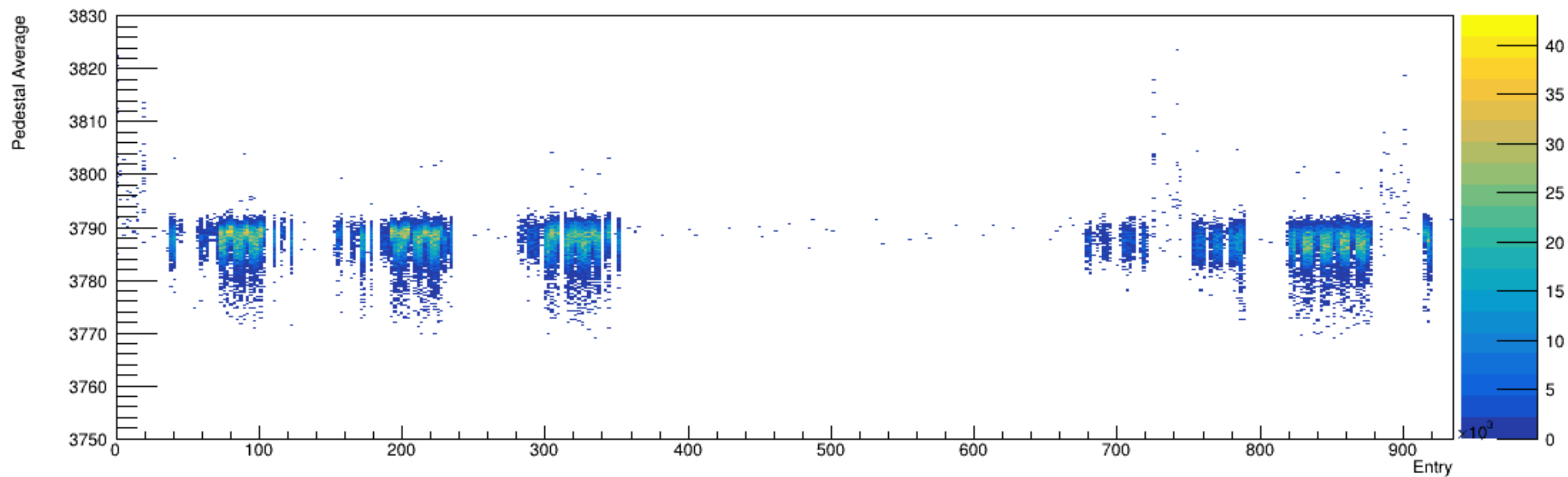
Run 5369, snapshots: Pedestal vs. Time
