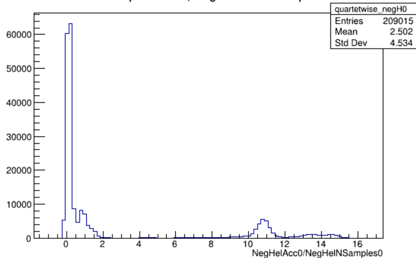
Run 5370 quartetwise, NegHelAcc0/NSamples0: All
