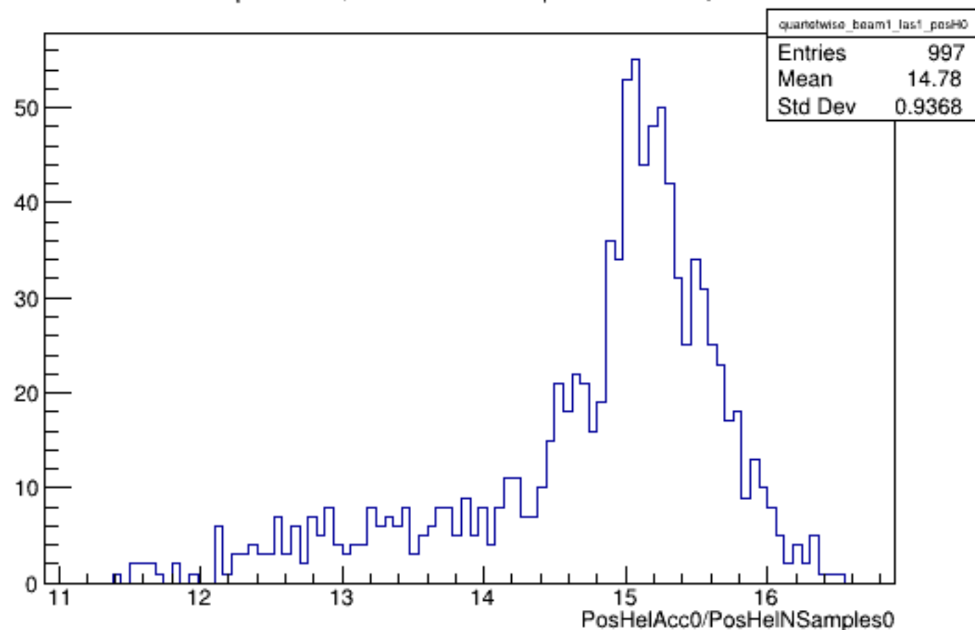
Run 5370 quartetwise, PosHelAcc0/NSamples0: Beam ON, Laser ON
