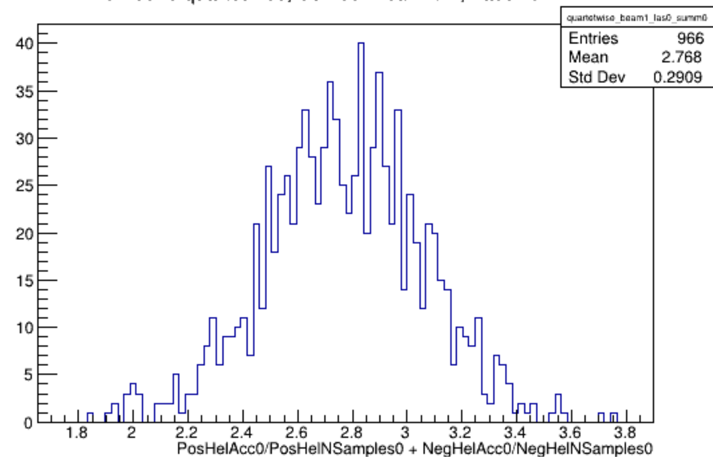
Run 5370 quartetwise, Sums0: Beam ON, Laser OFF
