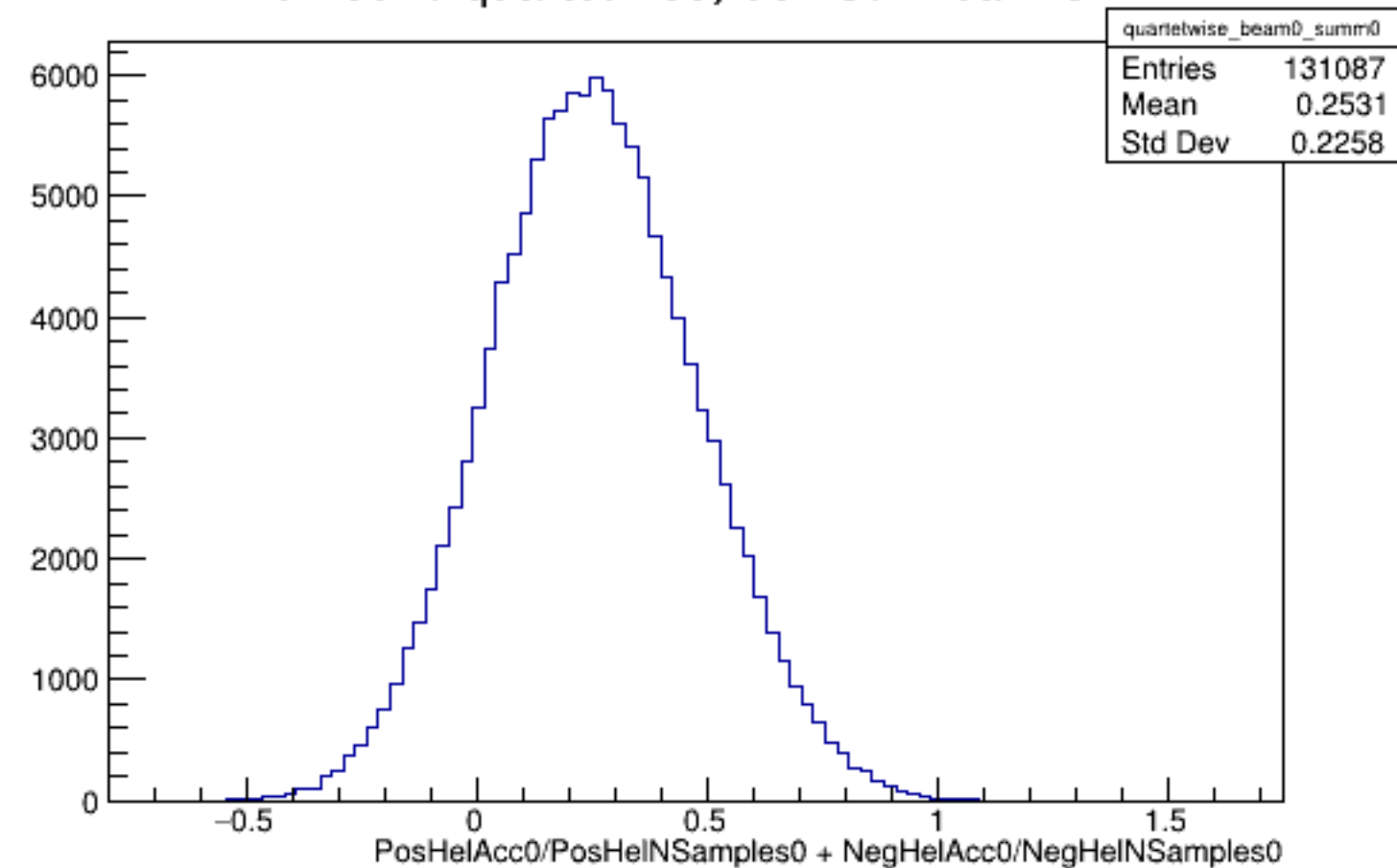
Run 5370 quartetwise, Sums0: Beam OFF
