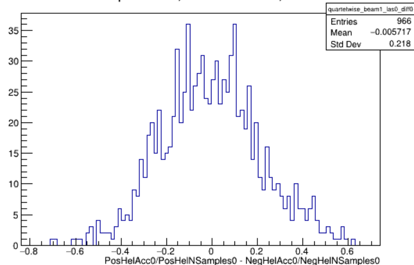
Run 5370 quartetwise, Diffs0: Beam ON, Laser OFF
