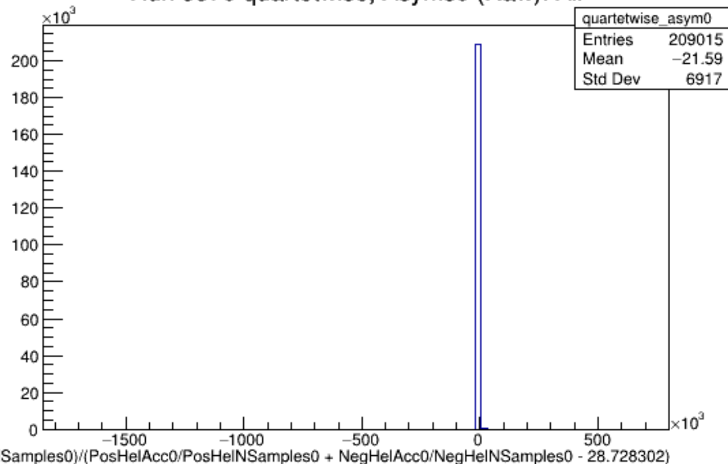
Run 5370 quartetwise, Asyms0 (Raw): All
