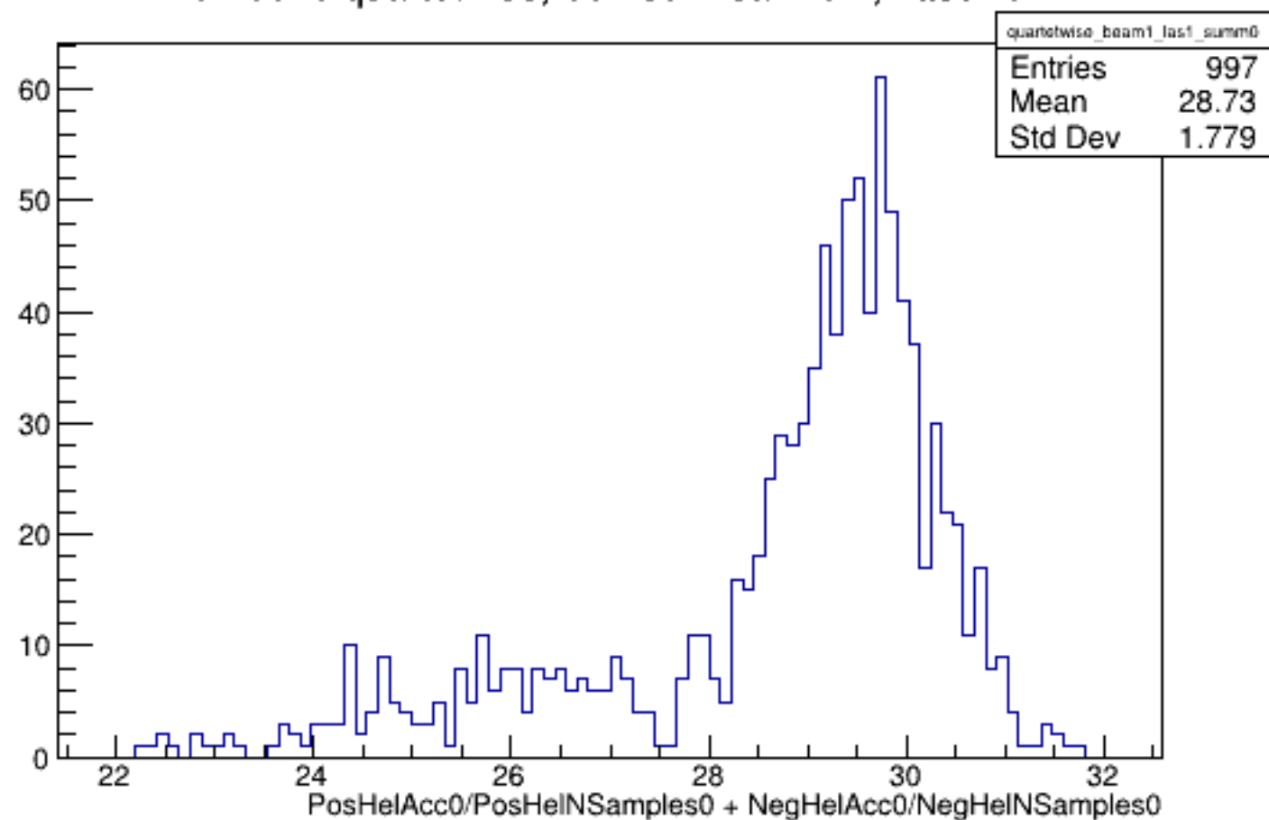
Run 5370 quartetwise, Sums0: Beam ON, Laser ON
