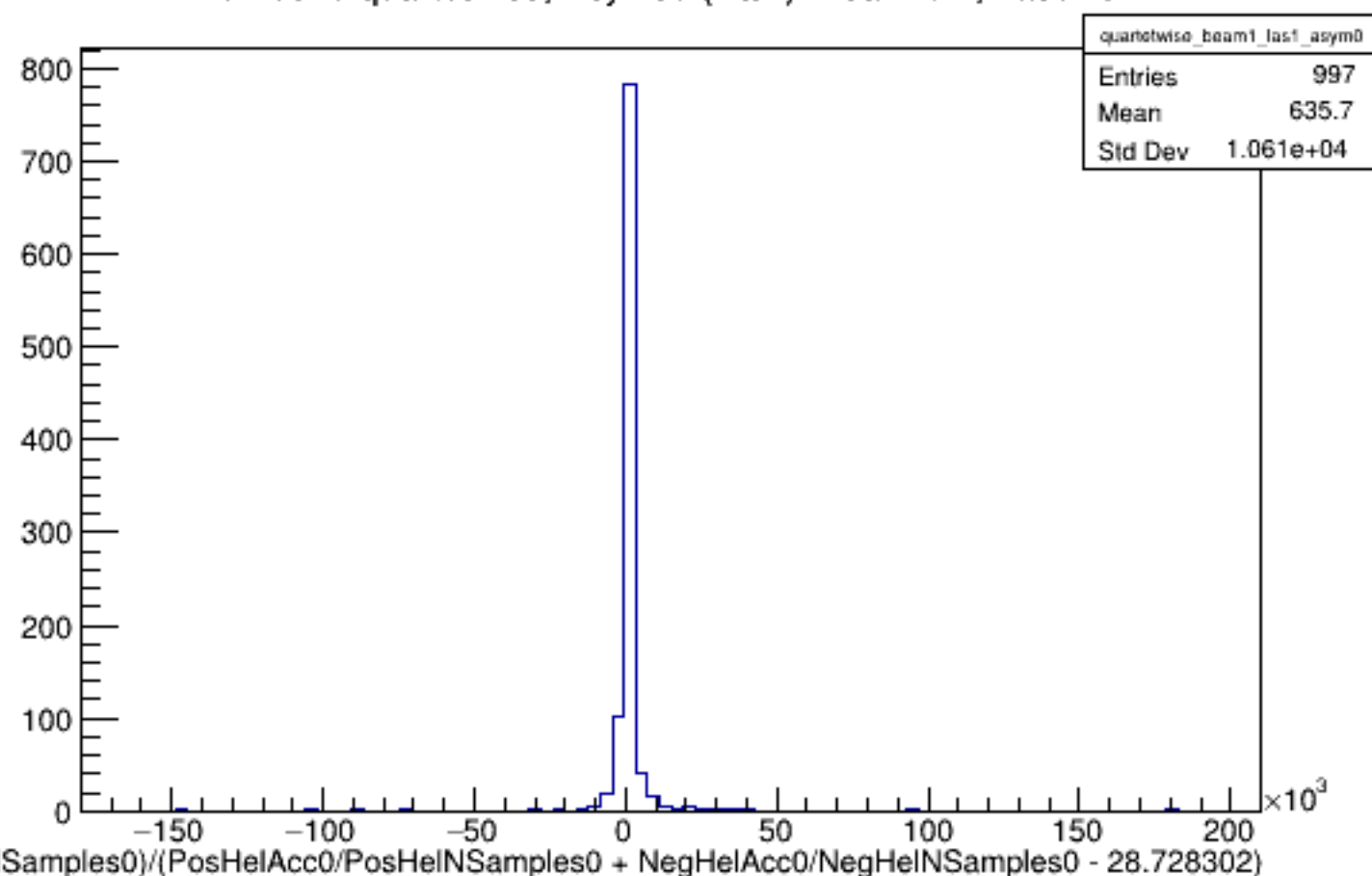
Run 5370 quartetwise, Asyms0 (Raw): Beam ON, Laser ON
