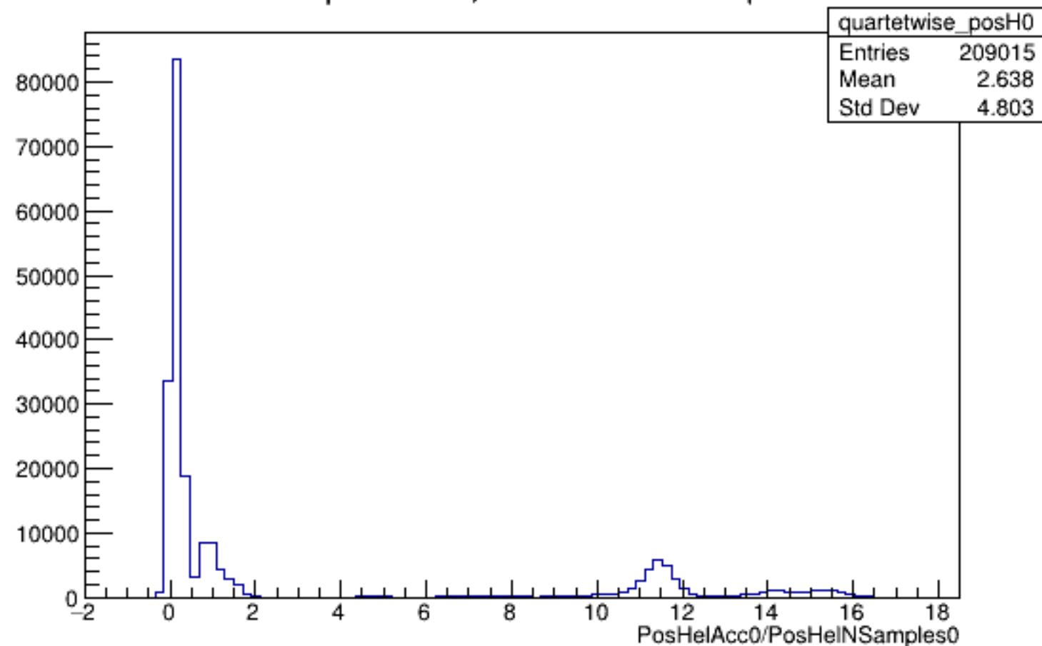
Run 5370 quartetwise, PosHelAcc0/NSamples0: All
