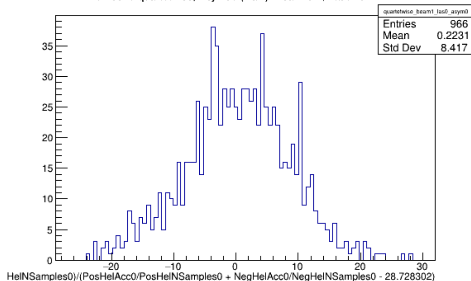
Run 5370 quartetwise, Asyms0 (Raw): Beam ON, Laser OFF
