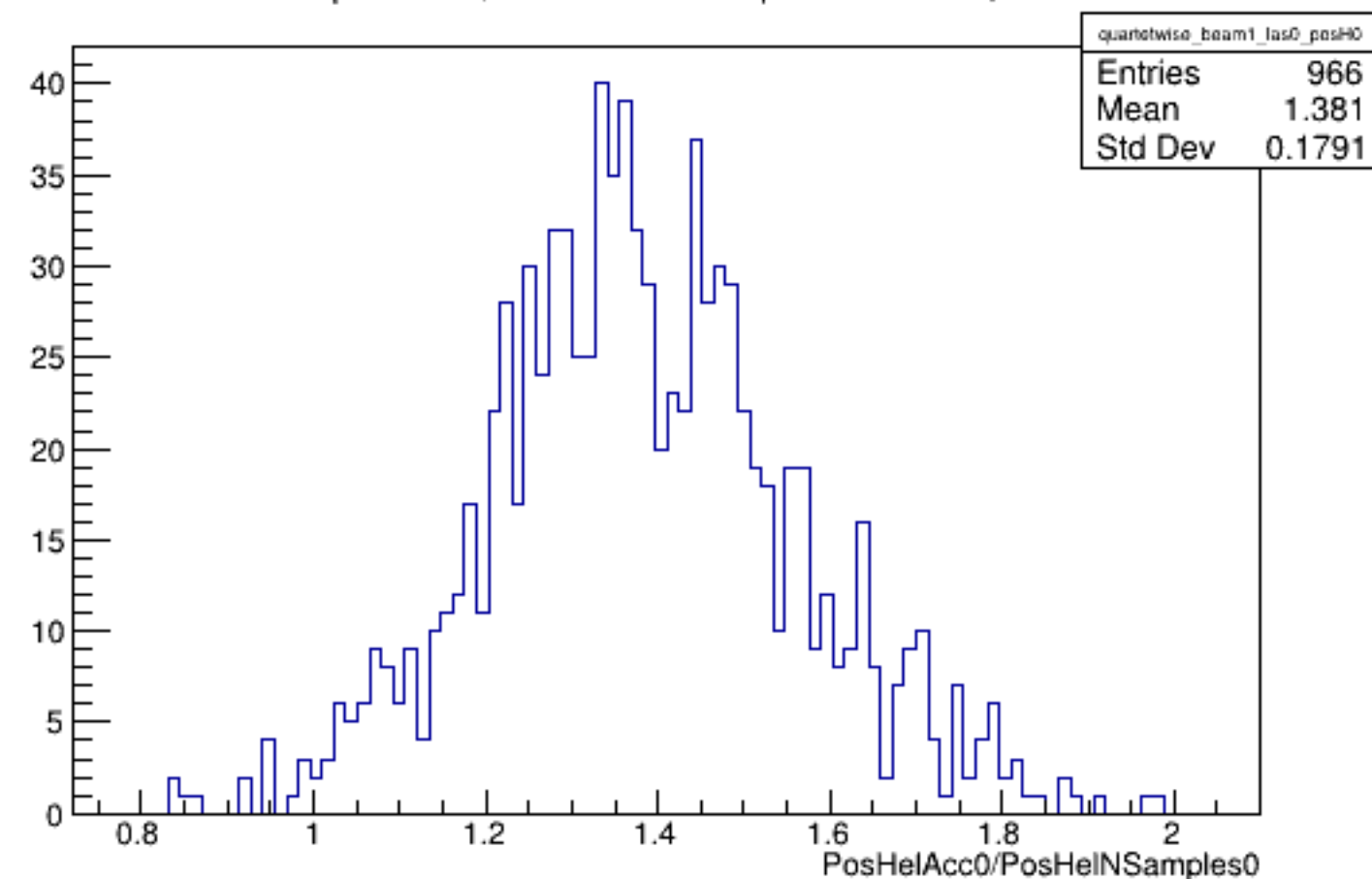
Run 5370 quartetwise, PosHelAcc0/NSamples0: Beam ON, Laser OFF
