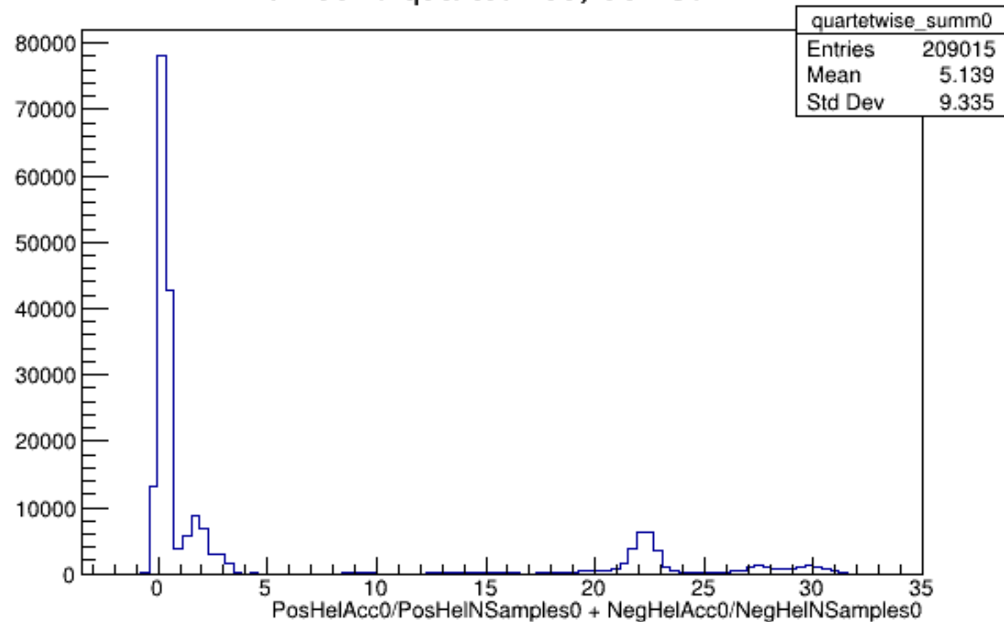
Run 5370 quartetwise, Sums0: All
