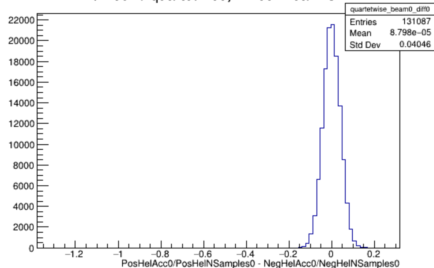
Run 5370 quartetwise, Diffs0: Beam OFF
