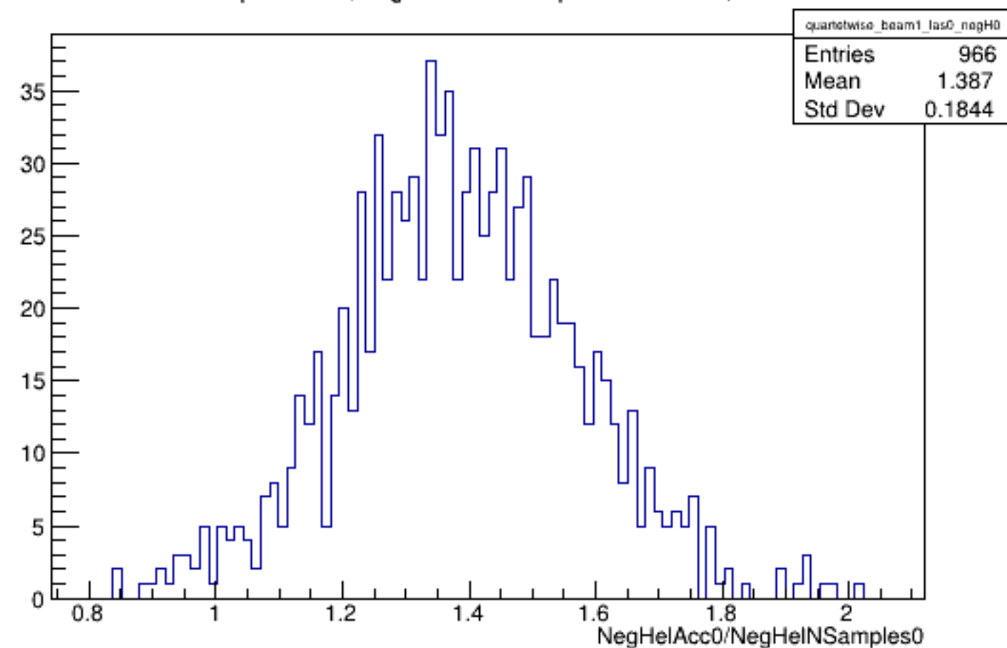
Run 5370 quartetwise, NegHelAcc0/NSamples0: Beam ON, Laser OFF
