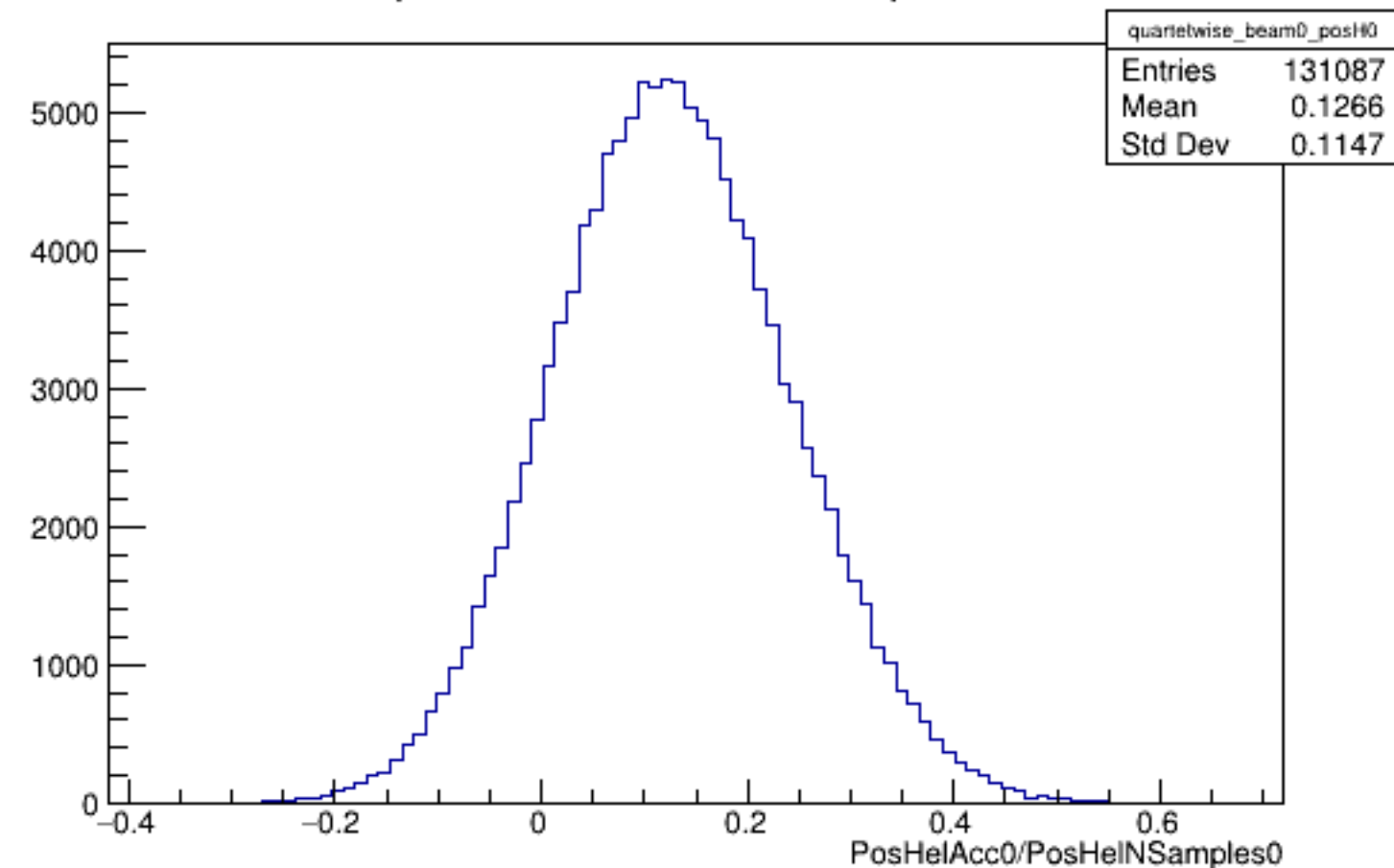
Run 5370 quartetwise, PosHelAcc0/NSamples0: Beam OFF
