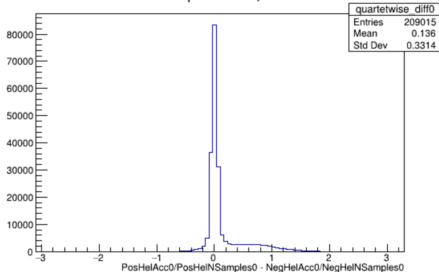
Run 5370 quartetwise, Diffs0: All
