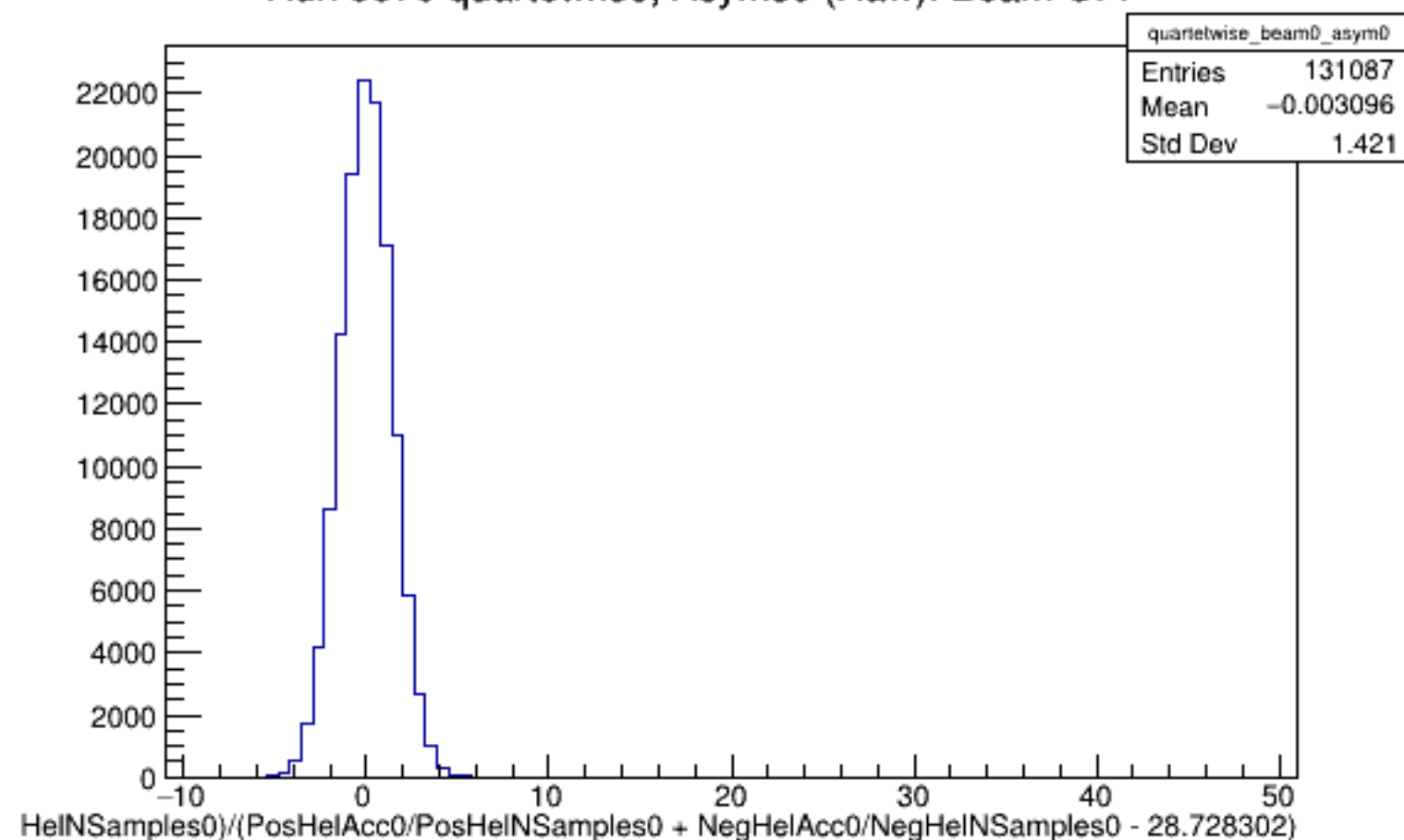
Run 5370 quartetwise, Asyms0 (Raw): Beam OFF
