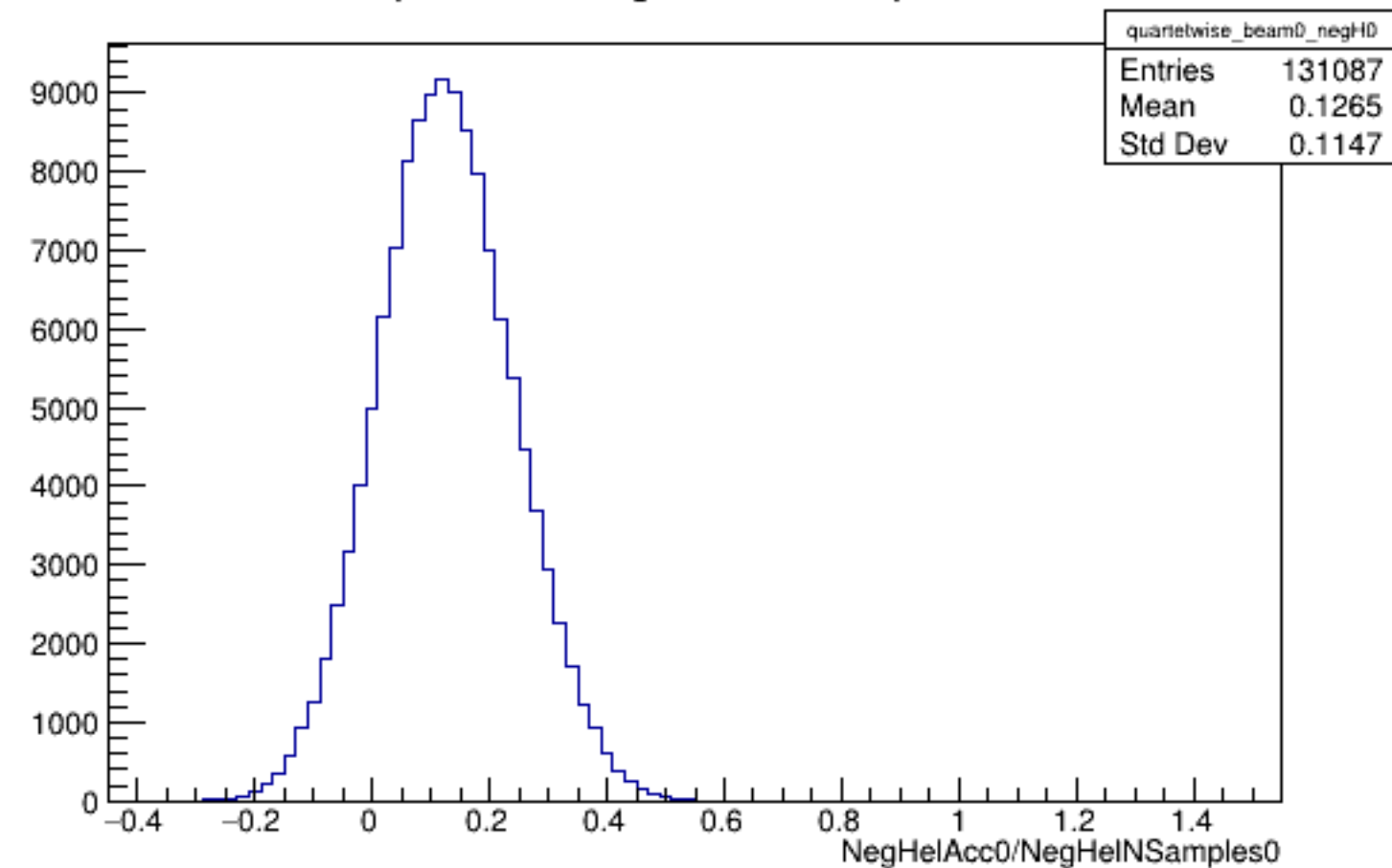
Run 5370 quartetwise, NegHelAcc0/NSamples0: Beam OFF
