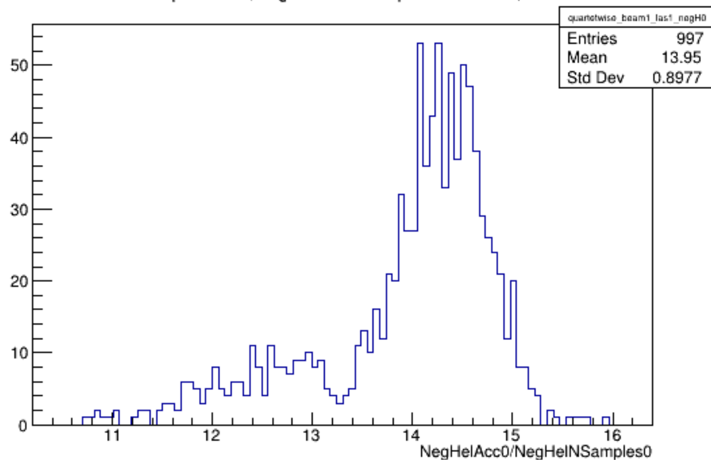
Run 5370 quartetwise, NegHelAcc0/NSamples0: Beam ON, Laser ON
