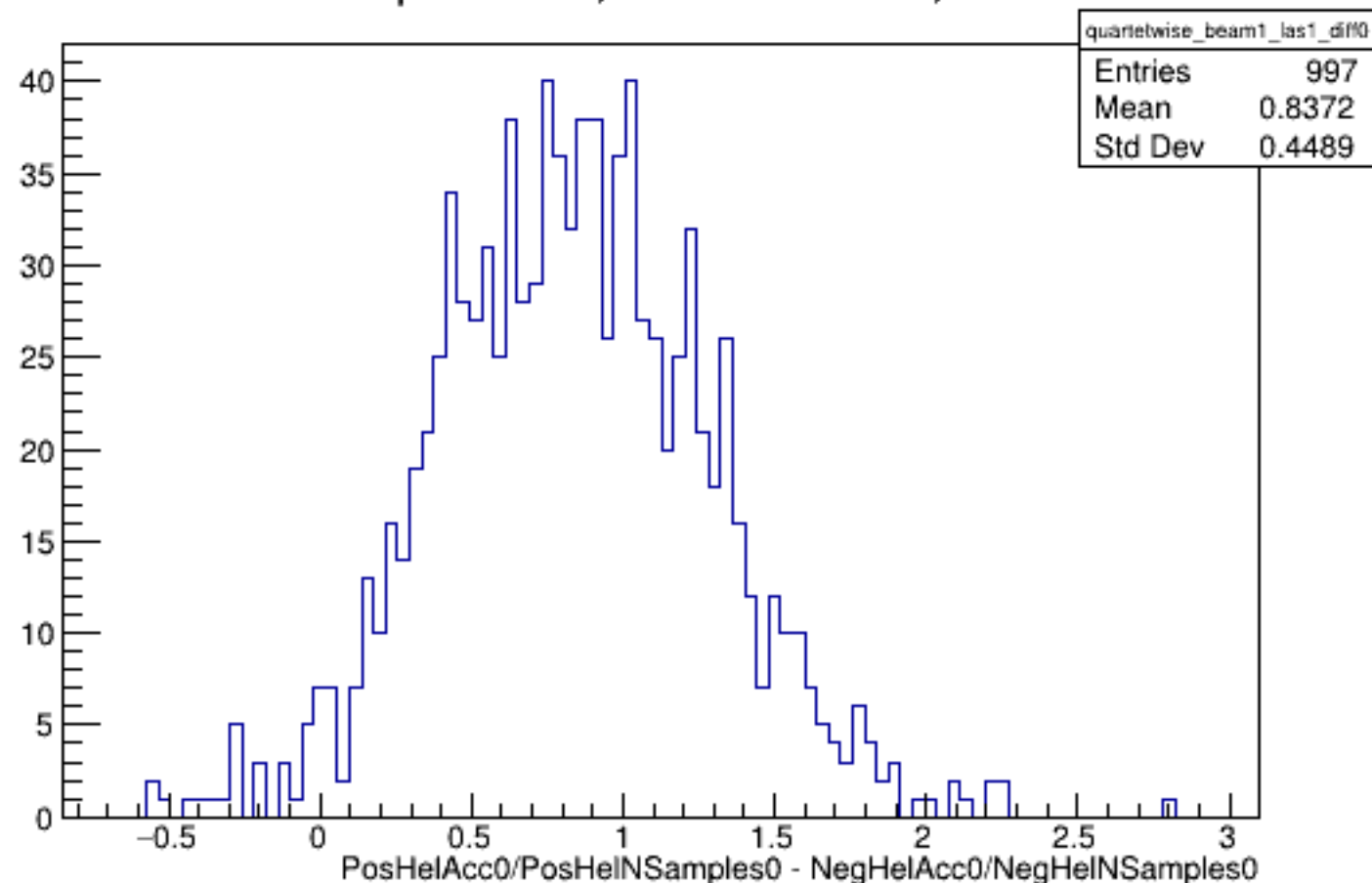
Run 5370 quartetwise, Diffs0: Beam ON, Laser ON
