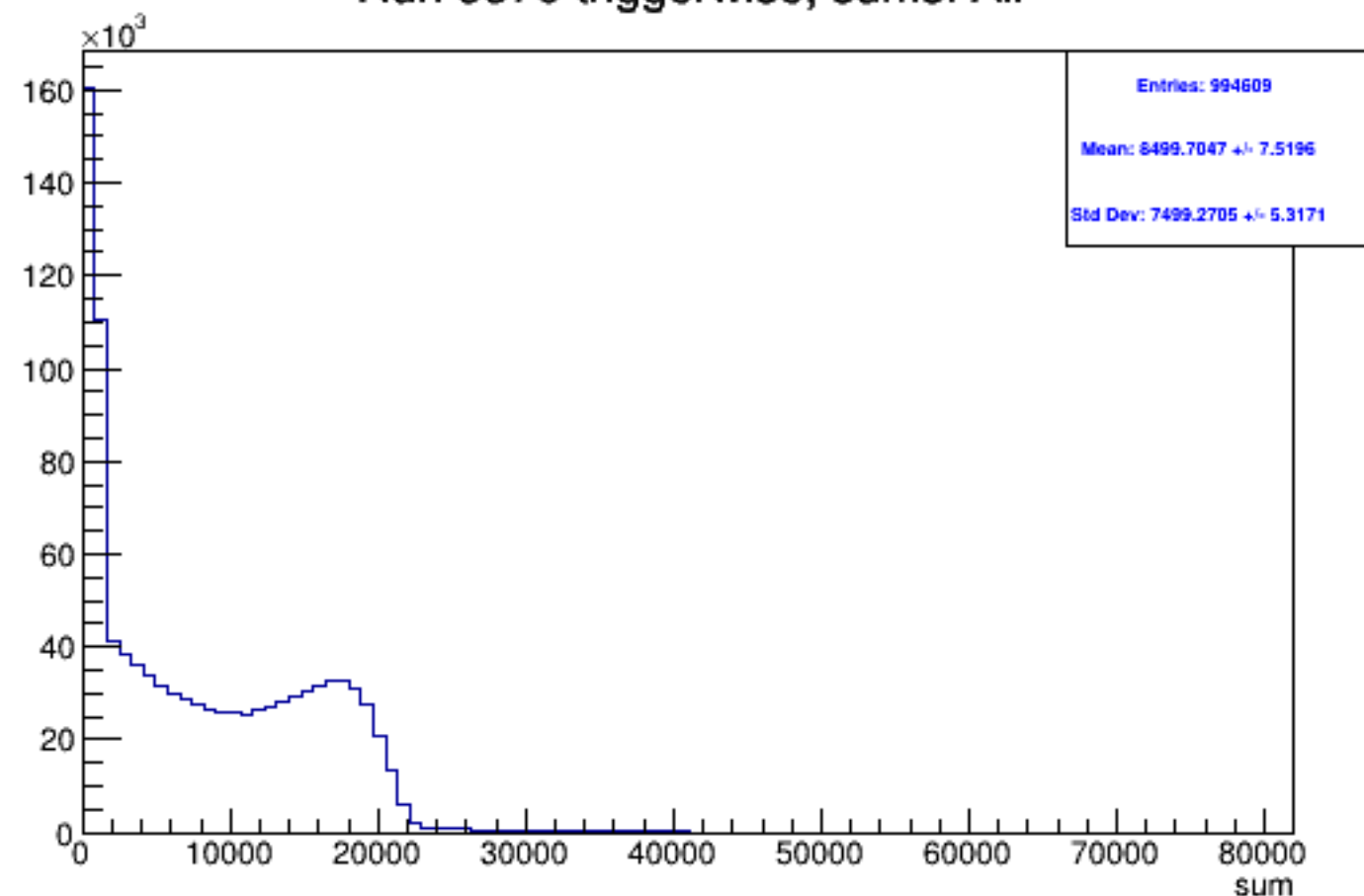
Run 5370 triggerwise, sums: All
