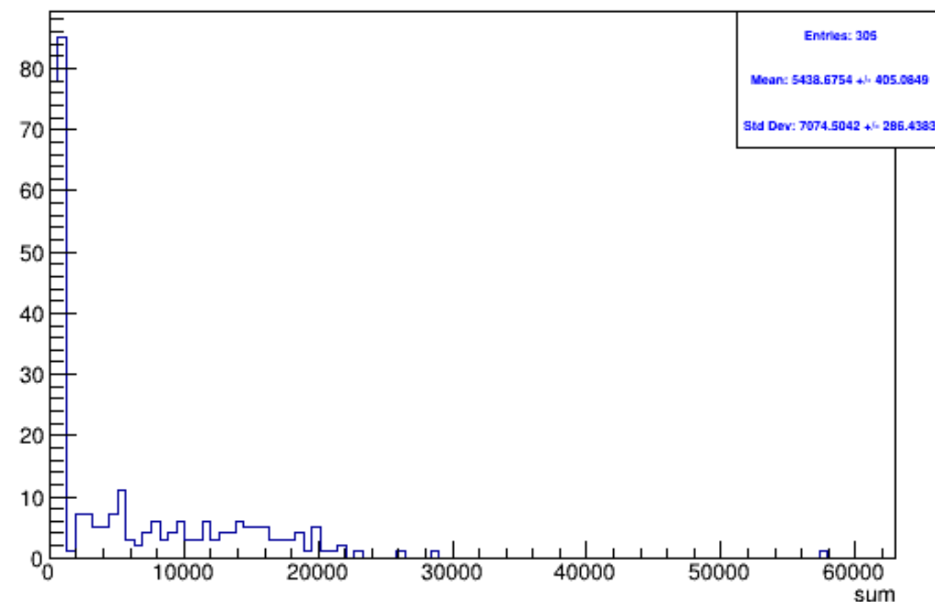
Run 5370 triggerwise, sums: Beam OFF
