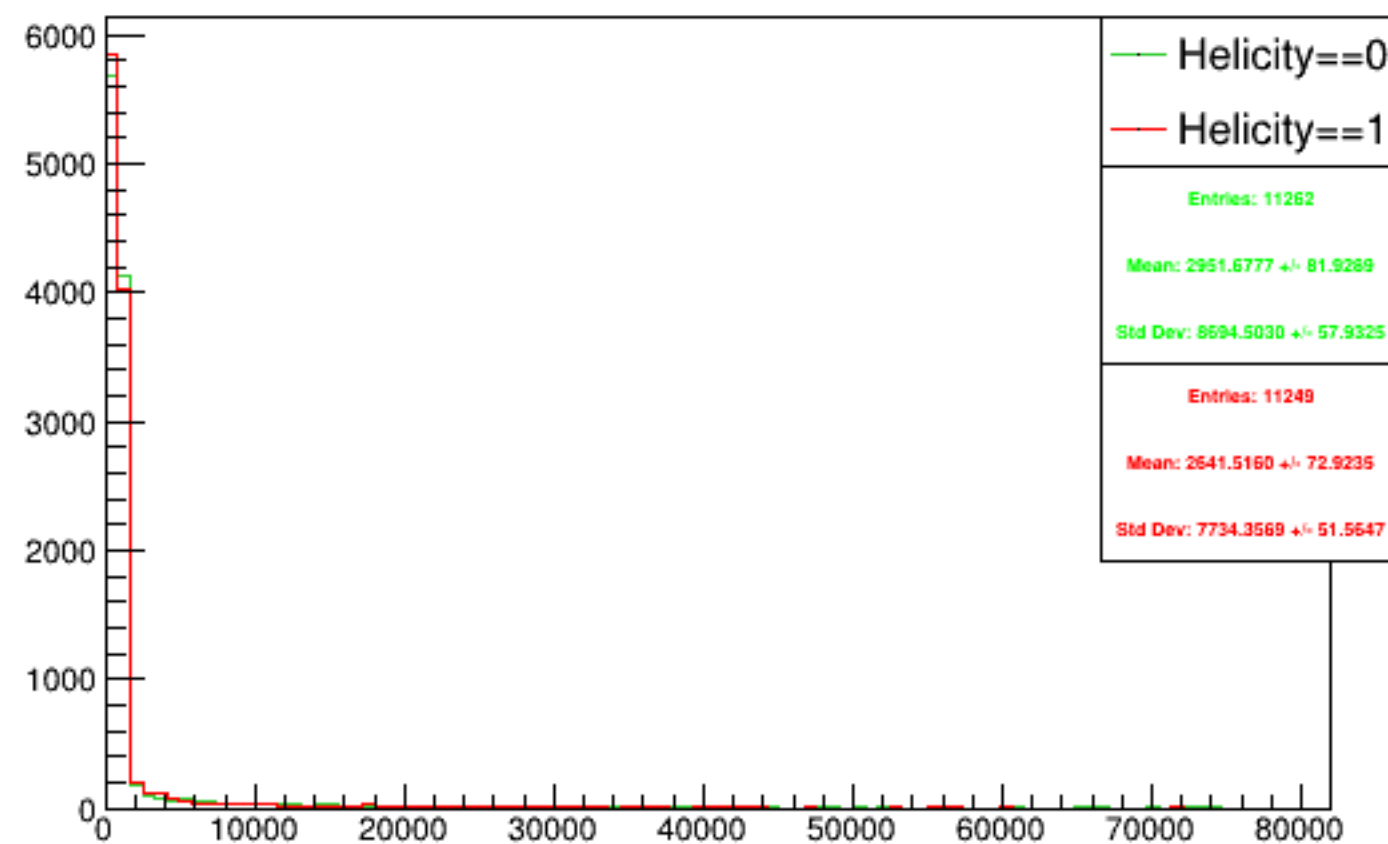
Run 5370 triggerwise, sums: Beam ON, Laser OFF
