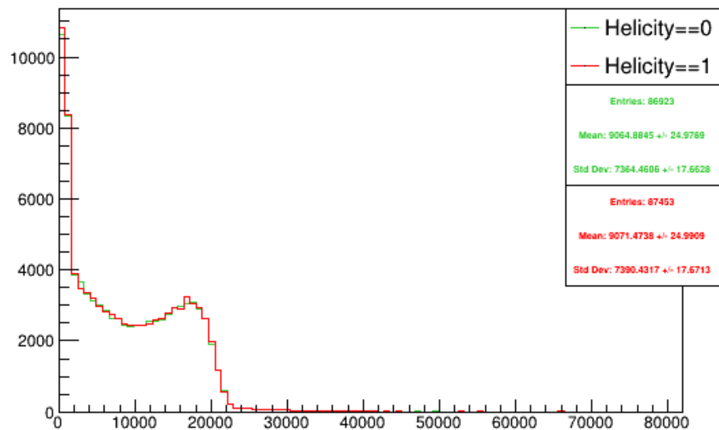
Run 5370 triggerwise, sums: Beam ON, Laser ON
