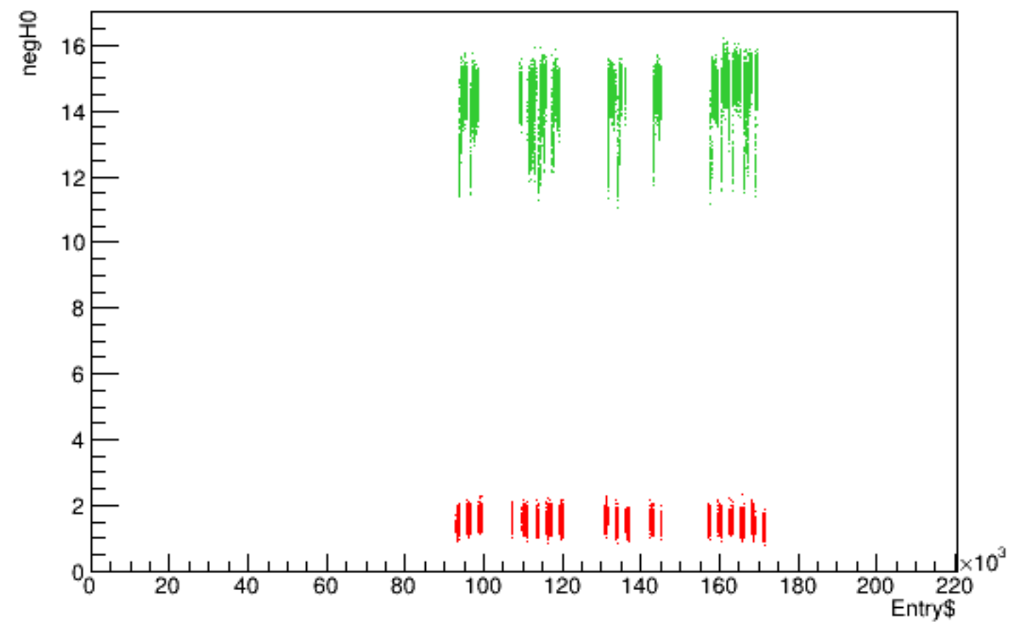
Run 5371 quartetwise, negH0 vs time
