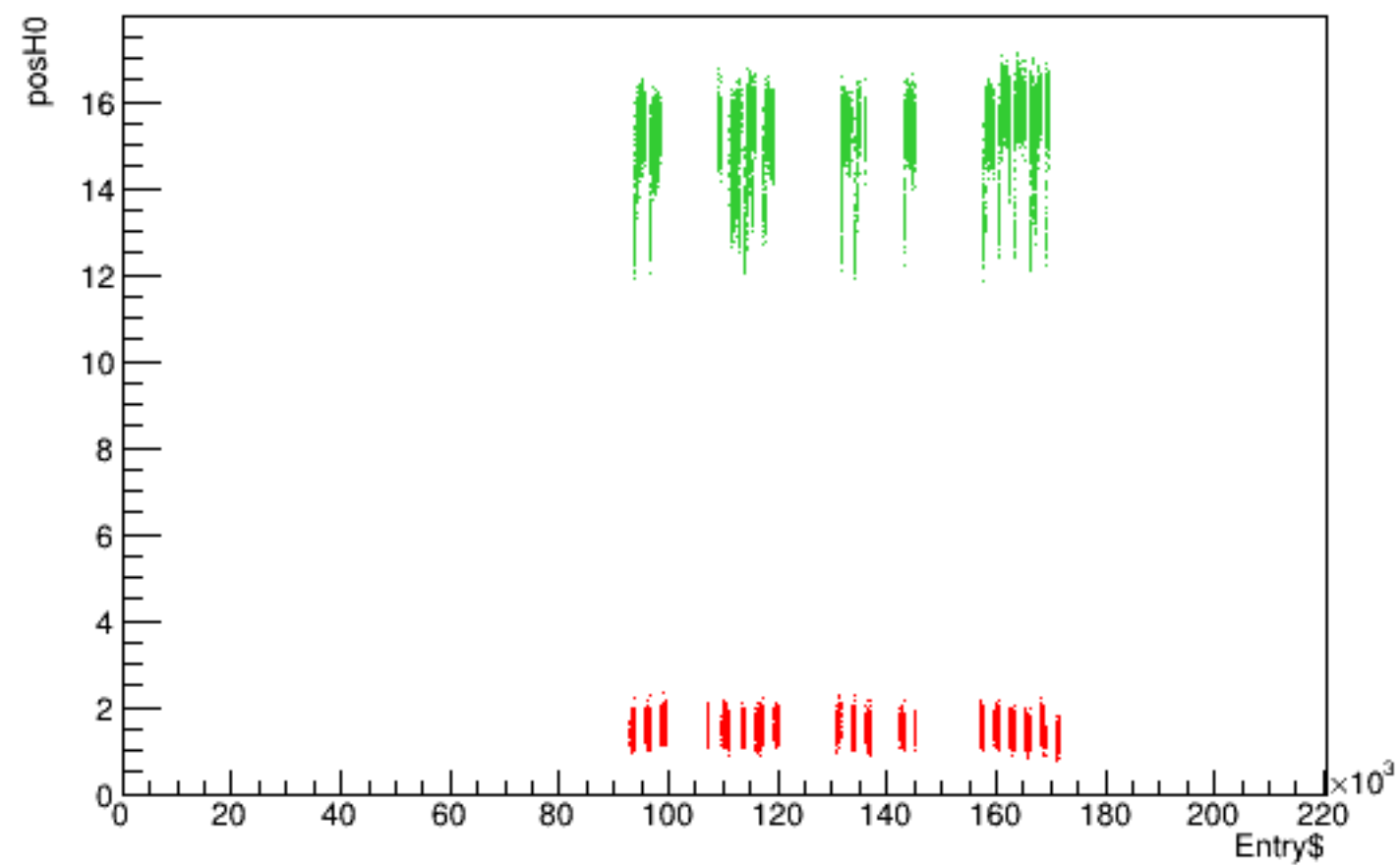
Run 5371 quartetwise, posH0 vs time
