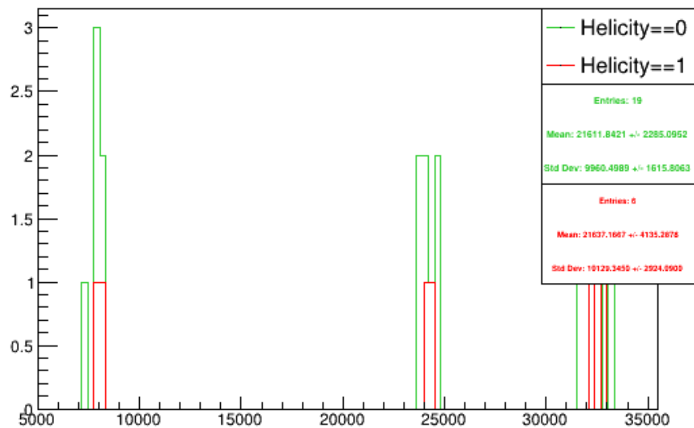
Run 5377 triggerwise, sums: Beam ON, Laser ON
