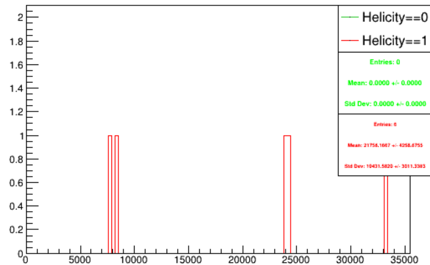
Run 5377 triggerwise, sums: Beam ON, Laser OFF
