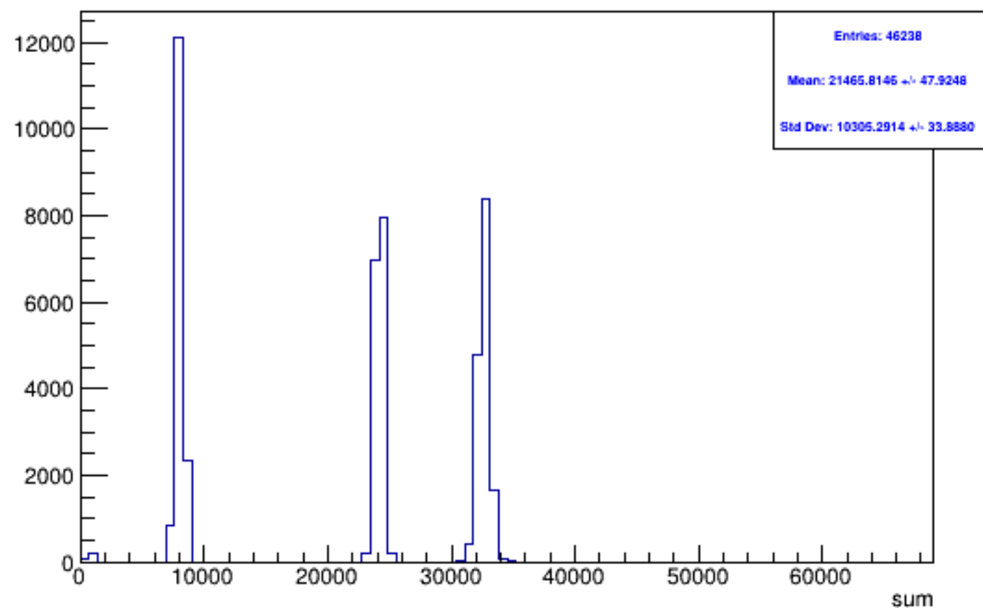
Run 5377 triggerwise, sums: All
