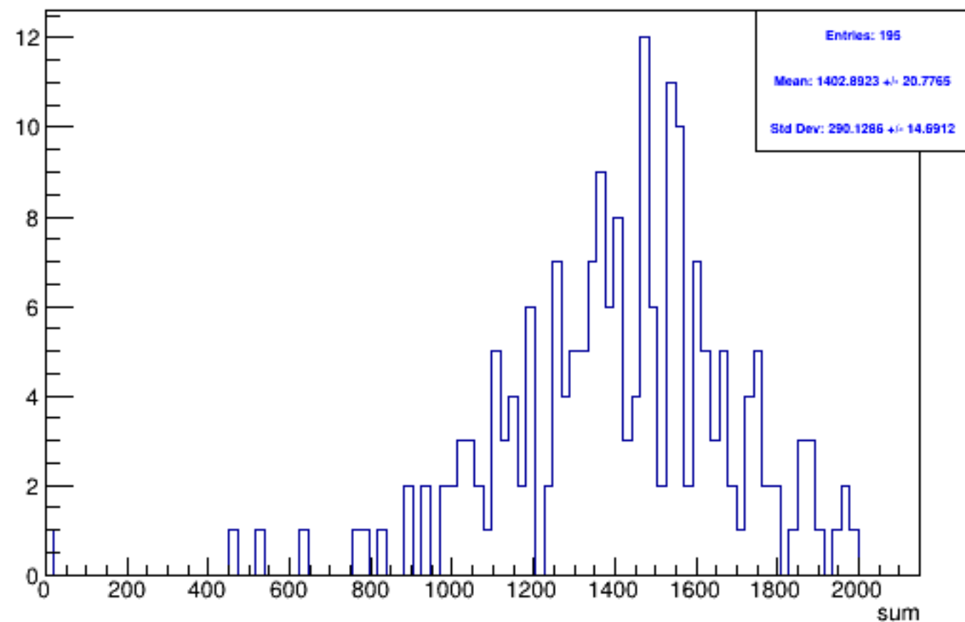
Run 5382 triggerwise, sums: Beam OFF
