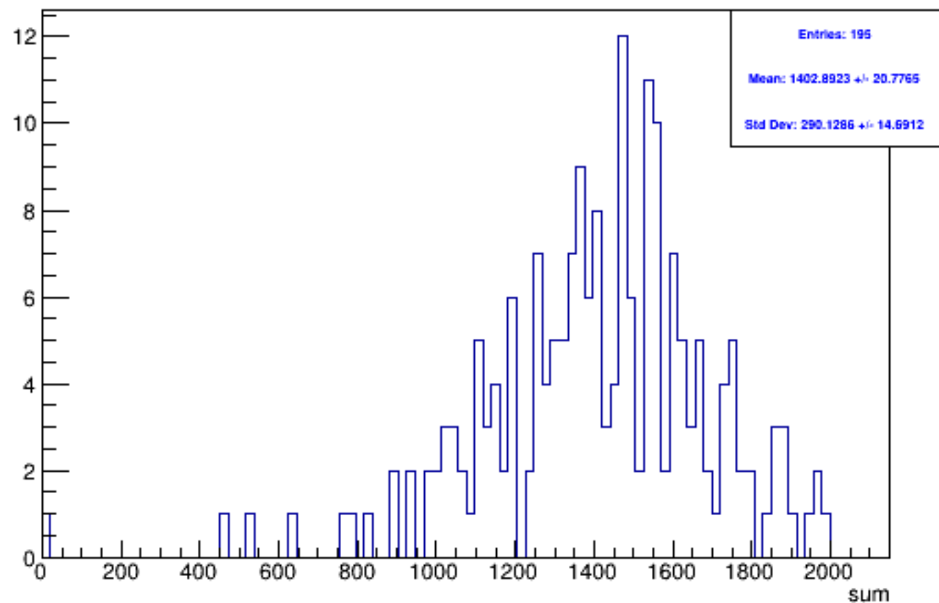
Run 5382 triggerwise, sums: All
