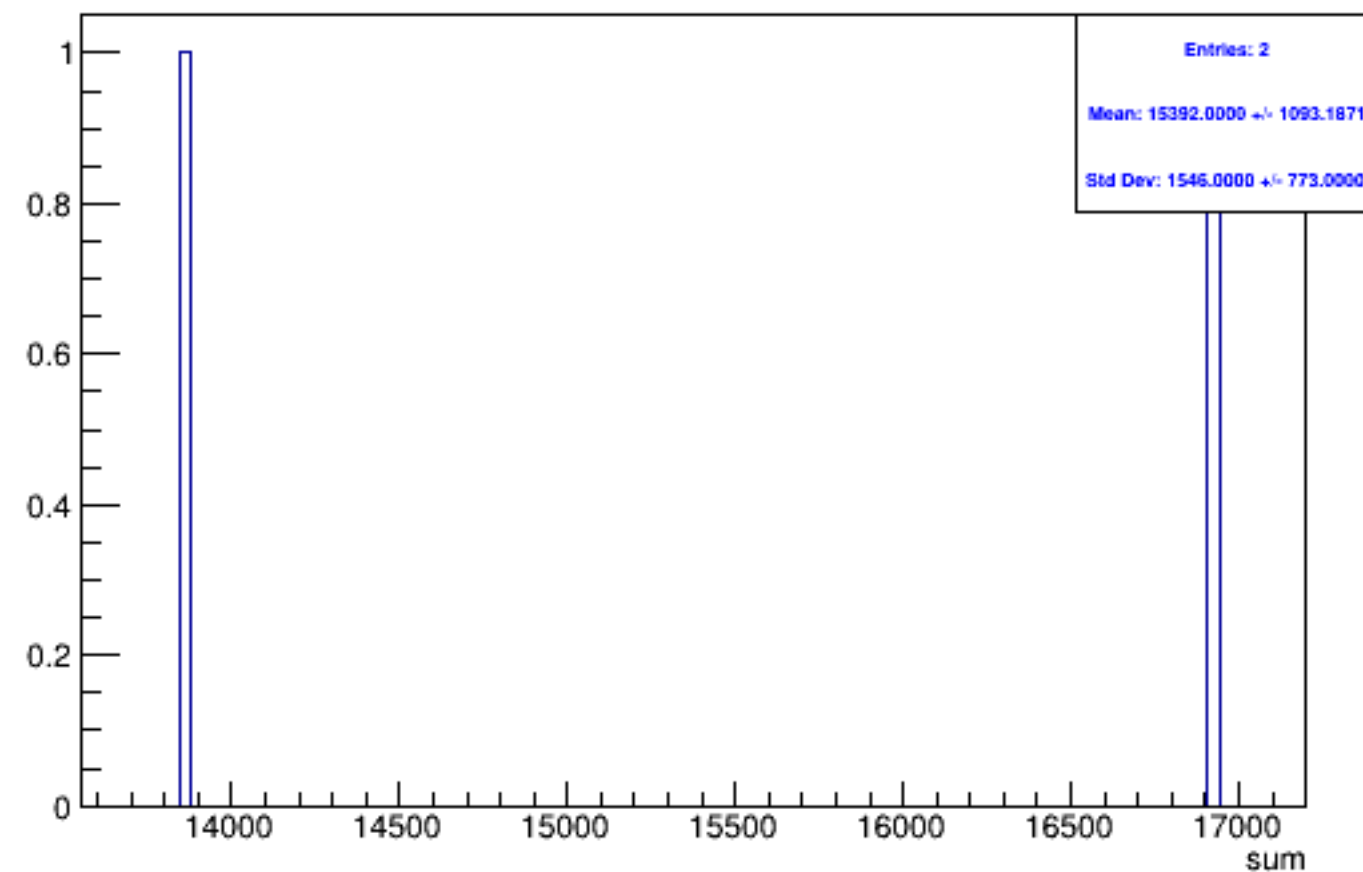
Run 5383 triggerwise, sums: Beam OFF
