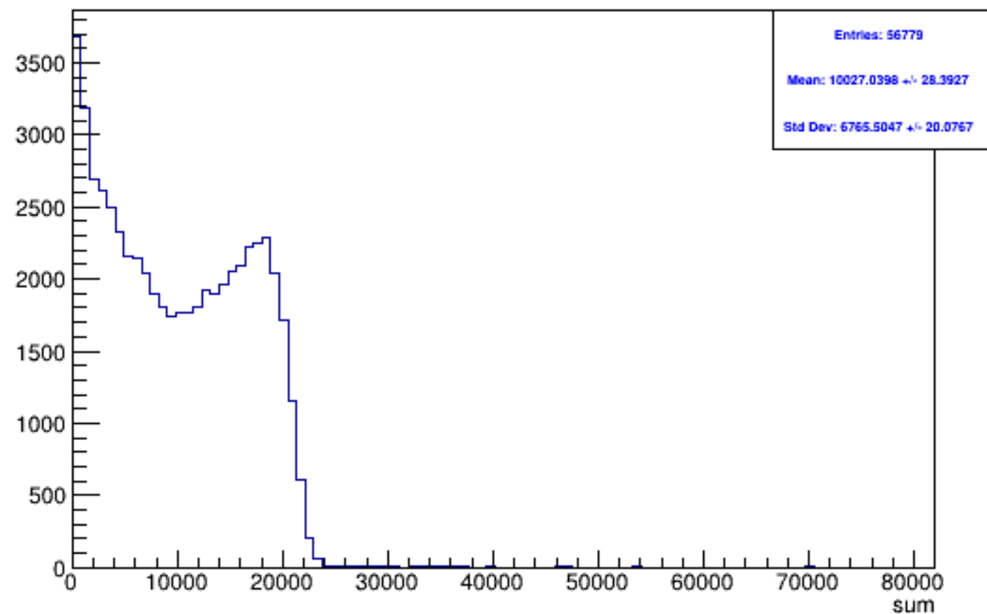
Run 5383 triggerwise, sums: All
