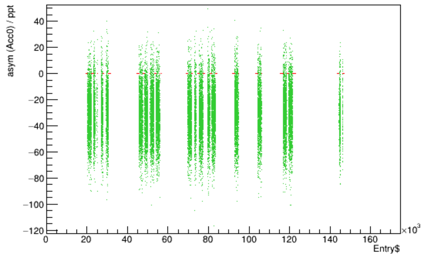
Run 5389 quartetwise, asym0sub vs time
