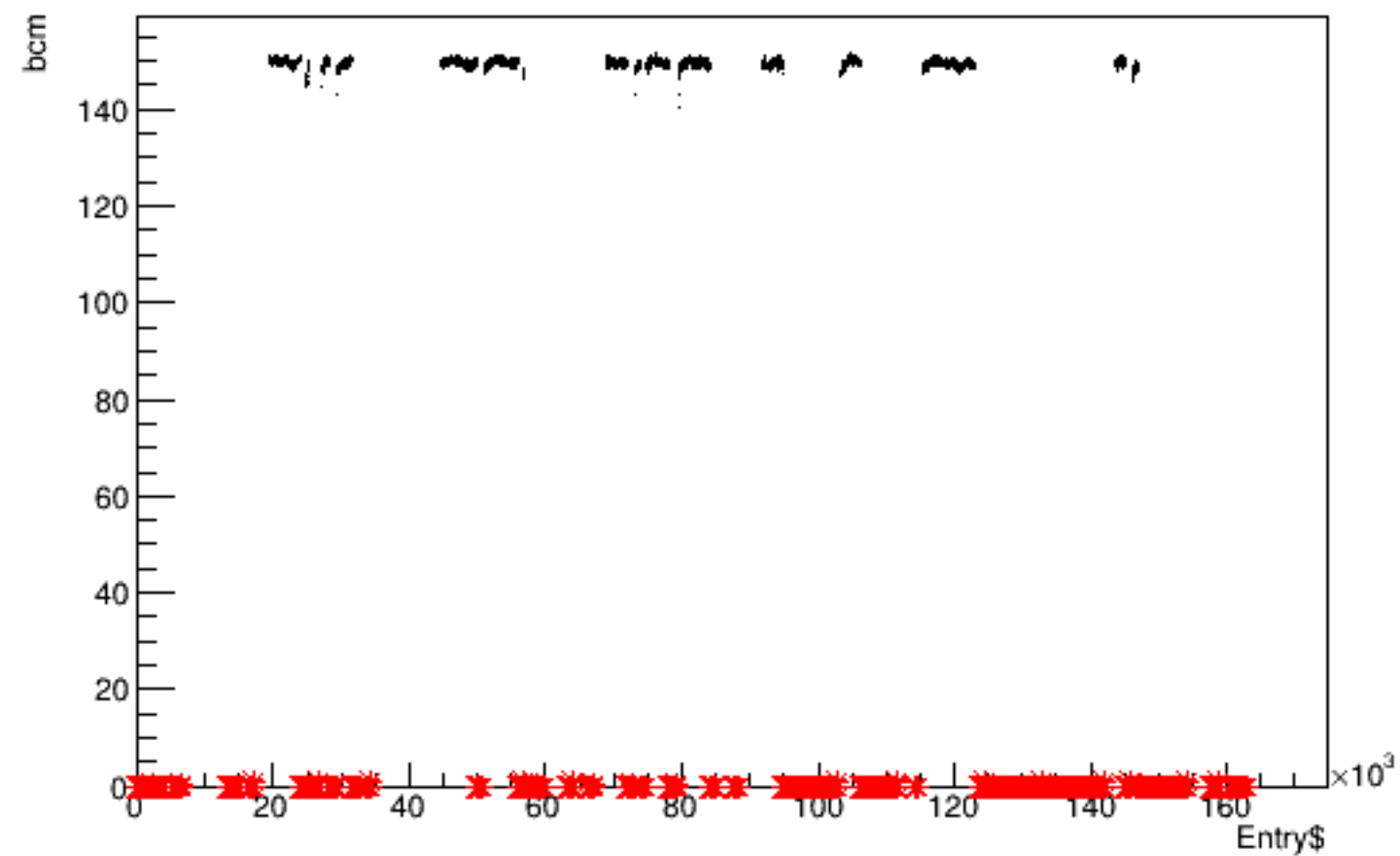
Run 5389 quartetwise, bcm vs time
