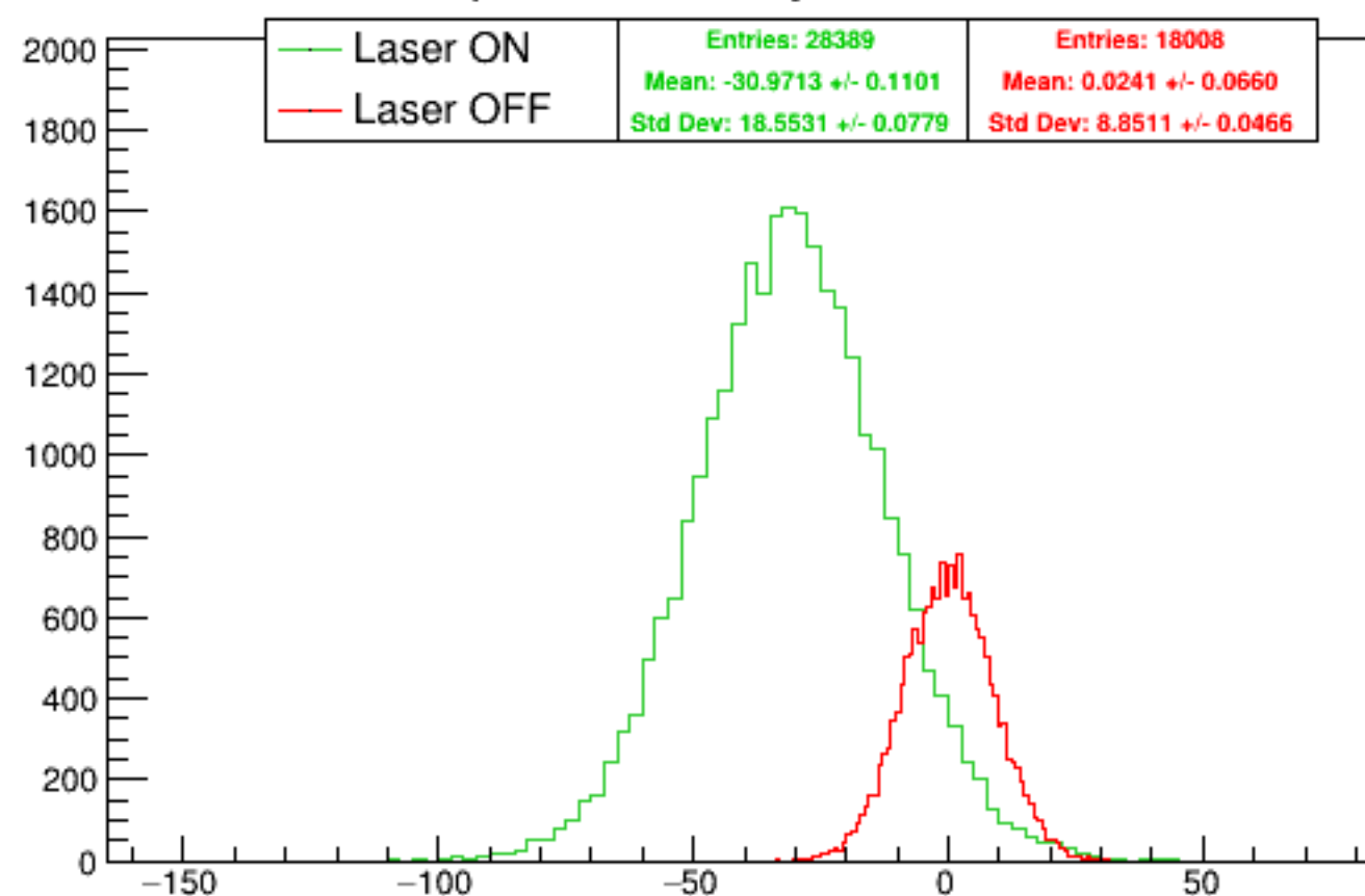
Run 5389 quartetwise, asym0sub: Beam ON
