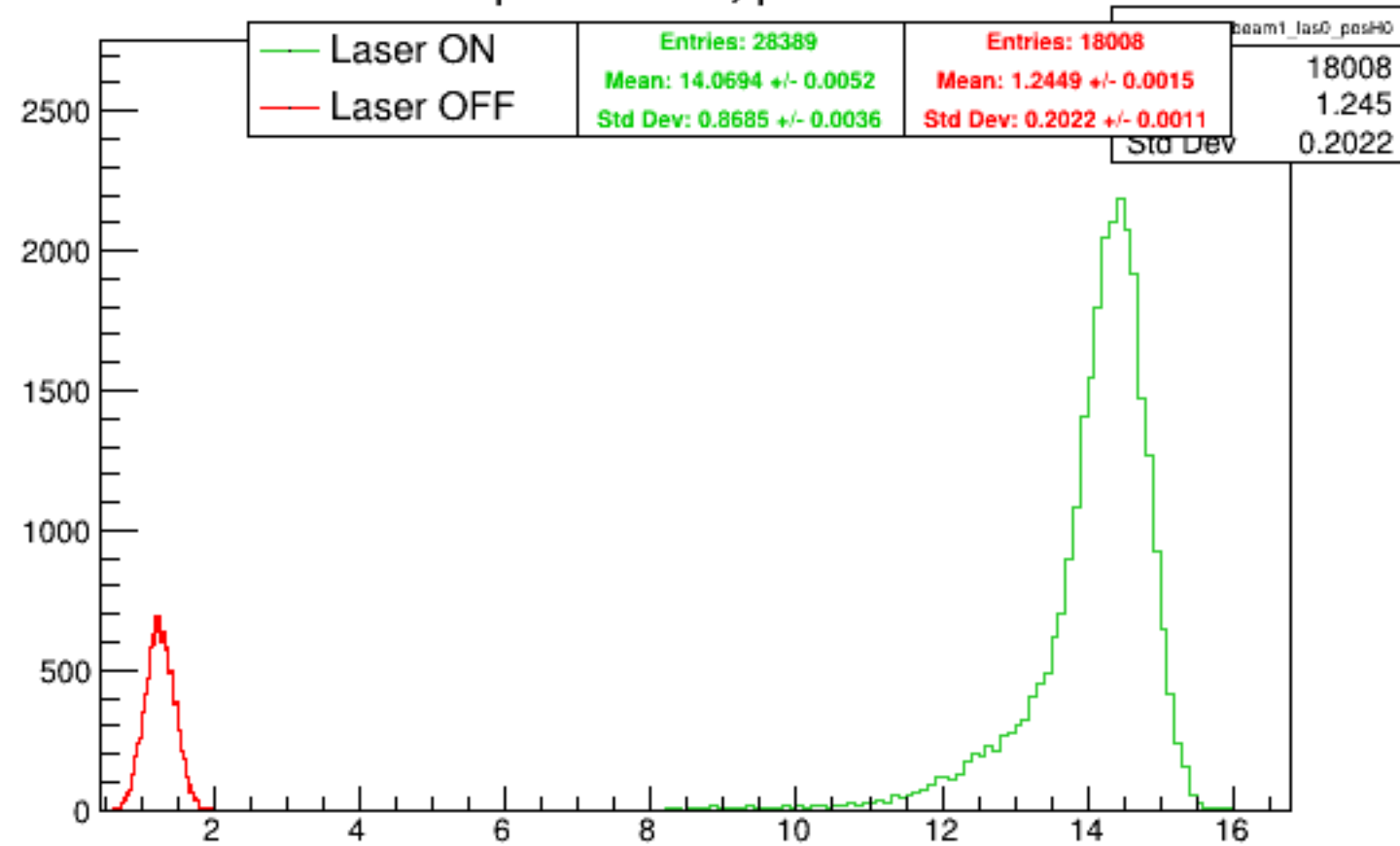
Run 5389 quartetwise, posH0: Beam ON
