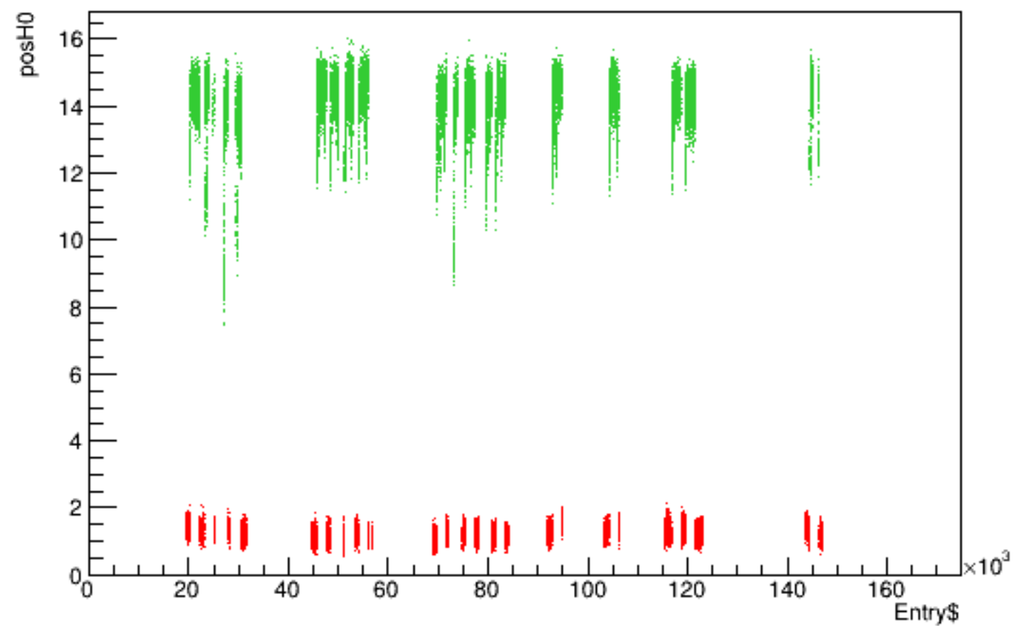
Run 5389 quartetwise, posH0 vs time
