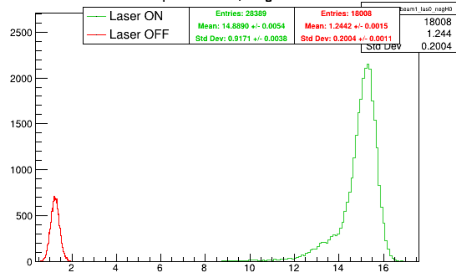
Run 5389 quartetwise, negH0: Beam ON
