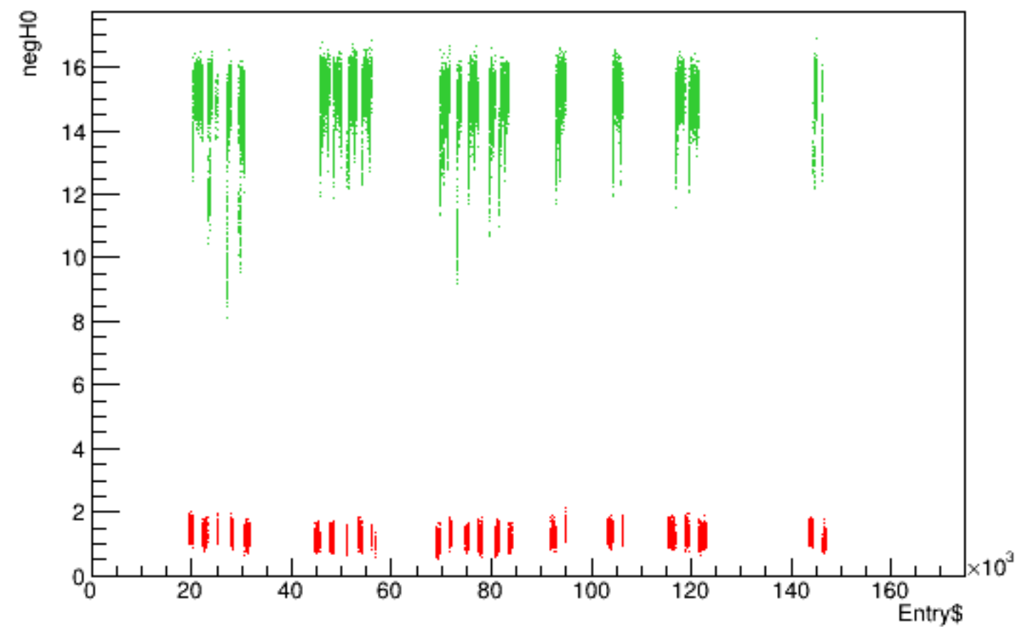
Run 5389 quartetwise, negH0 vs time
