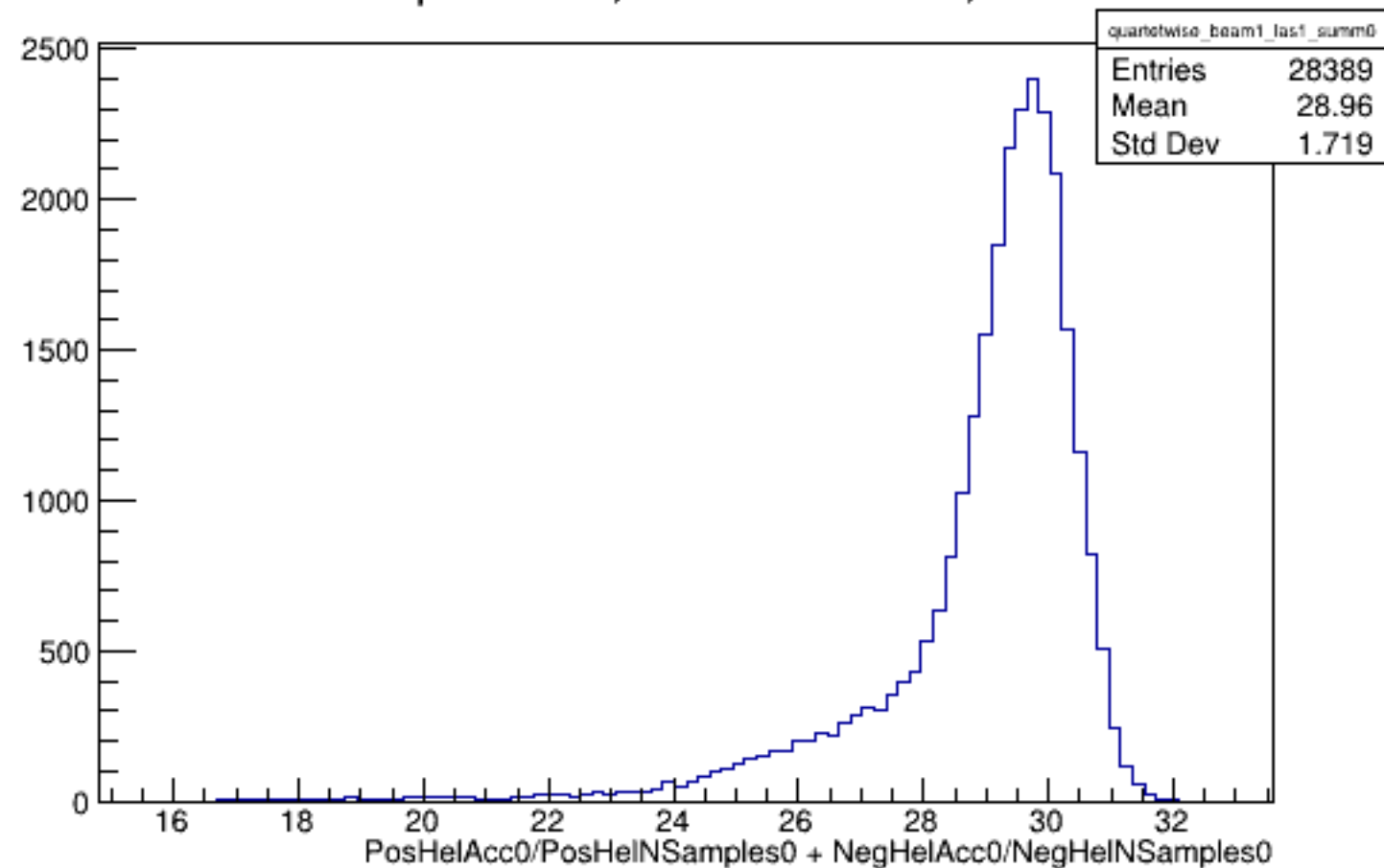
Run 5389 quartetwise, Sums0: Beam ON, Laser ON
