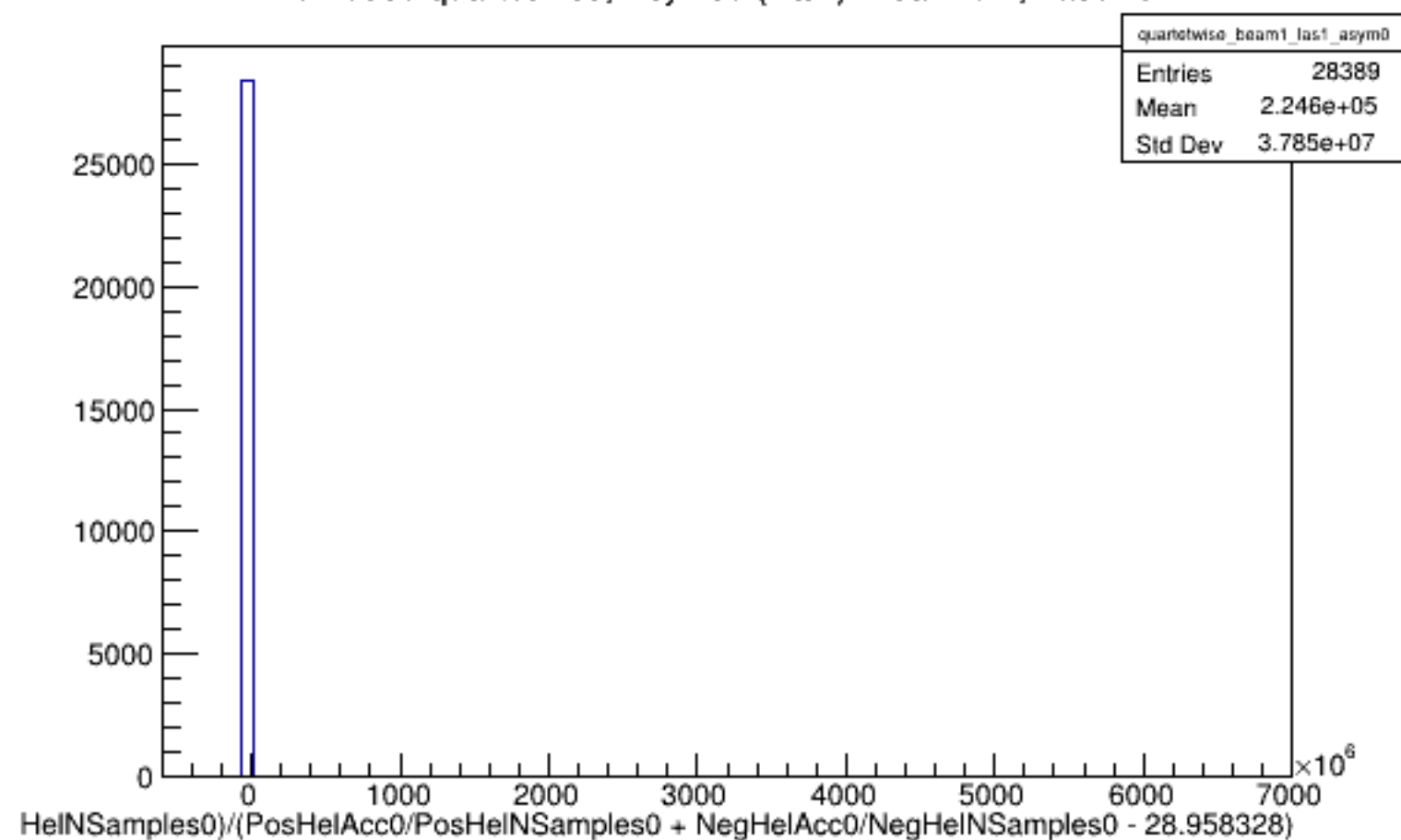
Run 5389 quartetwise, Asyms0 (Raw): Beam ON, Laser ON
