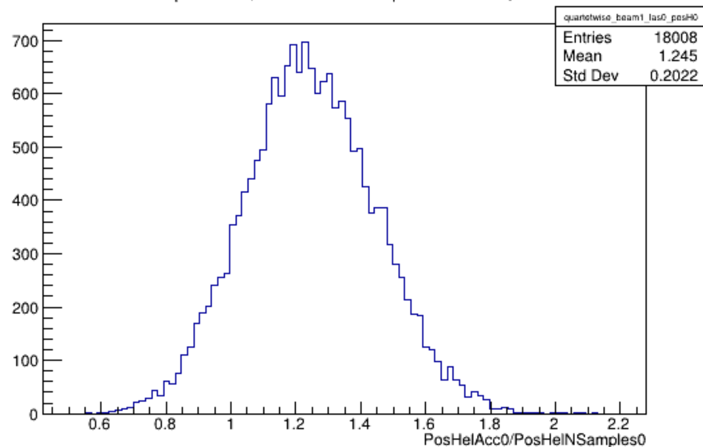
Run 5389 quartetwise, PosHelAcc0/NSamples0: Beam ON, Laser OFF
