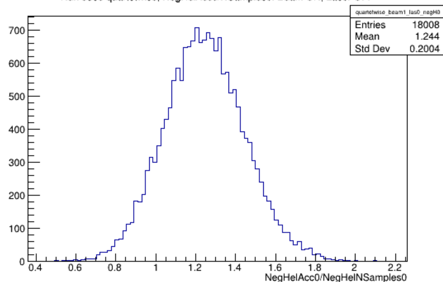
Run 5389 quartetwise, NegHelAcc0/NSamples0: Beam ON, Laser OFF
