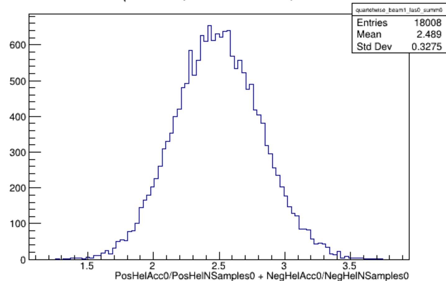
Run 5389 quartetwise, Sums0: Beam ON, Laser OFF
