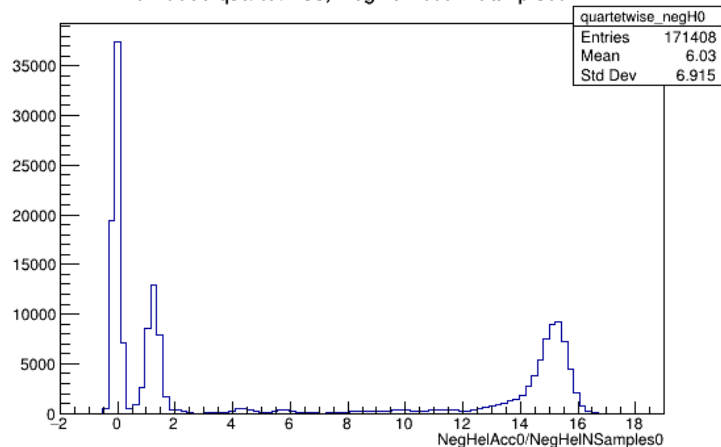
Run 5389 quartetwise, NegHelAcc0/NSamples0: All
