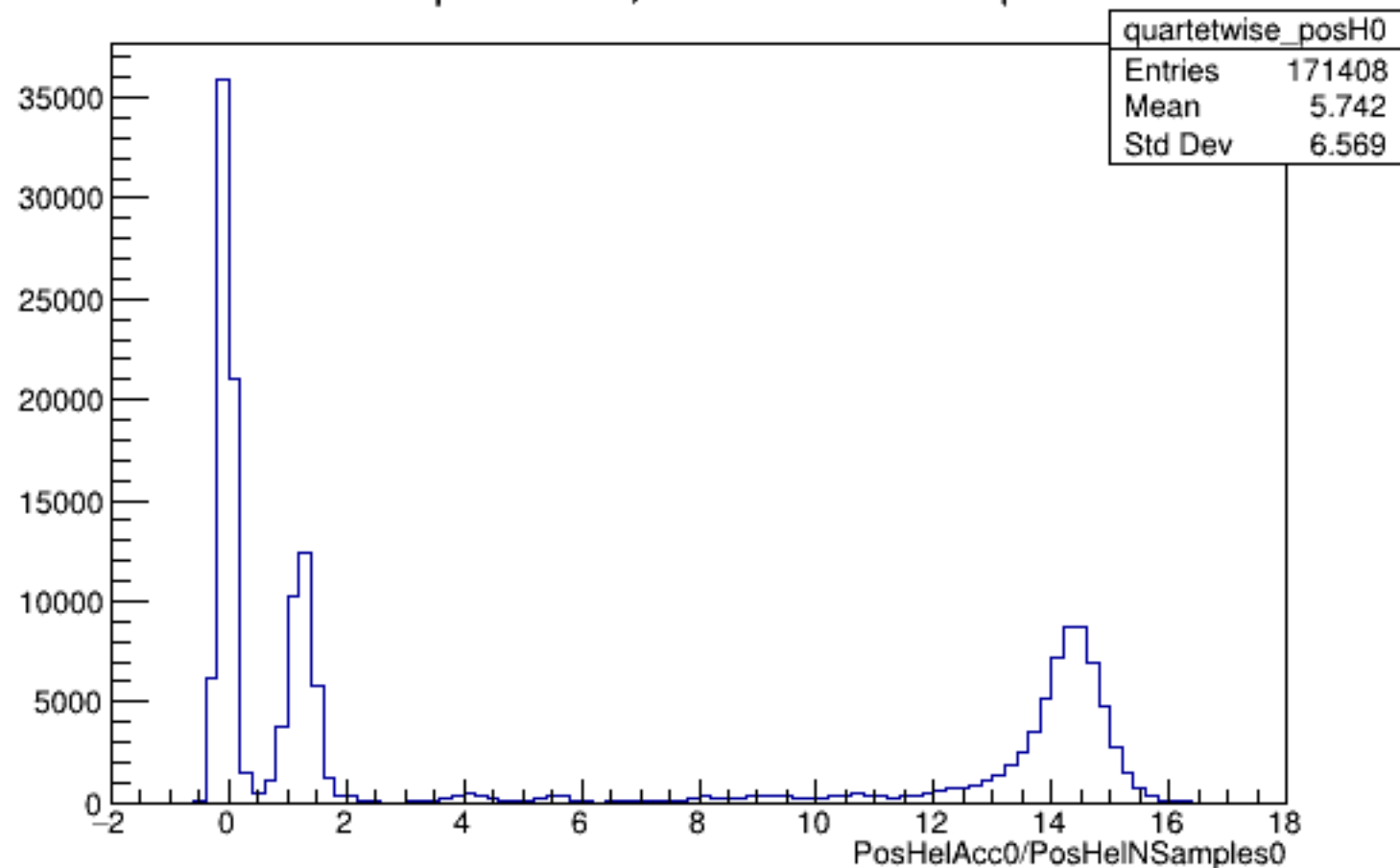
Run 5389 quartetwise, PosHelAcc0/NSamples0: All
