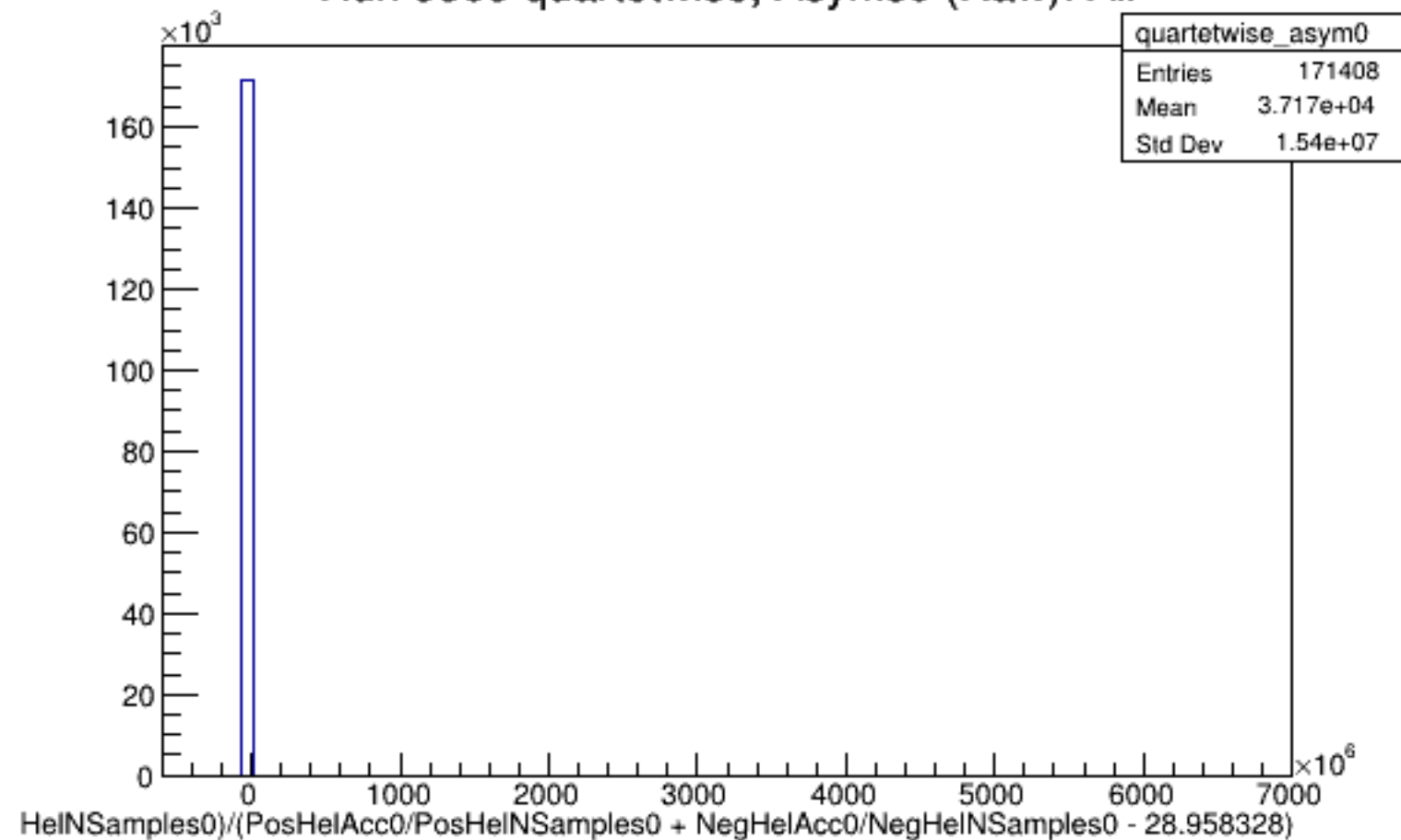
Run 5389 quartetwise, Asyms0 (Raw): All
