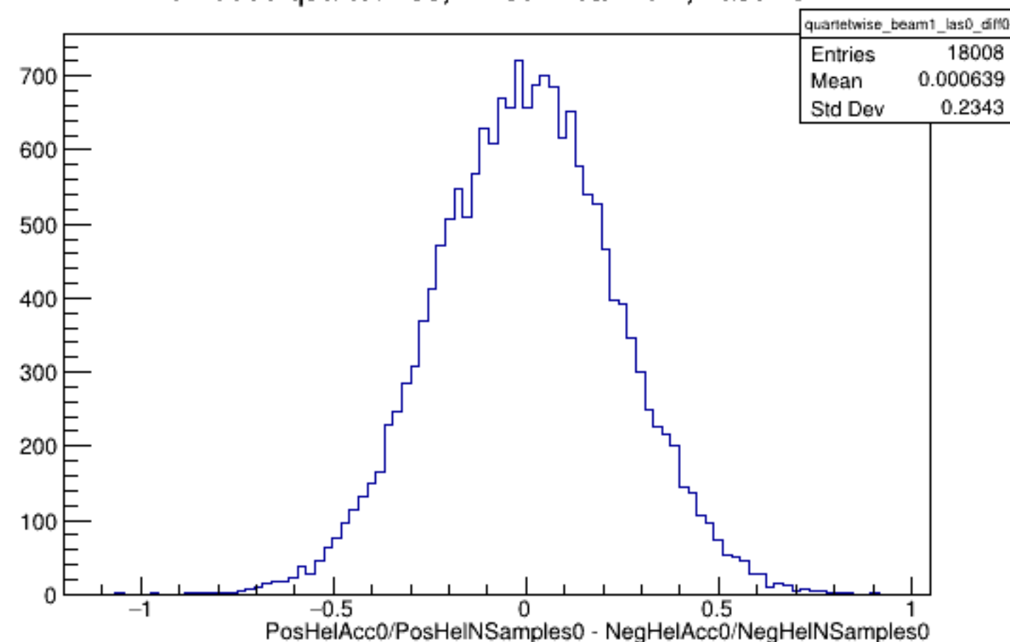
Run 5389 quartetwise, Diffs0: Beam ON, Laser OFF
