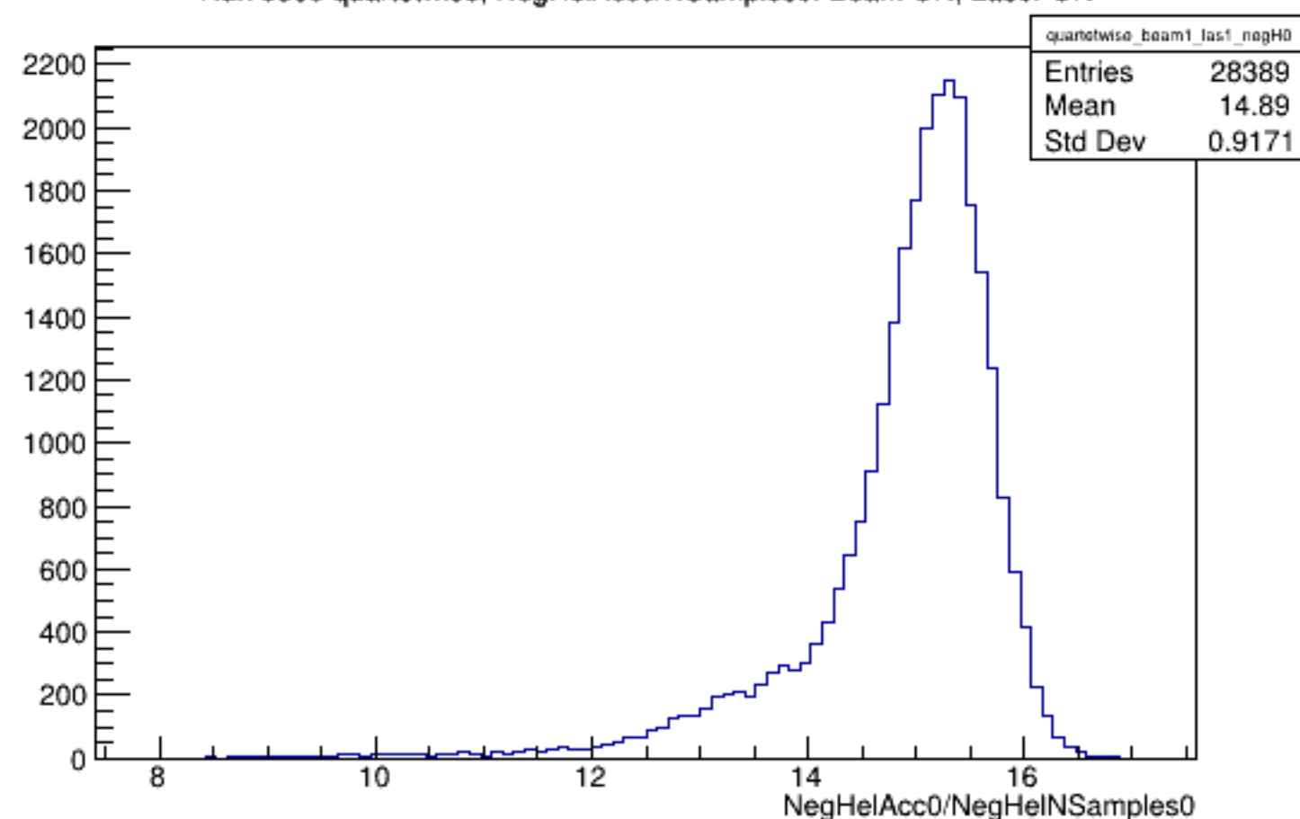
Run 5389 quartetwise, NegHelAcc0/NSamples0: Beam ON, Laser ON
