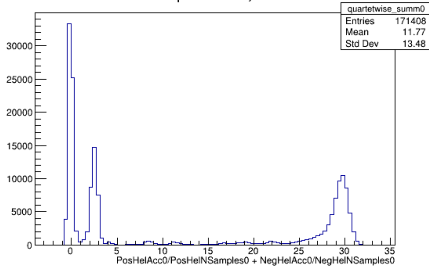
Run 5389 quartetwise, Sums0: All
