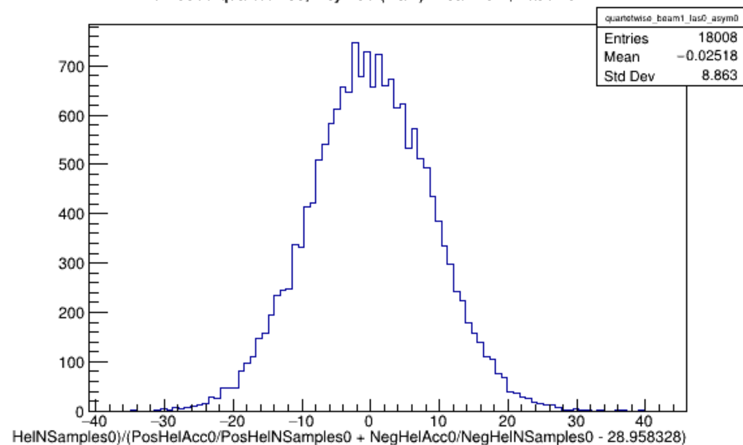
Run 5389 quartetwise, Asyms0 (Raw): Beam ON, Laser OFF
