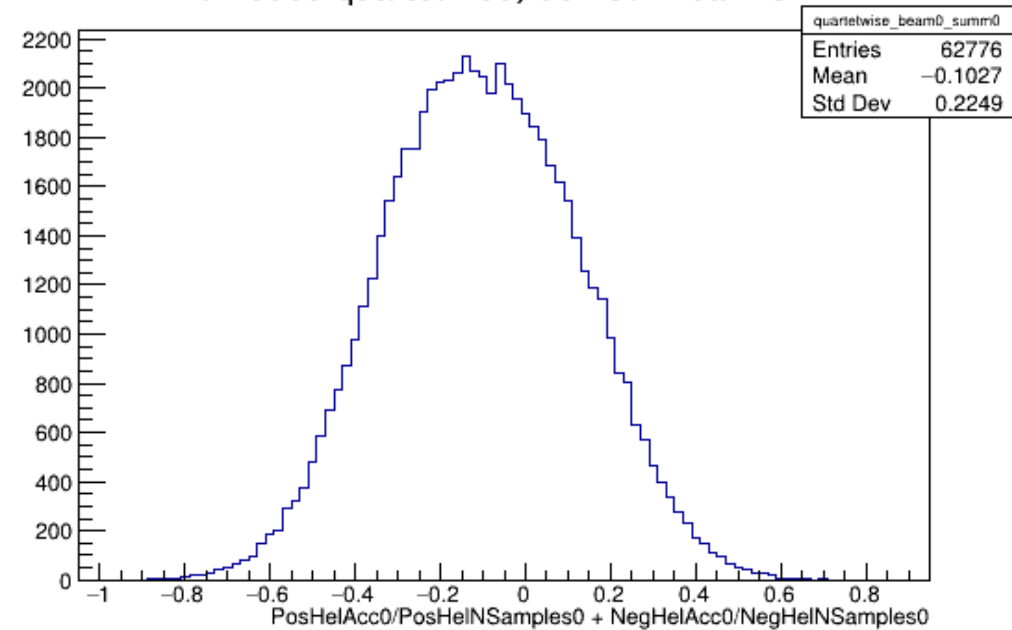
Run 5389 quartetwise, Sums0: Beam OFF
