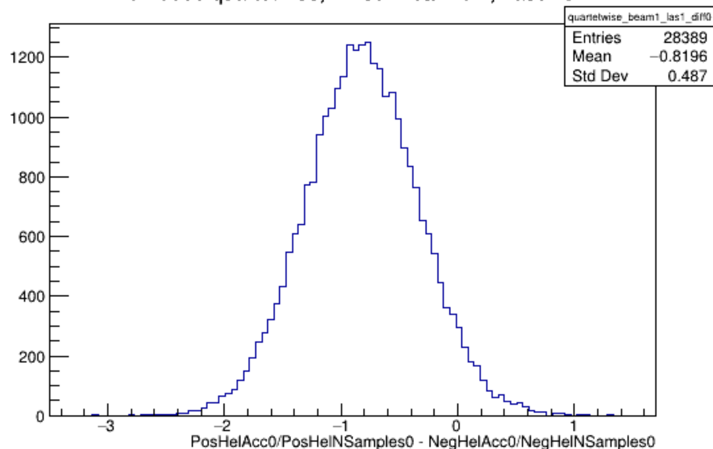
Run 5389 quartetwise, Diffs0: Beam ON, Laser ON
