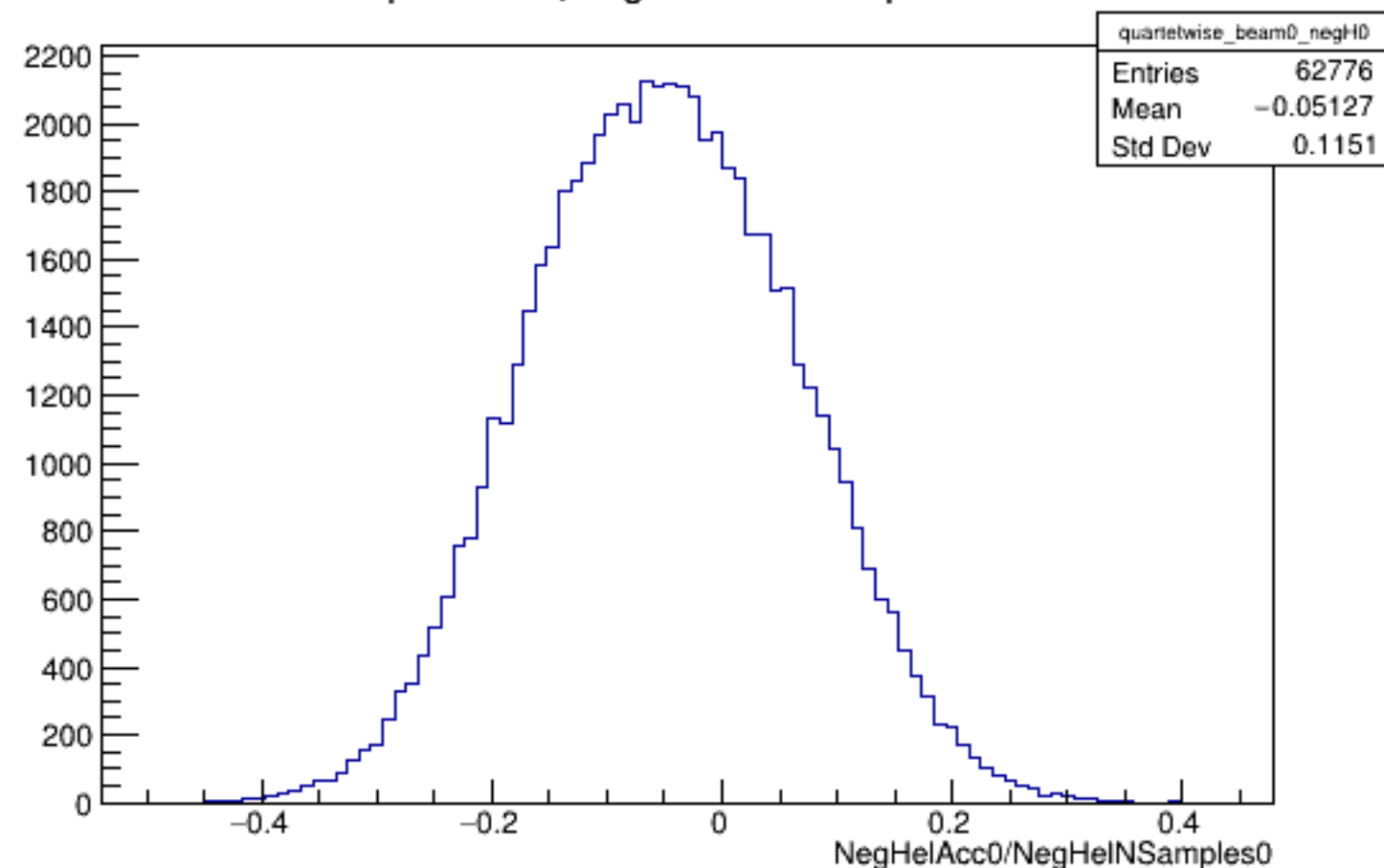
Run 5389 quartetwise, NegHelAcc0/NSamples0: Beam OFF
