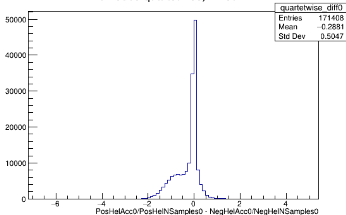
Run 5389 quartetwise, Diffs0: All
