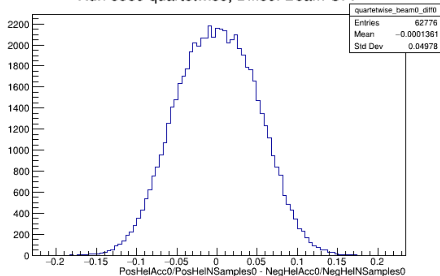
Run 5389 quartetwise, Diffs0: Beam OFF
