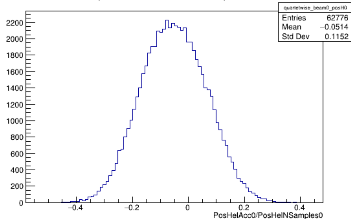
Run 5389 quartetwise, PosHelAcc0/NSamples0: Beam OFF
