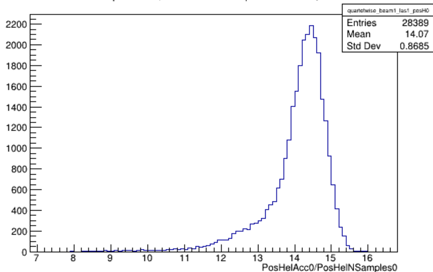
Run 5389 quartetwise, PosHelAcc0/NSamples0: Beam ON, Laser ON
