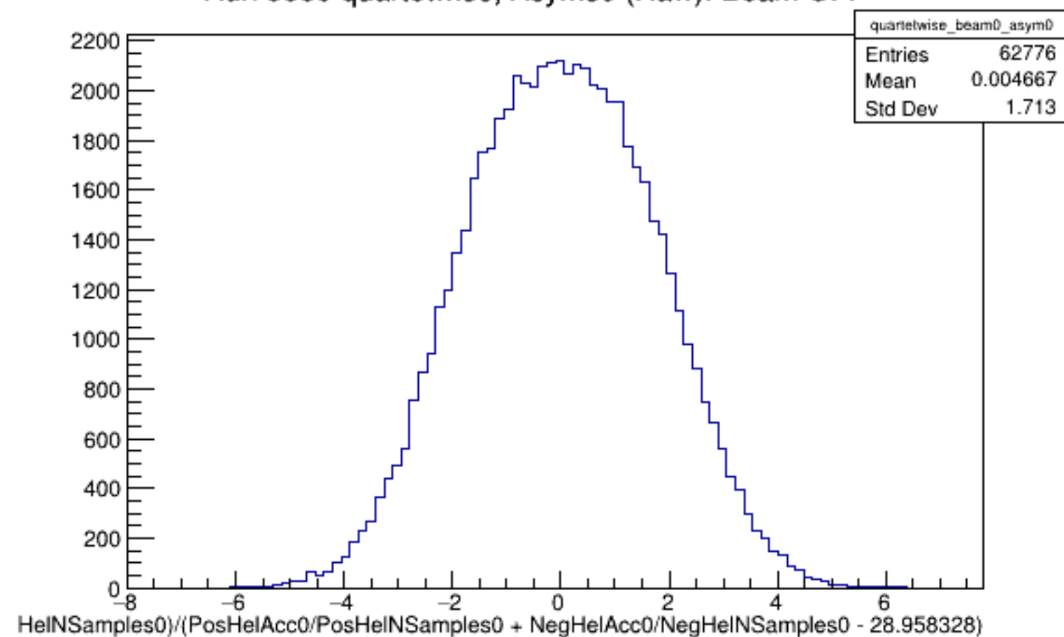
Run 5389 quartetwise, Asyms0 (Raw): Beam OFF
