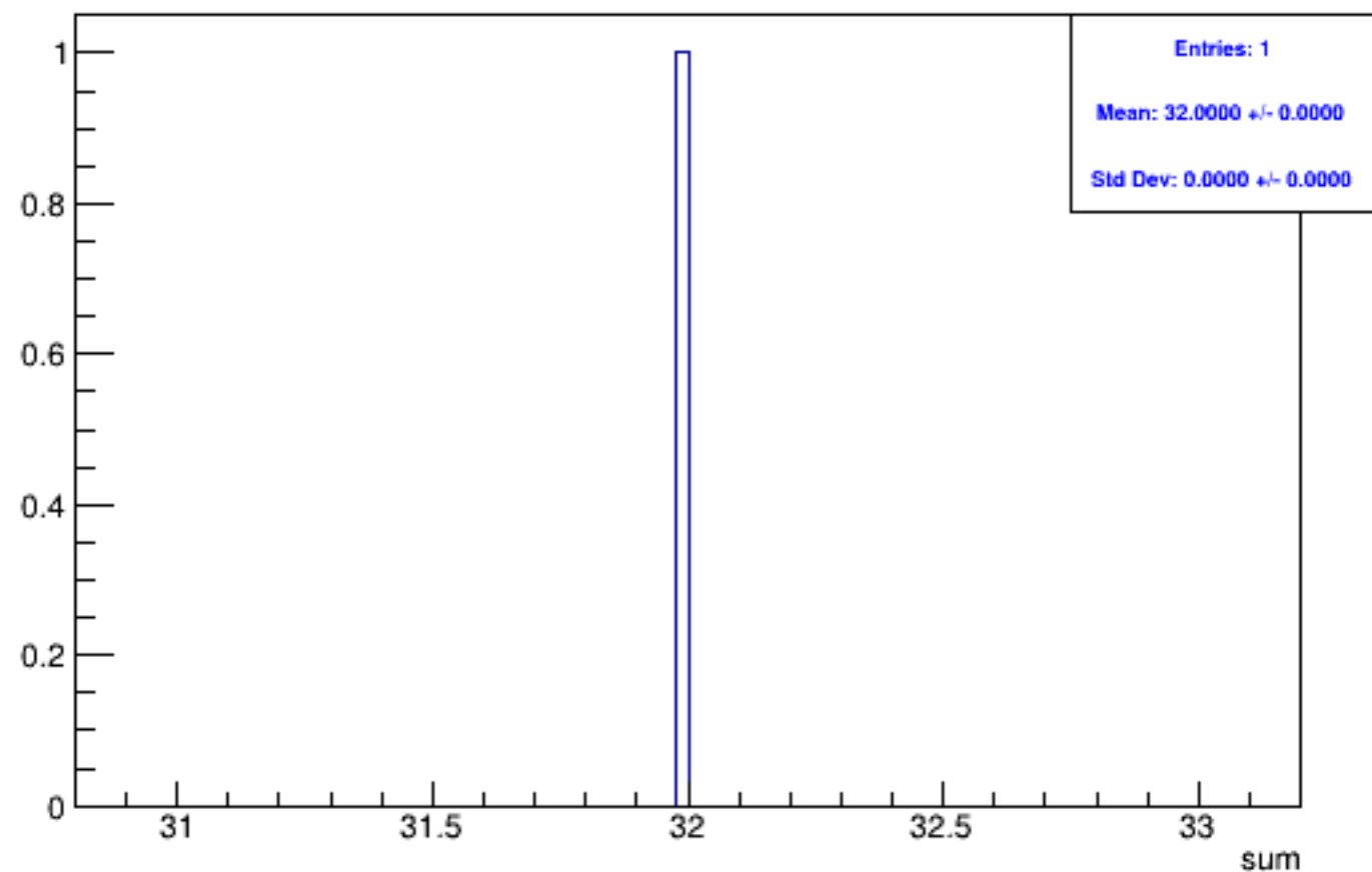
Run 5391 triggerwise, sums: All
