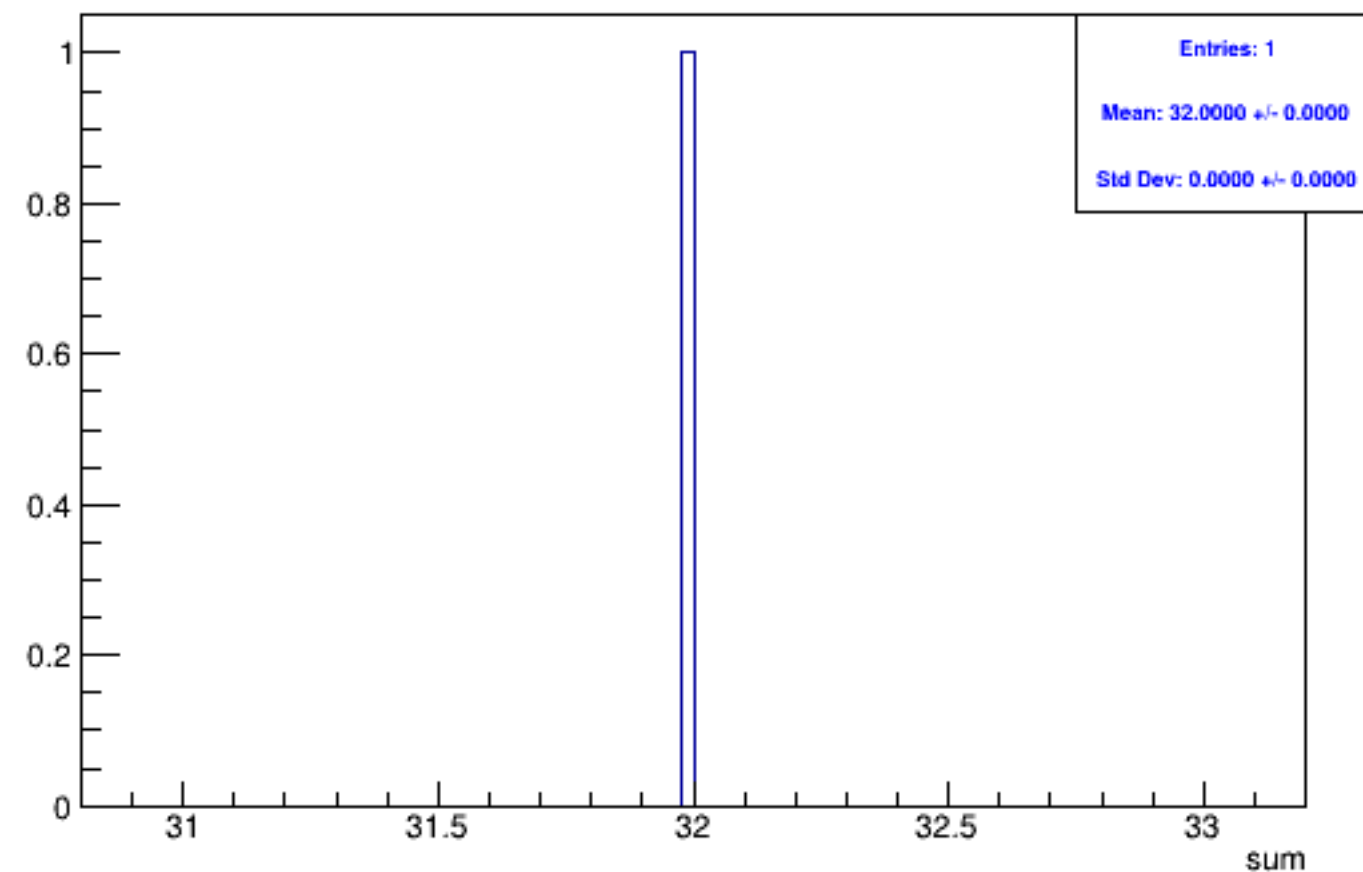
Run 5391 triggerwise, sums: Beam OFF
