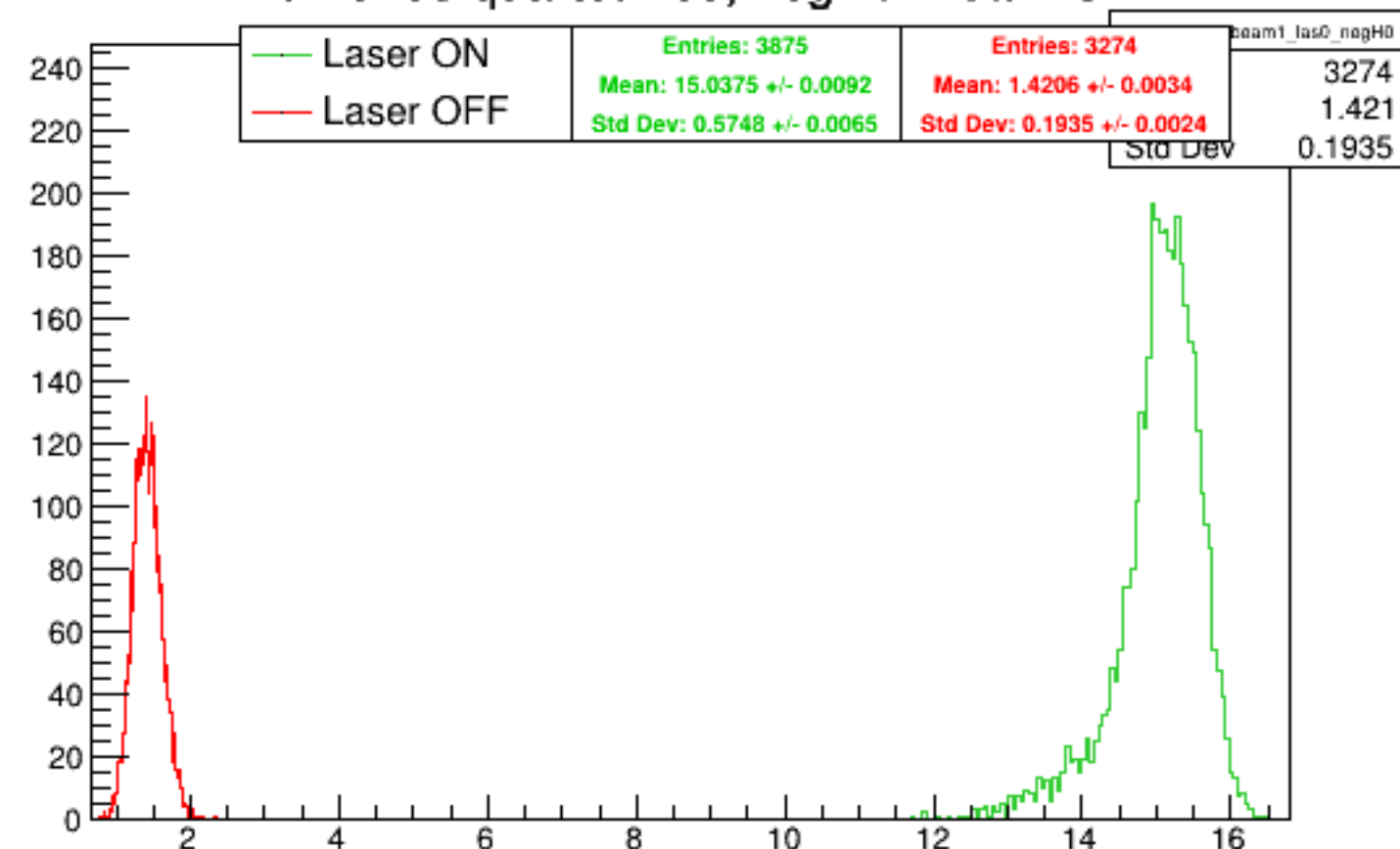
Run 5403 quartetwise, negH0: Beam ON
