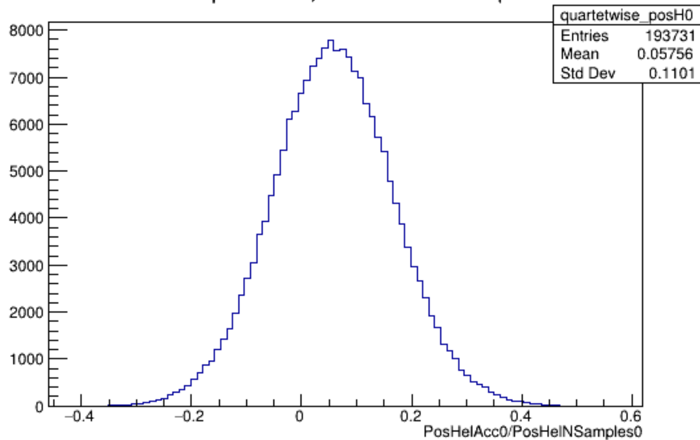
Run 5410 quartetwise, PosHelAcc0/NSamples0: All
