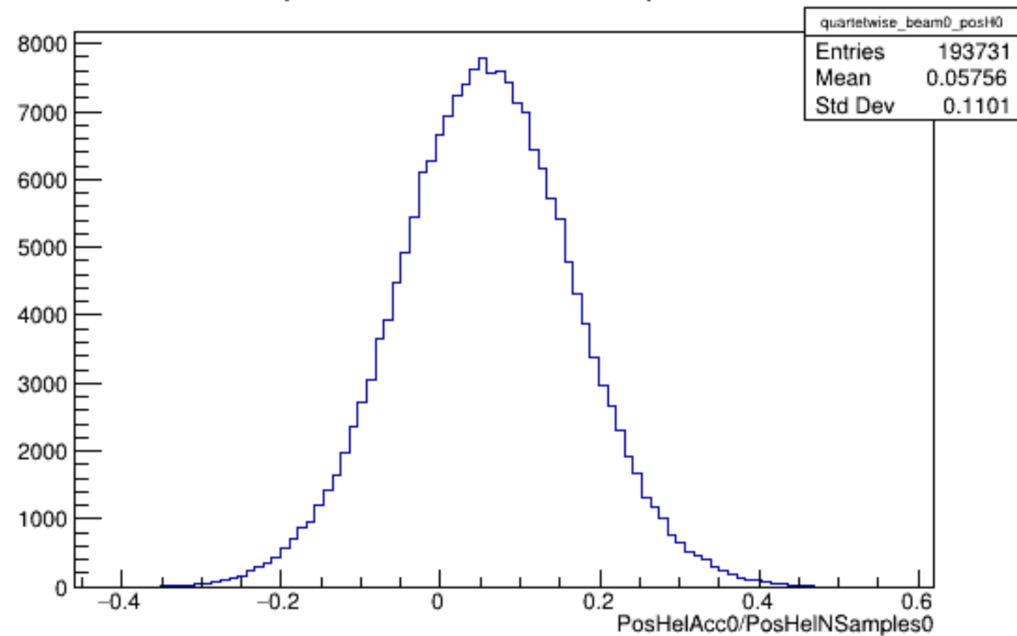
Run 5410 quartetwise, PosHelAcc0/NSamples0: Beam OFF
