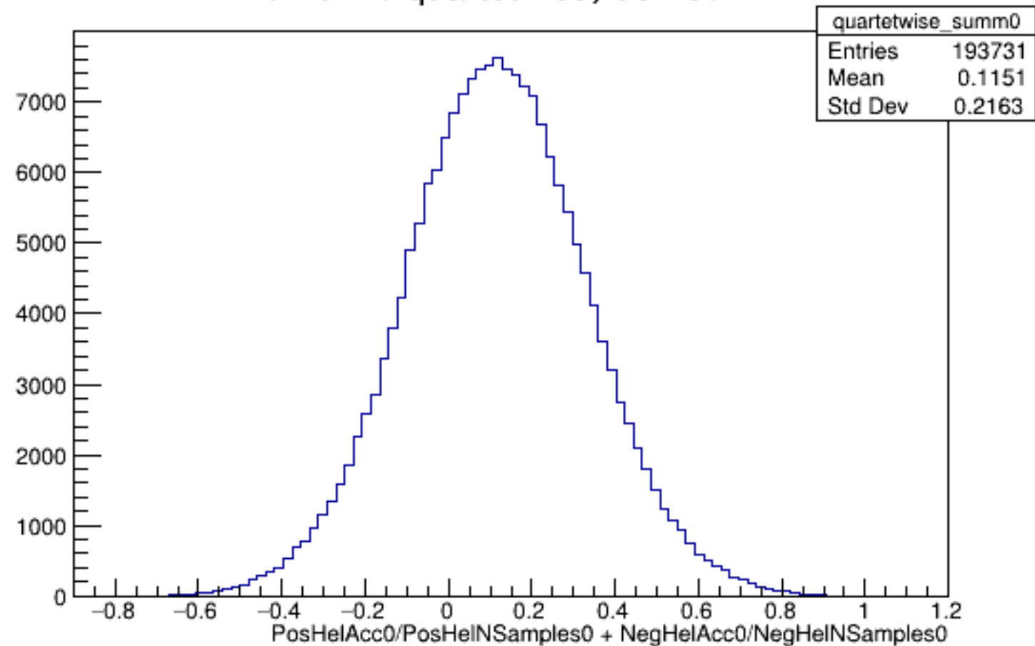
Run 5410 quartetwise, Sums0: All
