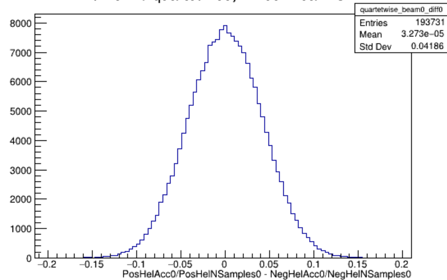
Run 5410 quartetwise, Diffs0: Beam OFF
