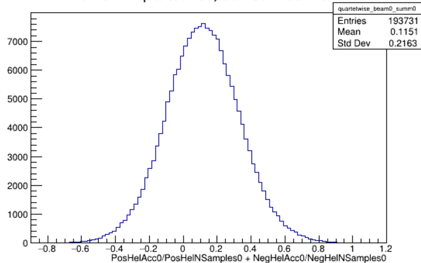
Run 5410 quartetwise, Sums0: Beam OFF
