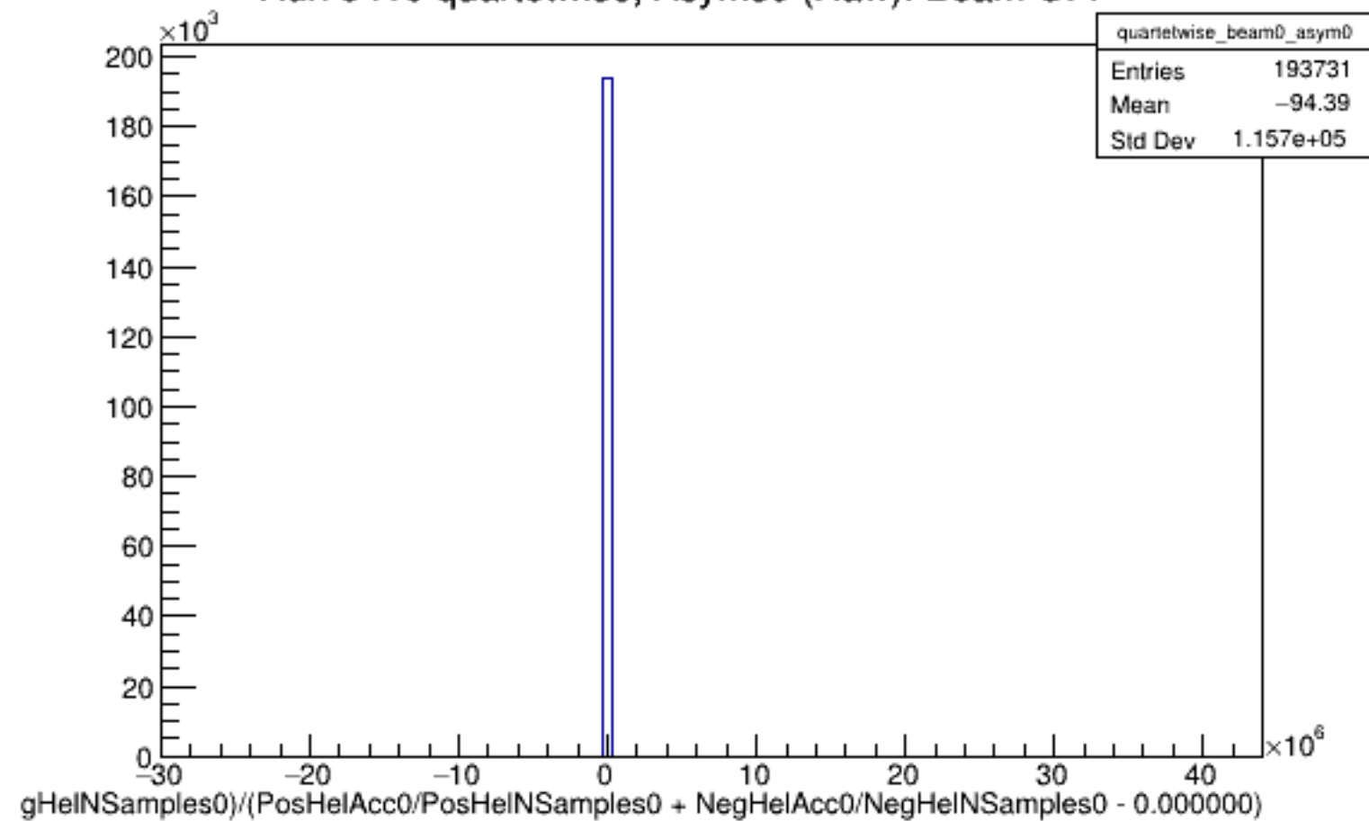
Run 5410 quartetwise, Asyms0 (Raw): Beam OFF
