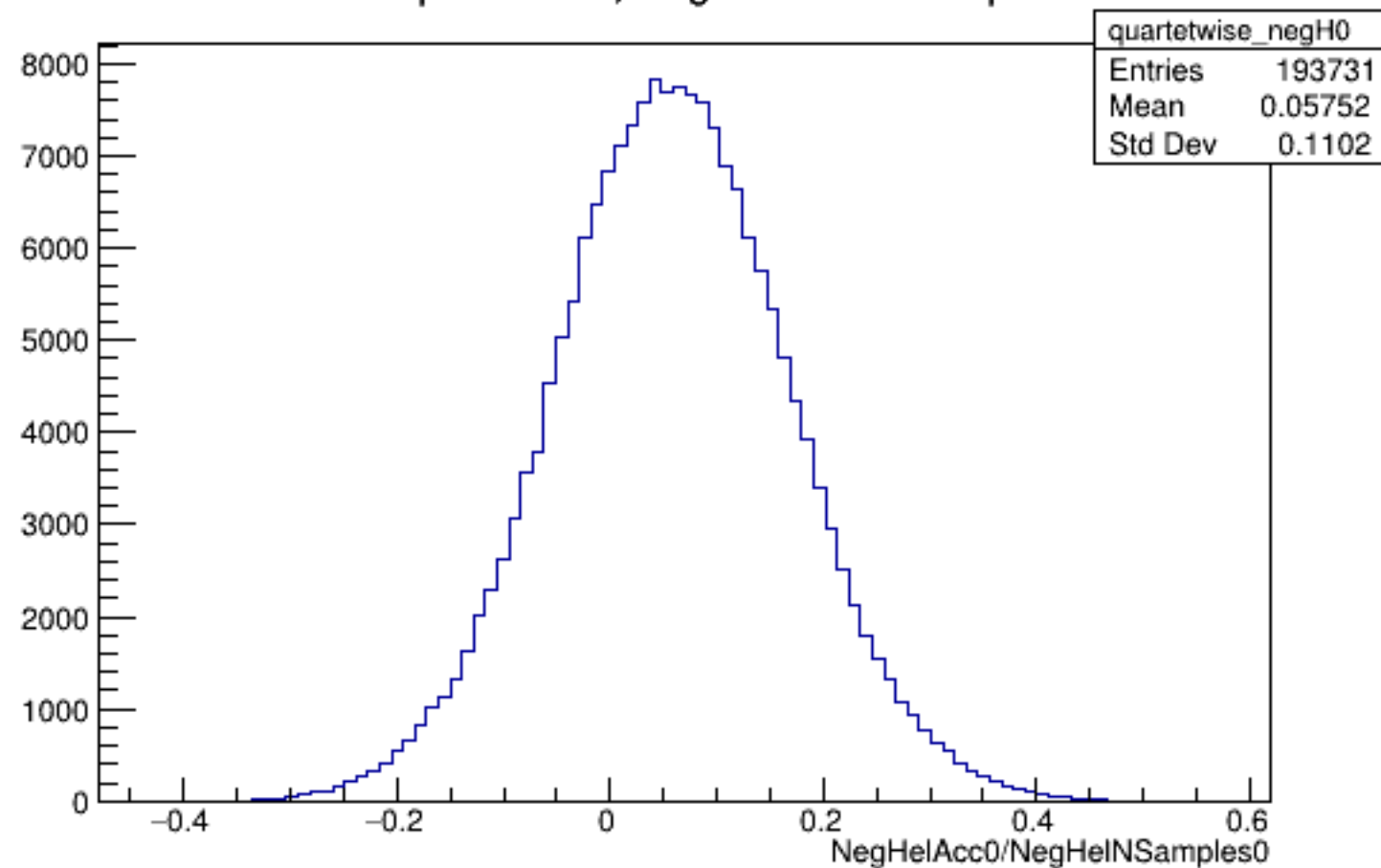
Run 5410 quartetwise, NegHelAcc0/NSamples0: All
