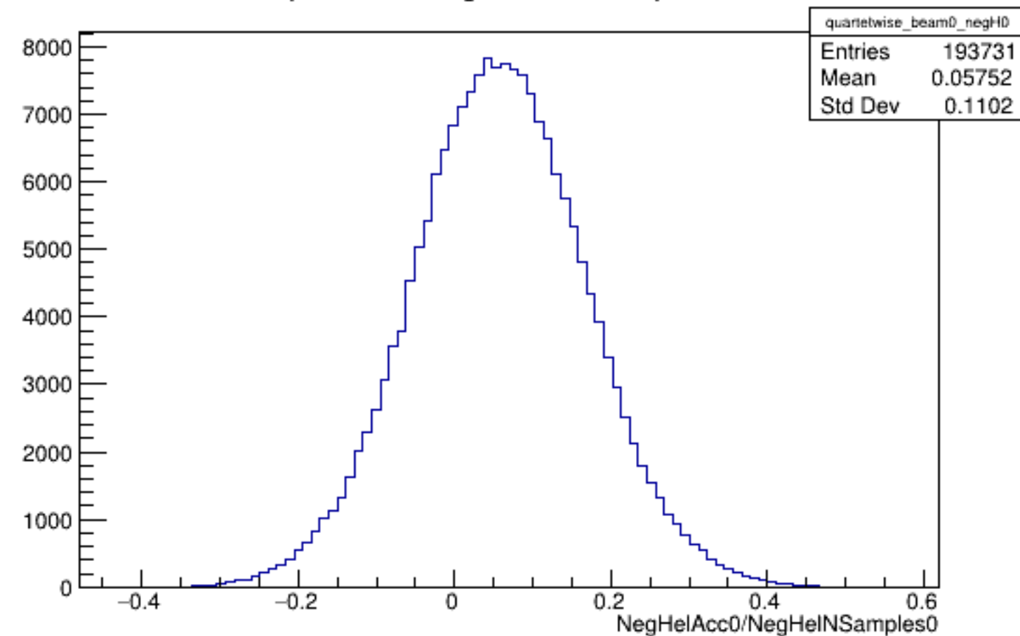
Run 5410 quartetwise, NegHelAcc0/NSamples0: Beam OFF
