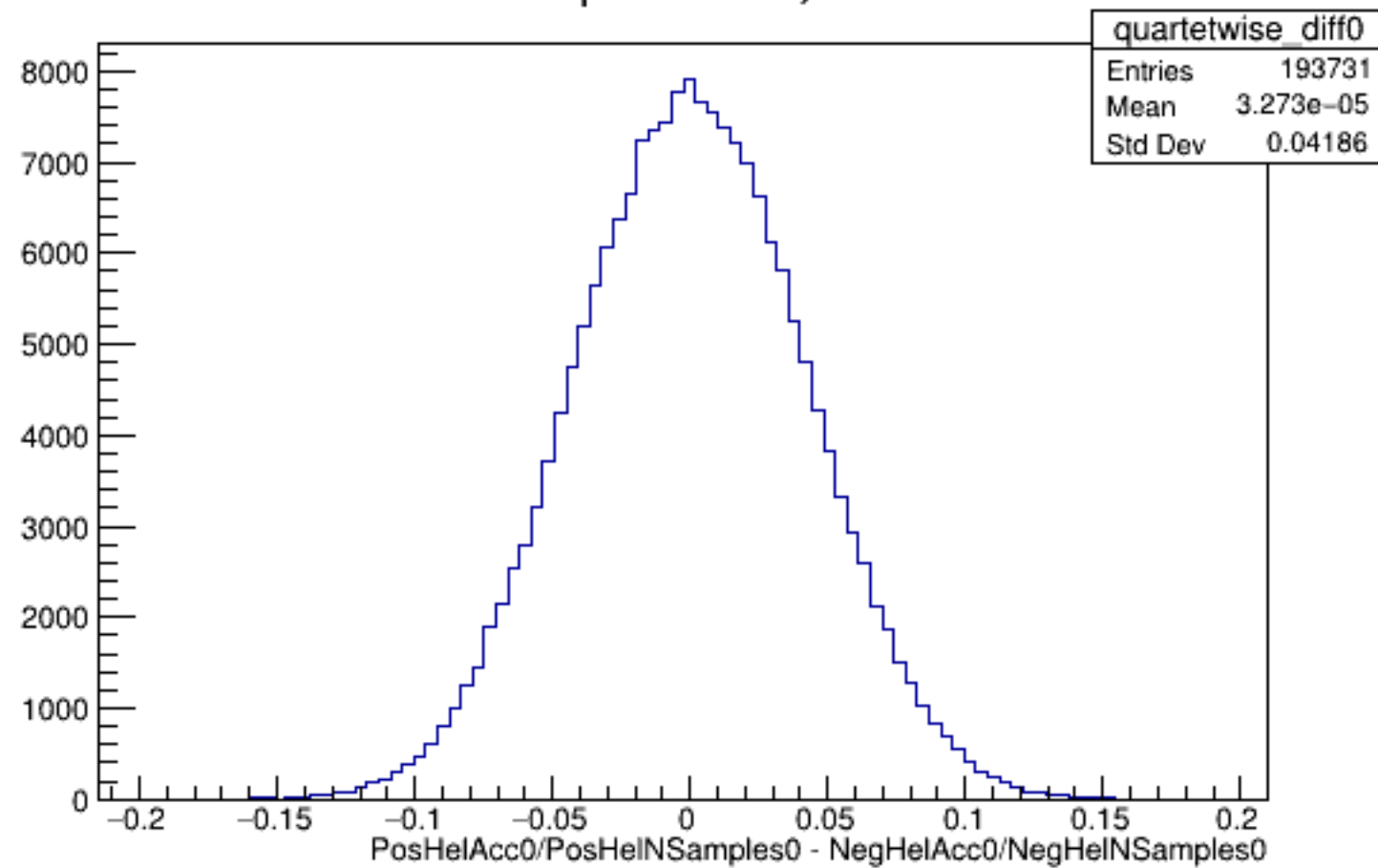
Run 5410 quartetwise, Diffs0: All
